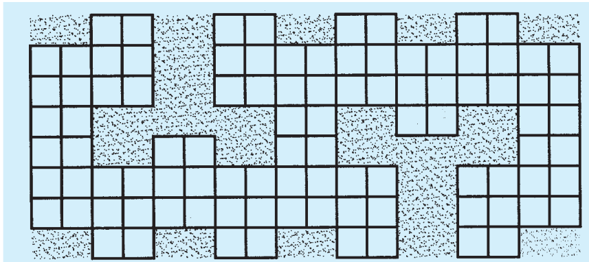
FIG. 7 OPEN CLUSTER
