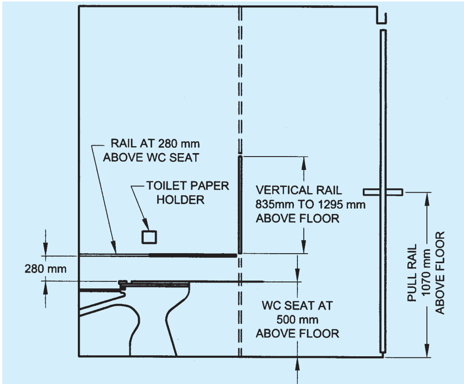
FIG. 20 SECTION THROUGH WC COMPARTMENT FOR THE AMBULANT DISABLED
