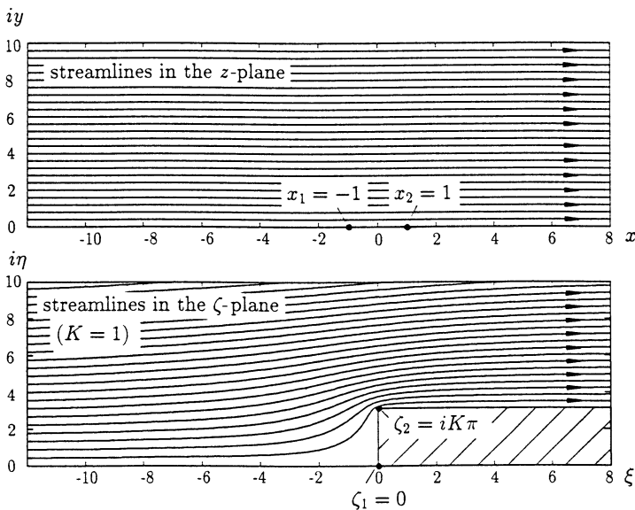
Fig. 10.38. Step in parallel flow
