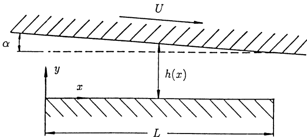
Fig. 8.1. Lubrication gap
