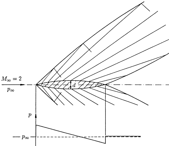
Fig. 11.23. Supersonic flow past an airfoil
