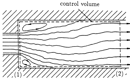
Fig. 9.7. Step expansion of the cross-section
