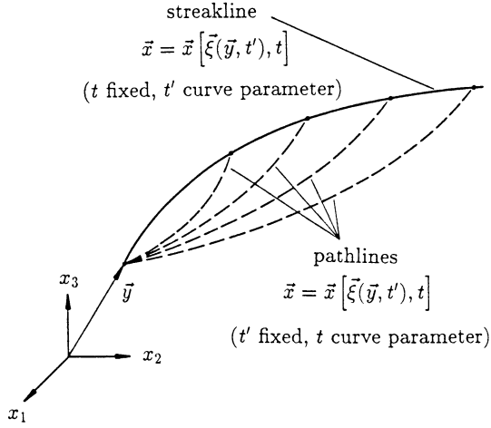
Fig. 1.5. Streaklines and pathlines
