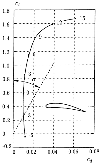
Fig. 10.50. Polar representation of lift and drag
