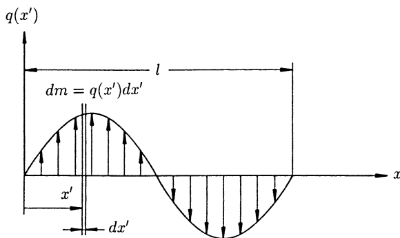
Fig. 10.13. Source distribution
