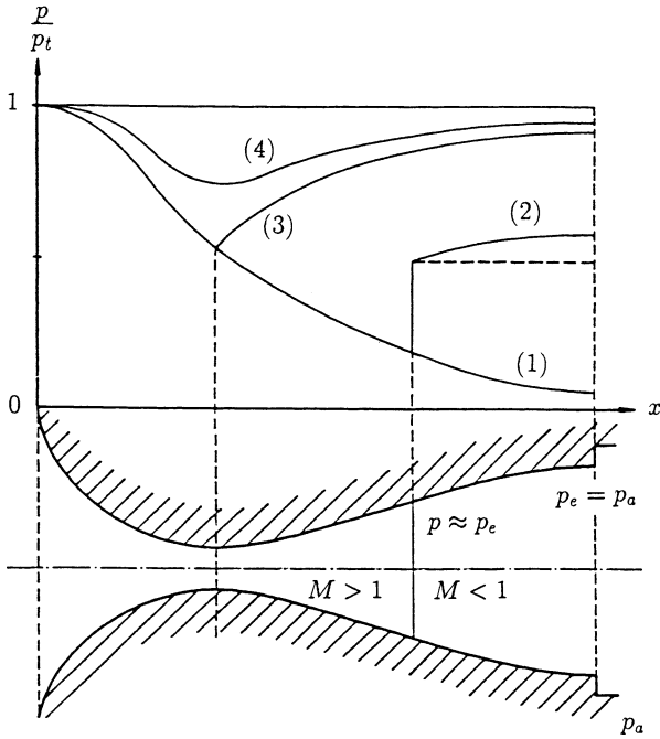
Fig. 9.15. Overexpanding nozzle
