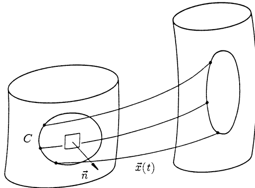
Fig. 4.23. Helmholtz's second vortex theorem
