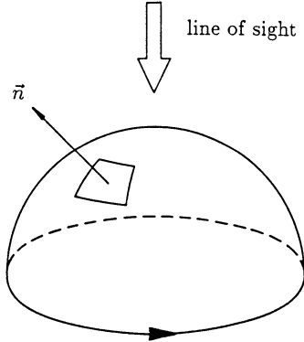
Fig. 4.10. Assigning the direction of integration in Stokes' integral theorem
