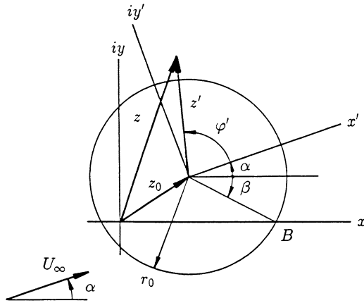
Fig. 10.46. Coordinate transformation
