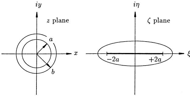
Fig. 10.43. Mapping of a circle onto a slit and ellipse
