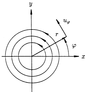
Fig. 10.25. Potential vortex
