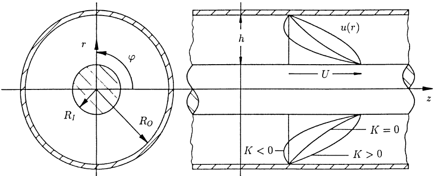
Fig. 6.7. Generalized Hagen-Poiseuille flow
