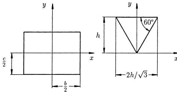
Fig. 6.8. Channels with rectangular and triangular cross-section
