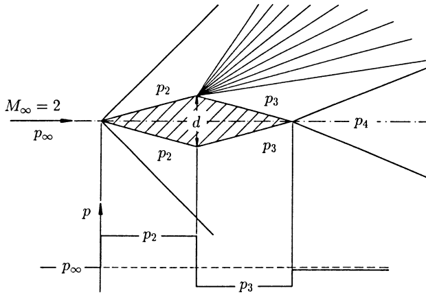
Fig. 11.22. Supersonic flow past a diamond airfoil
