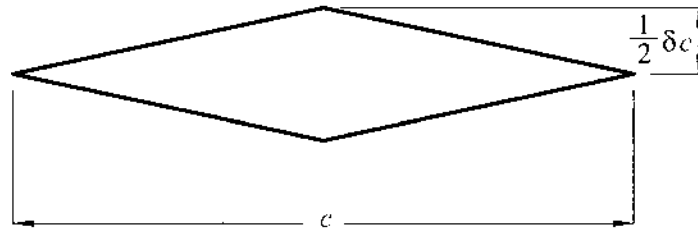
FIGURE 13.6 Double-wedge airfoil.
