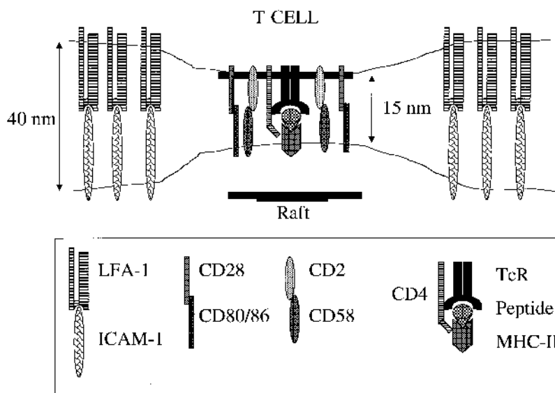
Fig. 4.7 Diagrammatic representation of the topography of T cell–APC cell interaction. In the areas where the T-cell receptors interact with peptide–MHC II complexes, the cells are in very close apposition. The rafts designate cholesterol-rich membrane domains in the T-cell membrane where the TcR, CD4, and other co-stimulating molecules interact with their respective ligands on in the APC. These interactions are primarily responsible for the close apposition of the T cell and APC membranes and for assembling the early signaling complex. Other molecules, such as LFA-1 and ICAM-1, stabilize the interaction between T cells and APCs and are present outside the rafts. (Adapted from Dustin, M. L. and Shaw, A. S. Science , 283:649–50, 1999.)
