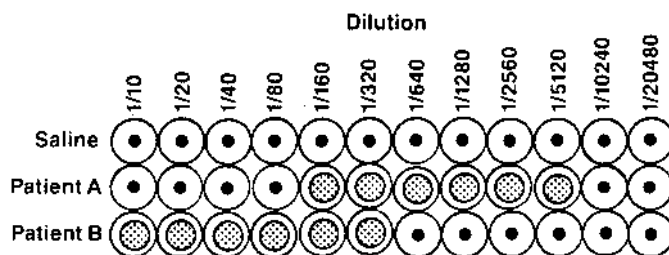
Fig. 8.9 Diagrammatic representation of a hemagglutination reaction performed in a microtiter plate. The objective of the study is to determine the existence and titer of hemagglutinating antibodies in three different samples. In the first step, each sample is sequentially diluted from 1/10 to 1/20480 in a separate row of wells (A,B,C). In a second step, a fixed amount of red cells is added to each serum dilution. In row A, no agglutination can be seen, and the sample is considered negative. In row B, the first three dilutions do not show agglutination (prozone), but of the next dilutions, up to 1/5120 are positive; this sample is positive, and the titer is 5120. In row C, the agglutination is positive until the 1/320 dilution; the titer of the sample is 320.
