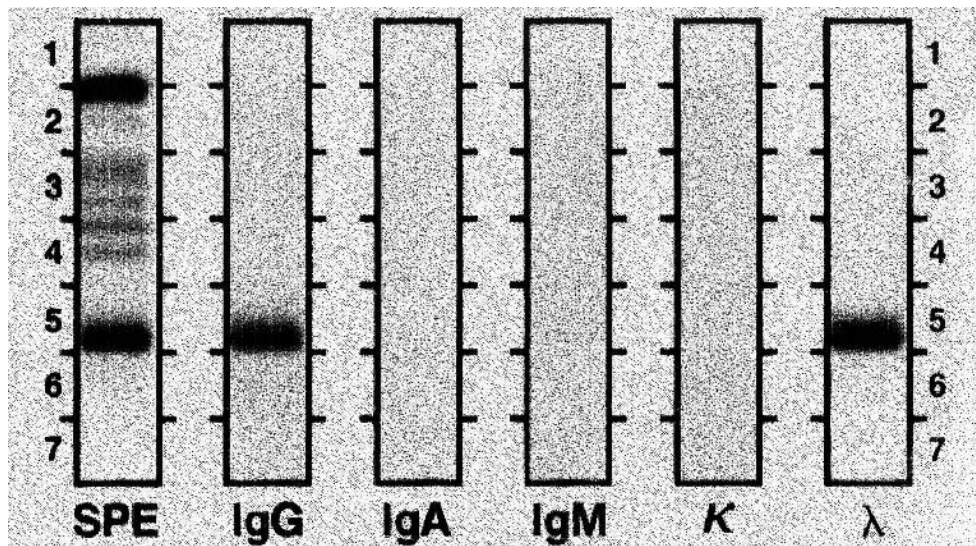
Fig. 27.3 Immunoblot of the serum protein of a patient with multiple myeloma. The lane labeled SPE was fixed and stained after electrophoresis and shows a homogeneous fraction in the gamma globulin region, near the bottom part of the separation region. The remaining lanes were blotted with the following antisera: anti-IgG, anti-IgA, anti-IgM, anti- \kappa chains, and anti- \lambda chains. Notice that the antisera specific for IgG and for \lambda chains reacted with the homogeneous fraction, which therefore was identified as an IgG \lambda monoclonal protein. (Immunoblot courtesy of Dr. Sally Self, Department of Pathology and Laboratory Medicine, Medical University of South Carolina.)
