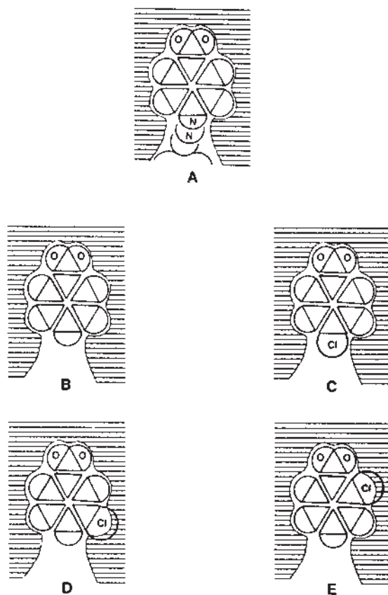
Fig. 8.1 Diagrammatic representation of the “closeness of fit” between antigenic determinants and antibody binding sites. Antibodies were raised against the p -azobenzoate group of a protein- p -benzoate conjugate. The resulting anti- p -benzoate groups react well with the original protein- p -benzoate conjugate (A) and with p -benzoate itself (B). If a chlorine atom (Cl) is substituted for a hydrogen atom at the p position, the substituted hapten will react strongly with the original antibody (C). However, if chlorine atoms are substituted for hydrogen atoms at the o or m positions (D,E), the reaction with the antibody is disturbed, since the chlorine atoms at those positions cause a significant change in the configuration of the benzoate group. (Redrawn from Van Oss, C. J. In: Principles of Immunology , 2nd ed. (N. Rose, F. Milgrom, and C. Van Oss, eds.). McMillan, New York, 1979.)
