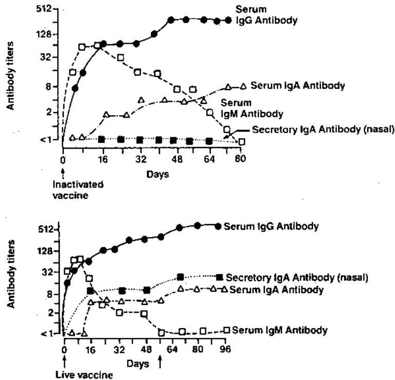
Fig. 12.4 Comparison of the systemic and mucosal immune responses in human volunteers given killed polio vaccine (top) and live, attenuated polio vaccine (bottom). Note that secretory antibody was only detected in children immunized with live, attenuated vaccine. (Modified from Ogra, P. L., Karzon, D. T., Roghthand, F., and MacGillivray, M. N. Engl. J. Med. 279:893, 1968.)
