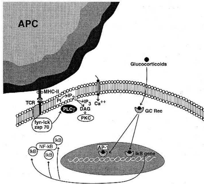
Fig. 24.1 Diagrammatic representation of the mechanism of action responsible for the downregulation of cytokine synthesis by glucocorticoids. Once internalized in the cytoplasm, glucocorticoids combine with their receptor and the complex is translocated to the nucleus, where it interacts with the nuclear binding protein AP-1, preventing its interaction with cytokine gene enhancers and with a glucocorticoid-responsive element that upregulates the expression of the I \kappa B gene. The excess of I \kappa B protein prevents the activation of NF- \kappa B, another nuclear binding protein, which normally activates the expression of cytokine genes (see Chapters 4 and 11).
