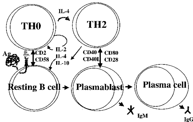
Fig. 11.6 Diagrammatic representation of the sequence of signals and interactions between T_H cells and B cells taking place at the onset of an immune response. The B lymphocyte receives activating signals from the occupancy of the binding sites of membrane immunoglobulin and by the interaction of antigen-associated C3d with CD21. Other models could involve initial B-cell interaction with a professional APC presenting membrane-associated antigen in the context of co-stimulation. The B lymphocyte, having ingested and processed the antigen that was bound to the surface immunoglobulin, later presents MHC-I-associated peptides to a T_H0 lymphocyte. This triggers the initial activation sequence of the T_H0 cells that involves synthesis of IL-2 and IL-4 (the latter becoming predominant) and upregulation of CD40 and of the “active” form of CD2 (CD2R). The upregulation of these membrane molecules allows mutual activation of the interacting cells. The nature of earlier co-signals that determine the initial shift towards IL-4 synthesis has not been defined, but once IL-4 starts to predominate it determines differentiation of CD4^+ T lymphocytes with T_H2 activity. At that later stage both cells express a full complement of membrane proteins, cytokines, and cytokine receptors, involved in the delivery of co-stimulating signals that will cause the proliferation and differentiation of both types of cells. Interactions involving CD40 and CD80/86 on B lymphocytes and CD40L and CD28 on T lymphocytes is essential for further progression of the response.
