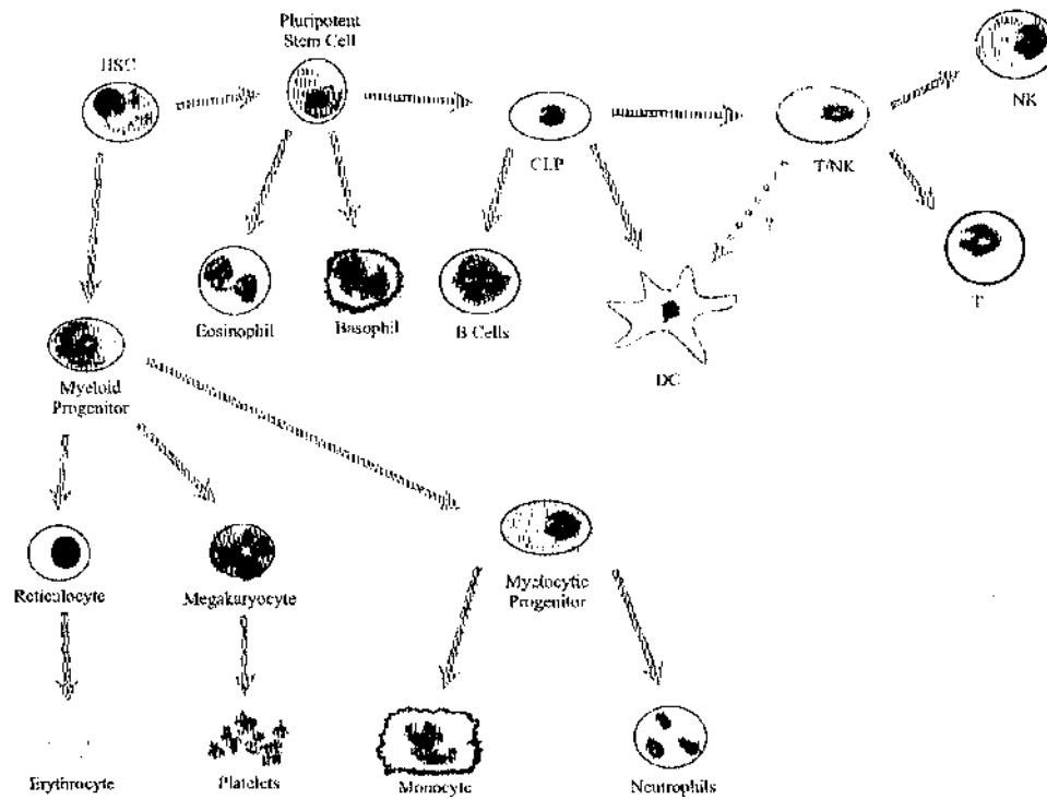
Fig. 10.1 Hypothetical model of hematopoietic stem cell differentiation. Multipotential hematopoietic stem cells (HSC) give rise to more restricted progenitor cells with self-renewal capacity. The common lymphoid progenitor cells (CLP) give rise to T, B, NK, and DC lymphocytes. Another group of hematopoietic cells, for which the immediate progenitor is a more differentiated myeloid progenitor (MP), includes erythrocytes, megakaryocytes, and platelets as well as the granulocyte, monocyte/macrophage series. (The assistance of Christopher J. Lada in the preparation of this figure is gratefully acknowledged.)
