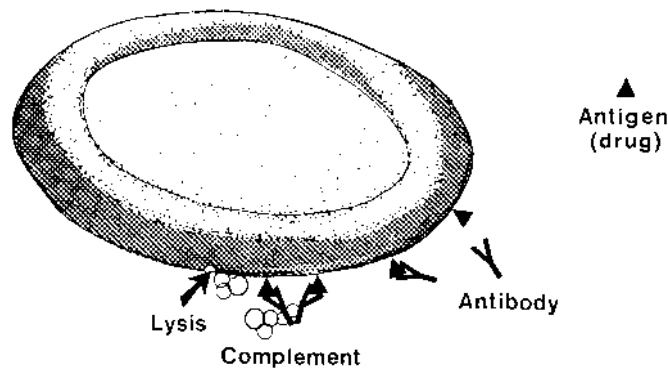
Fig. 22.3 Diagrammatic representation of the pathogenesis of drug-induced hemolytic anemia as a consequence of adsorption of a drug to the red cell membrane.
