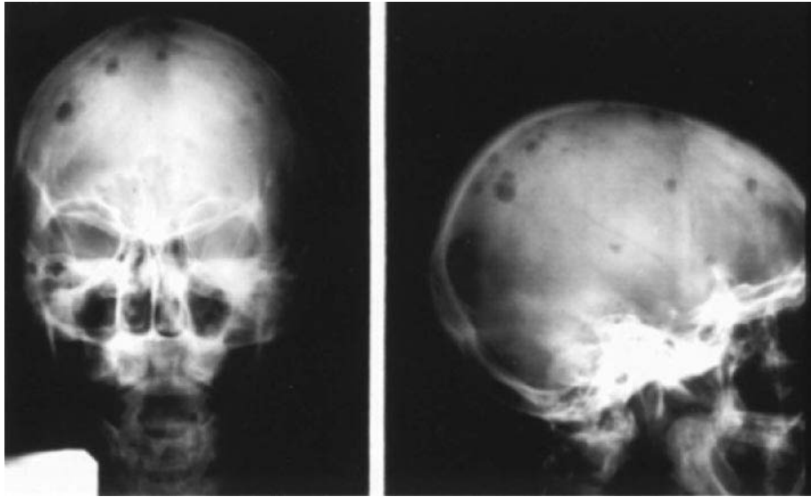
Fig. 27.6 X-ray of the skull of a patient with multiple myeloma showing typical osteolytic lesions. (Courtesy of Dr. S. Richardson.)
