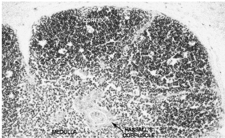
Fig. 2.6 Morphology of a thymic lobe. The densely packed cortex is mostly populated by T lymphocytes and by some cortical dendritic epithelial cells and cortical epithelial cells. The more sparsely populated medulla contains epithelial and dendritic cells, macrophages, T lymphocytes, and Hassell's corpuscles. (Image courtesy of Professor Robert W. Ogilvie, Department of Cell Biology and Anatomy, Medical University of South Carolina.)
