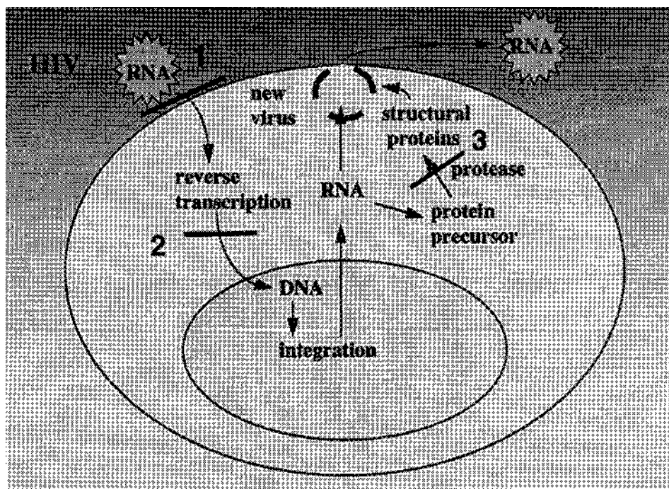
Fig. 30.3 Diagrammatic representation of the HIV life cycle and the points of action of antiretroviral agents. The first antiretrovirals introduced were the reverse transcriptase inhibitors, which block the first step of viral replication after the virus has penetrated into a competent cell (2). The next generation of antiretrovirals was the protease inhibitors, which prevented the processing of viral proteins, a step essential for the assembly of viral progeny (3). Agents able to prevent the penetration of HIV into competent cells (1) are currently being evaluated.
