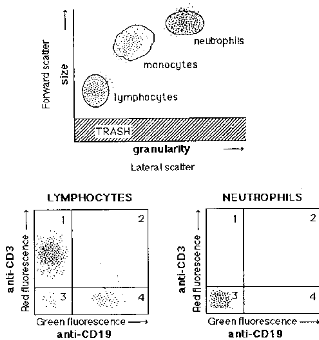
Fig. 15.13 Diagrammatic representation of the data processing sequence in flow cytometry. The top drawing illustrates a plot of forward vs. lateral light scattering of peripheral blood mononuclear cells. Three leukocyte populations can be segregated by their size and granularity: neutrophils (the largest and most granular), monocytes, and lymphocytes (the smallest and less granular). The lines surrounding these populations correspond to “gating,” i.e., instructing the computer to process separated data from these three populations. The two lower graphs represent analysis of fluorescence for two of the leukocyte populations. The lymphocytes can be separated into two different subpopulations: those reacting with rhodamine-labeled anti-CD3 antibodies, which emit red fluorescence and correspond to T lymphocytes, and those that treat with fluorescein-labeled anti-CD19, which emits green fluorescence and corresponds to B lymphocytes. The analysis of neutrophils shows lack of reactivity with both antisera.
