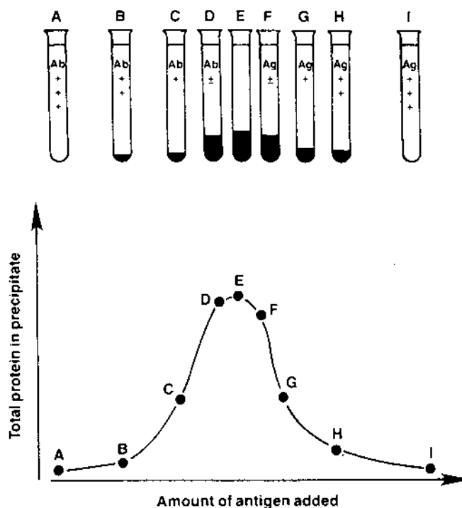
Fig. 8.5 The precipitin curve. When increasing amounts of antigen are added to a fixed concentration of antibody, increasing amounts of precipitate appear as a consequence of the antigen-antibody interaction. After a maximum precipitation is reached, the amounts of precipitate begin to decrease. Analysis of the supernatants reveals that at low antigen concentrations there is free antibody left in solution (antibody excess); at the point of maximal precipitation, neither antigen nor antibody are detected in the supernatant (equivalence zone); with greater antigen concentrations, antigen becomes detectable in the supernatant (antigen excess).
