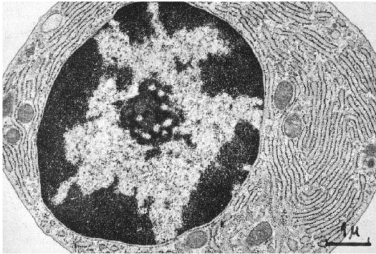
Fig. 6.1 Ultrastructure of a mature plasma cell. Note the eccentric nucleus with clumped chromatin, the large cytoplasm containing abundant, distended, endoplasmic reticulum. (Electron microphotograph courtesy of Professor P. Groscurth, M. D., Institute of Anatomy, University of Zurich, Switzerland.)
