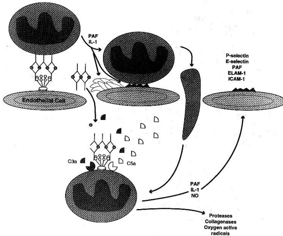
Fig. 23.3 The initial stages of circulating immune complex deposition require a sequence of events that enables circulating IC and inflammatory cells to cross the endothelial barrier. In this representation of such a hypothetical sequence, the first event is the binding of circulating IC containing IgG antibodies and associated C1q to C1q receptors on the endothelial cell. The immobilized IC are then able to interact with circulating cells expressing Fc \gamma receptors, such as PMN leukocytes. Such interaction results in PMN activation and release of mediators, such as platelet-activating factor (PAF) and IL-1. These two mediators have a variety of effects: PAF induces vasodilatation and activates platelets, which form aggregates and release vasoactive amines. The resulting increased vascular permeability allows circulating IC to cross the endothelial barrier. IL-1 activates endothelial cells and induces the expression of selectin molecules that interact with glycoproteins and sialoglycoproteins on the leukocyte membrane. This interaction slows down PMNs along the endothelial surface, a phenomenon known as “rolling.” As endothelial cells continue to receive activating signals, they start expressing membrane-associated PAF, which interacts with PAF receptors on neutrophils, ICAM-1, which interacts with leukocyte integrins of the CD11/CD18 family, and VCAM-1, which interacts with VLA (very late antigen)-1, upregulated on PMN leukocytes as a consequence of the occupancy of Fc receptors. This promotes firm adhesion of leukocytes to endothelial cells. At the same time the IC that diffuse to the subendothelial space activate complement and generate chemotactic factors, such as C5a and C3a. Adherent PMN leukocytes are attracted to the area and insinuate themselves between endothelial cells, reaching the area of IC deposition. Interaction with those extravascular IC with associated C3b delivers additional activation signals to already primed granulocytes, resulting in the release of metalloproteinases (including proteases and collagenases), oxygen active radicals, and nitric oxide. These compounds can cause tissue damage and can further increase vascular permeability, and in doing so contribute to the perpetuation of an inflammatory reaction.
