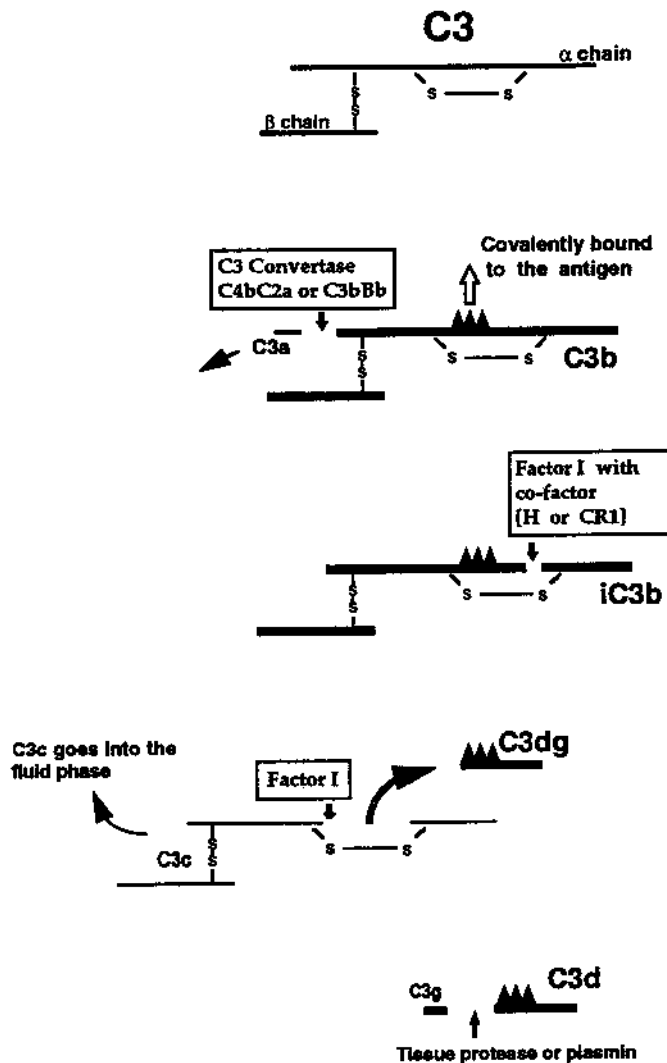
Fig. 9.7 Diagrammatic summary of the different steps involved in C3 inactivation.
