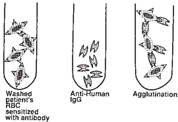
Fig. 22.1 Diagrammatic representation of a direct Coombs' test using anti-IgG antibodies.
