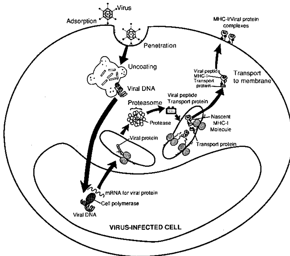
Fig. 4.9 Diagrammatic representation of the general steps involved in the presentation of viral-derived peptides on the membrane of virus-infected cells. The virus binds to membrane receptors and is endocytosed, its outer coats are digested, and the viral genome (in this case DNA) is released into the cytoplasm. Once released, the viral DNA diffuses back into the nucleus, where it is initially transcribed into mRNA by the cell's polymerases. The viral mRNA is translated into proteins that diffuse into the cytoplasm, where some will be broken down into oligopeptides. Those small peptides are transported back into the endoplasmic reticulum where they associate with newly synthesized MHC-I molecules. The MHC-I-oligopeptide complex becomes associated to a second transport protein and is eventually inserted into the cell membrane. In the cell membrane, it can be presented to CD8^+ T lymphocytes in traffic through the tissue where the viral infected cell is located. A similar mechanism would allow a MHC-II-synthesizing cell to present MHC-II/oligopeptide complexes to CD4^+ lymphocytes.
