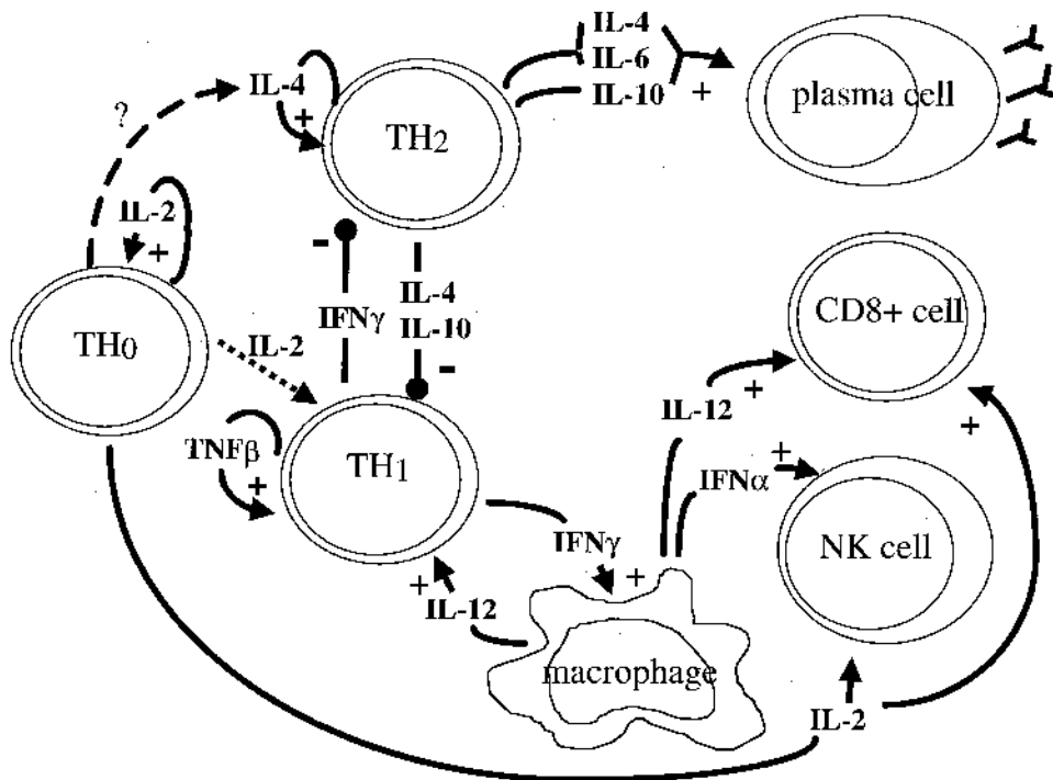
Fig. 11.5 Diagrammatic representation of the cytokine repertoire and functions of T_H1 and T_H2 helper lymphocyte subpopulations.
