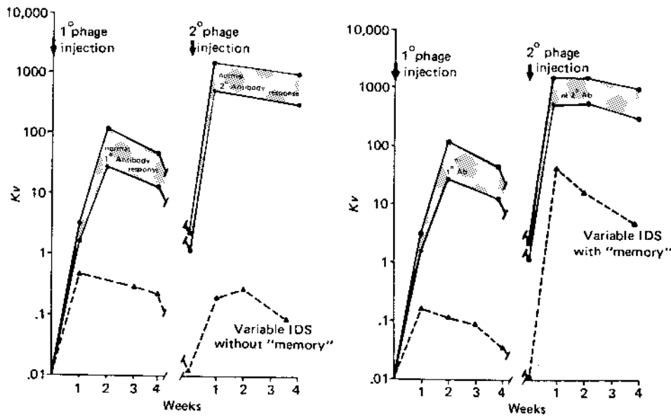
Fig. 28.2 Primary and secondary responses to bacteriophage ØX 174 in a patient with a variable immunodeficiency syndrome. The shaded area between the solid lines indicates the range for normal responses. The patient's response is the interrupted line. The patient studied on the left panel showed a definite but diminished antibody response; the secondary response was not greater than the primary—no memory/amplification occurred. The immunoglobulin class of antibody in both primary and secondary responses was entirely IgM. The patient studied on the right panel showed greater response to secondary immunization than to primary (memory/amplification) although both were diminished in comparison to the normal range. The immunoglobulin class of the secondary response was entirely IgM. (Reproduced with permission from Wedgewood, Ochs, and Davis, Birth Defects: Original Article Series 11:331 , 1975.)
