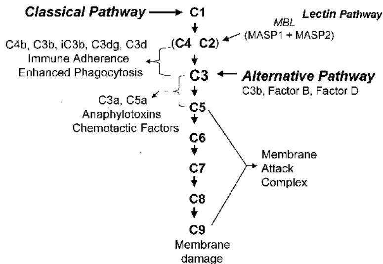
Fig. 9.9 The sequence of complement activation.
