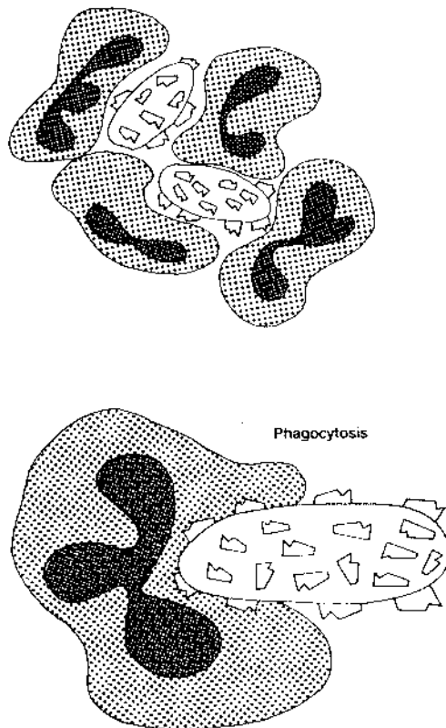
Fig. 9.6 Opsonization and phagocytosis. The top panel shows immune adherence of phagocytic cells to antigenic cells coated with antibody and complement, and the bottom panel illustrates the ingestion (phagocytosis) of an opsonized cell.
