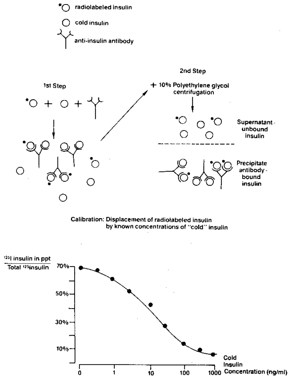
Fig. 15.14 Diagrammatic representation of the general principles of competitive radioimmunoassay in fluid phase. In this type of assay (e.g., insulin level assay), the free and antibody-bound antigens are separated either by physicochemical techniques, as shown in the diagram, or by using a second antibody (anti-immunoglobulin) to precipitate the insulin-antibody complexes formed in the first step of the assay.
