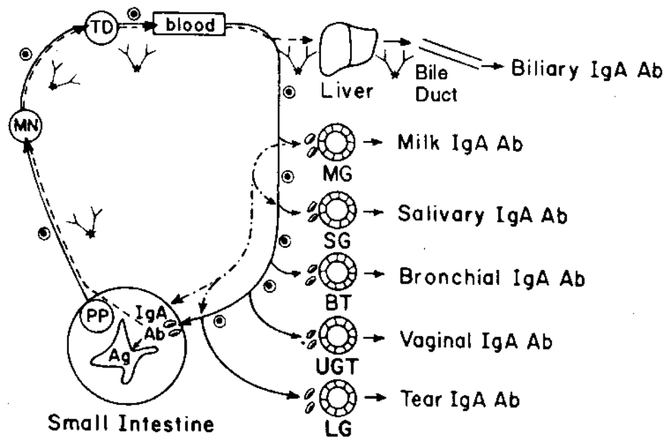
Fig. 12.5 Diagrammatic representation of the pathways leading to the expression of IgA antibodies after antigenic stimulation of the GALT. IgA immunocytes (*) originating in Peyer's patches (PP) migrate to mesenteric lymph nodes (MN). Cells leave MN via the thoracic duct (TD) and enter circulation with subsequent homing to the mammary gland (MG), salivary gland (SG), lacrimal gland (LG), and the lamina propria of the bronchial tree (BT), intestinal or urogenital tract (UGT) (*). The IgA antibodies are then expressed in milk, saliva, tears, and other secretions. IgA antibodies (---) entering circulation (---) are selectively removed by the liver and subsequently expressed in bile. Cell traffic between peripheral mucosal sites (- • - MG to SG, LG, and small intestine) is included in this scheme. (Reproduced with permission from Montgomery, P. C., Stander, C. A., and Majumdar, A. S. Evidence for migration of IgA bearing lymphocytes between peripheral mucosal sites. In Protides of the Biological Fluids , H. Peeters, ed. Pergamon, New York, 1985, p. 43.)
