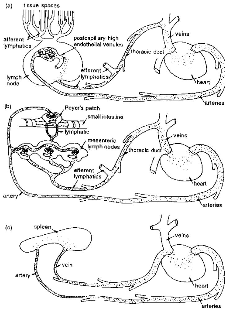
Fig. 2.9 Pathways of lymphocyte circulation: (a) blood lymphocytes enter lymph nodes, adhere to the walls of specialized postcapillary venules, and migrate to the lymph node cortex. Lymphocytes then percolate through lymphoid fields to medullary lymphatic sinuses and on to efferent lymphatics, which in turn collect in major lymphatic ducts in the thorax, which empty into the superior vena cava; (b) the gut-associated lymphoid tissues (Peyer's patches and mesenteric lymph nodes) drain into the thoracic duct, which also empties into the superior vena cava; (c) the spleen receives lymphocytes and disburses them mainly via the blood vascular system (inferior vena cava). (Reproduced with permission from Hood, L. E., Weissman, I. L., Wood, W. B., and Wilson, J. H. Immunology , 2nd ed. Benjamin/Cummings, Menlo Park, CA, 1984.)
