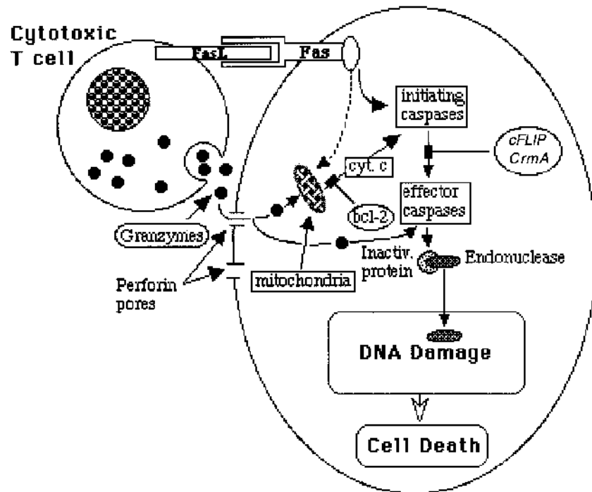
Fig. 11.8 Diagrammatic representation of the sequence of events leading to apoptosis of a target cell after interaction with an activated cytotoxic T lymphocyte. Two pathways leading to activation of a critical initiator caspases have been described: one involves the interaction between Fas and FasL, an interaction that activates caspase 8. The other involves granzymes, released by the T lymphocyte and diffused into the cytoplasm through polyperforin clusters. Granzymes can trigger apoptosis either by activating directly terminal caspases or by inducing increased mitochondrial permeability, followed by release of cytochrome c and other caspase activators. The activation of terminal caspases is followed by denaturation of an inactivating protein complexed with a cytoplasmic endonuclease. The activated endonuclease translocates to the nucleus, where it causes DNA breakdown, the hallmark of apoptosis. Two levels of control appear to exist: One, controlling mitochondrial permeability, is regulated by a member of the Bcl-2 proto-oncogene family. The other, blocking the pathway between initiator and effector caspases, involves Crma , the product of a cytokine response modifier gene, and cFLIP .
