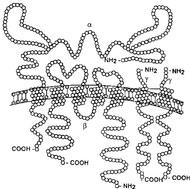
Fig. 21.5 Diagrammatic representation of the primary structure of the Fc_{\epsilon} -RI. (Modified from Metzger, H. Clin. Exp. Allergy 21:1, 1991.)
