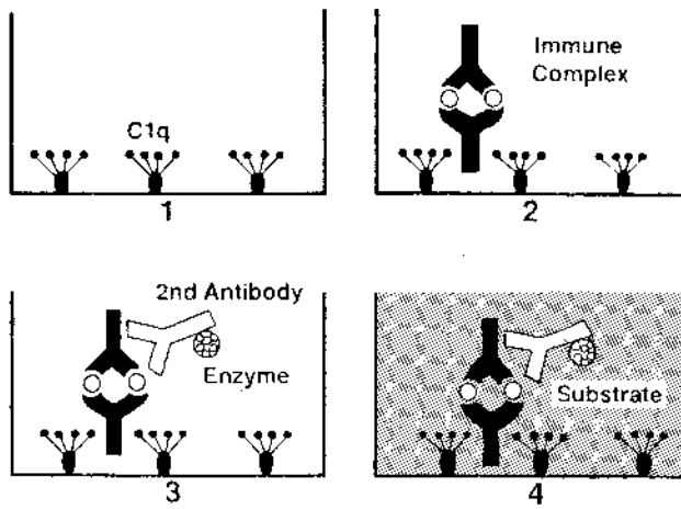
Fig. 23.7 Diagrammatic representation of the principle of the solid-phase C1q binding assay. Purified C1q is immobilized by adsorption to a solid phase. IC containing IgG antibodies will bind to the immobilized C1q. After washing off unbound proteins, an enzyme-labeled anti-IgG antibody is added to the solid phase. This antibody will bind to the immobilized immune complexes. After washing off unbound, labeled antibody, a colorless substrate will be added to the solid phase. The substrate is broken down into a colored compound, and the intensity of the color is directly proportional to the concentration of labeled antibody bound to the solid phase, which in turn is proportional to the concentration of IC bound to C1q.
