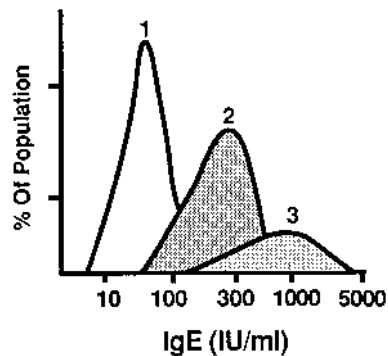
Fig. 21.3 Distribution of IgE levels in a population of nonallergic individuals. Three subpopulations appear to exist: one constituted by low-responder individuals (1), one by high-responder individuals (3), and a third population of individuals with intermediate levels of IgE (2).
