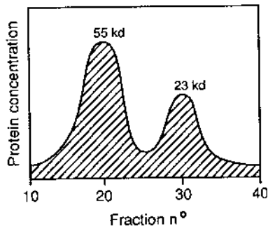
Fig. 5.3 Gel filtration of reduced and alkylated IgG (MW 150,000) on a dissociating medium. Two protein peaks are eluted, the first corresponding to a MW of 55,000 and the second corresponding to a MW of 23,000. The 2:1 ratio of protein content between the high and low molecular weight peaks is compatible with the presence of identical numbers of two polypeptide chains, one of which is about twice as large as the other.
