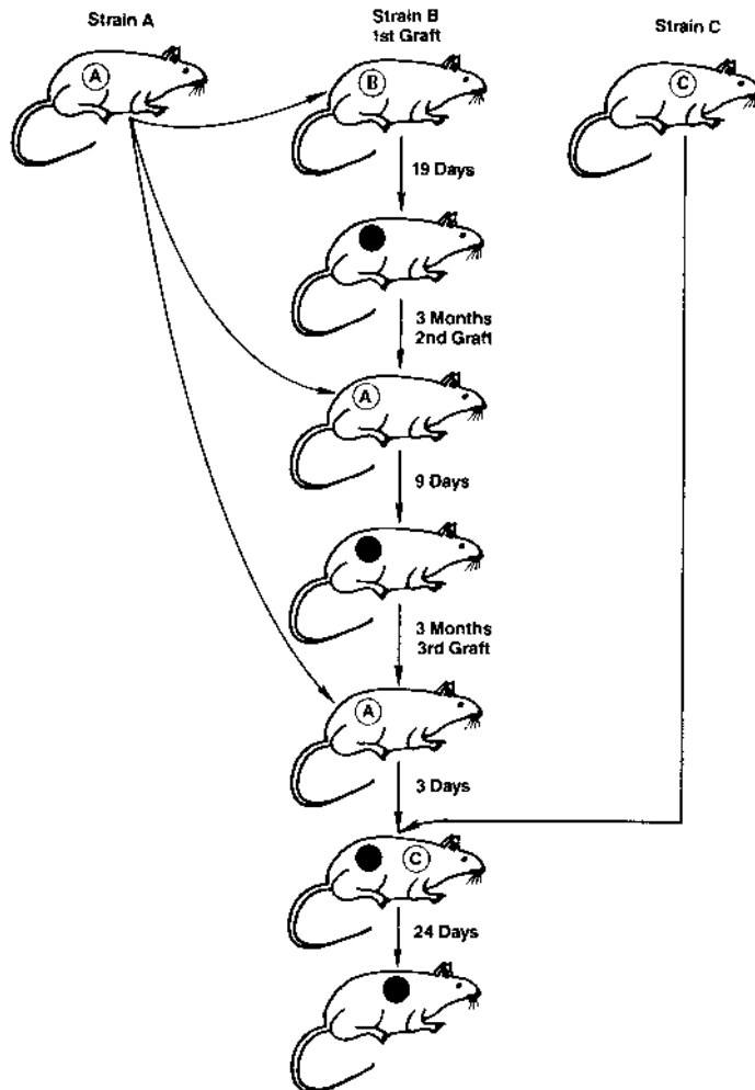
Fig. 3.1 Diagrammatic representation of an experiment designed to demonstrate the memory and specificity of graft rejection. Memory is demonstrated by the progressive shortening of the time it takes a mouse of strain B to reject consecutive skin grafts from a strain A. Specificity is demonstrated by the fact that the mouse of strain B is already able to reject a graft from strain A in an accelerated fashion, and if given a graft from a third, unrelated strain (C), rejection will take as long as the rejection of the first graft from strain A. In other words, sensitization of mouse B to strain A was strain-specific and did not extend to unrelated strains.
