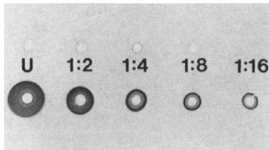
Fig. 15.2 The principle of radial immunodiffusion. Five wells carved into antibody-containing agar were filled with serial dilutions of the corresponding antigen. The antigen diffused, reacted with antibody in the agar, and eventually precipitated in a circular pattern. The diameters or areas of these circular precipitates are directly proportional to the concentration of antigen in each well.
