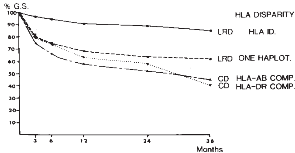
Fig. 25.1 Cumulative graft survival of living related donor (LRD) and cadaveric donor (CD) transplants. (Reproduced with permission from Flatmark and Thorsby, Transplant. Proc. 14:61, 1982.)
