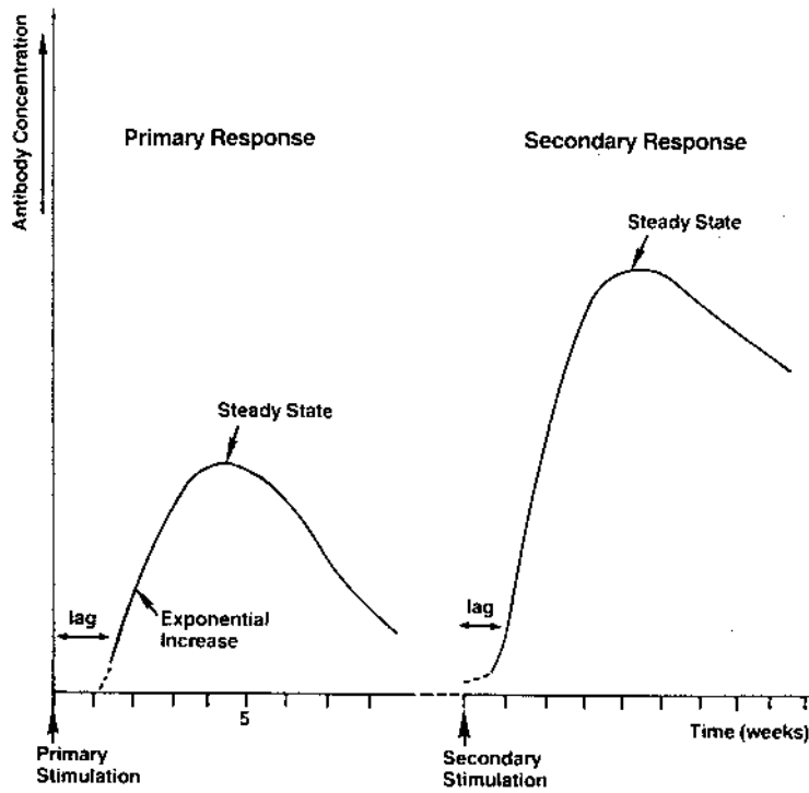
Fig. 12.1 Diagrammatic representation of the sequence of events during a primary and a secondary immune response. (Modified from Eisen, H. N. Immunology , 2nd ed. Harper & Row, Cambridge, 1980.)
