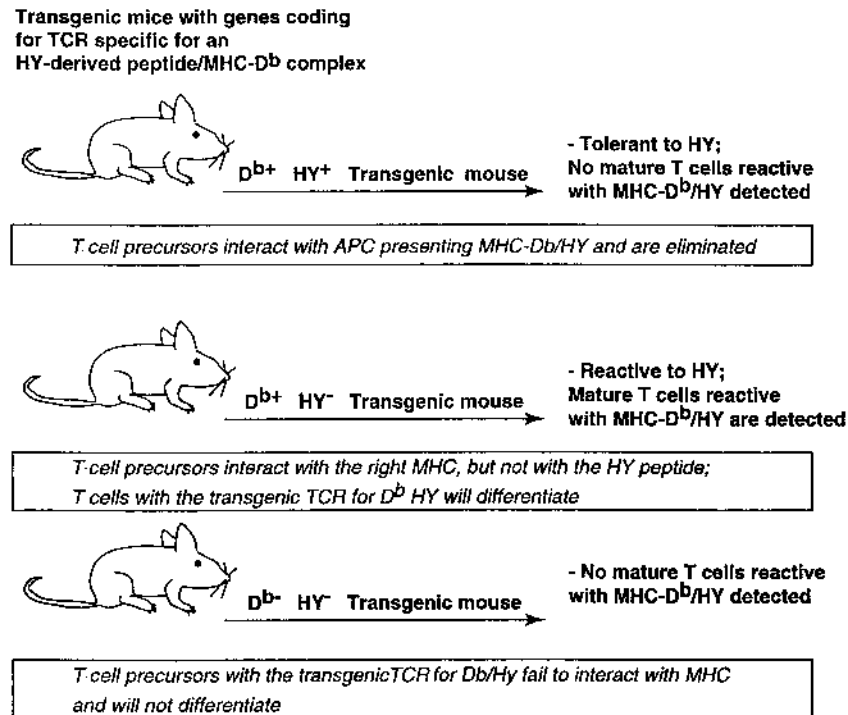
Fig. 16.2 Diagrammatic representation of an experiment in which transgenic animals expressing a TcR specific for an HY-derived peptide–MHC-D b complex were shown to become tolerant to the HY peptide, but only in D b+ animals. The tolerance in this model was apparently due to clonal deletion, since no mature T cells reactive with MHC-D b /HY were detected in the tolerant animals.
