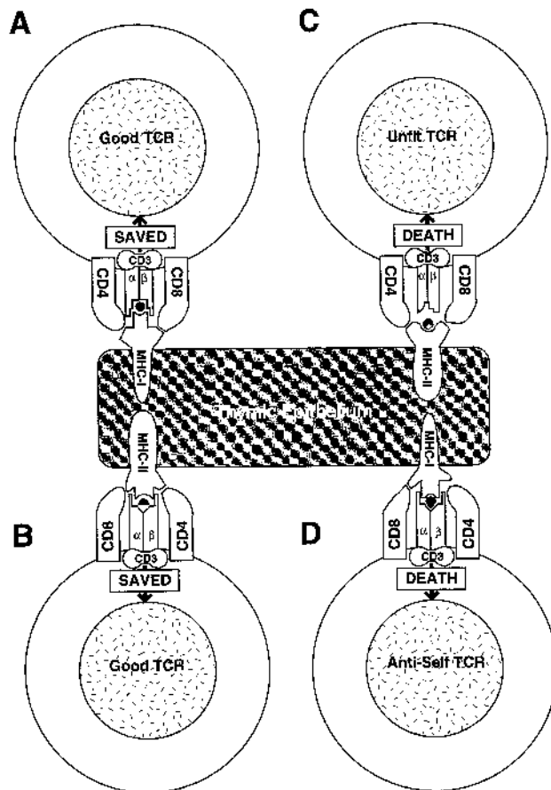
Fig. 10.9 Diagrammatic representation of the role played by MHC in clonal selection during intrathymic lymphocyte differentiation. TcR2 + pre-T lymphocytes, which co-express CD4 and CD8, interact with self-MHC class I and class II expressed on the thymic epithelium. (A) In this example, the TcR2 + has a good fit with self-MHC class I, the CD8 molecule also interacts with the MHC-I, but the TcR does not interact with a self peptide associated with the MHC-I molecule. The dual interaction between CD8 and TcR with MHC-I will deliver a positive signal, transduced by the CD3, which will rescue the lymphocyte from programmed death. At the same time, the gene coding for the CD4 molecule, which did not interact with the MHC-I, will be repressed. Thus, a CD8 + T lymphocyte clone will emerge from this positive selection process. (B) In this second example, the TcR2 + has a good fit with self-MHC class II, the CD4 molecule also interacts with MHC-II, but the TcR does not interact with a self peptide associated with the MHC-II molecule. This lymphocyte will be rescued from programmed death by a positive signal transmitted by the CD3, and since the CD8 molecule did not interact with the MHC, its expression will be repressed. Thus, a CD4 + T lymphocyte clone will emerge from the selection process. (C) If the TcR2 does not interact either with class I or class II MHC, that T cell does not receive any positive signal from CD3 and dies as programmed. (D) In this final example, a self-reactive pre-T cell is depicted. Its TcR interacts with MHC-I and with the self peptide associated with it. This results in a high-affinity interaction between the lymphocyte and the thymic epithelium that accelerates the process of apoptosis, thus eliminating the autoreactive lymphocyte. This process of negative selection can eliminate both CD8 + and CD4 + autoreactive cells.
