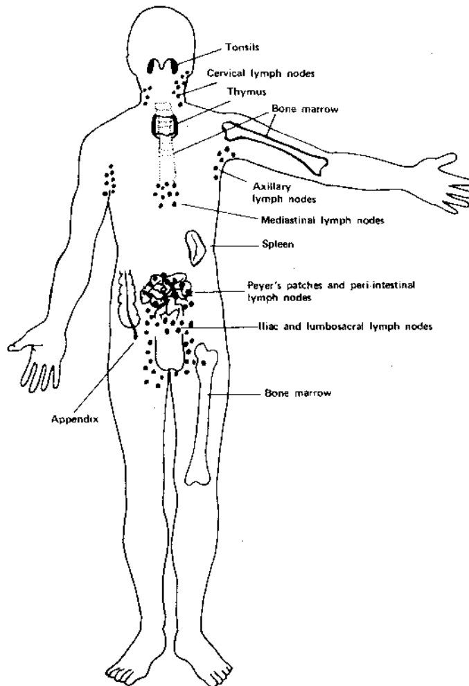
Fig. 2.3 Diagrammatic representation of the distribution of lymphoid tissues in humans. (Modified from Mayerson, H. S. Sci. Am. , 208:80, 1963.)
