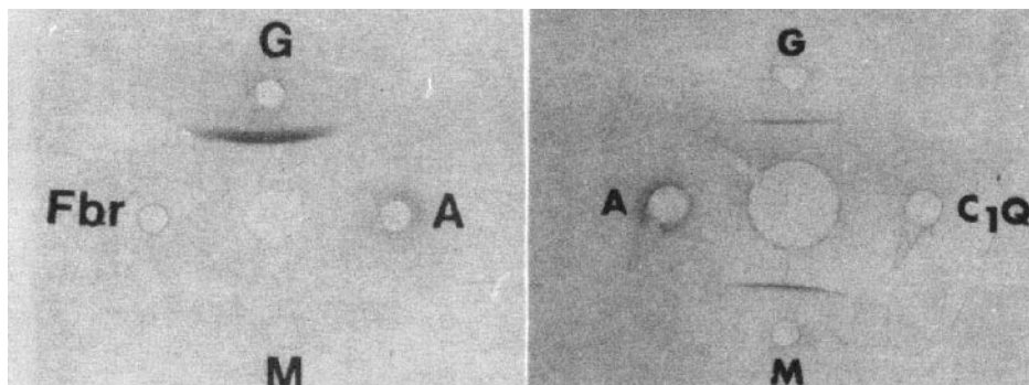
Fig. 23.5 Characterization of two washed cryoglobulins. In both studies, the washed and redissolved cryoglobulin was placed on the center well and four different antisera in the surrounding wells. The cryoglobulin studied on the left reacted with anti-IgG (G) only and was classified as a monoclonal cryoglobulin; the one studied on the right reacted with anti-IgG (G) and anti-IgM (M) and was classified as a mixed cryoglobulin.
