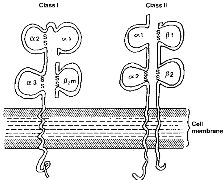
Fig. 3.3 Diagrammatic representation of the structure of human class I and class II histocompatibility antigens. (Modified from Hood, L. E., et al. Immunology , 2nd ed. Benjamin/Cummings, Menlo Park, CA, 1984.)
