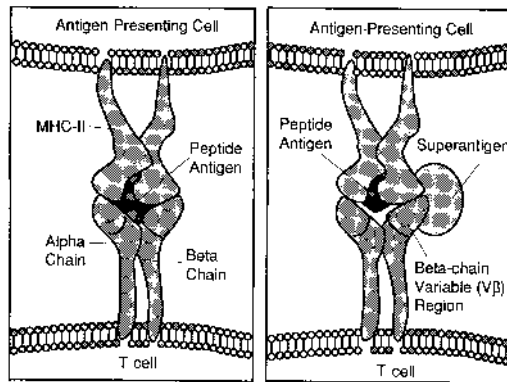
Fig. 14.4 Diagrammatic comparison of the mechanisms of T-cell stimulation by conventional antigens and staphylococcal enterotoxins. While conventional antigens are processed into oligopeptides, which bind to MHC-II molecules and then bind specifically to a TcR binding site (left panel), bacterial “superantigens” interact with nonpolymorphic areas of the V chain of the TcR and of the MHC-II molecule on an APC (right panel). Notice that “superantigen” binding overrides the need for TcR recognition of the MHC-II-associated oligopeptide, and thus T cells of many different specificities can be activated. It is also important to note that both APC and T cells can be stimulated as a consequence of the extensive cross-linking of membrane proteins. (Modified from Johnson, H. M., Russell, J. K., and Pontzer, C. H. Sci. Am. 266(4):92, 1992.)
