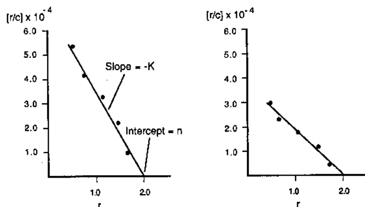
Fig. 8.2 Schematic representation of the Scatchard plots correlating the quotient between moles of hapten bound per moles of antibody ( r ) and the concentration of free hapten ( c ) with the concentration of hapten bound per mole of antibody ( r ). The slopes of the plots correspond to the affinity constants, and the intercept with the horizontal axis correspond to the number of hapten molecules bound per mole of antibody at a theoretically infinite hapten concentration ( n or valency of the antibody molecule). The plot on the left panel corresponds to a high-affinity antibody, and the slope is very steep; the plot on the right panel corresponds to a low-affinity antibody, and its slope is considerably less steep.
