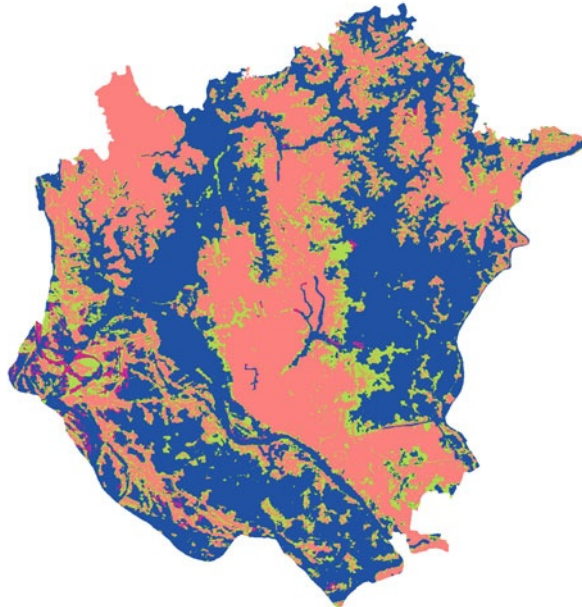
Fig. 5.2 (a) Flood-affected frequency and (b) floodwater depth
