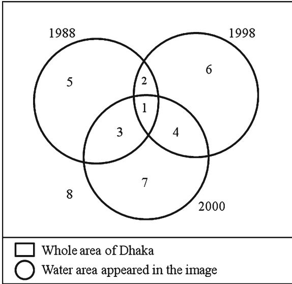
Fig. 5.1 Concept of flood-affected frequency (Adapted from Islam and Sado 2000)
