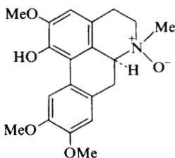
Thalictmidine N -oxide (22) Thalictrum minus 29
