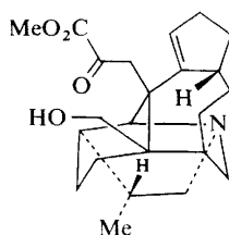
(81)
