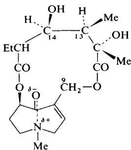
Syneilesine (12)
