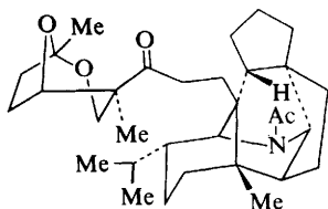
Daphniteijsmanine (82) R = H (87) R = Ac
