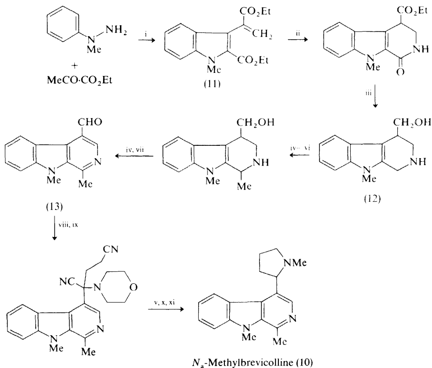
Scheme 5
