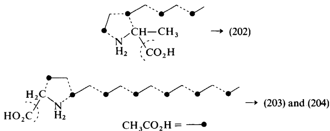
Scheme 24
