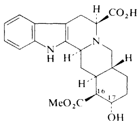
5-β-Carboxycorynanthine (74)
