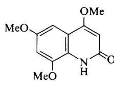
Halfordamine (6)
