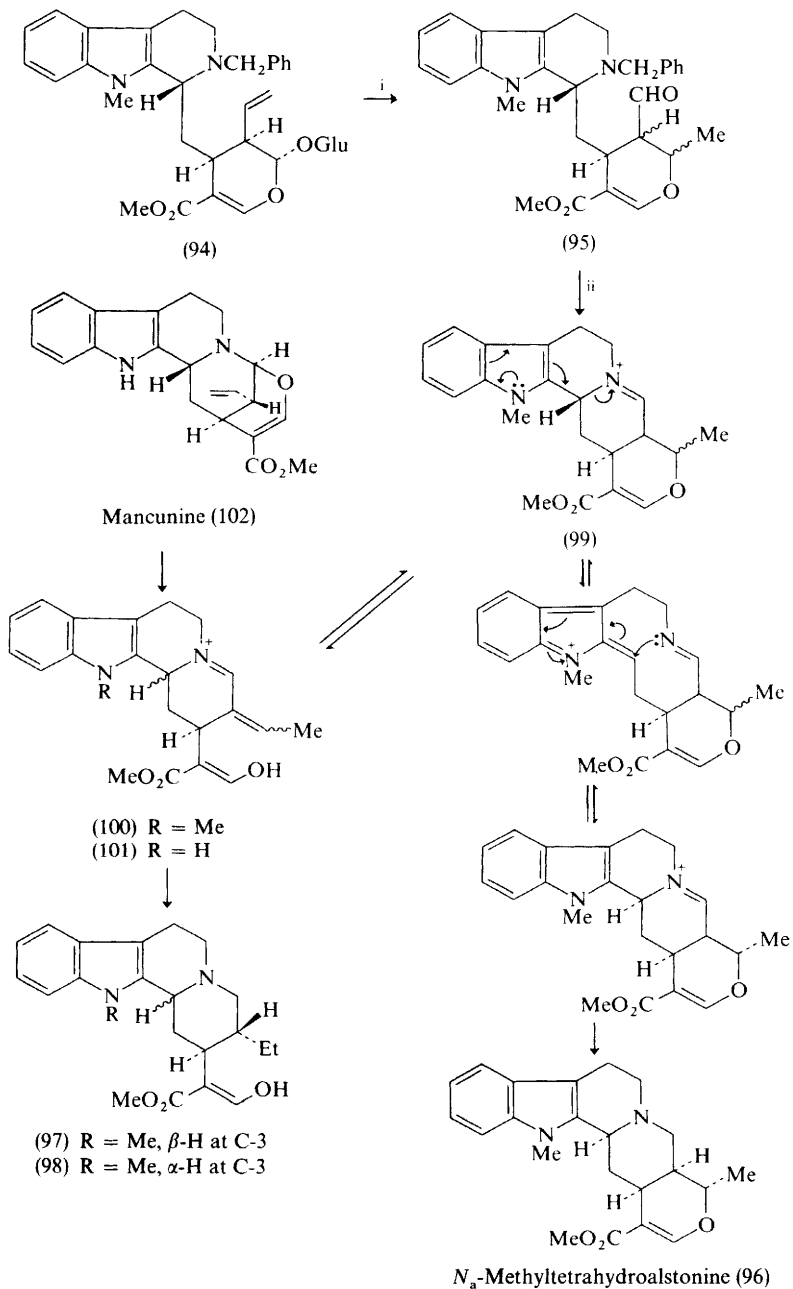
Scheme 15
