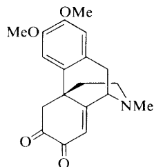
(87)
