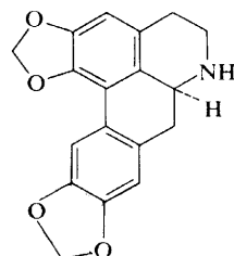
(+)-Cryptodorine (14) Cryptocarya odorata (Panch. et Seb.) Guillaum. 24
