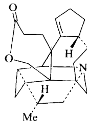
Daphnilactone-B (5)
