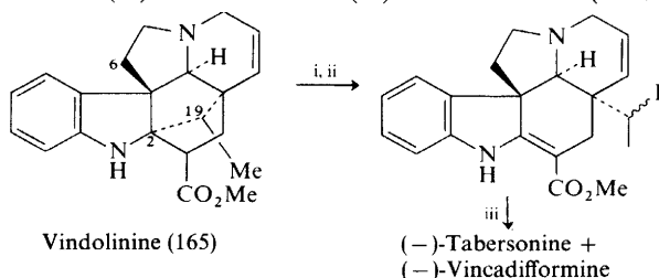
Scheme 30
