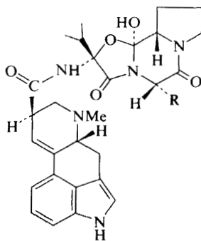
Ergocryptine (134) R = Bu i Ergocornine (135) R = Pr i
