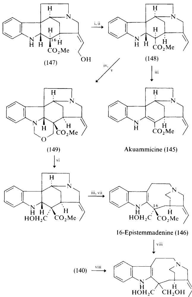
Scheme 25
