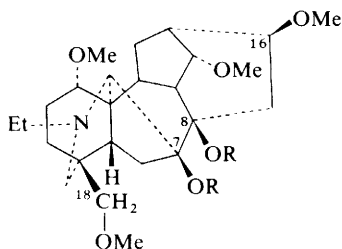
Deoxydelcorine (21) RR = CH 2 (22) R = H
