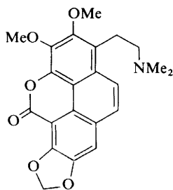
(94)
