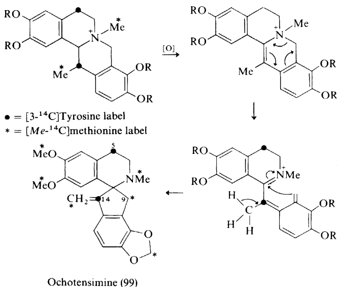
Scheme 13
