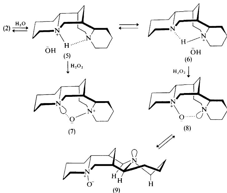
Scheme 1
