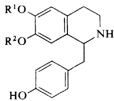
(77) R^1 = \text{Me}, R^2 = \text{H} (78) R^1 = \text{H}, R^2 = \text{Me}
