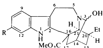
3-Hydroxyisovoacangine (193) R = OMe 3-Hydroxycoronaridine (194) R = H
