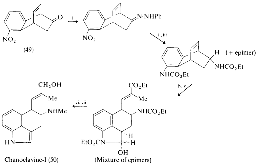
Scheme 10
