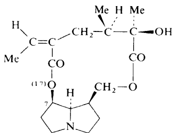
Platyphylline (39)
