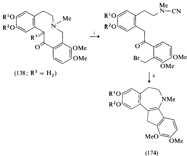
Scheme 19
