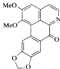
Oxonantenine (63) Cassipoupa racemosa Nees. 72
