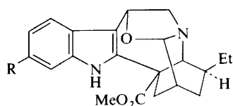
Eglandine (195) R = H 3,6-Oxido-isovoacangine (197) R = OMe (11-Methoxyeglandine)
