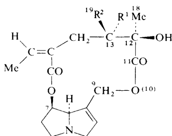
Senecionine (40) R^1 = H, R^2 = Me Seneciphylline (41) R^1, R^2 = CH_2
