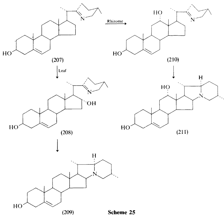
Scheme 25
