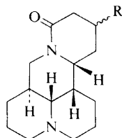
Albertamine (20) R = OH Darvasamine (21) R = H
