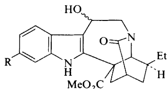
Eglandulosine (196) R = H (-)-6-Hydroxy-3-oxo-isovoacangine (198) R = OMe (11-Methoxyeglandulosine)
