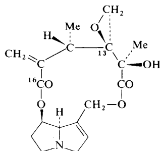
Swazine (6)
