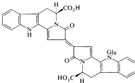
Trichotomine G 1 (235)
