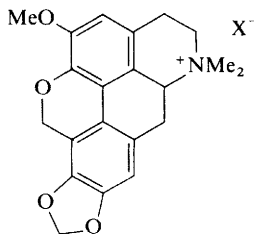
(98)
