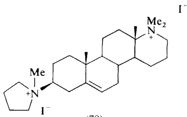
(78)
