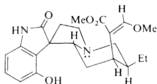
Speciofoline (83)
