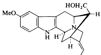
Lochvinerine (110)
