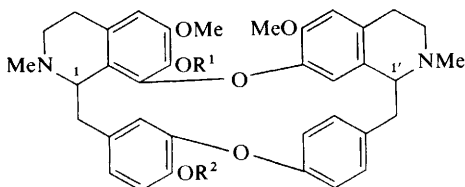
(196)
