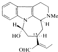
Akagerine (68)
