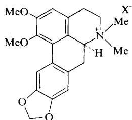
(+)-Nantenine methochloride (8) Thalictrum polygamum Muhl. 19
