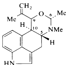
Paspoclavine (39)
