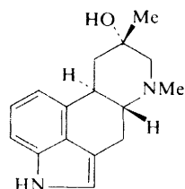
Dihydrosetoclavine-I (38)
