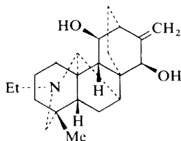
Denudatine (70)
