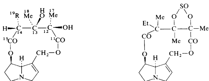
Monocrotaline (21) R = Me Trichodesmine (22) R = Me 2 CH
