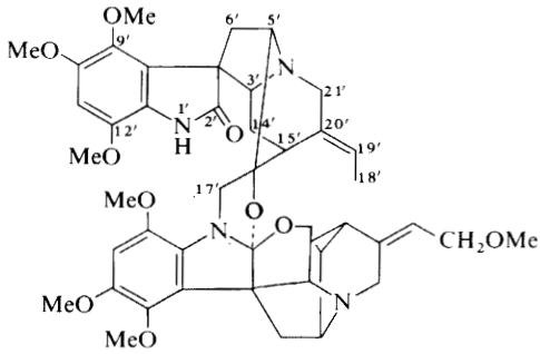
Gardmultine (229)
