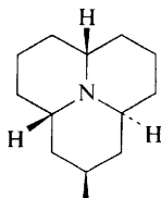
Hippodamine (47)
