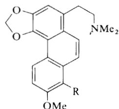
(89) R = H (90) R = OMe
