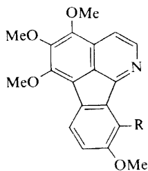
(99) R = OMe (100) R = H
