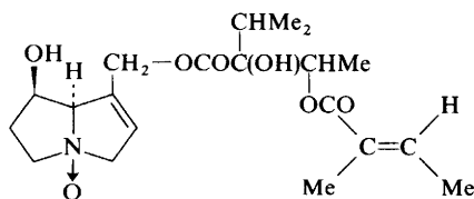
Anadoline N -oxide (11)
