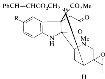
Lanciferine (116) R = H 10-Methoxylanciferine (117) R = OMe 10-Hydroxylanciferine (118) R = OH
