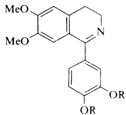
(103) R + R = CH 2 (104) R = Me
