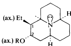
Poranthericine (51) R = H O -Acetylporanthericine (52) R = Ac
