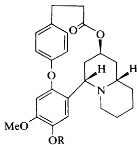
Decaline (29) R = Me Desmethyldecaline (30) R = H
