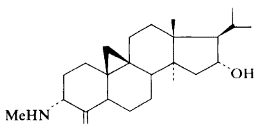
(67)
