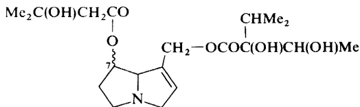
Uluganine (29)
