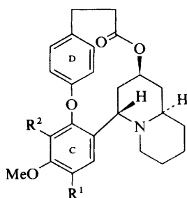
Vertaline (32) R 1 = OMe, R 2 = H Lagerine (33) R 1 = H, R 2 = OH O-Methyl-lagerine (34) R 1 = H, R 2 = OMe
