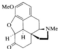
(78)
