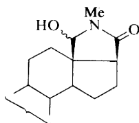
(50)
