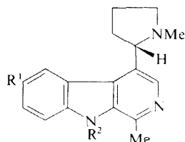
Brevicolline (8) R^1 = R^2 = H 6-Bromobrevicolline (9) R^1 = Br, R^2 = H N_a -Methylbrevicolline (10) R^1 = H, R^2 = Me
