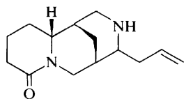
Angustifoline (10)
