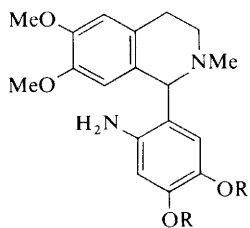
(101) R + R = CH 2 (102) R = Me
