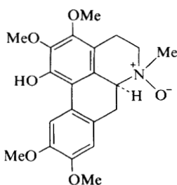
Preocoteine N -oxide (23) Thalictrum minus 29
