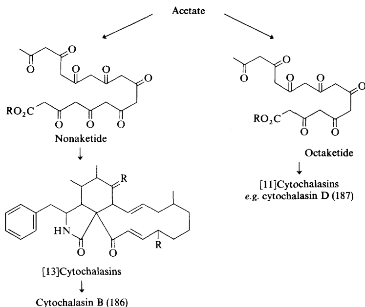
Scheme 20
