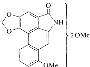
Aristo-red (73) 90 Aristolochia reticulata
