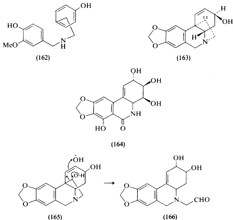
Scheme 18
