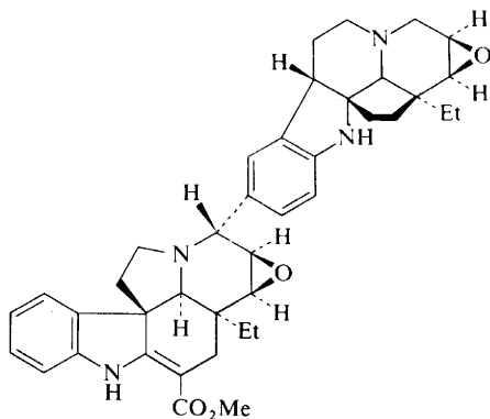
Cryophylline (222)
