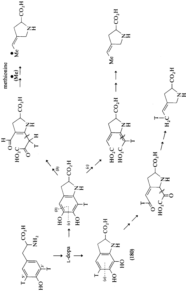
Scheme 19
