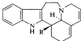
Andranginine (143) R = CO_2Me Andrangininol (144) R = CH_2OH
