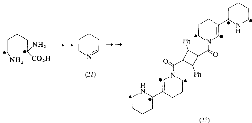
Scheme 5
