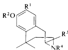
(103)
