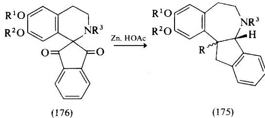
Scheme 20
