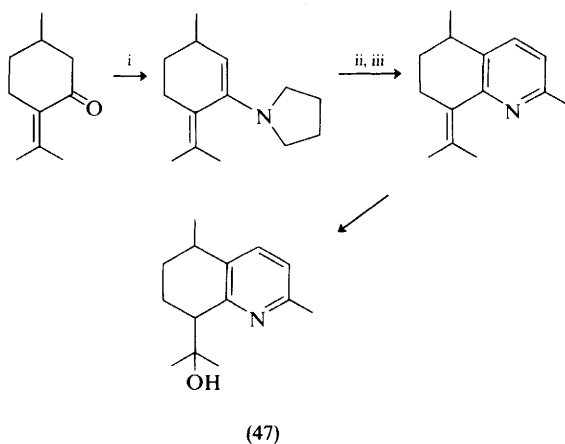
Scheme 8
