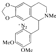
(86)
