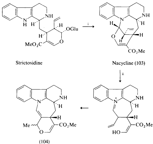
Scheme 16
