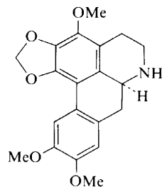
(+)-O-Methylcassyfiline (26) Cassythia americana 32
