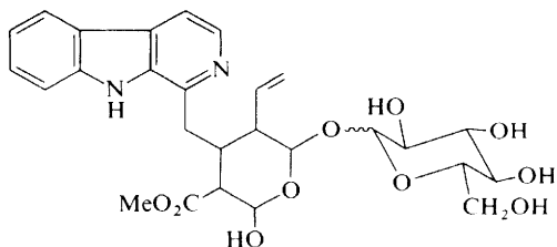
Palinine (67)
