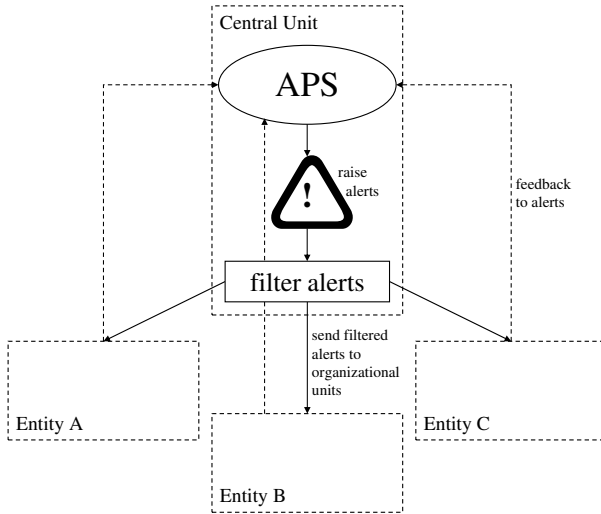
Fig. 13.2. Alert monitor
