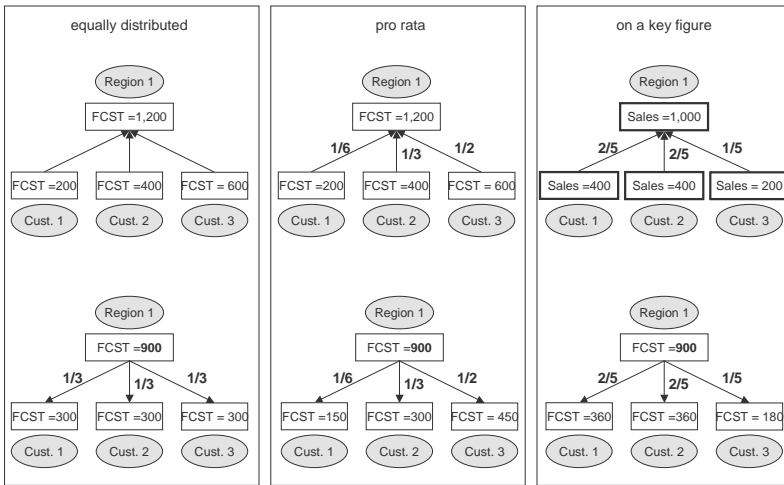
Fig. 23.5. Disaggregation rules
