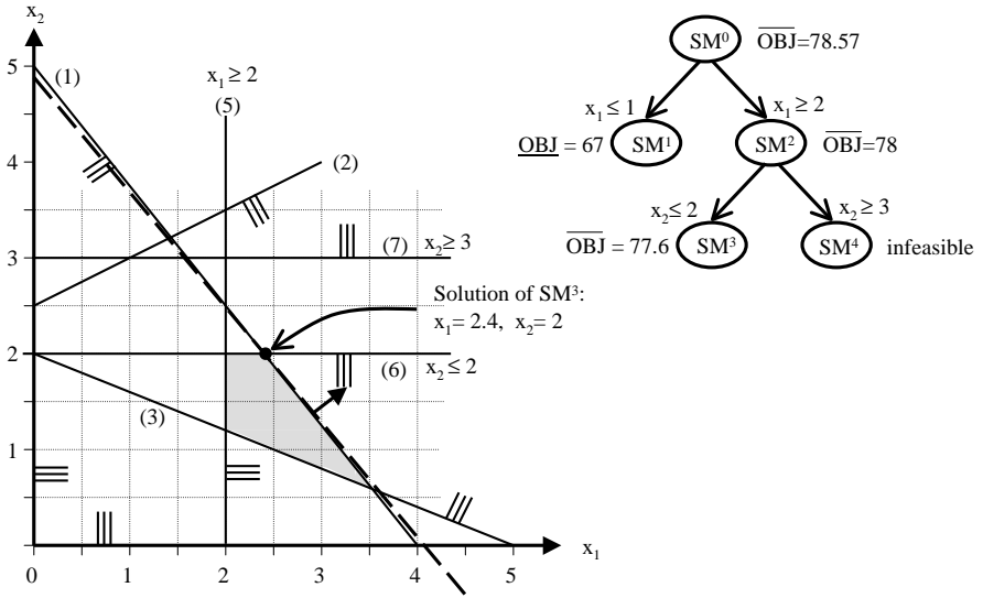
Fig. 29.6. A graphical representation of the third and fourth submodel
