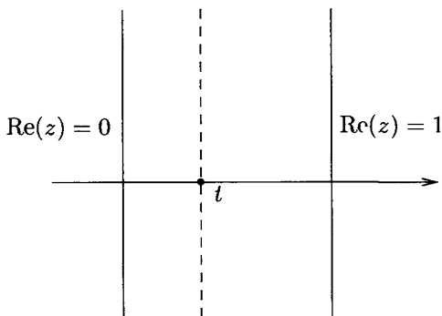
Figure 2. The domain of the function \Phi
