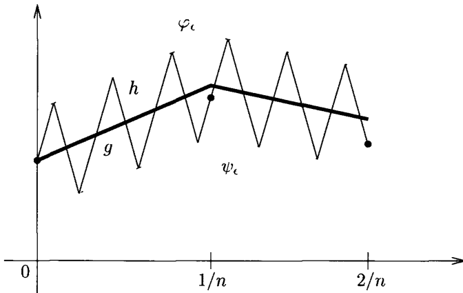
Figure 1. Approximation by \mathcal{P}_M
