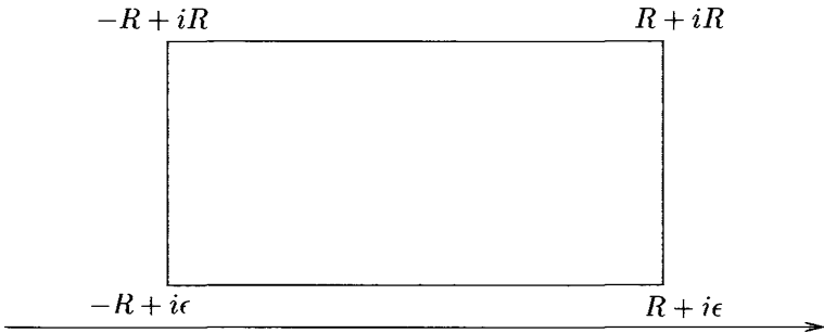
Figure 6. The rectangle of integration \gamma
