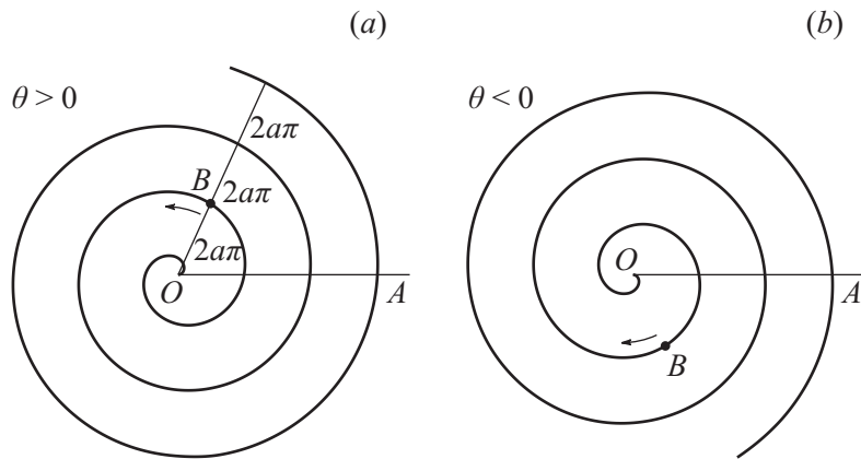
Figure 4.9. A spiral of Archimedes \rho = a\theta corresponding to the positive (a) and negative (b) values of \theta .
