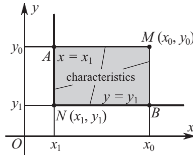
Figure 14.4. Domain of influence of the solution to the Goursat problem at a point M .
