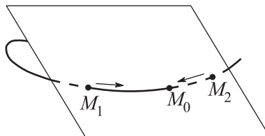
Figure 9.16. The osculating plane.
