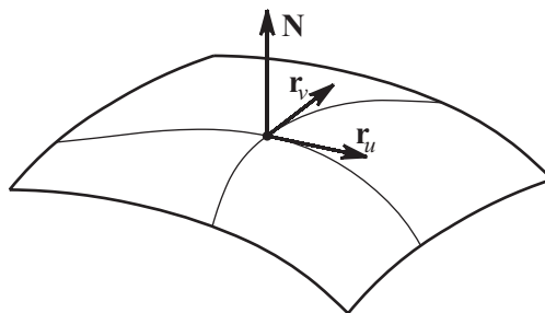
Figure 9.21. Coordinate vectors.
