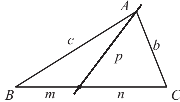
Figure 3.7. Stewart's theorem.
