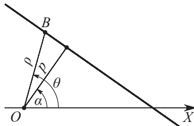
Figure 4.16. A straight line with equation in polar coordinates.
