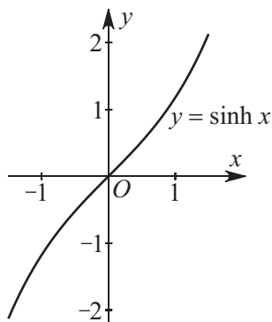
Figure 2.14. The graph of the function y = \sinh x .
