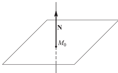
Figure 4.47. Straight line passing through point and perpendicular to plane.
