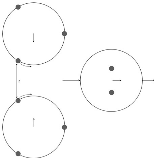
Fig. 9.1 Schematic of a possible newly created hadrons jet generation mechanism via the approach of two baryons leading to the formation of a jet in a direction perpendicular to the hadrons motion
