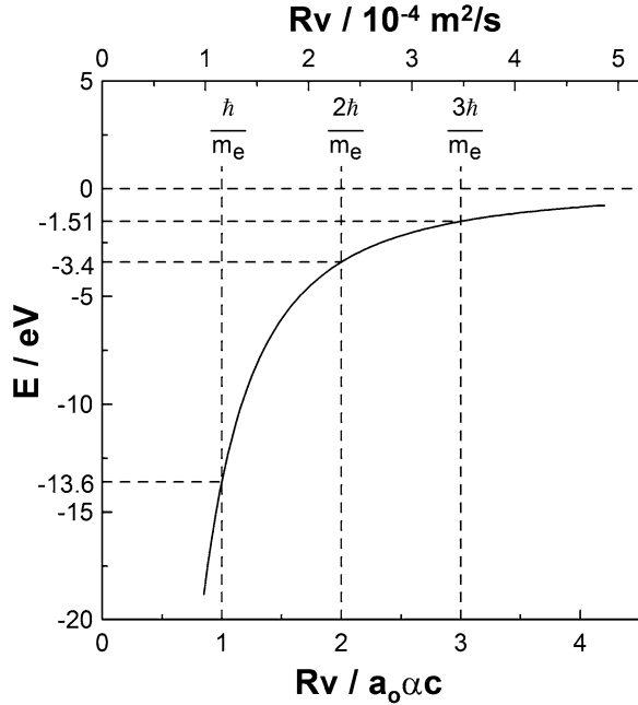
Fig. 12.5 Graphical solution of the Bohr model equations for the H atom written in the form E = -e^4/2\varepsilon^2m_e(Rv)^2 (particle) and Rv = n\hbar/m_e (wave); \alpha(= e^2/\varepsilon c\hbar) is the fine structure constant and a_0(= \hbar/m_e\alpha c) is the Bohr radius
