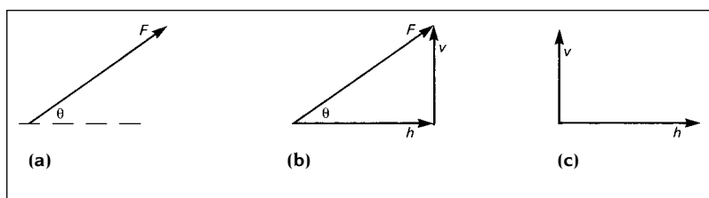
Fig. A1.3 Resolution of a force into components. (a) A single force. (b) A triangle of forces used to determine the vertical and horizontal components of the single force: v = F \sin \theta ; h = F \cos \theta . (c) The vertical and horizontal components are exactly equivalent to the original force.
