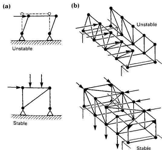
Fig. 2.4 Conditions for stability of frameworks. (a) The two-dimensional system is stable if it is capable of achieving equilibrium in response to forces from two mutually perpendicular directions. (b) The three-dimensional system is stable if it is capable of resisting forces from three directions. Note that in the case illustrated the resistance of transverse horizontal load is achieved by the insertion of rigid joints in the end bays.
