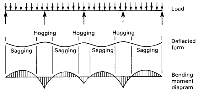
Fig. A3.6 A beam which is continuous over a number of supports is a statically indeterminate structure. The magnitudes of the bending moments in each span are lower than if hinge joints were provided at each support (the statically determinate form).
