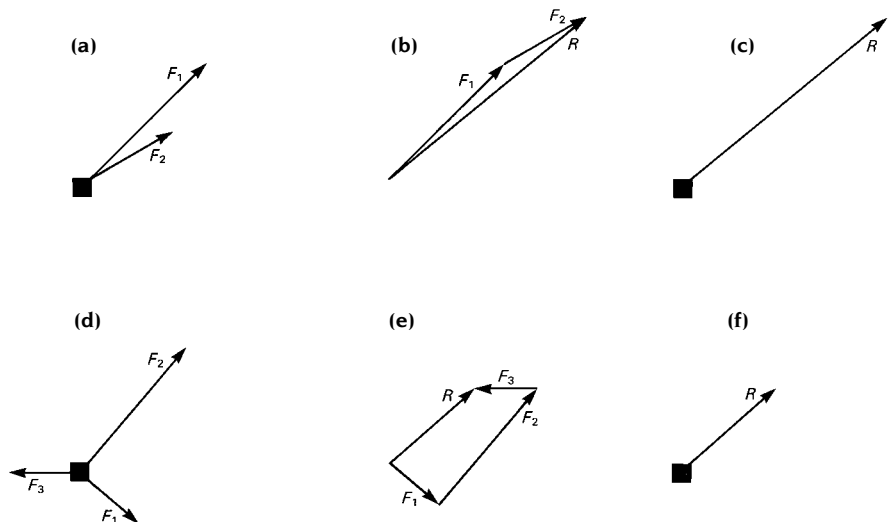
Fig. A1.1 Force is a vector quantity and can be represented by a line whose length is proportional to its direction and whose direction is parallel to its direction.
