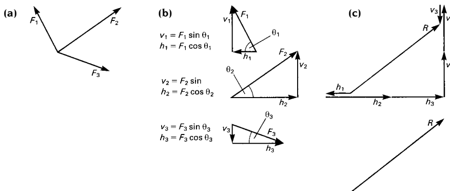
Fig. A1.4 Use of resolution of forces into components to determine the resultant of a set of forces. (a) Three concurrent forces. (b) Resolution of the forces into vertical and horizontal components. (c) Determination of the resultant by vector addition of the components.
