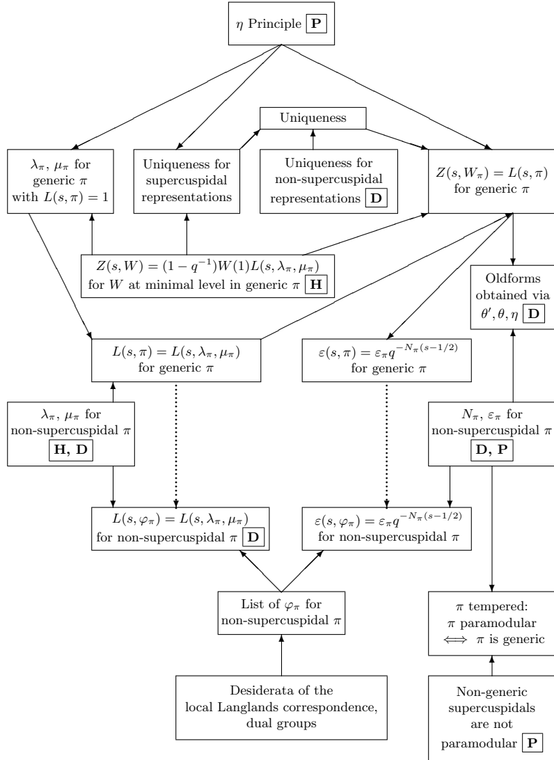
Fig. 1.5. Relations between major results. The symbols \mathbf{P} , \mathbf{D} and \mathbf{H} indicate the use of P_3 -theory, double coset decompositions, and Hecke operators, respectively. The factor L(s, \lambda_\pi, \mu_\pi) is defined by the formulas in i), ii) and iii) of Theorem 7.5.3 or Theorem 7.5.9. The dashed arrows indicate motivation.
