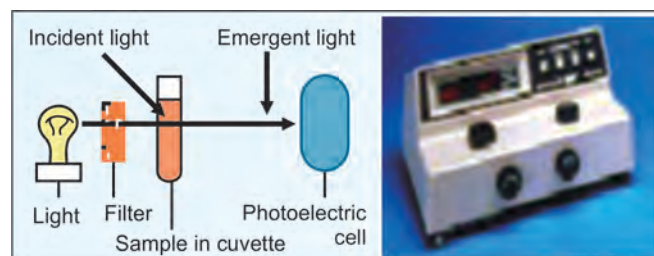
Fig. 35.18: Photoelectric colorimeter
