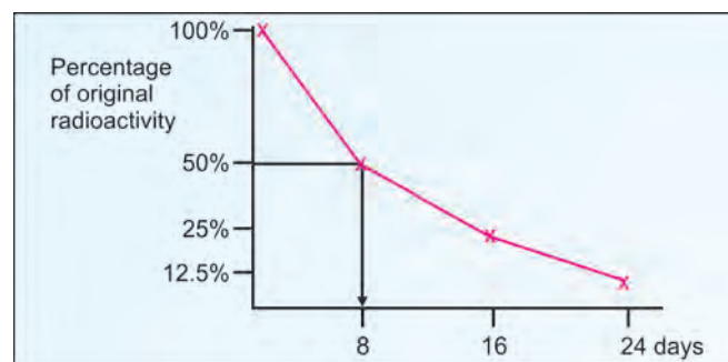
Fig. 59.1: Radioactive decay and half-life of ^{131}\text{I}
