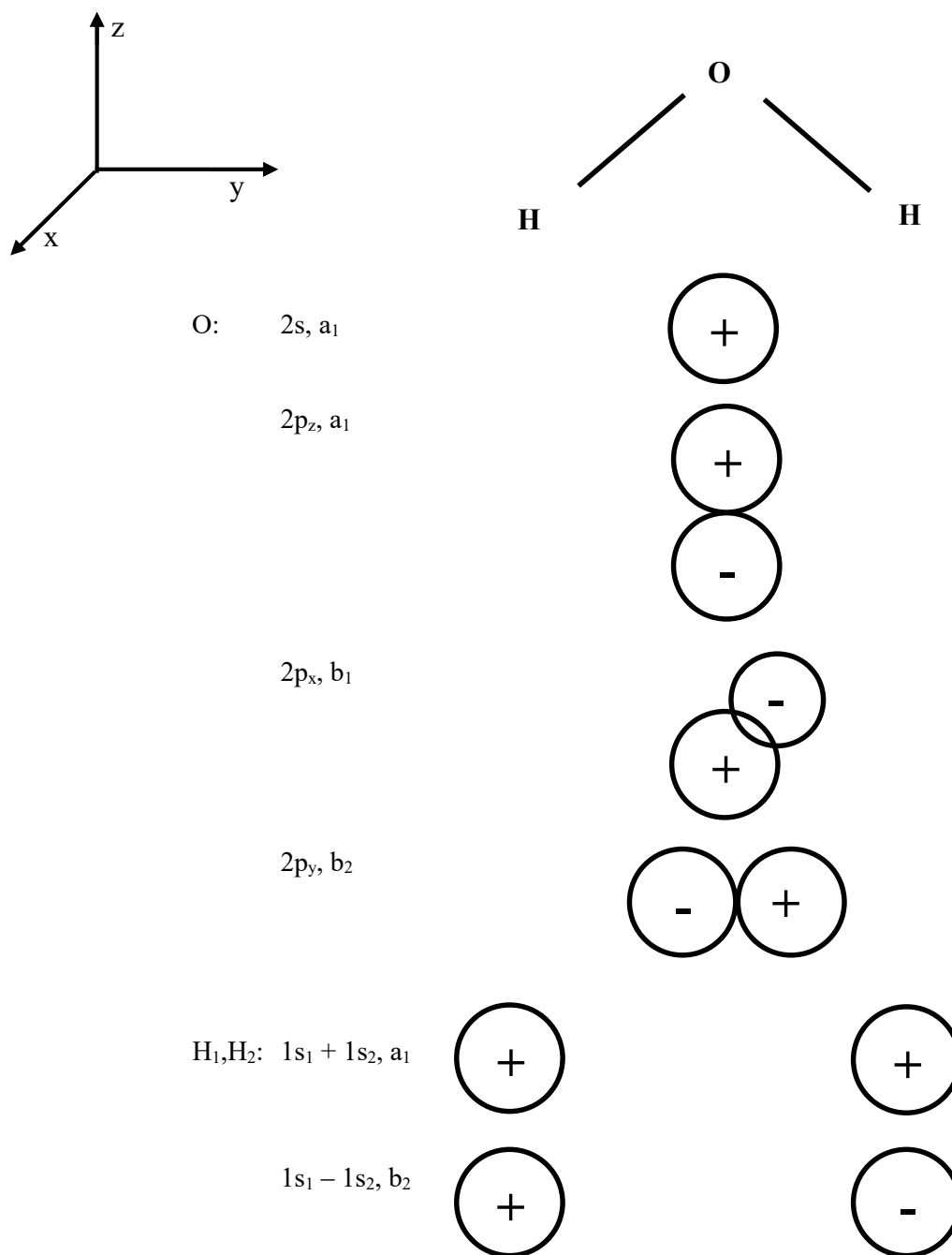
Figure 3.9: Symmetries of atomic orbitals constituting the molecular orbitals of H_2O . The sign + , - symbolizes the phase of the corresponding wave function. Note that for the hydrogen atoms, a linear combination has to be considered to obtain an irreducible representation of the symmetry group C_{2v} .
