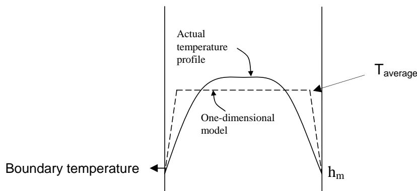
Figure 7.1 Schematic diagram of temperature distribution assumed for 1-dimensional, NI-NA reactor.
