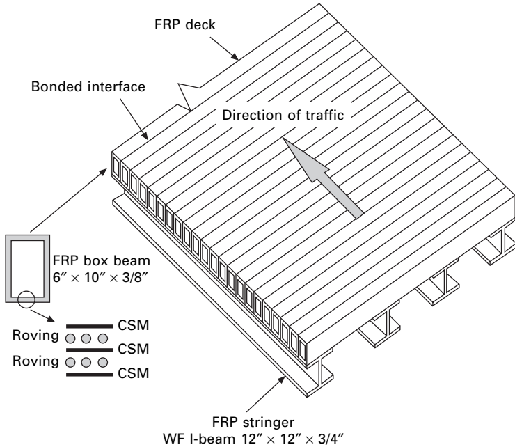
4.44 Schematic of FRP deck on FRP stringers.
