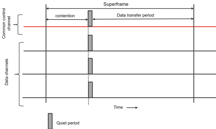
Fig. 1.9 Superframe structure of OSA-MAC. All nodes switch to the common control channel during the contention period. The winning node pair move to the agreed data channel and perform sensing of the channel during quiet-period. Based on the sensing result, the node pair either defer their communication for the current superframe or go ahead with the communication
