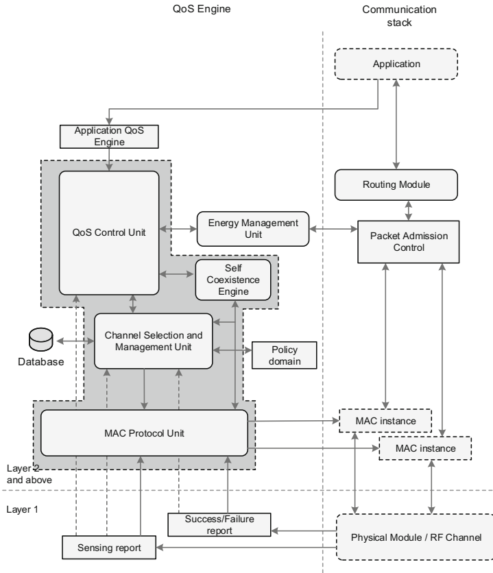
Fig. 7.1 Modules responsible for self-coexistence in cognitive radio networks
