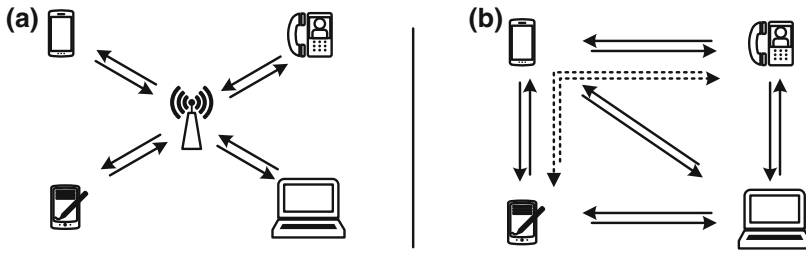
Fig. 1.7 Different types of CR networks: a Infrastructure based CR Network. b Cognitive Radio based ad-hoc network (CRAHN)
