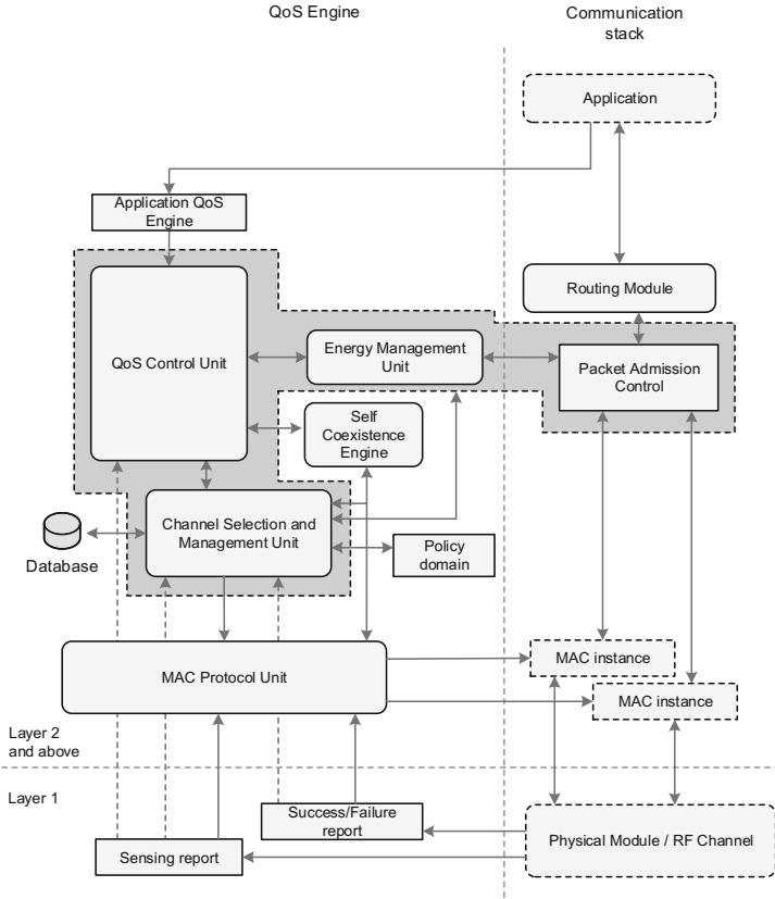
Fig. 6.1 Modules responsible for energy aware spectrum decision in the discussed QoS provisioning framework
