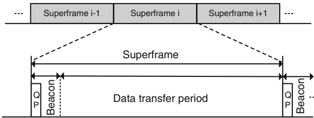
Fig. 7.6 Superframe structure of a medium access scheme
