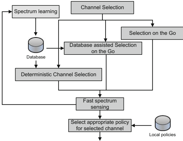
Fig. 4.2 Channel selection flow
