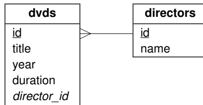
Figure 12.1 The DVD program’s database design
