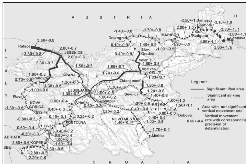
Figure 2. Vertical movement rate (mm/yr) in Slovenia determine from 1 st , 2 nd Yugoslav leveling and post-1989 leveling.
