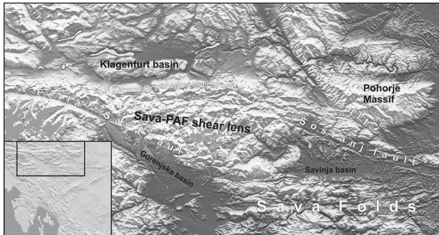
Figure 5. Topographic expression of the transpressional “shear lens” between the Sava fault and the Periadriatic fault.
