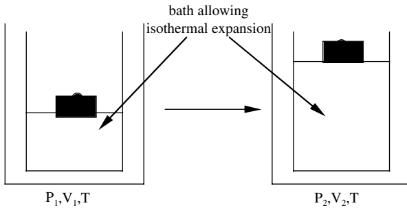
FIGURE 1.3 A cylinder with a frictionless piston holds a gas undergoing an isothermal expansion.
