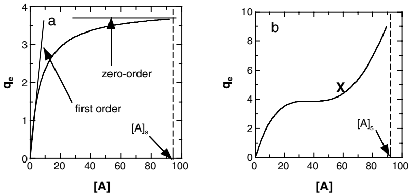
FIGURE 4.1 Langmuir and BET adsorption isotherms.
