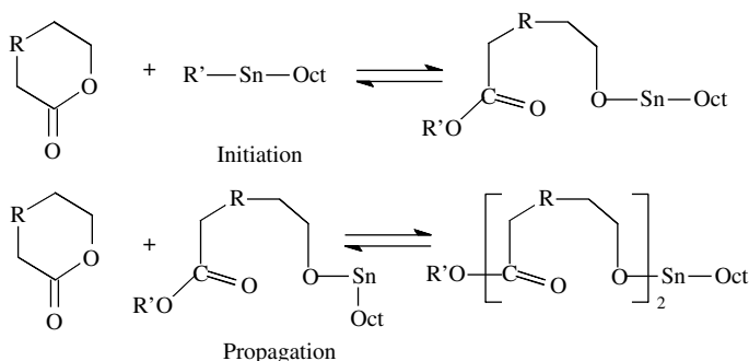
FIGURE 7.27 Initiation and propagation mechanism of \text{Sn}(\text{Oct})_2 -catalyzed polymerization of lactide.
