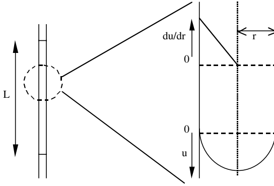
FIGURE 7.5 Capillary viscometer.
