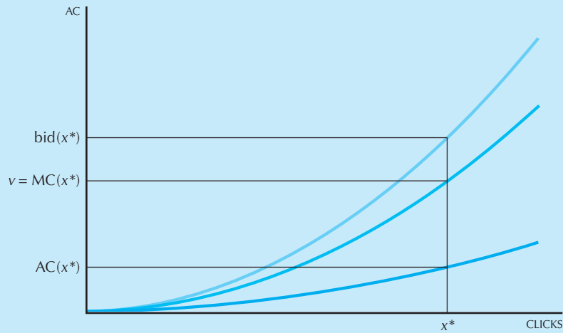
Click-cost curves. The profit-maximizing number of clicks is where value equals marginal cost, which determines the appropriate bid and average cost per click.
