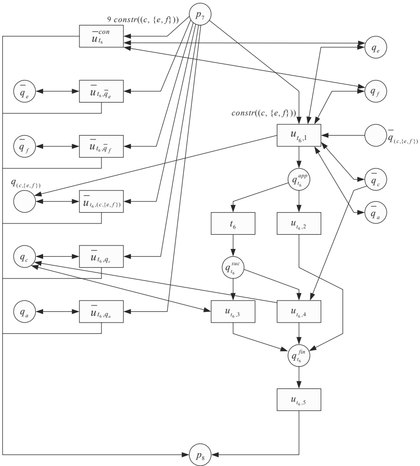
Fig. A.4. Translation of transition t_6
