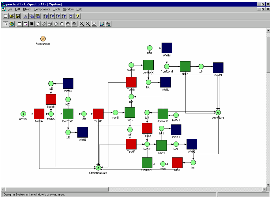
Fig. C1. ExSpect model of "handling of appeals" workflow
