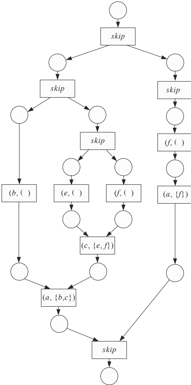
Fig. 3.14. Workflow model W15
