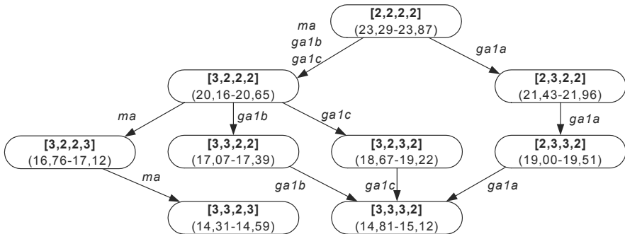
Fig. 5.10. Allocation decisions for N-construction
