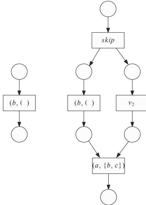
Fig. 3.12. Workflow models WF_3 and WF_4
