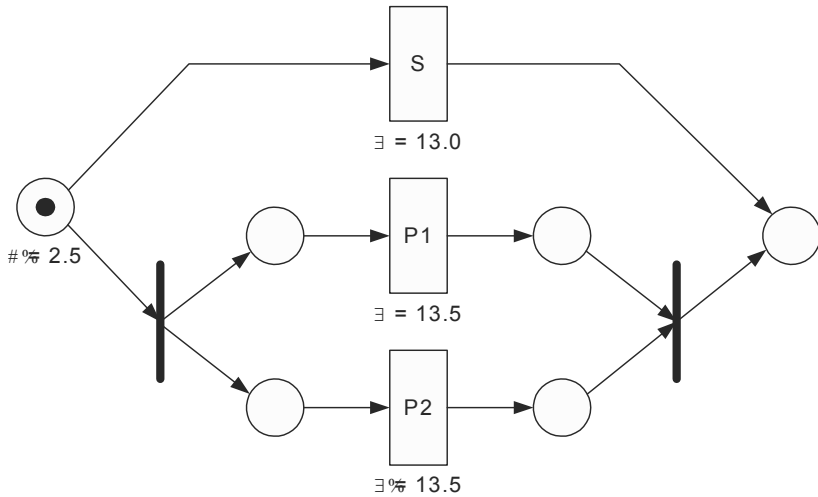
Fig. 5.5. Counter example for both strategies
