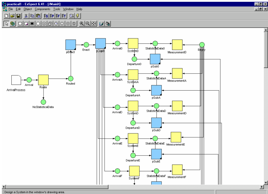
Fig. C2. Instantiated ExSpect framework for "handling of appeals"
