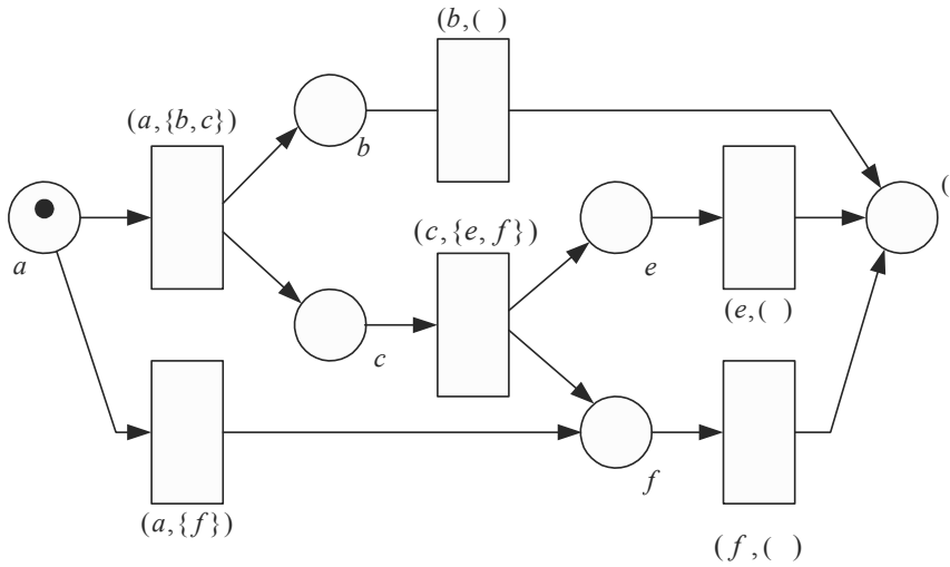
Fig. 3.8. Finding the solution for cost optimal plan S_2 .
