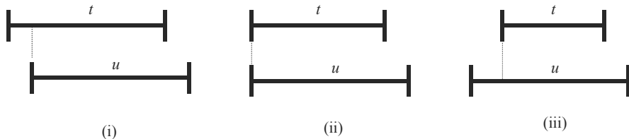
Fig. 2.2. The race semantics
