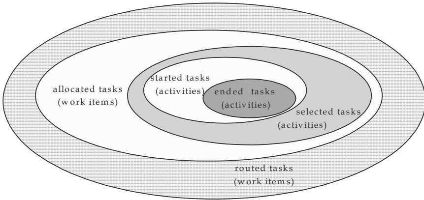
Fig. 7.2. Status of tasks in progress
