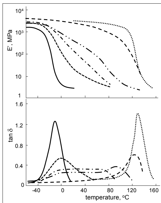
Figure 7.25 E' and \tan \delta vs. temperature for PU/PMMA compositions by weight of (—) 100/0; (---) 80/20; (- · - · -) 70/30; (- · · · -) 50/50; (- - - -) 20/80 and (.....) 0/100 (source: Akay & Rollins 1993)
