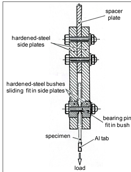
Figure 6.25 An illustration of specimen test fixture for bearing strength
