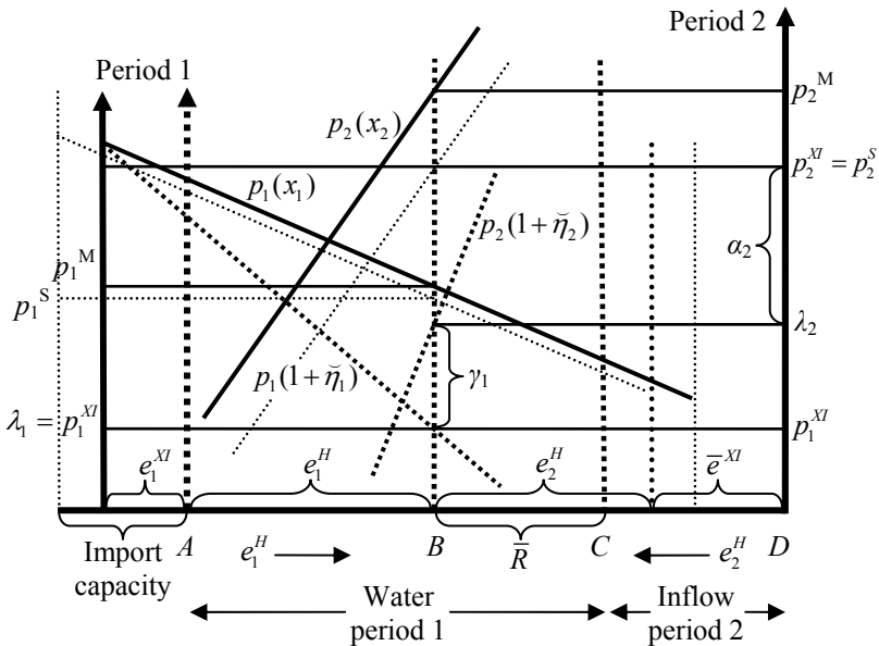
Figure 8.8. Monopoly, trade, and reservoir constraints. Social solution shown by thin dotted lines.
