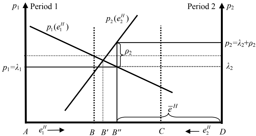
Figure 3.7. Production constraint binding in period 2.
