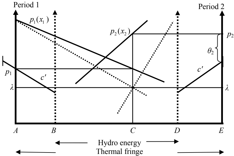
Figure 8.12. Dominant firm and constraint on the fringe output.
