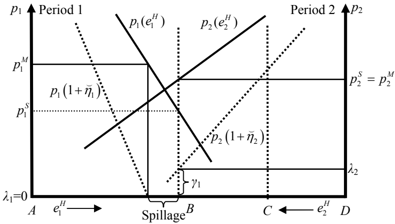
Figure 8.7. Monopoly with reservoir constraint and spillage. Social solution shown by dotted horizontal line.
