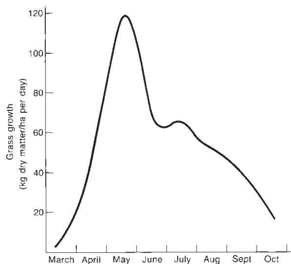
Fig. 4.12 Seasonal pattern of grass growth. Source: Milk from Grass (GRI and ICI).
