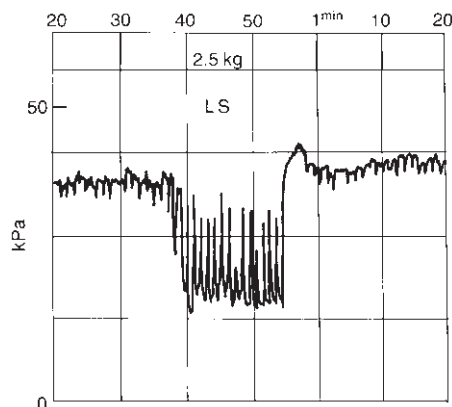
Fig. 26.7 Liner slip at the teat end during milk flow. LS, liner slip; 2.5 kg, flow rate of 2.5 kg/min.
