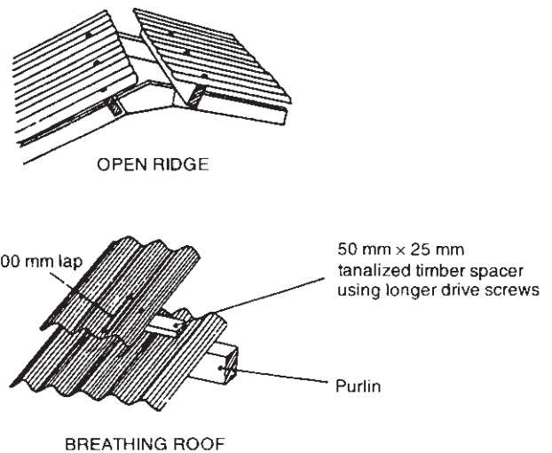
Fig. 4.26 Ventilation for a covered straw yard (reprinted from Hughes, 2000).
