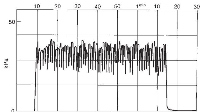
Fig. 26.5 Vacuum changes (cyclic fluctuations) at the teat end during milk flow.
