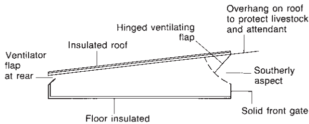
Fig. 56.4 Cross-section of a mono-pitch ('kennel') naturally ventilated stock building.
