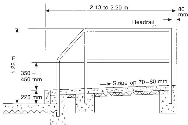
Fig. 4.20 A metal cubicle division.
