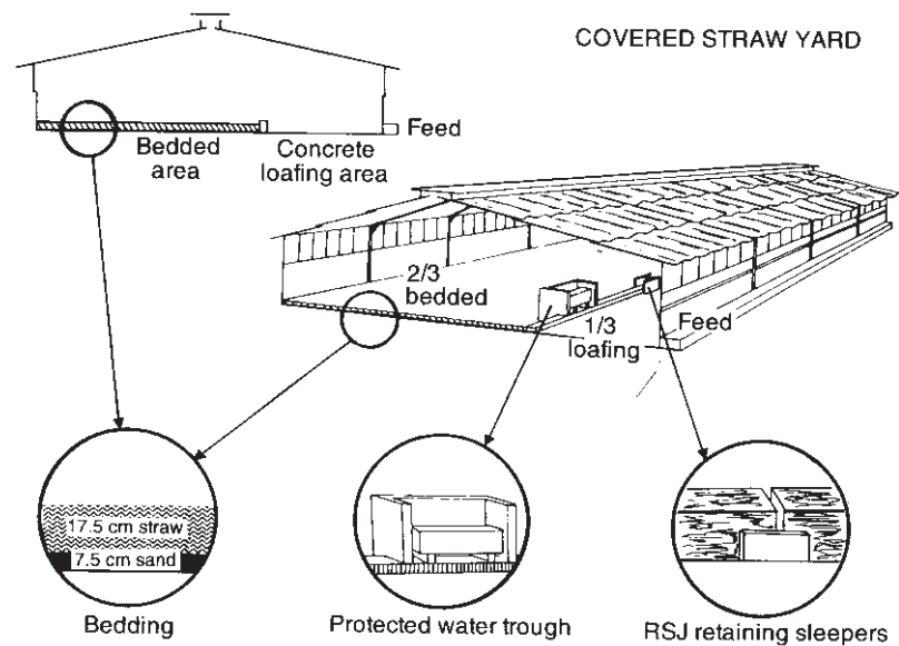
Fig. 4.25 Structures within a covered straw yard (reprinted from Hughes, 2000).
