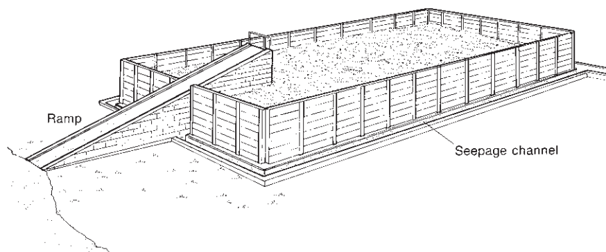
Fig. 4.27 A weeping-walled slurry compound.
