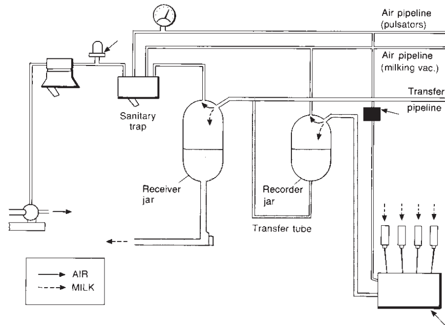
Fig. 26.3 Recorder milking machine.
