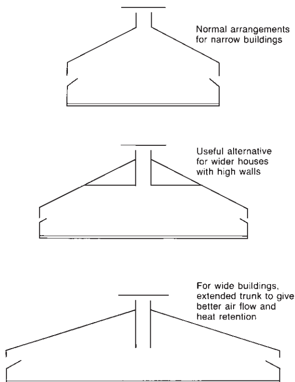
Fig. 56.2 Alternative arrangements suitable for natural ventilation of various widths of buildings and using outlet ('chimney') trunks.
