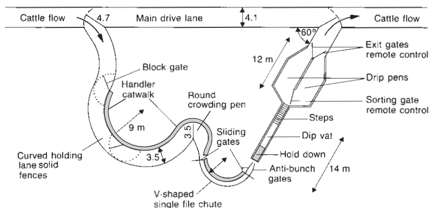
Fig. 55.5 Races for cattle should have no long straights or sharp corners so Grandin (1980) designed this race for movement to vehicles. (Measurements are in metres.)
