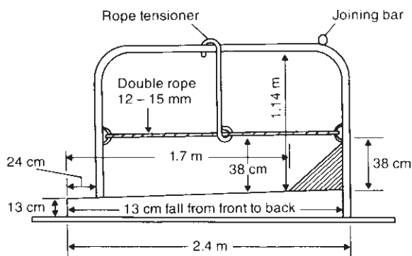
Fig. 4.21 A cubicle suitable for a Holstein cow (courtesy of J. Hughes).
