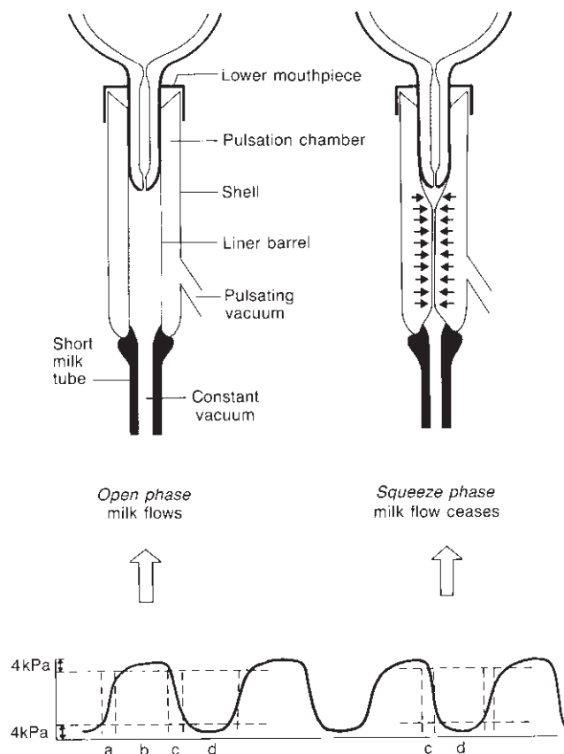
Fig. 26.4 Pulsation chamber waveform.
