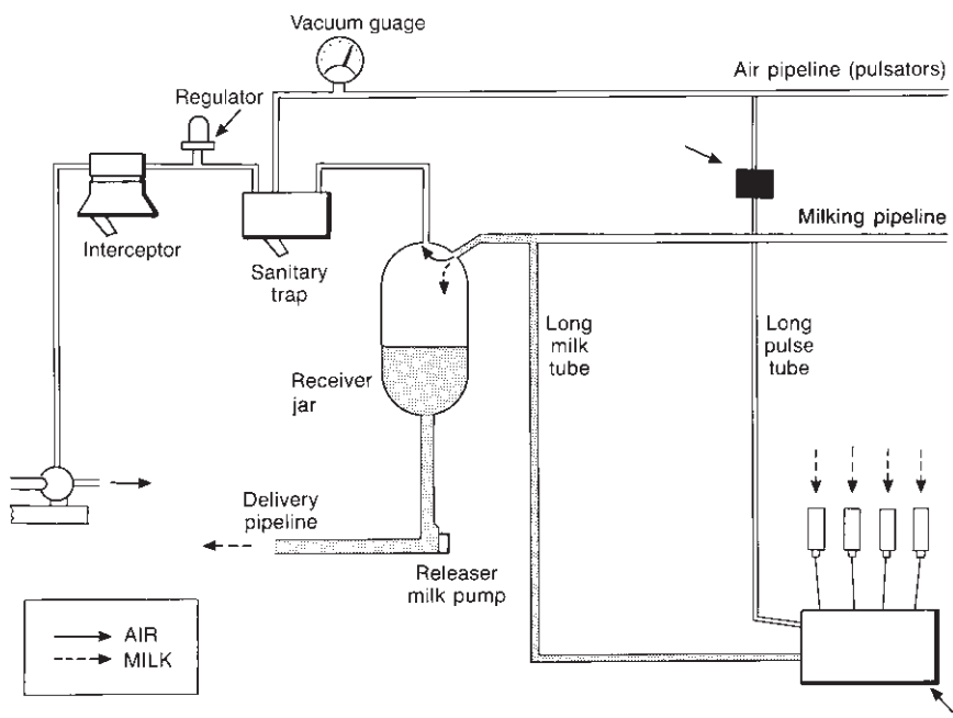
Fig. 26.2 Milking pipeline machine.
