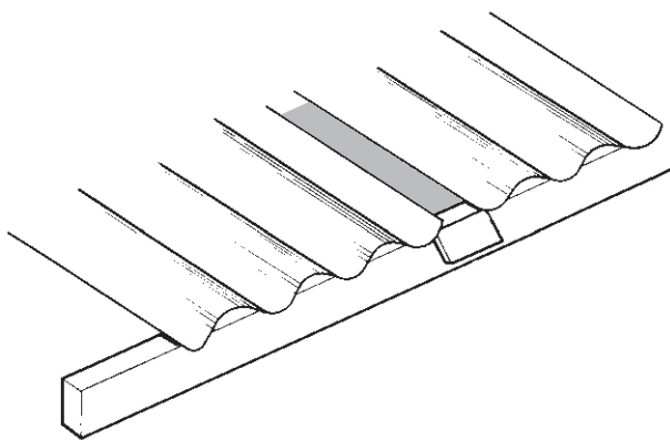
Fig. 56.9 The 'breathing' roof: ventilation achieved by leaving a gap between the roof sheets.
