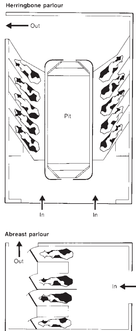
Fig. 4.18 An abreast and a herringbone parLOUR.
