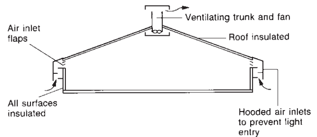
Fig. 56.3 Cross-section of a typical conventionally ventilated controlled environment house with roof fan extraction and hooded wall inlets.
