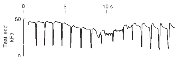
Fig. 26.6 Vacuum changes (irregular fluctuations) at the teat end during milk flow. Source: Nyhan (1968).
