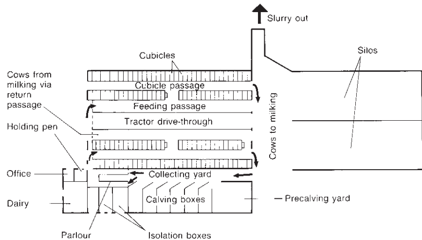
Fig. 4.17 Typical layout of a dairy unit.
