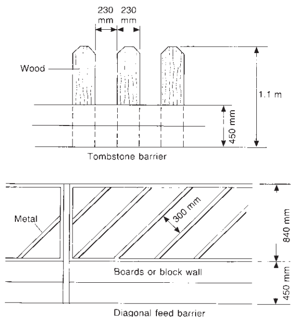
Fig. 4.15 Two types of feed barrier.
