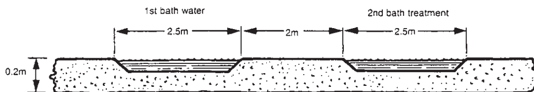
Fig. 31.12 Two footbaths in series.
