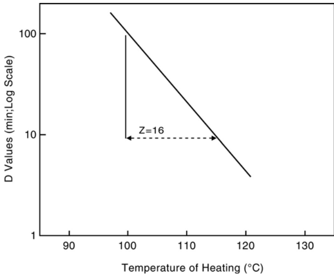
Figure 32.2 Hypothetical thermal death time curve. D , decimal reduction time; Z , ^\circ C required for the thermal death time curve to transverse over a \log_{10} cycle.
