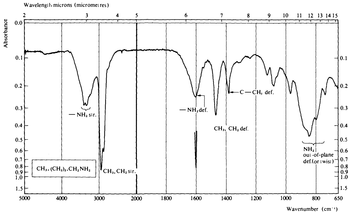
Fig. 3.26 Infrared spectrum of butylamine recorded as a liquid film.
