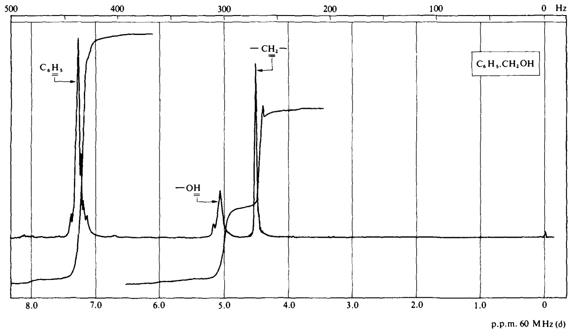
Fig. 3.65 Proton magnetic resonance spectrum of benzyl alcohol in CDCl_3 solution; sweep width 500 Hz.
