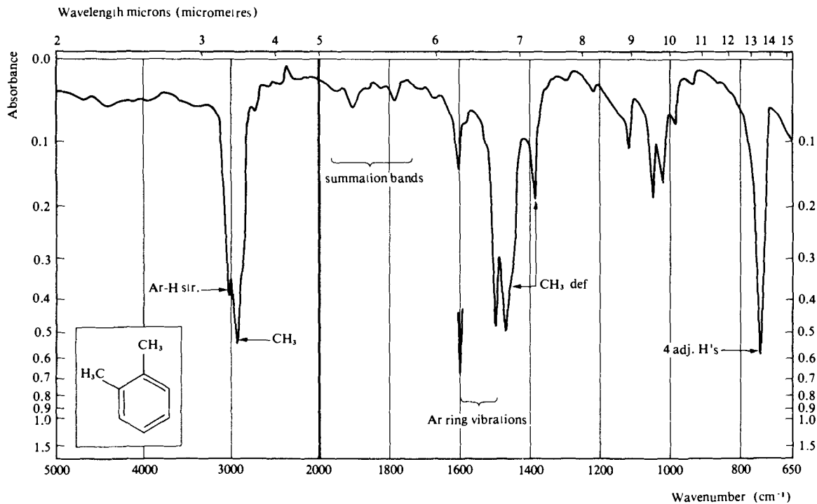
Fig. 3.16 Infrared spectrum of o -xylene recorded as a liquid film.
