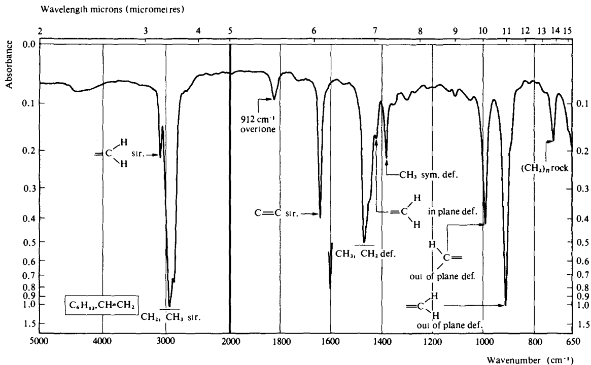
Fig. 3.14 Infrared spectrum of oct-1-ene recorded as a liquid film.
