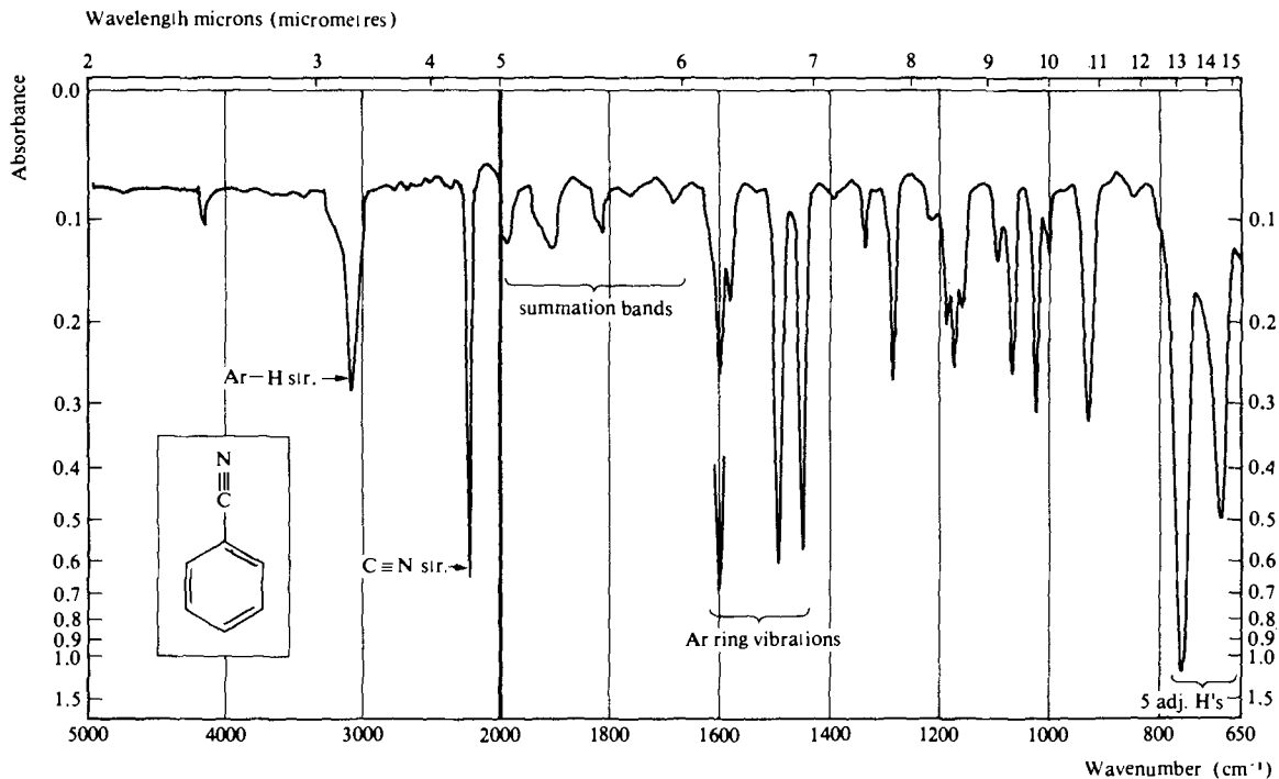
Fig. 3.39 Infrared spectrum of benzonitrile recorded as a liquid film.
