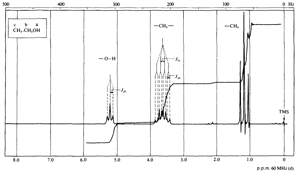
Fig. 3.67 Proton magnetic resonance spectrum of pure ethanol; sweep width 500 Hz.
