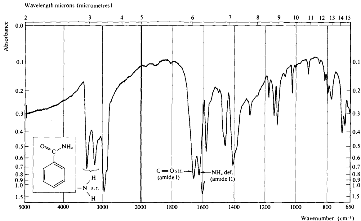
Fig. 3.35 Infrared spectrum of benzamide recorded as a Nujol mull.
