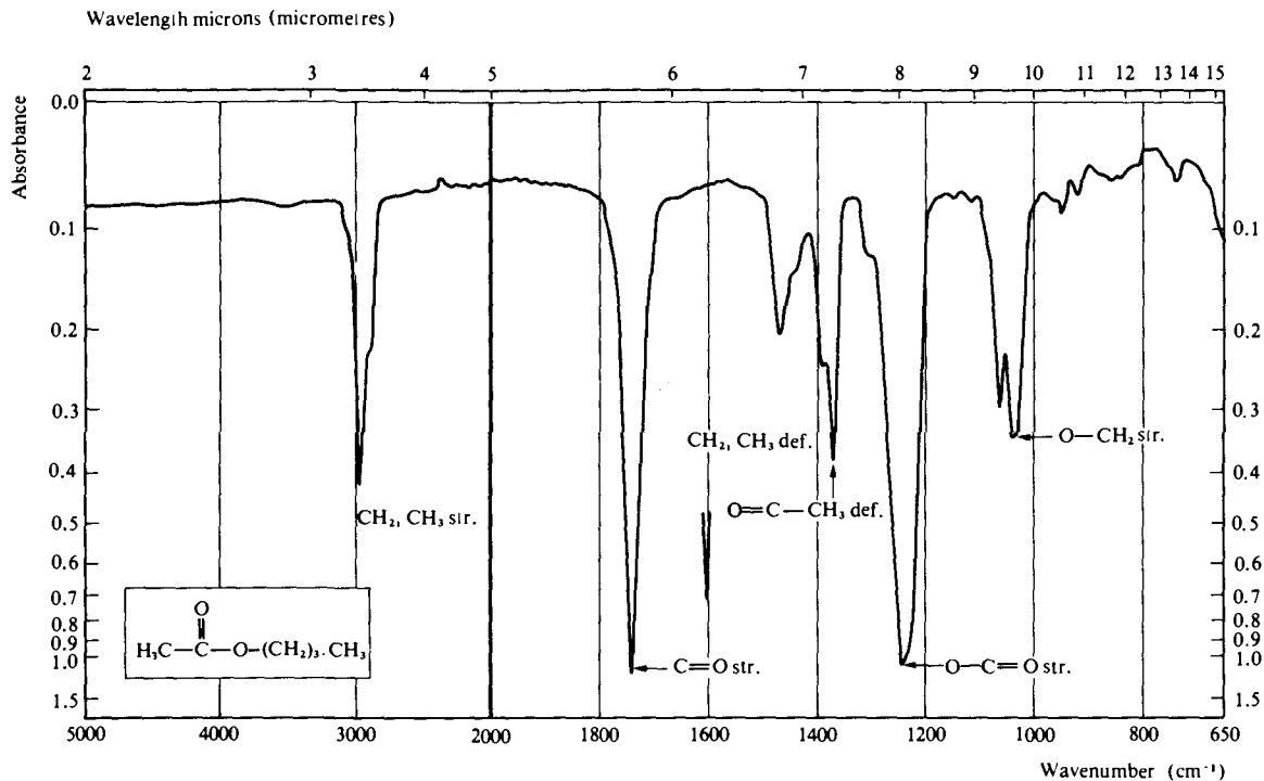
Fig. 3.33 Infrared spectrum of butyl acetate recorded as a liquid film.
