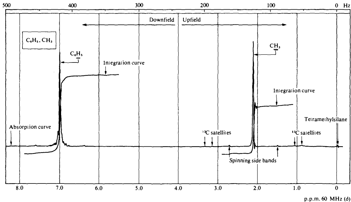
Fig. 3.42 Proton magnetic resonance spectrum of neat toluene; sweep width 500 Hz.
