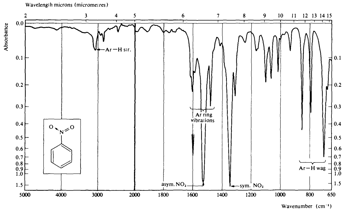
Fig. 3.38 Infrared spectrum of nitrobenzene recorded as a liquid film.
