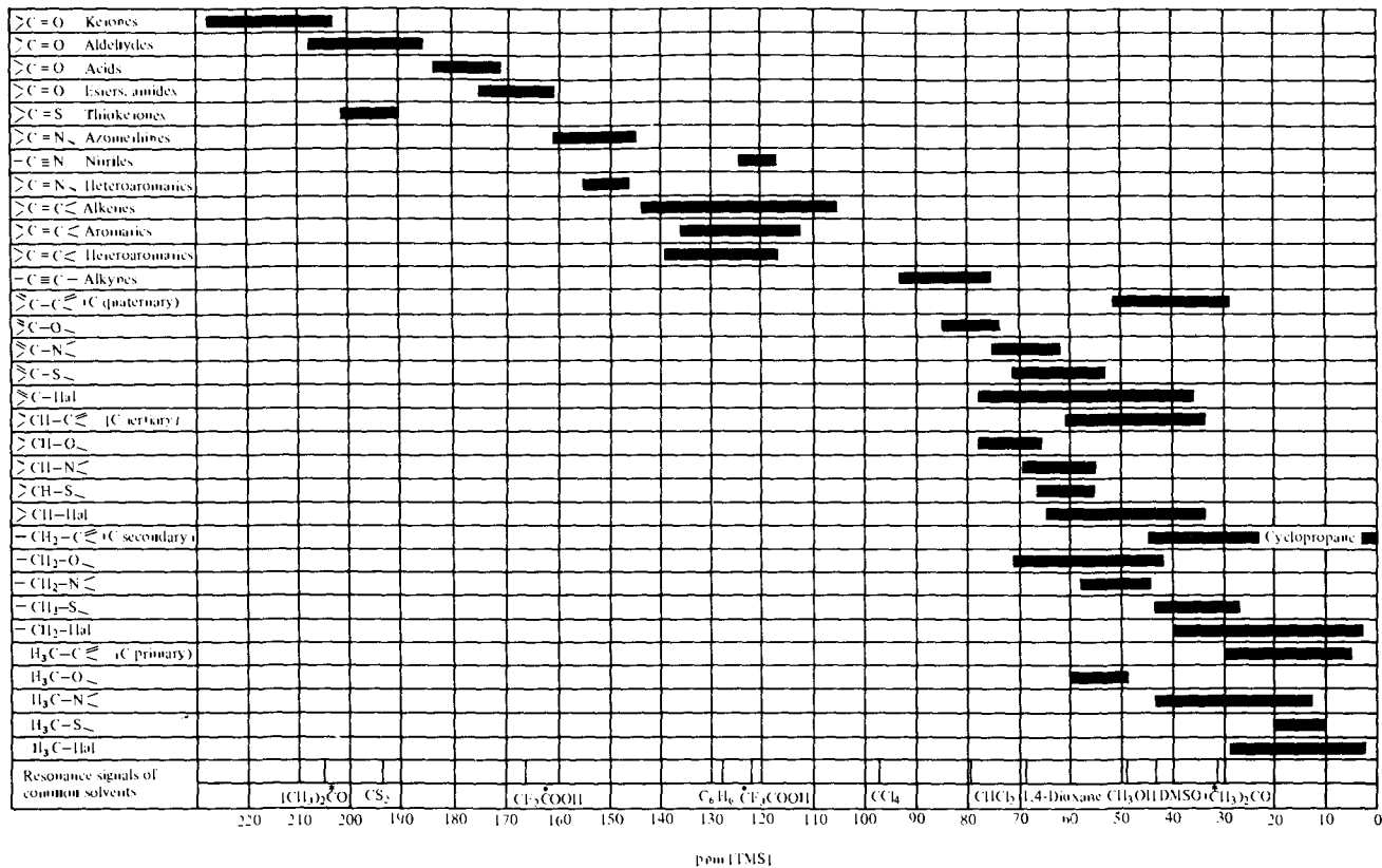
Fig. 3.45 ^{13}\text{C} chemical shifts in organic compounds. Data reproduced from E. Breitmaier, G. Jung and W. Voelter (1971). Angew. Chem. Int. Edn. Engl. , 10, 679.
