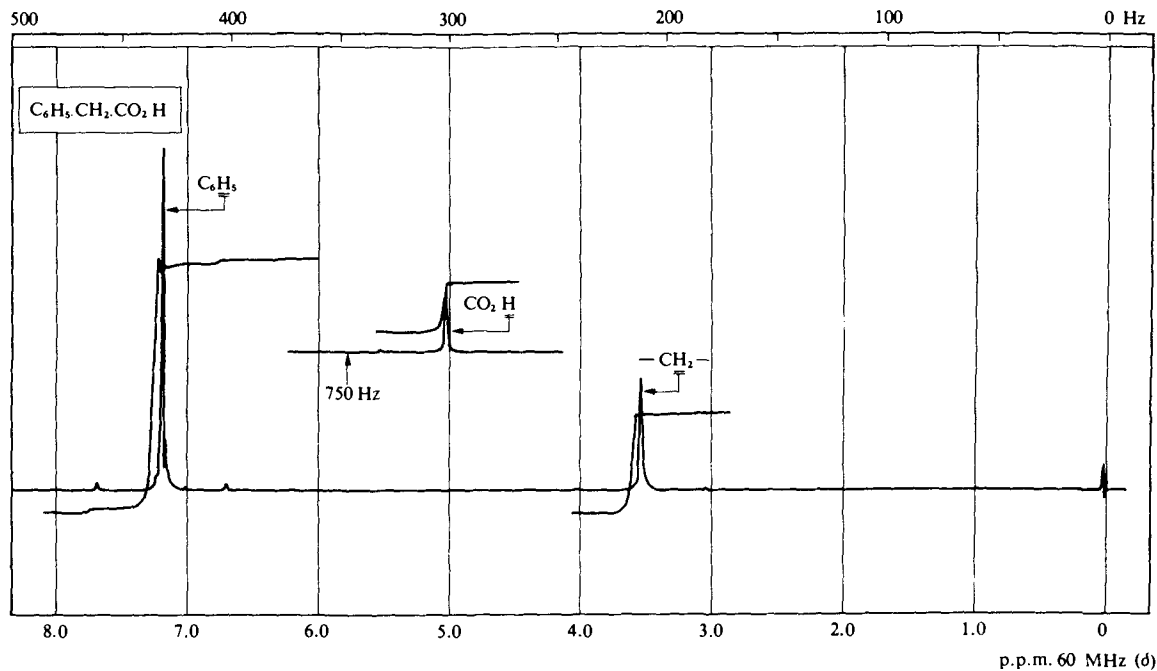
Fig. 3.47 Proton magnetic resonance spectrum of phenylacetic acid in \text{CDCl}_3 solution; sweep width 500 Hz. Inset: sweep offset 400 Hz.
