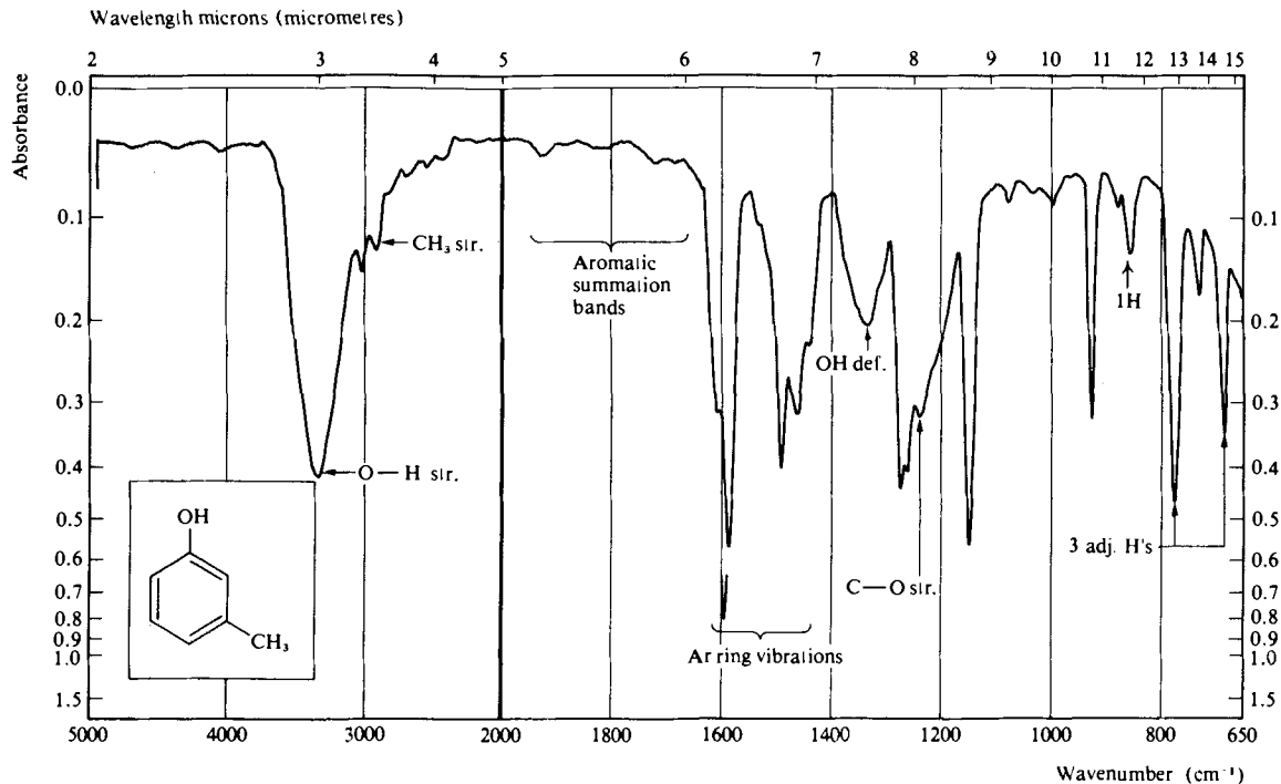
Fig. 3.22 Infrared spectrum of m -cresol recorded as a liquid film.
