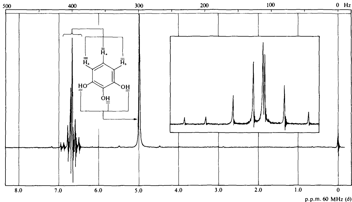
Fig. 3.60 Proton magnetic resonance spectrum of pyrogallol (AB 2 ) in D 2 O solution; reference DSS, and sweep width 500 Hz. Inset: sweep offset 380 Hz, sweep width 50 Hz. The signal at \delta 5 is due to HOD and arises from exchange of the three phenolic hydrogens with the solvent.
