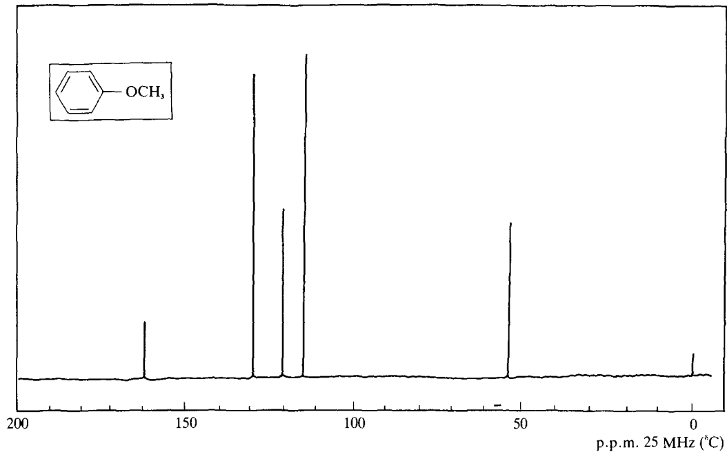
Fig. 3.54 ^{13}\text{C} nuclear magnetic resonance spectrum of anisole in \text{CDCl}_3 ; sweep width 200 p.p.m. Data reproduced from the Standard Carbon-13NMR Spectra Collection, © Sadtler Research Laboratories, Division of Bio-Rad Laboratories, Inc.
