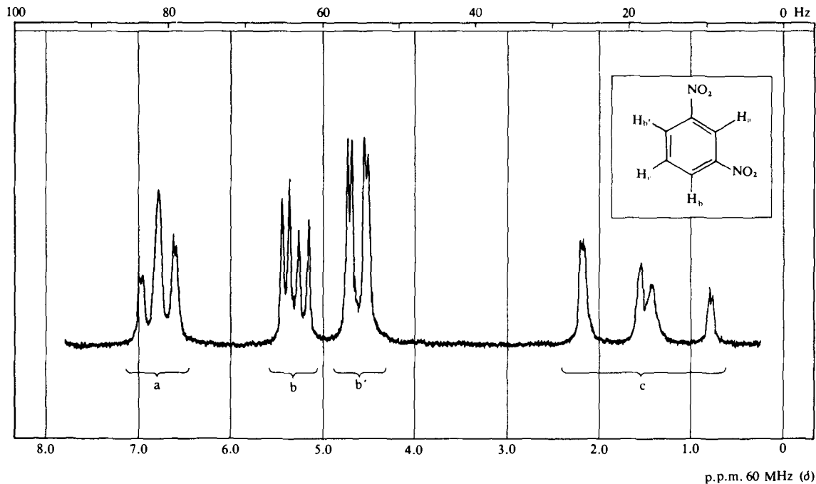
Fig. 3.64 Proton magnetic resonance of m -dinitrobenzene in \text{CDCl}_3 solution; sweep offset 460 Hz, sweep width 100 Hz. The \delta scale is not applicable in this case; actual \delta values may be obtained by dividing the chemical shift values in Hz by 60 (cf. Fig. 3.47) and relevant discussion p. 325).
