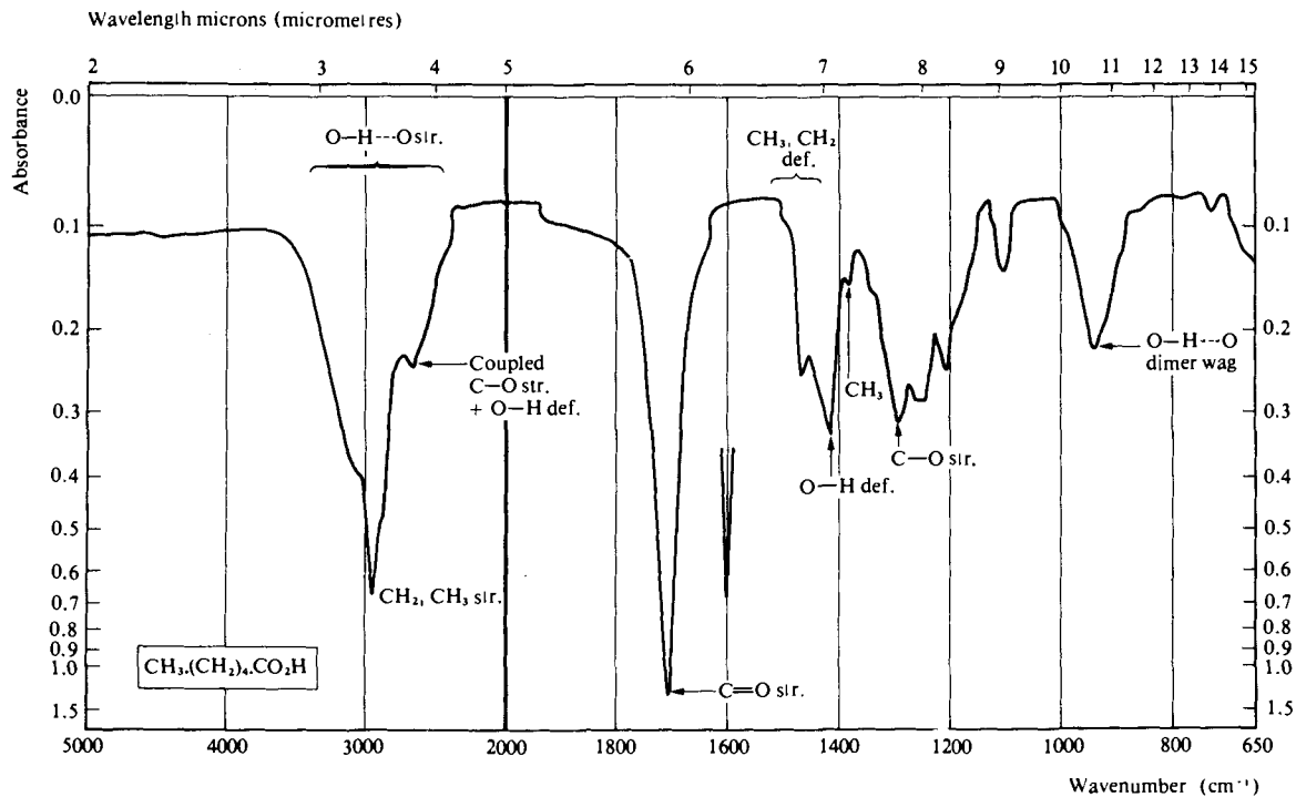
Fig. 3.31 Infrared spectrum of hexanoic acid recorded as a liquid film.
