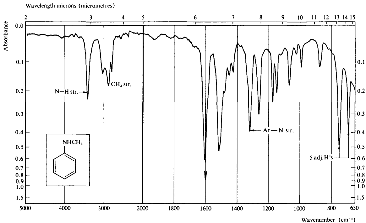
Fig. 3.27 Infrared spectrum of N -methylaniline recorded as a liquid film.
