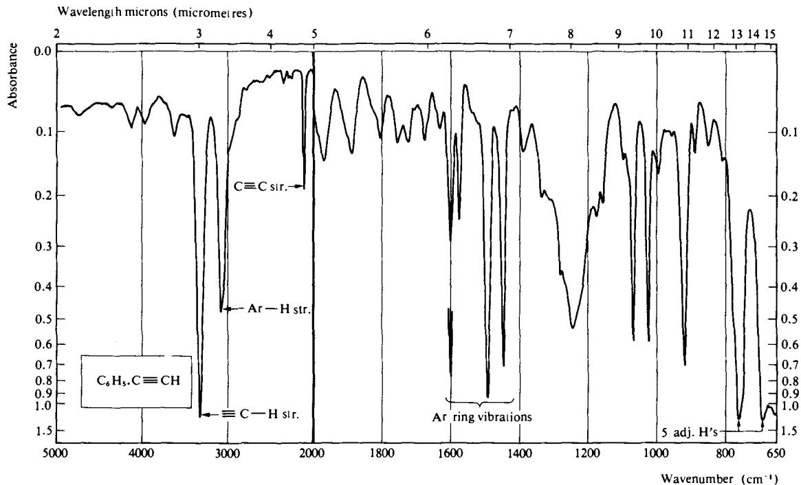
Fig. 3.19 Infrared spectrum of phenylacetylene recorded as a liquid film.
