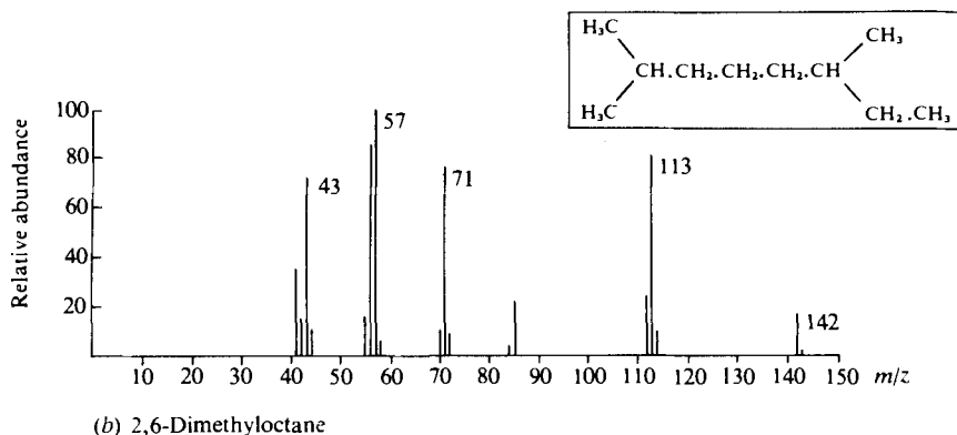
Fig. 3.79 Comparison of the mass spectra of straight chain and branched chain saturated hydrocarbons (a) decane; (b) 2,6-dimethyloctane.
