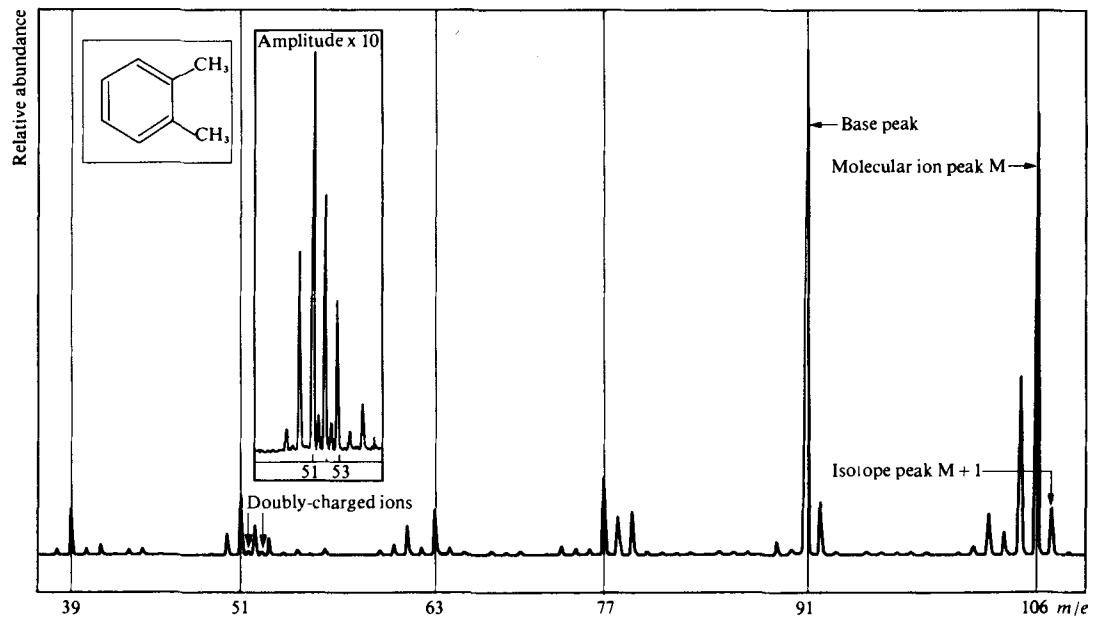
Fig. 3.75 Part of a low resolution mass spectrum of o -xylene.
