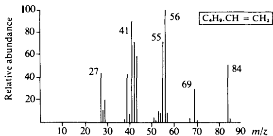
Fig. 3.80 Mass spectrum of hex-1-ene.
