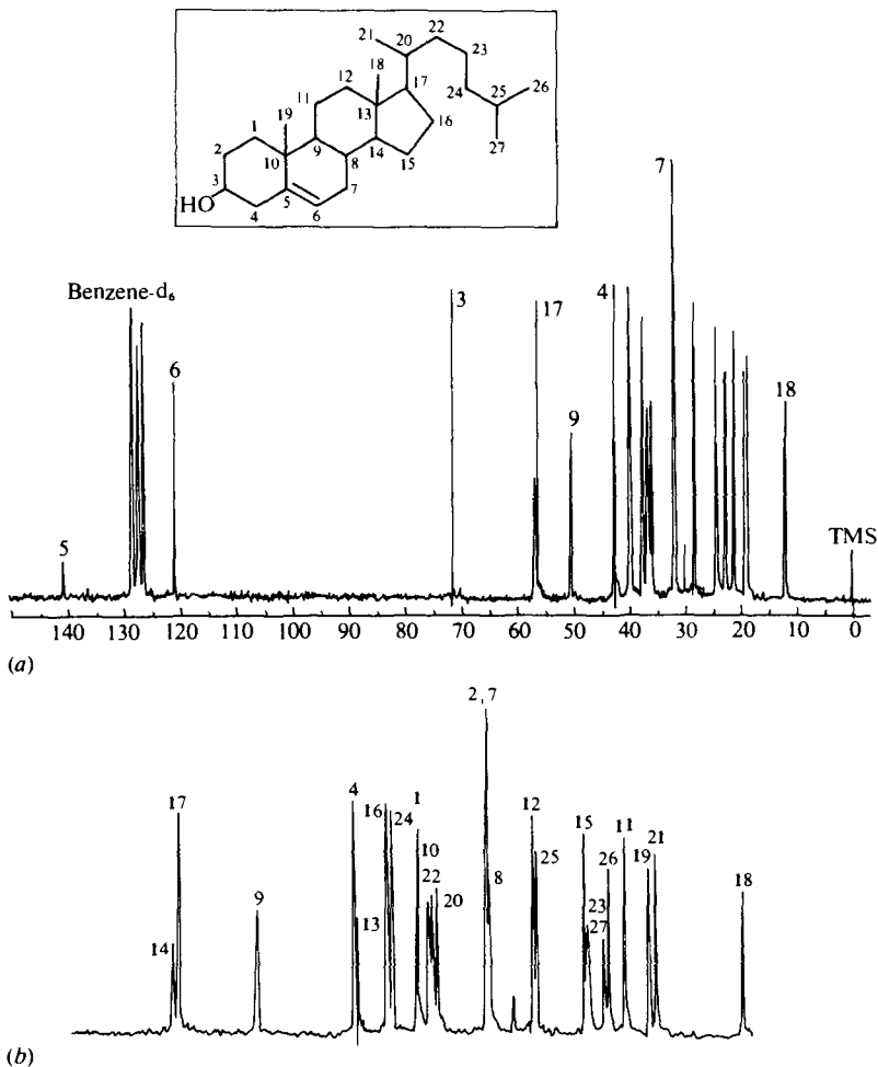
Fig. 3.56 (a) The 5000 Hz FT c.m.r. spectrum of 0.2 M cholesterol; pulse interval 0.4 seconds (total time, 3.4 hours). (b) The 1800 Hz plot expansion of the data in (a). All resonances assigned. Data reproduced from G. C. Levy and G. L. Nelson (1972). Carbon-13 Nuclear Resonance for Organic Chemistry . New York; Wiley-Interscience, pp. 164 and 165.
