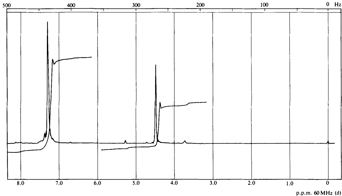
Fig. 3.66 Proton magnetic resonance spectrum of benzyl alcohol in CDCl 3 solution with added D 2 O. (See also Fig. 3.65).
