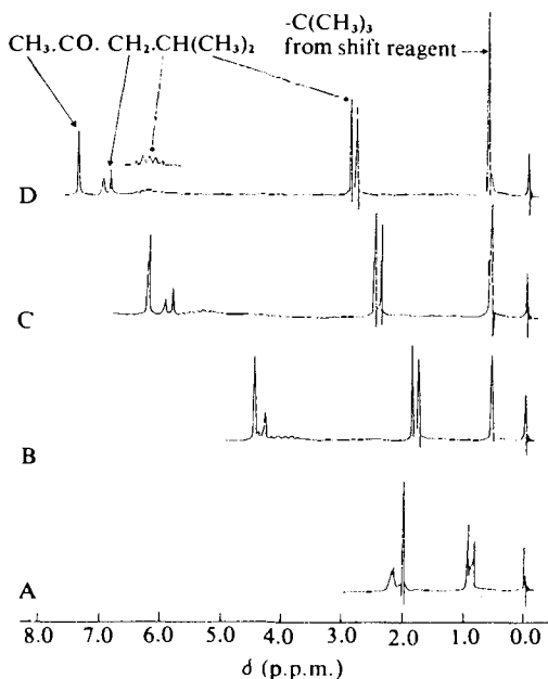
Fig. 3.69 60 MHz proton magnetic resonance spectra of methyl isobutyl ketone ( 10.6 \text{ mg} , 1.1 \times 10^{-4} \text{ mol} ) in \text{CCl}_4 ( 0.5 \text{ ml} ) containing various amounts of \text{Eu}(\text{pfd})_3 ; A, 0.0 \text{ mg} ; B, 13.5 \text{ mg} ; C, 21.1 \text{ mg} ; D, 29.0 \text{ mg} . Data reproduced from H. E. Francis and W. F. Wagner (1972), 'Induced Chemical Shifts in Organic Molecules; Intermediate Shift Reagents', Organic Magnetic Resonance , 4, 190 (Fig. 1), Heyden and Son Ltd.
