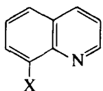
X = H, NO 2 , OH (100)
