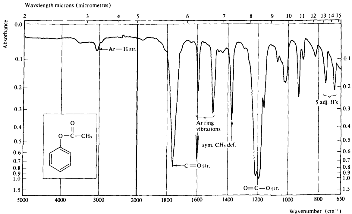
Fig. 3.32 Infrared spectrum of phenyl acetate recorded as a liquid film.
