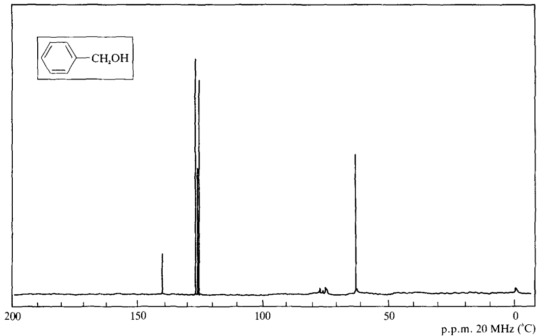
Fig. 3.53 ^{13}\text{C} nuclear magnetic resonance spectrum of benzyl alcohol in \text{CDCl}_3 ; sweep width 200 p.p.m. Data reproduced from the Standard Carbon-13NMR Spectra Collection, © Sadtler Research Laboratories, Division of Bio-Rad Laboratories, Inc.
