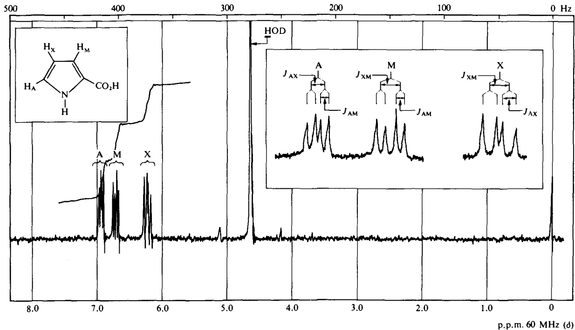
Fig. 3.61 Proton magnetic resonance spectrum of pyrrole-2-carboxylic acid in D_2O/NaOD solution; reference DSS, and sweep width 500 Hz. Inset: expansion of aromatic proton absorptions, sweep width 50 Hz.
