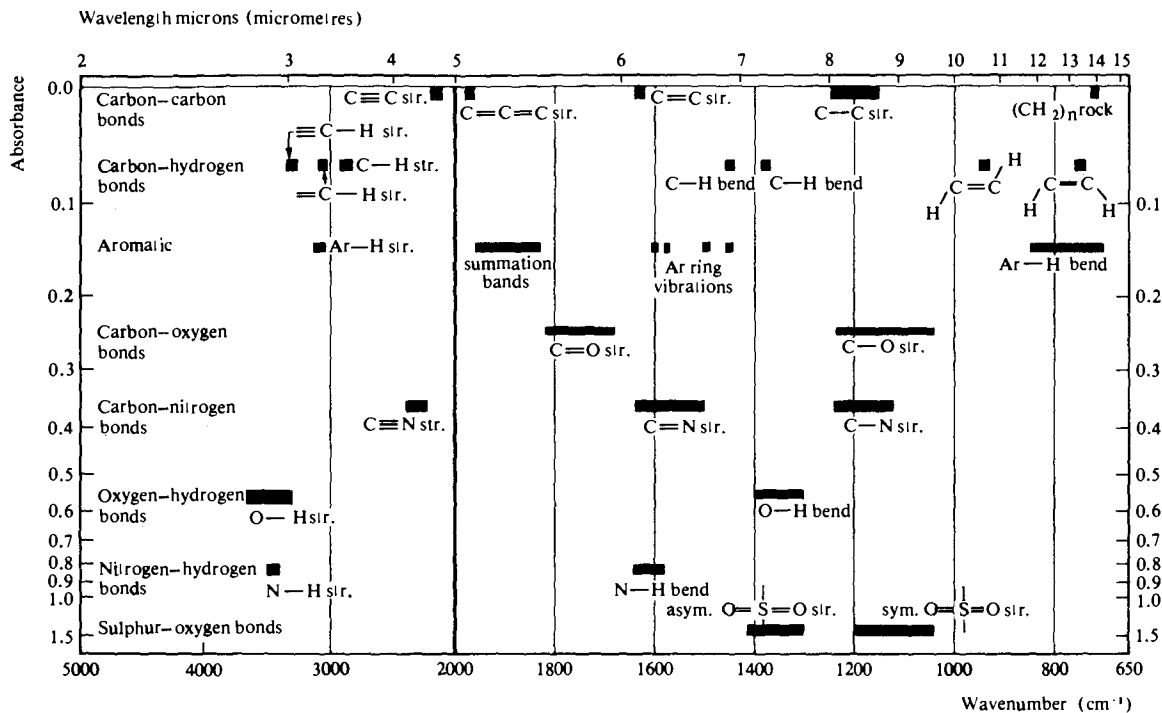
Fig. 3.10 Simplified correlation chart of absorption positions of important bonding types.
