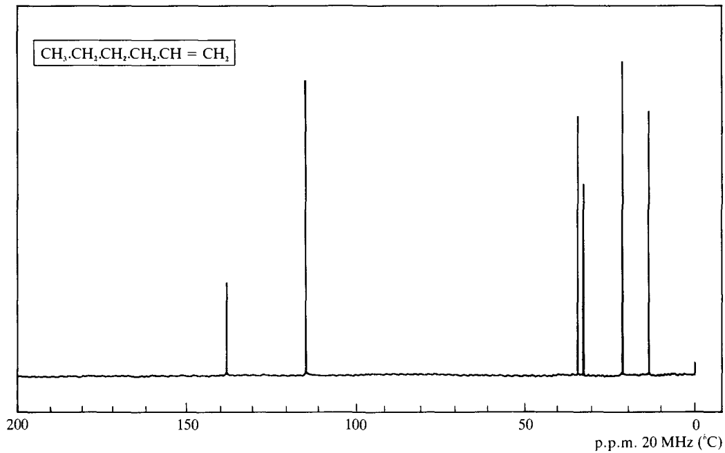
Fig. 3.51 13 C nuclear magnetic resonance spectrum at hex-1-ene in CDCl 3 ; sweep width 200 p.p.m. Data reproduced from the Standard Carbon-13NMR Spectra Collection, © Sadtler Research Laboratories, Division of Bio-Rad Laboratories, Inc.
