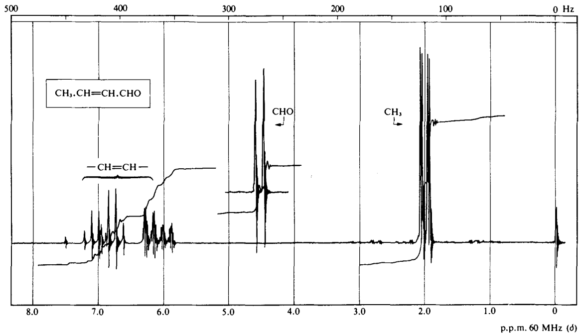
Fig. 3.72 Proton magnetic resonance spectrum of crotonaldehyde in \text{CDCl}_3 , solution; sweep offset 300 Hz, sweep width 500 Hz.
