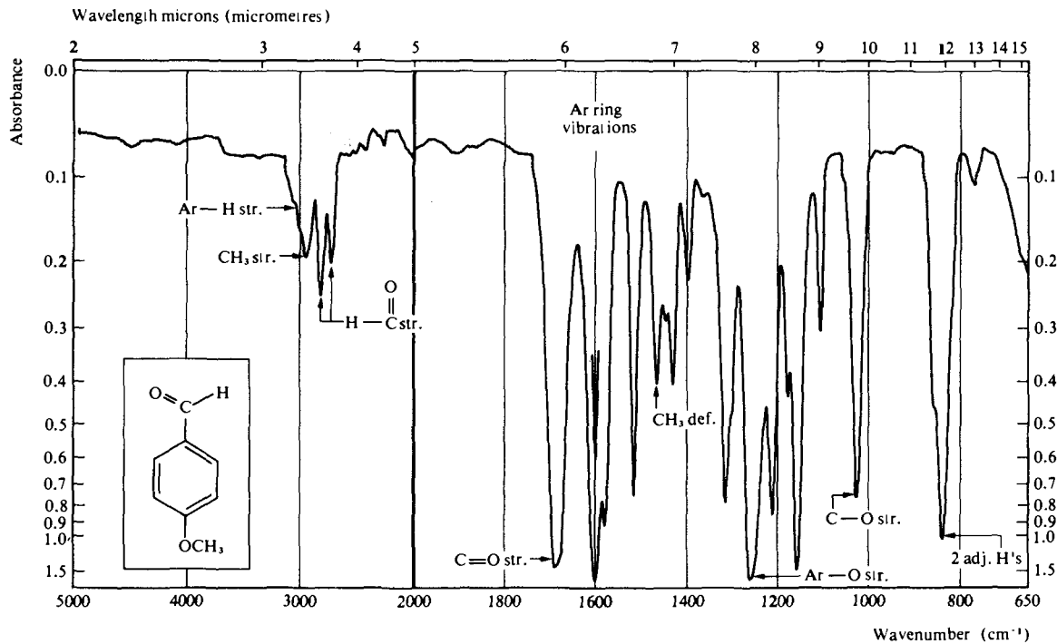
Fig. 3.30 Infrared spectrum of anisaldehyde recorded as a liquid film.
