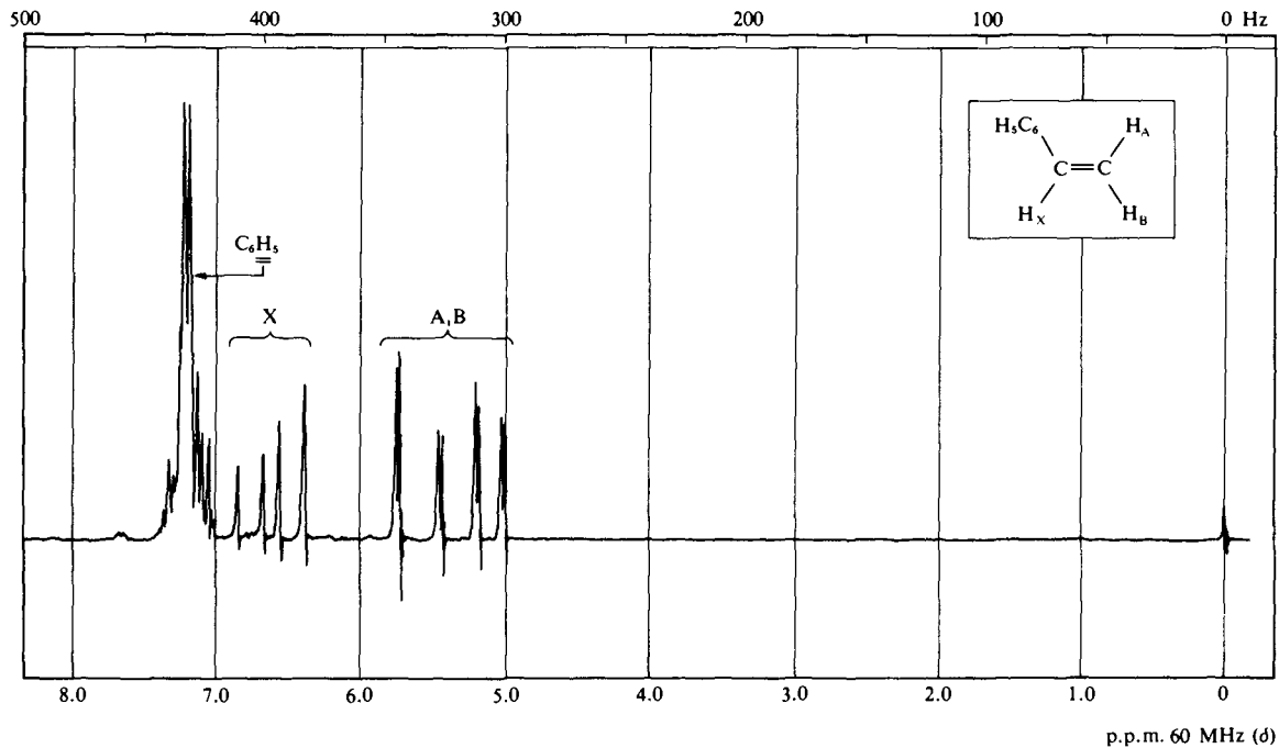
Fig. 3.62 Proton magnetic resonance spectrum of styrene in \text{CDCl}_3 solution; sweep width 500 Hz.
