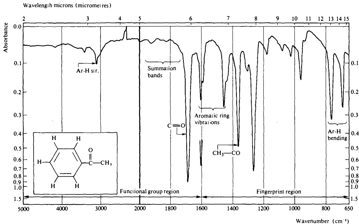
Fig. 3.9 Infrared spectrum of acetophenone recorded as a thin film.
