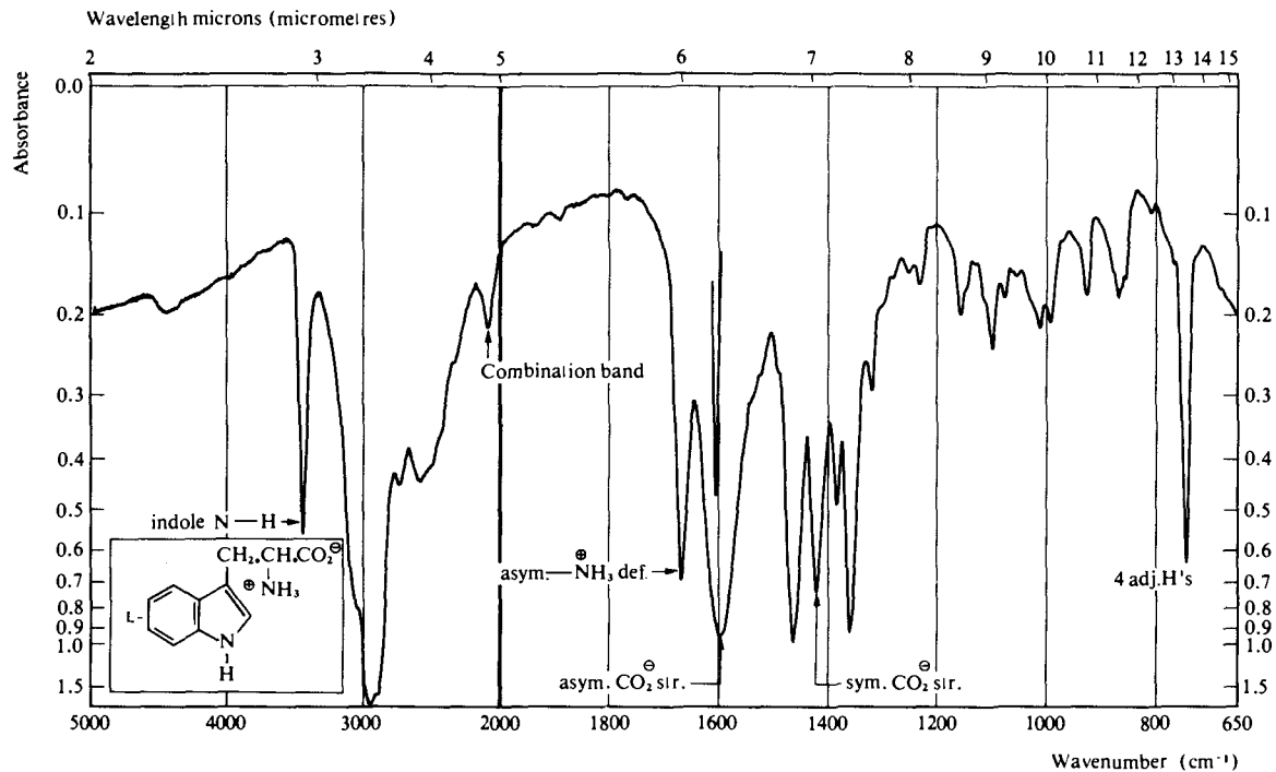
Fig. 3.37 Infrared spectrum of L-tryptophan recorded as a Nujol mull.
