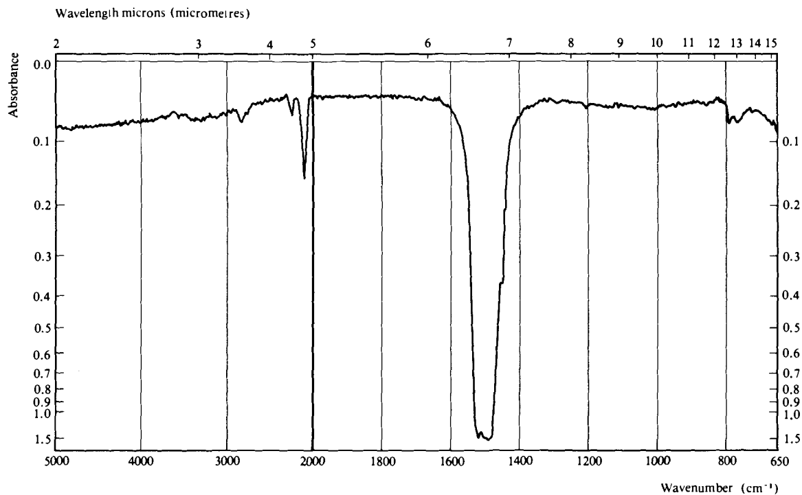
Fig. 3.5(c) Carbon disulphide (recorded in a variable path length cell, set at 0.015 mm path length).
