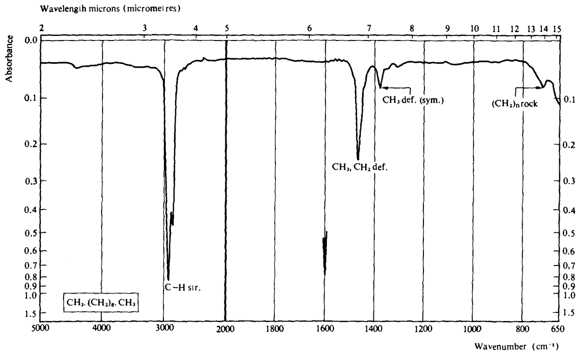
Fig. 3.12 Infrared spectrum of decane recorded as a liquid film on a prism spectrophotometer.
