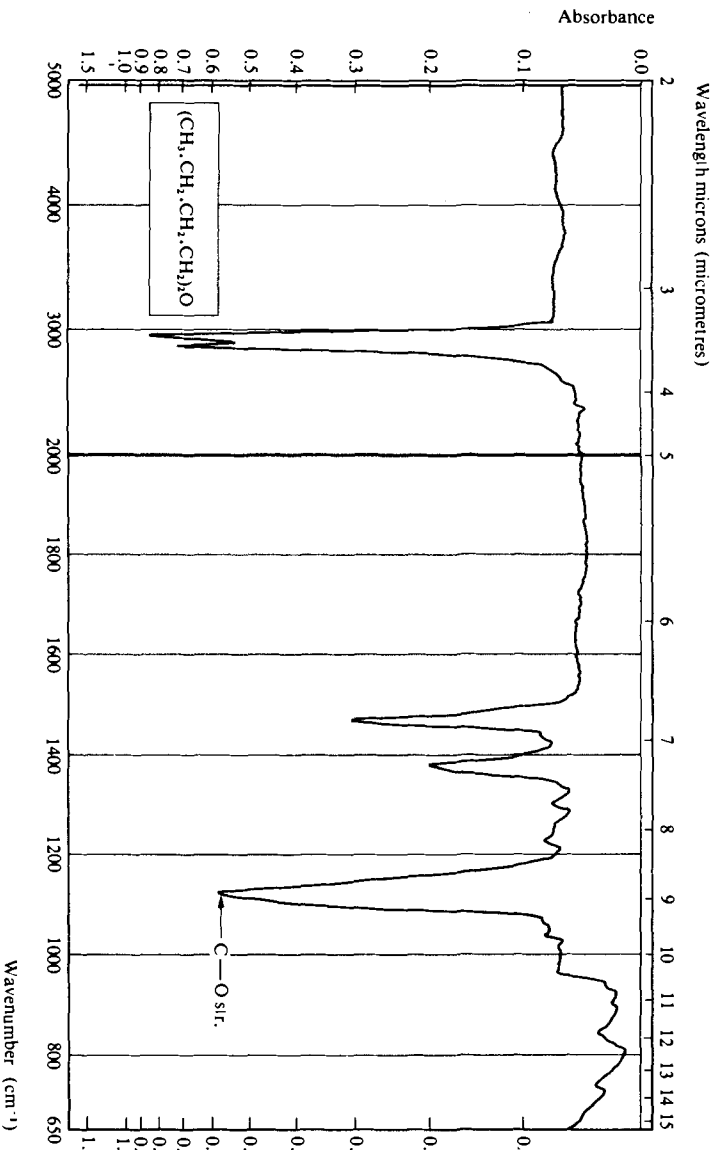
Fig. 3.24 Infrared spectrum of dibutyl ether recorded as a liquid film.
