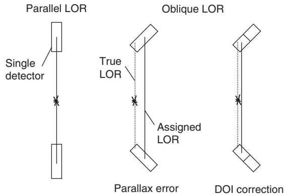
Figure 27.7 Depth-of-interaction (DOI) correction. Photons with an oblique trajectory path may cause a parallax error. The true LOR may not correspond to the assigned LOR, which is defined to intersect the detector’s center-of-mass. DOI measurements can partially correct for this error by deriving information about the location of the \gamma photon interaction within a crystal element. This can be achieved by splitting up a single detector element into several regions with separate data readouts.
