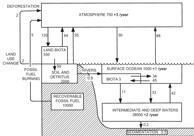
Figure 2.4 Global carbon reservoirs (gigatonnes of carbon (GtC): where 1 Gt = 10^9 metric tons = 10^{12} kg) and gross annual fluxes (GtC yr -1 ). Numbers emboldened in the reservoirs suggest the net annual accumulation due to anthropogenic causes.
