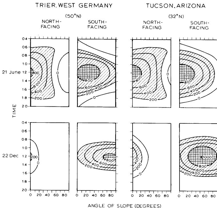
Figure 3.20 Average direct beam solar radiation ( \text{W m}^{-2} ) incident at the surface under cloudless skies at Trier, West Germany, and Tucson, Arizona, as a function of slope, aspect, time of day and season of year.
