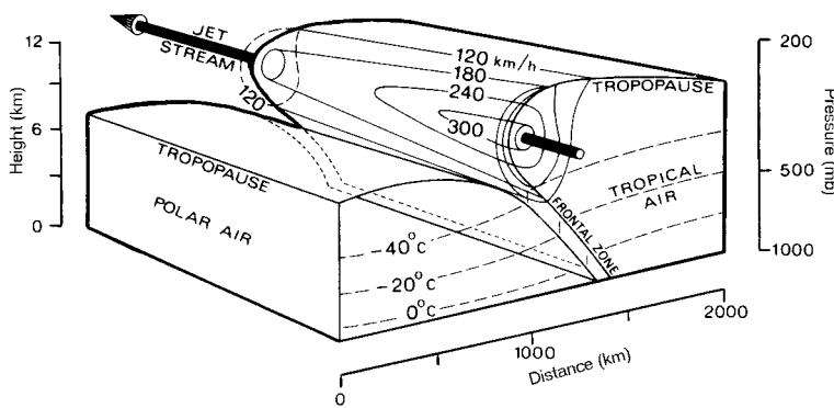
Figure 7.7 Structure of the mid-latitude frontal zone and associated jet stream showing generalized distribution of temperature, pressure and wind velocity.
