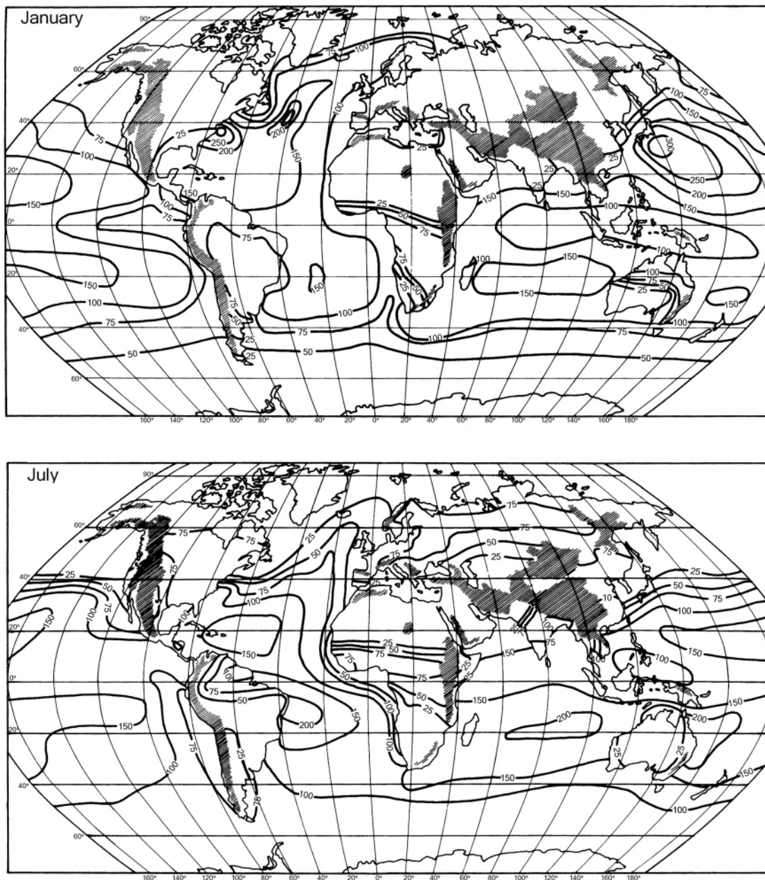
Figure 4.6 Mean evaporation (mm) for January and July.
