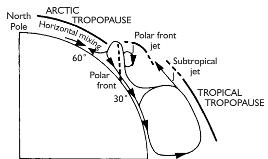
Figure 7.20 General meridional circulation model for the northern hemisphere in winter.
