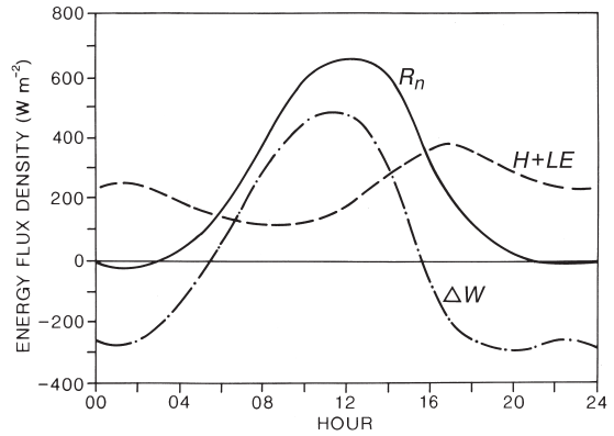
Figure 12.5 Average diurnal variation of the energy balance components in and above the tropical Atlantic Ocean during the period 20 June to 2 July 1969.
