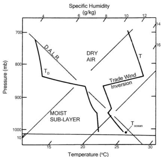
Figure 11.5 The vertical structure of trade wind air between the surface and 700 mb in the central equatorial Atlantic, 6 to 12 February 1969, showing air temperature ( T ), dew-point temperature ( T D ). The specific humidity can be read off the upper scale.
