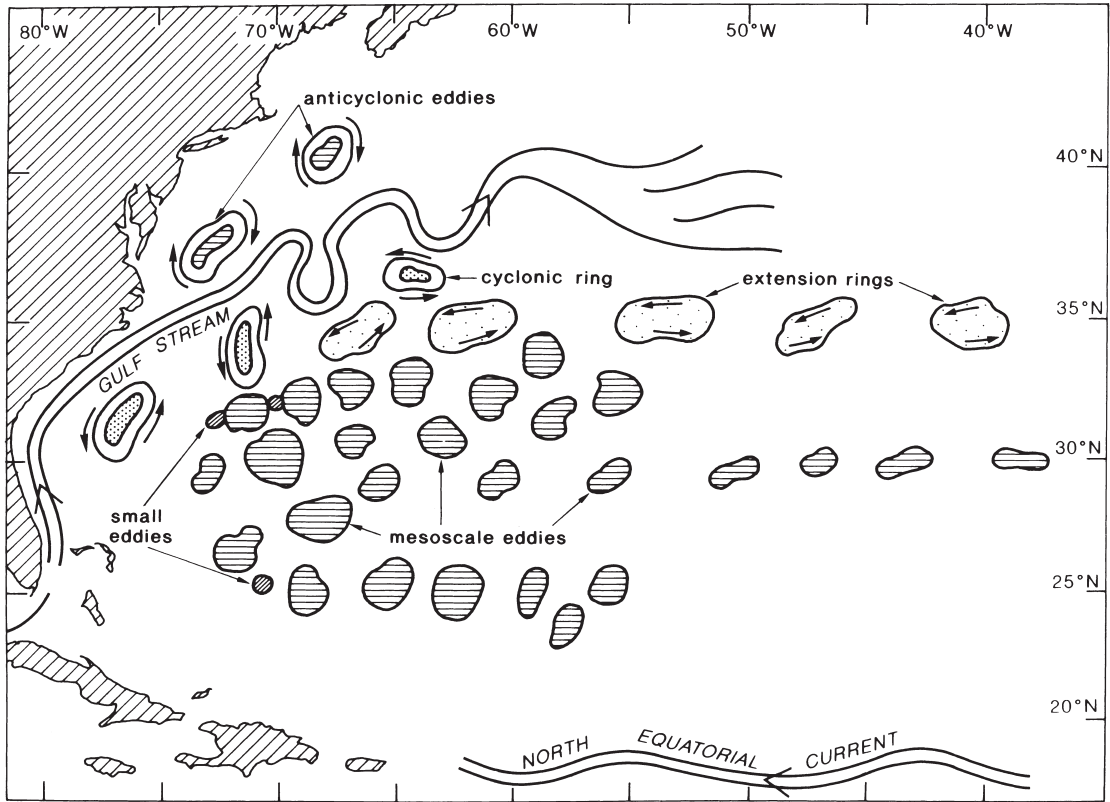
Figure 7.30 Schematic map of the western North Atlantic showing the major types of ocean surface circulation.
