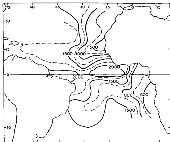
Figure 11.6 The height (in metres) of the base of the trade wind inversion over the tropical Atlantic.
