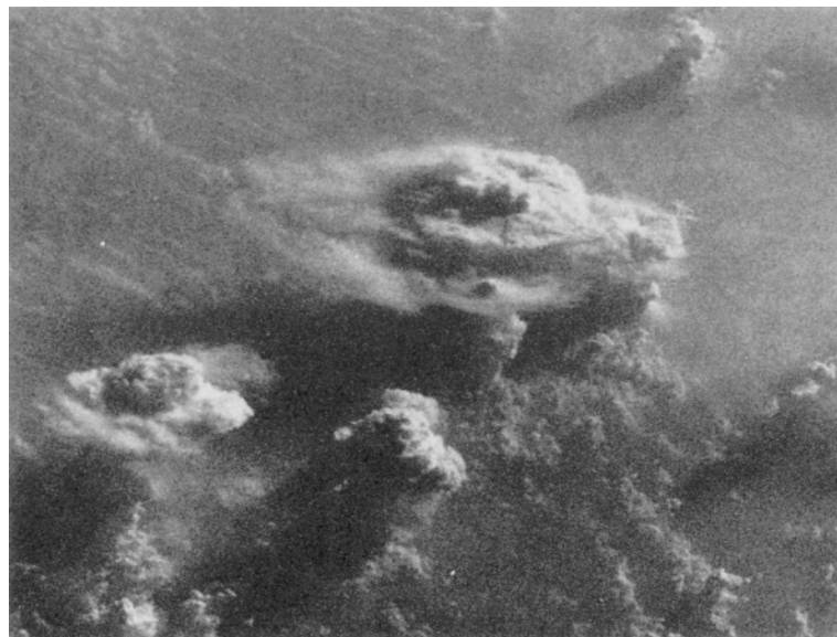
Plate 4 Cumulus towers with powerful thunderstorms along the ITCZ over Zaire photographed in April 1983 from the space shuttle at an elevation of 280 km. The largest tower shows a double mushroom cap reaching to more than 15,240 m and the symmetrical form of the caps indicates a lack of pronounced airflow at high levels (courtesy of NASA).
