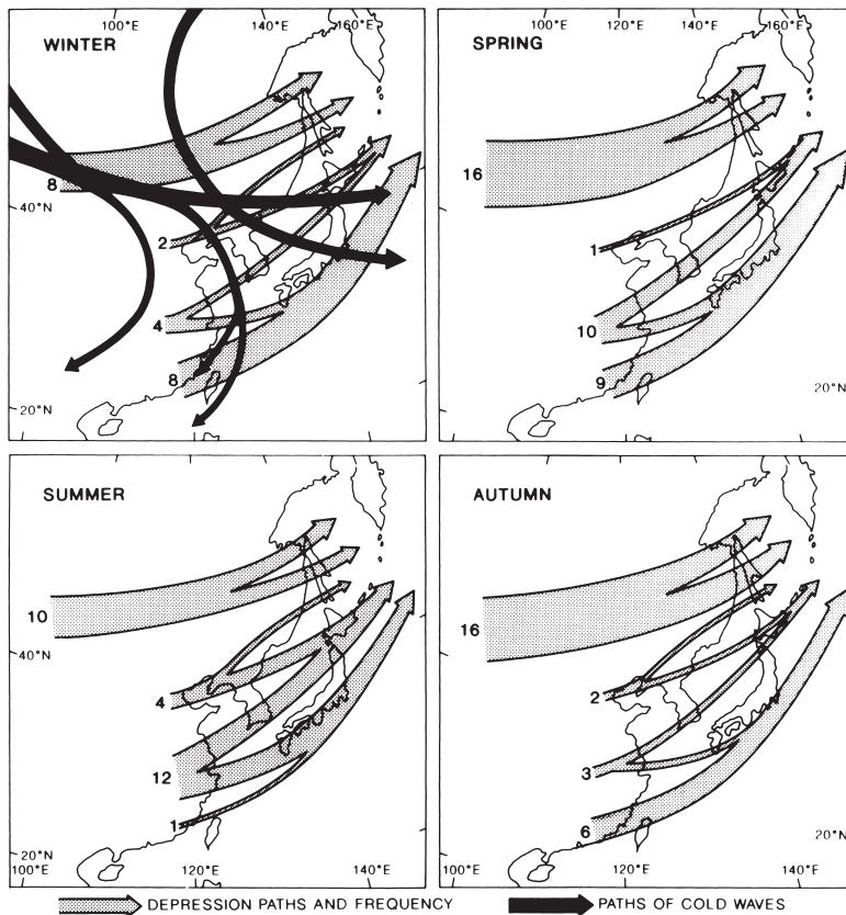
Figure 11.22 Seasonal depression paths and frequencies over China and Japan, together with typical paths of winter cold waves.
