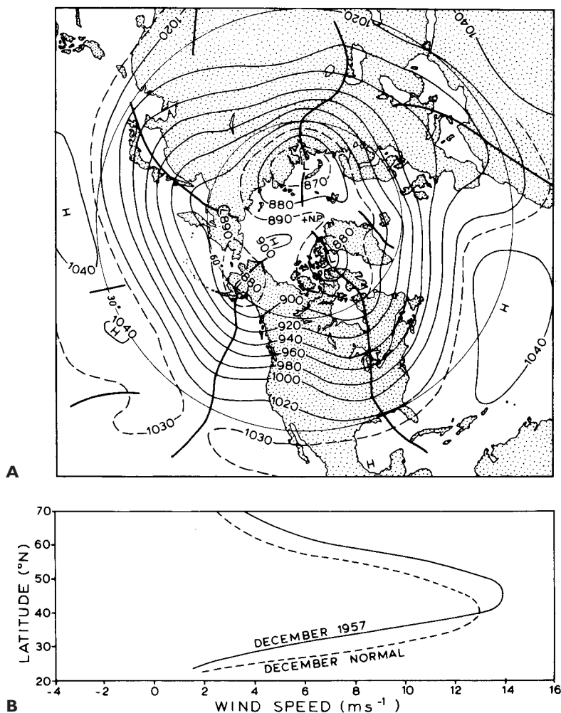
Figure 7.24 (A) Mean 700-mb contours (in tens of feet) for December 1957, showing a fast, westerly, small-amplitude flow typical of a high zonal index. (B) Mean 700-mb zonal wind speed profiles ( m s^{-1} ) in the western hemisphere for December 1957, compared with those of a normal December. The westerly winds were stronger than normal and displaced to the north.
