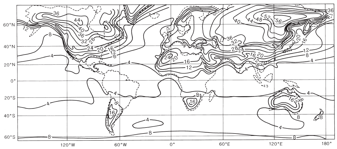
Figure 3.24 The mean annual temperature range (°C) at the earth's surface. Source: Monin, Crowley and North (1991). Courtesy of the World Meteorological Organization.
