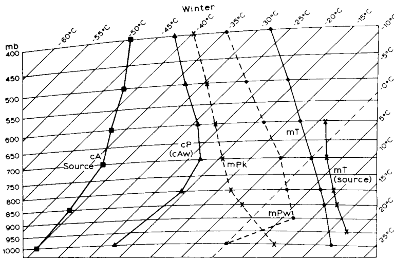
Figure 9.3 The average vertical temperature structure for selected airmasses affecting North America at about 45 to 50°N, recorded over their source areas or over North America in winter.
