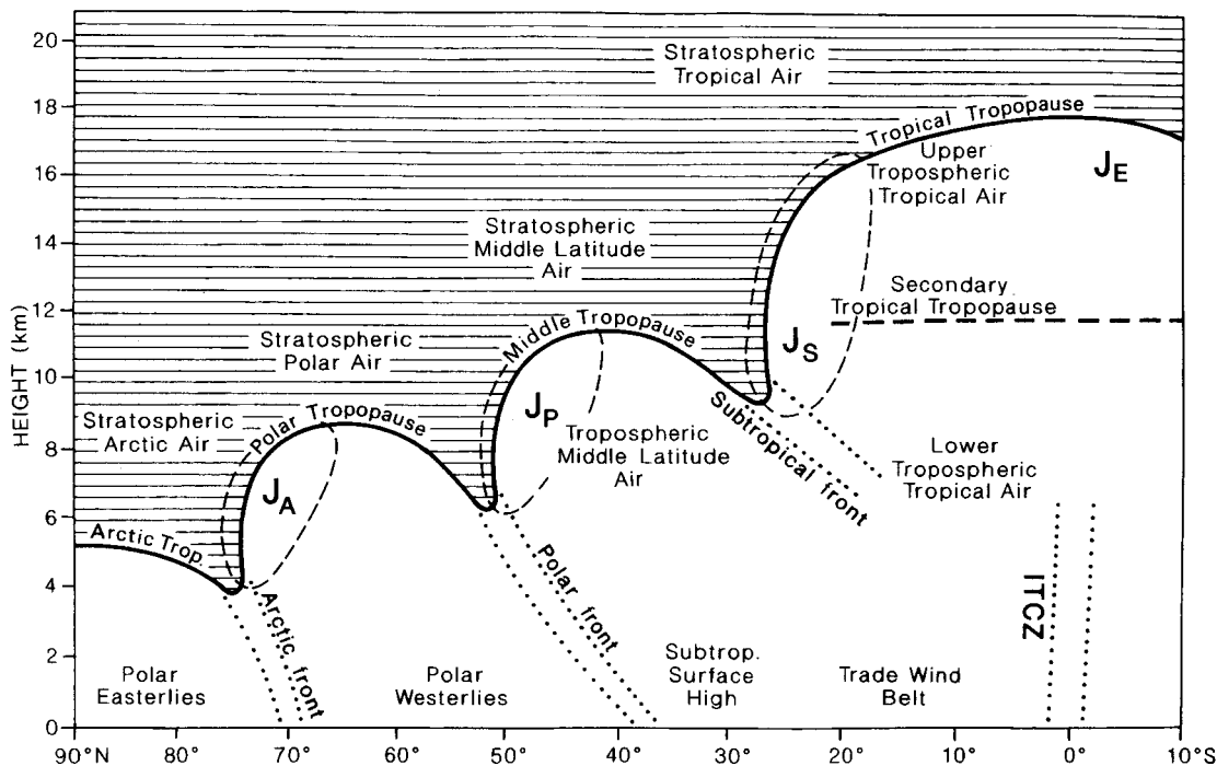
Figure 7.8 The meridional structure of the tropopause and the primary frontal zones. The 40 \text{ m s}^{-1} isotach (dashed) encloses the Arctic ( J_A ), polar ( J_P ) and subtropical ( J_S ) jet streams. The tropical easterly ( J_E ) jet stream is also shown. Occasionally, the Arctic and polar or the polar and subtropical fronts and jet streams may merge to form single systems in which about 50 per cent of the pole-to-equator mid-tropospheric pressure gradient is concentrated into a single frontal zone approximately 200 km wide. The tropical easterly jet stream may be accompanied by a lower easterly jet at about 5 km elevation. (see chapter 11 C, D).
