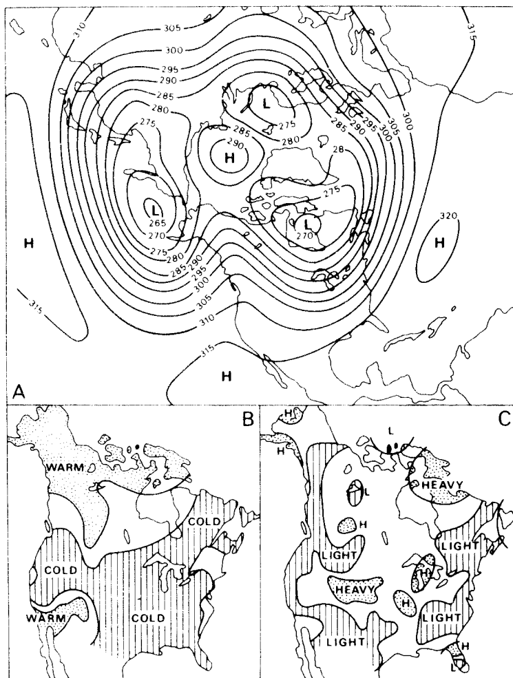
Figure 8.8 Actual North American weather for December 1985 (cf. Figure 8.7). Observed 700-mb contours (5 gp dam) corresponding to Figure 8.7A, B and C. Observed temperature (B) and precipitation (C), corresponding to Figure 8.7B and C.
