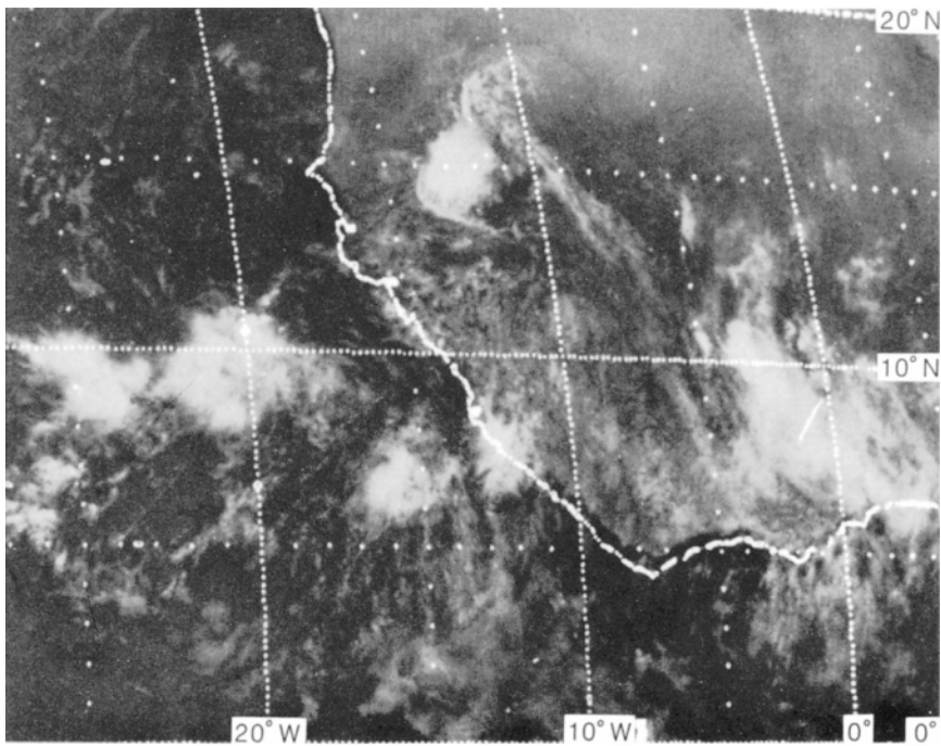
Plate 29 Visible satellite image showing five large tropical cloud clusters topped by cirrus shields situated between latitudes 5^{\circ} and 10^{\circ} N in the vicinity of West Africa, together with one squall line cloud cluster at 15^{\circ} N having a well-defined arc cloud squall line on its leading (southwest) edge. Taken by SMS-1 satellite at 11:30 hours GMT on 5 September 1974 (courtesy of NOAA).
