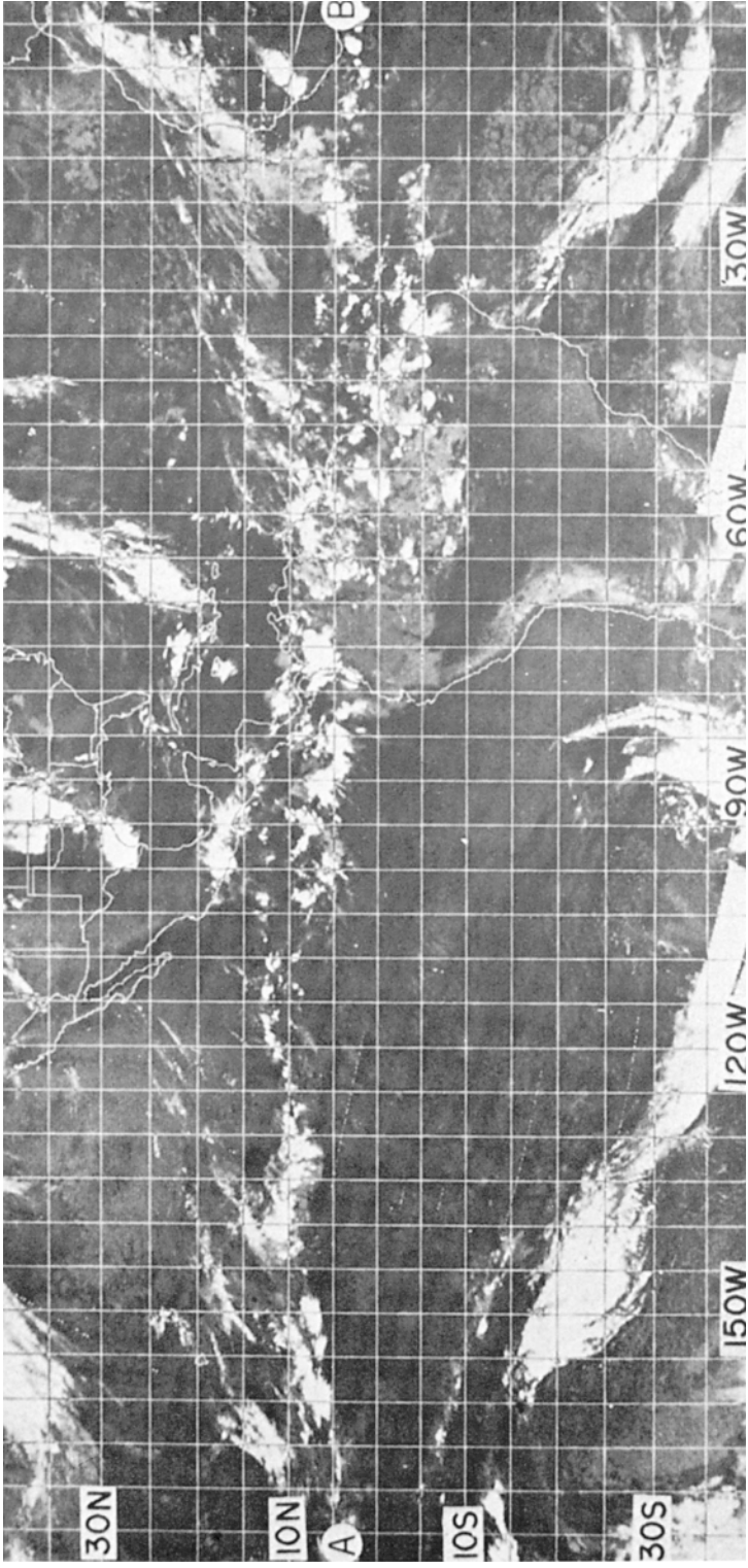
Plate 24 Infra-red photograph showing the intertropical convergence zone on 1 June 1971, along which active thunderstorms appear as bright spots. There is also a cyclonic cloud band in the western South Pacific representing the South Pacific convergence zone (NOAA-1 photograph, World Meteorological Organization 1973).
