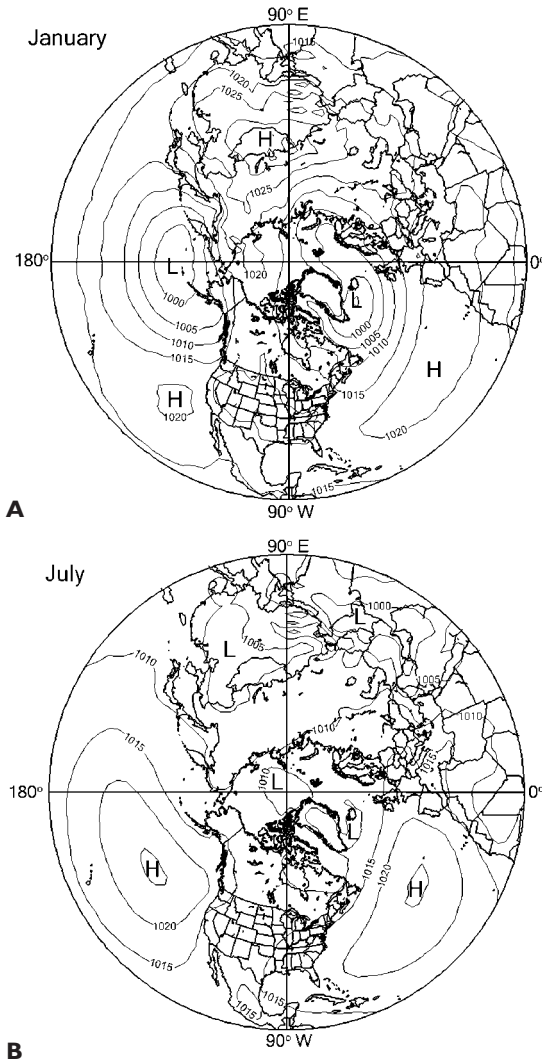
Figure 7.9 The mean sea-level pressure distribution (mb) in January and July for the northern hemisphere, 1970 to 1999.
