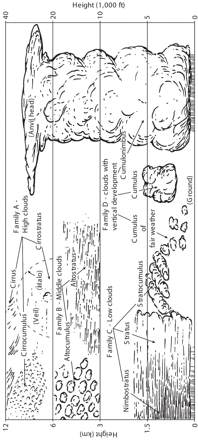
Figure 5.10 The ten basic cloud groups classified according to height and form.
