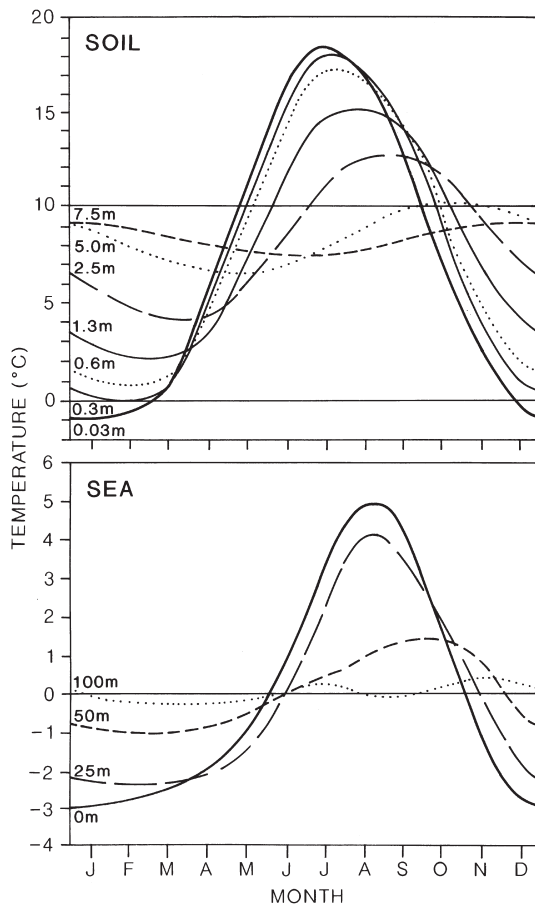
Figure 3.16 Annual variation of temperature at different depths in soil at Kaliningrad, European Russia (above) and in the water of the Bay of Biscay (at approximately 47° N, 12°W) (below), illustrating the relatively deep penetration of solar energy into the oceans as distinct from that into land surfaces. The bottom figure shows the temperature deviations from the annual mean for each depth.
