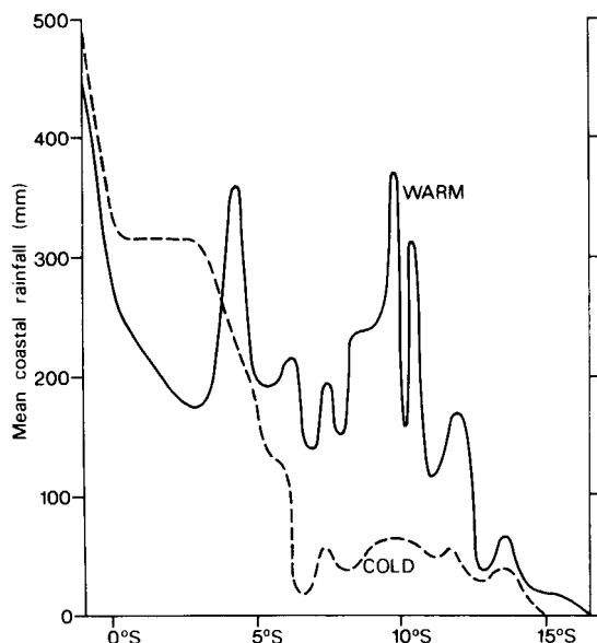
Figure 11.55 March rainfall along the southwestern coast of Africa (Gabon and Angola) associated with warm and cold sea-surface conditions.
