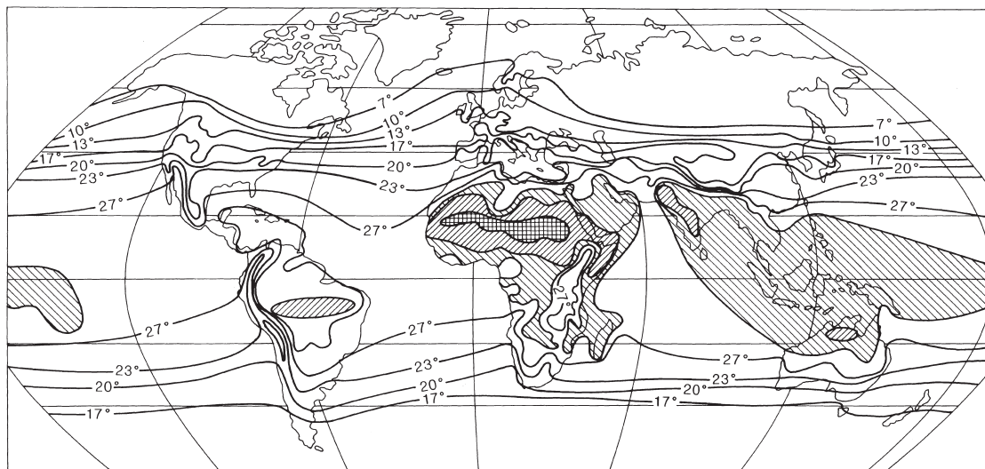
Figure 3.10 Mean daily maximum shade air temperature (C).
