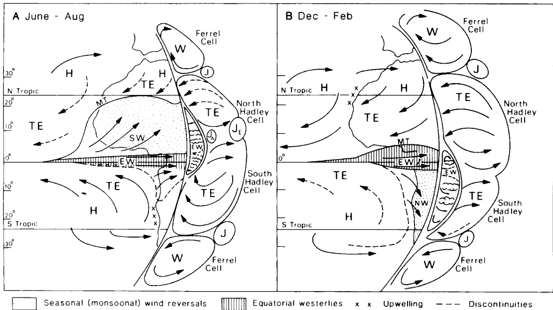
Figure 11.38 The major circulation in Africa in (A) June to August and (B) December to February. H: subtropical high-pressure cells; EW: equatorial westerlies (moist, unstable but containing the Congo high-pressure ridge); NW: the northwesterlies (summer extension of EW in the southern hemisphere); TE: tropical easterlies (trades); SW: southwesterly monsoonal flow in the northern hemisphere; W: extratropical westerlies; J: subtropical westerly jet stream; J_A and J_E : the African easterly and tropical easterly jet streams; and MT: monsoon trough.
