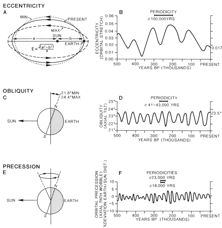
Figure 13.3 The astronomical (orbital) effects on the solar irradiance and their timescales over the past 500,000 years. (A) and (B) Eccentricity or orbital stretch. (C) and (D) Obliquity or axial tilt. (E) and (F) Precession or axial path wobble.
