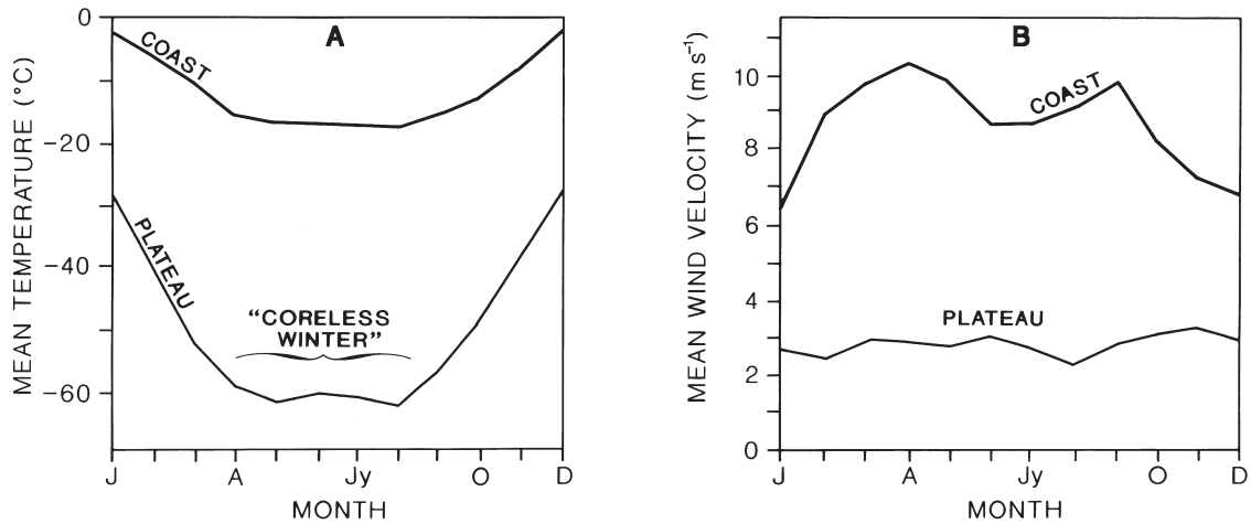
Figure 10.39 Annual course of (A) mean monthly air temperature (°C) and (B) wind speed ( \text{m s}^{-1} ) for 1980 to 1989 at Dome C (3280 m), 74.5°S, 123.0°E (plateau) and D–10, an automatic weather station at 240 m, 66.7°S, 139.8°E (coast).
