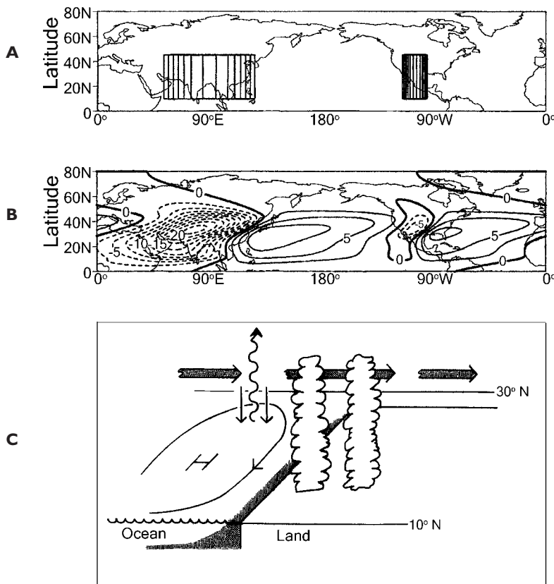
Figure 7.21 Schematic illustrations of suggested processes that form/maintain the northern subtropical anticyclones in summer. (A) Boxes where summer heat sources are imposed in the atmospheric model; (B) Pattern of resultant stationary planetary waves (solid/dashed lines denote positive/negative height anomalies) (Chen et al. , 2001); (C) Schematic of the circulation elements proposed by Hoskins (1996). Monsoon heating over the continents with descent west- and poleward where there is interaction with the westerlies. The descent leads to enhanced radiative cooling acting as a positive feedback and to equatorward motion; the latter drives Ekman ocean drift and upwelling.
