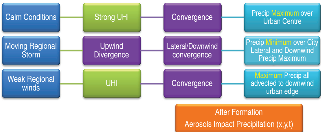
FIGURE A.4 Processes that influence precipitation resulting from summer thunderstorms. Figure created based on presentation by RD Bornstein (2011) Urban impacts on summer thunderstorms. International Workshop on Urban Weather and Climate. Beijing, July 12-15, 2011.
