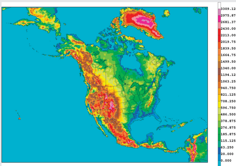
The NCEP Regional Reanalysis domain and its 32 km topography. Terrain elevation (m) is indicated by the color scale at the right. SOURCE: Mesinger et al., 2006. (c) American Meteorological Society. Reprinted with permission.
