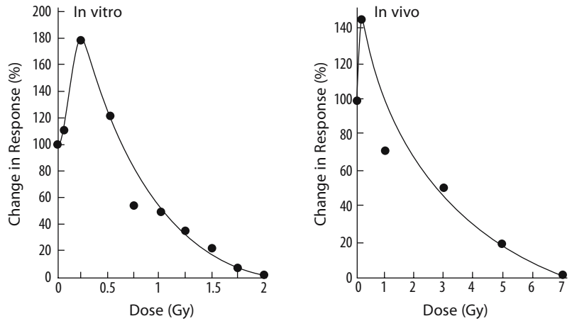
Fig. 3.4. Immune system response to radiation. Mouse splenic cells primed with antigenic sheep red blood cells (MAKINODAN and JAMES 1996)
