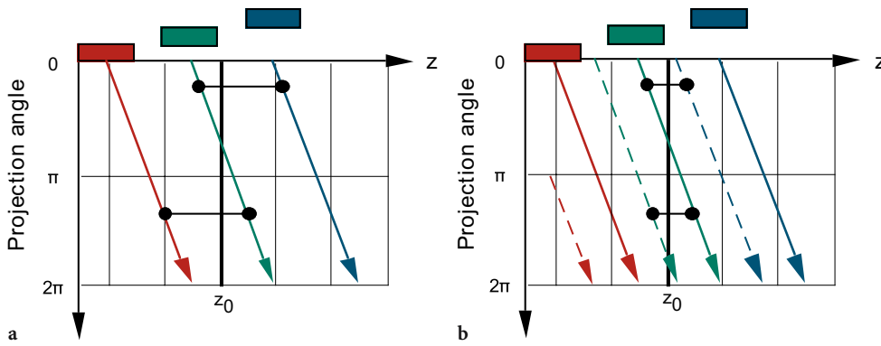
Fig. 4.16a,b. The most common interpolation schemes for single-slice scanners are either 360° LI (a) or 180° LI (b). Both schemes employ two data points closest to the position z_0 of the reconstructed slice for each projection angle. Making use of the virtual ( complementary ) data ( dashed lines ), a shorter interpolation distance is achieved with 180° LI, resulting in a narrower slice profile
