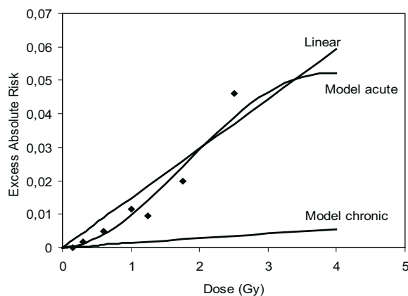
Fig. 2.13. An illustration of how a linear-quadratic model might be fitted to the data (shown in Fig. 2.1) for the acute exposure of the atomic bomb survivors compared with a linear interpretation. The lower straight line shows the risk that would be predicted by the model for chronic exposure
