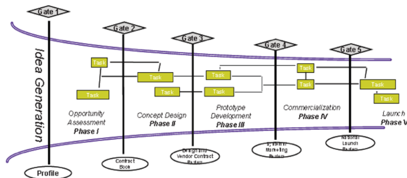
Figure 21: Phase gate model
