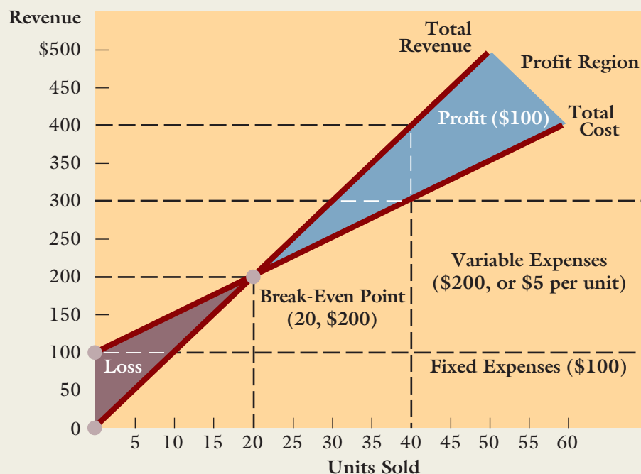
EXHIBIT 17-5 Cost-Volume-Profit Graph
