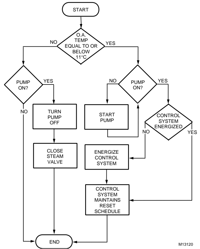
Fig. 18. Flowchart Example.
