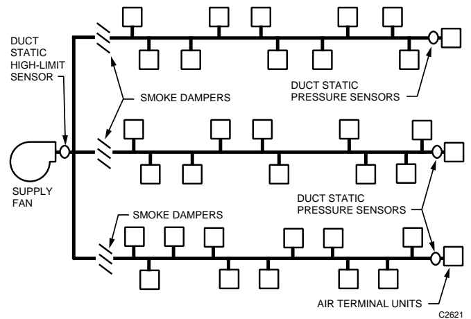
Fig. 26. Controlling Static High-Limit.
