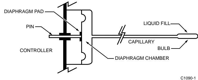
Fig. 9. Remote-Bulb Temperature Sensor.
