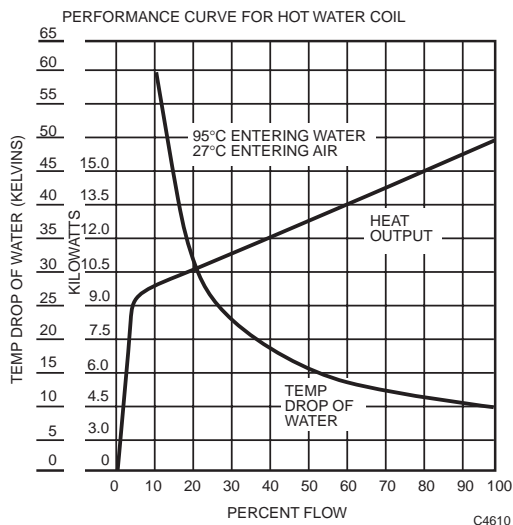
Fig. 91. Effect of Flow Control on Hot Water Coil Heat Output.
