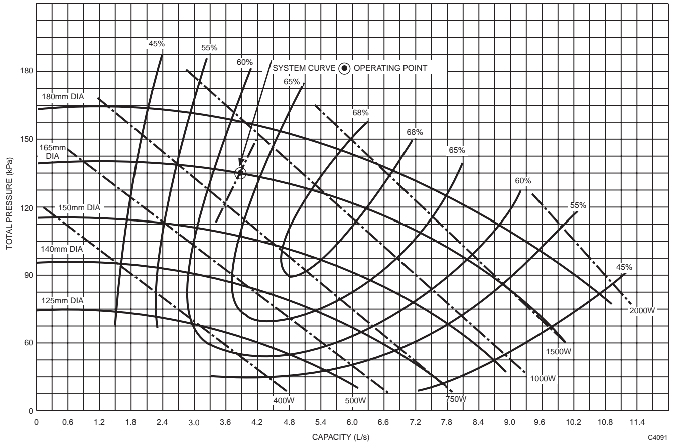
Fig. 55. Pump Curve for 1750 RPM Operation.
