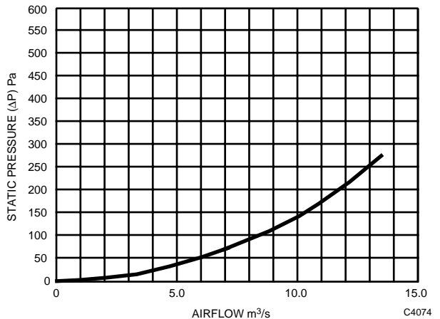
Fig. 6. System Curve.
