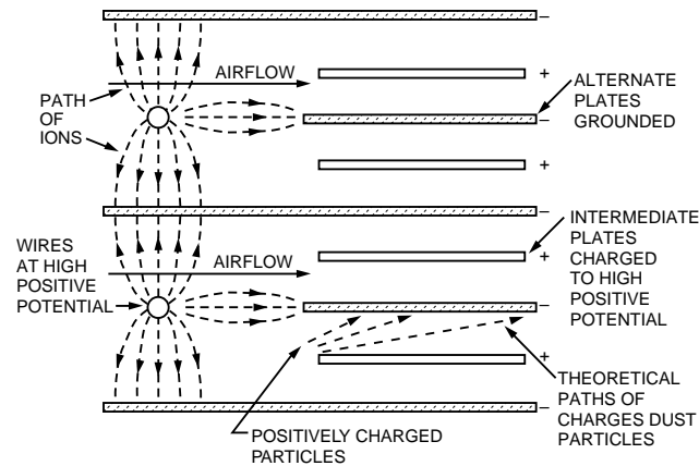
Fig. 18. Electrostatic Filter.
