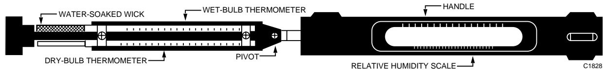
Fig. 1. Sling Psychrometer.
