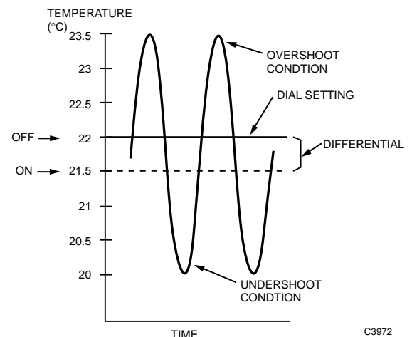
Fig. 21. Typical Operation of Basic Two-Position Control.
