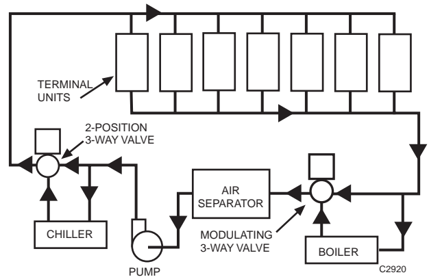
Fig. 99. Two-Pipe Dual-Temperature System.
