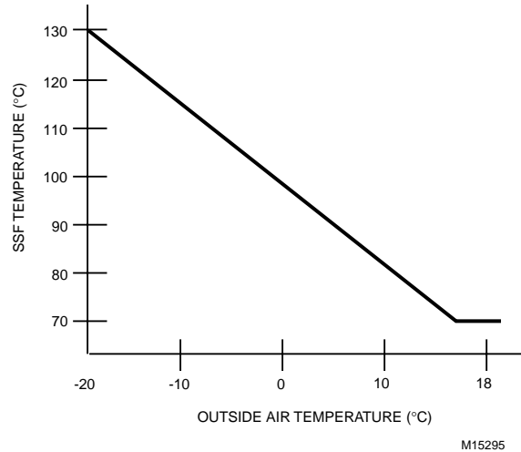
Fig. 139. SSF Temperature Reset Schedule.
