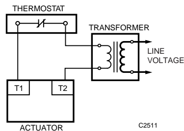
Fig. 10. Series 80 Actuator Application.
