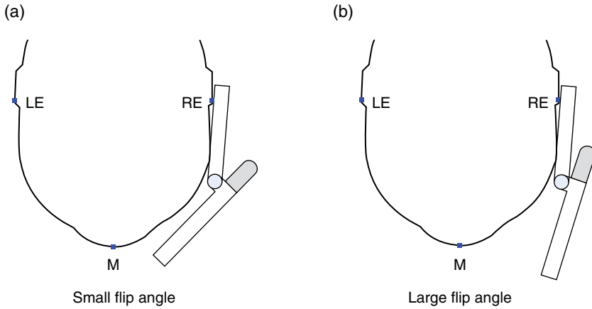
Figure 6.16 Flip angle on a clam shell phone, stubby antenna.
