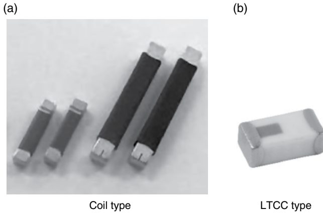
Figure 4.51 Monopole-type ceramic antennas (not to scale). (a) (Source: Panasonic Corporation.) and (b) (Source: Reproduced with permission of Johanson Technology.)
