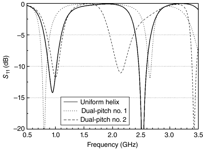
Figure 3.39 Simulated reflection coefficients.
