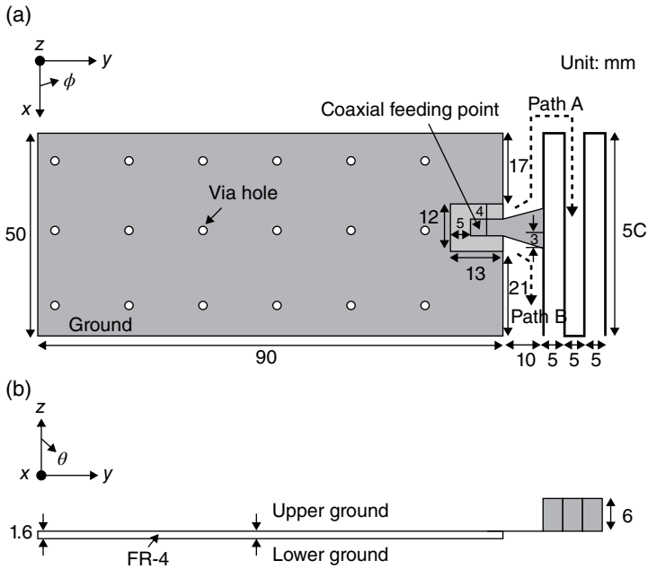
Figure 3.86 Multiband monopole antenna. (Source: Kim et al. [27]. Reproduced with permission of IET.)
