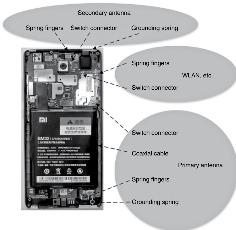
Figure 4.110 Xiaomi 4’s PCB. (Source: Reproduced with permission of Xiaomi, Inc.)
