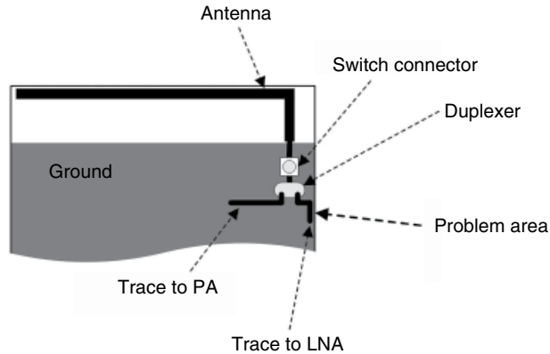
Figure 5.32 An example of incorrect routing.
