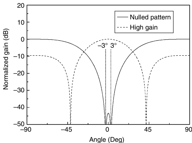
Figure 4.85 Send independent signal to individual receiver by using nulled pattern.
