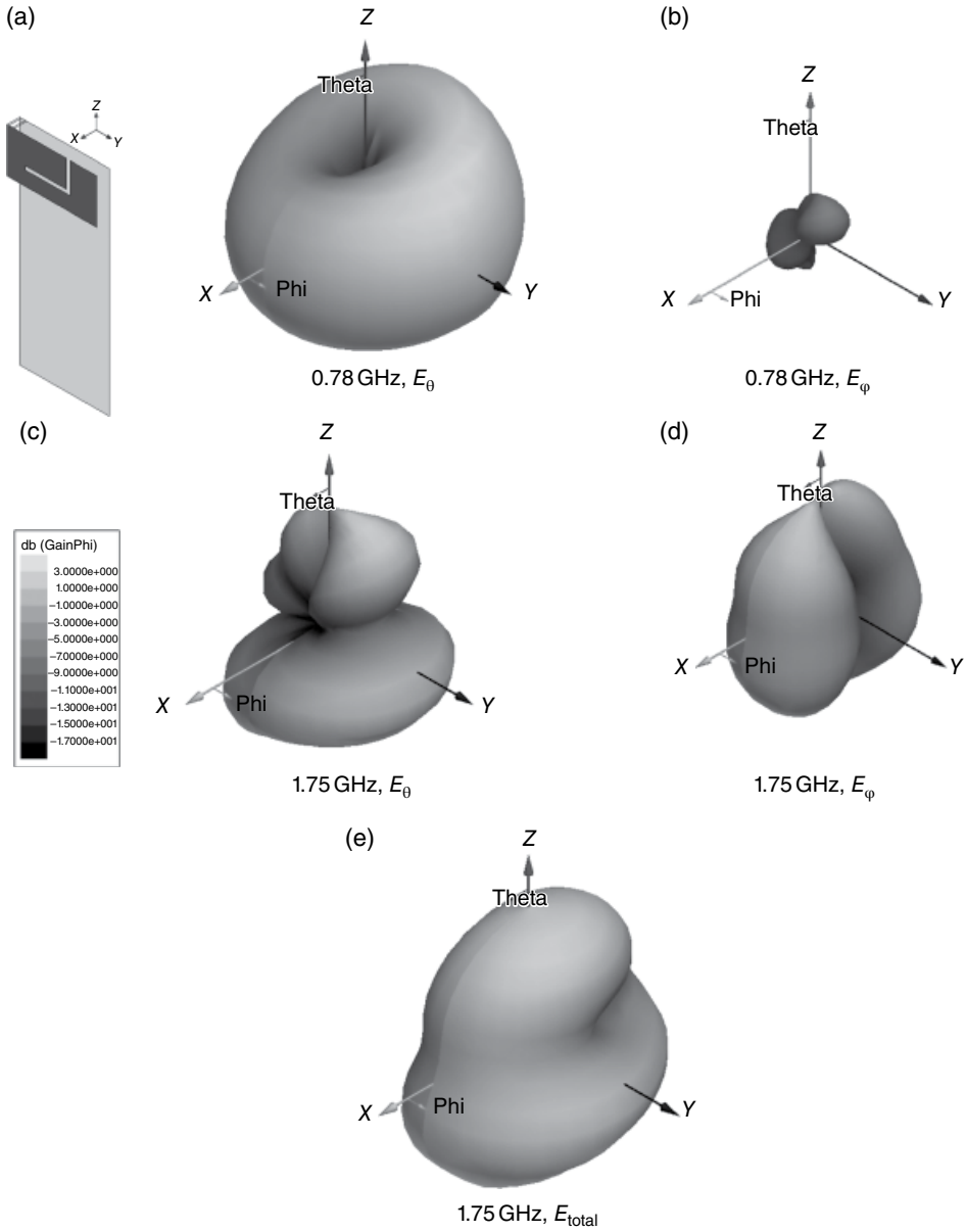
Figure 4.19 Radiation patterns of PIFA, P=15 mm, D=15 mm, C=40 mm.
