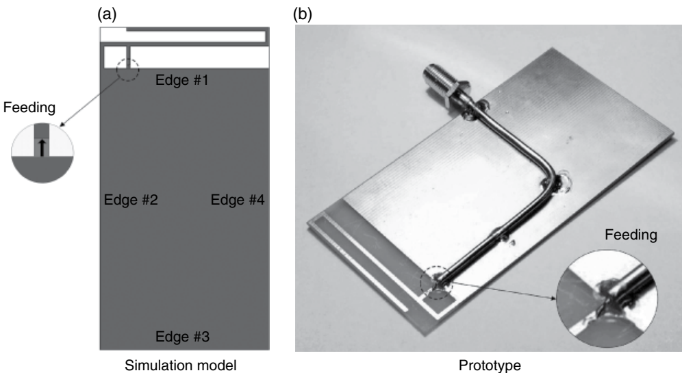
Figure 5.9 Making a prototype.
