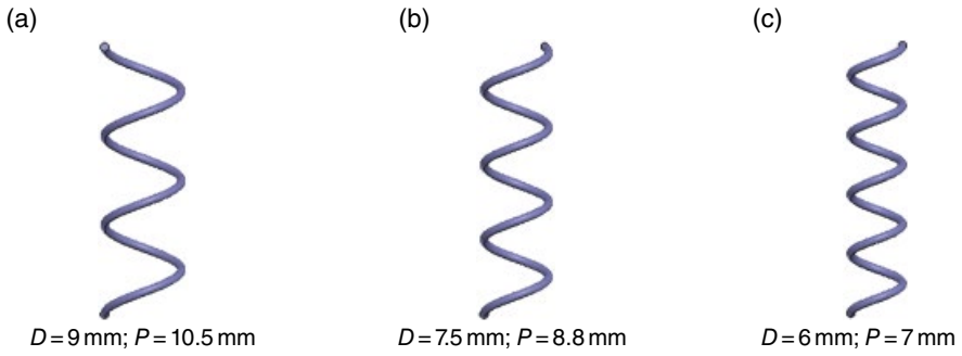
Figure 3.14 Three 90 mm-long helices with the same height of 31.5 mm.
