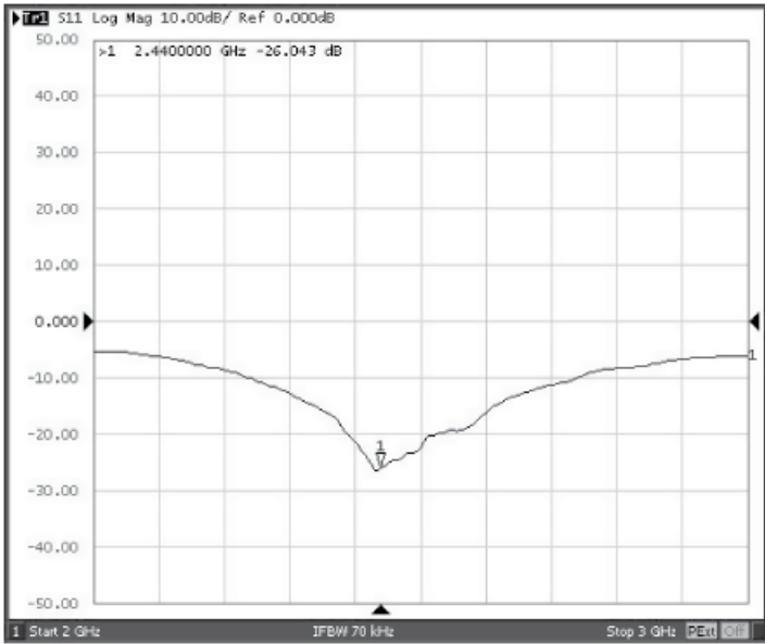
S_{11} of the final design
