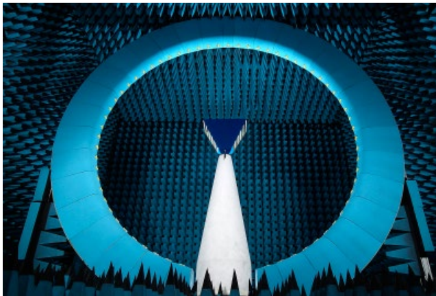
Figure 5.25 Near-field chamber. ( Source: Reproduced with permission of Microwave Vision.)
