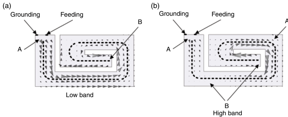
Figure 4.26 Current distributions of a “small” PIFA.
