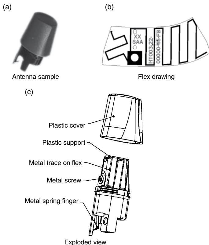
Figure 3.88 Stubby antenna made of flex. (Source: Reproduced with permission of Shanghai Amphenol Airwave.)
