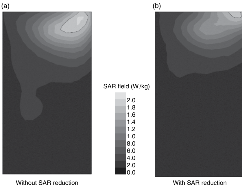
Figure 6.20 SAR distribution of an IFA.
