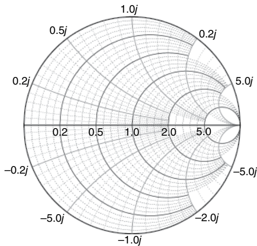
Figure 2.3 The Smith chart.
