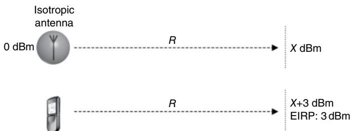
Figure 5.27 Illustration of EIRP.
