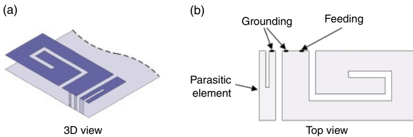
Figure 4.29 PIFA with parasitic element.
