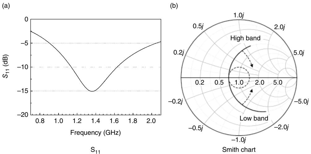
Figure 2.17 Antenna example—bandwidth widened.
