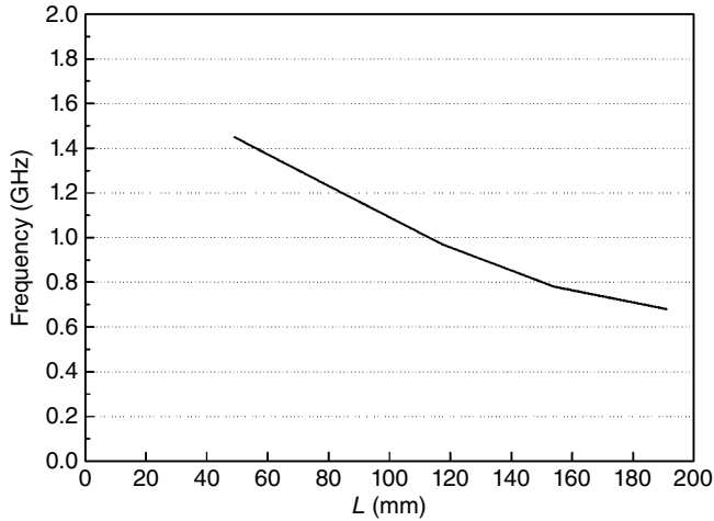
Figure 3.17 Resonant frequency versus length of helix, H=31.5 mm and D=6 mm.
