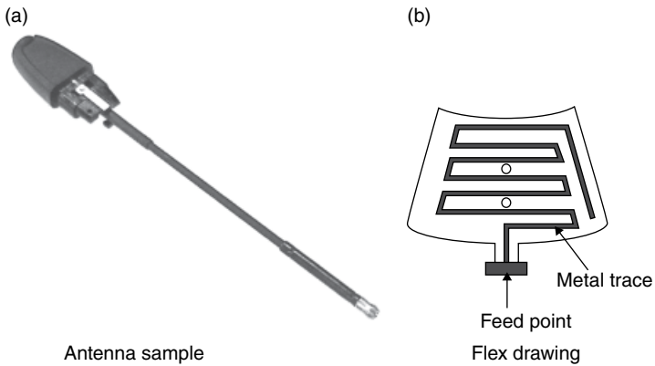
Figure 3.91 Retractable antenna made of flex. (Source: Reproduced with permission of Shanghai Amphenol Airwave.)
