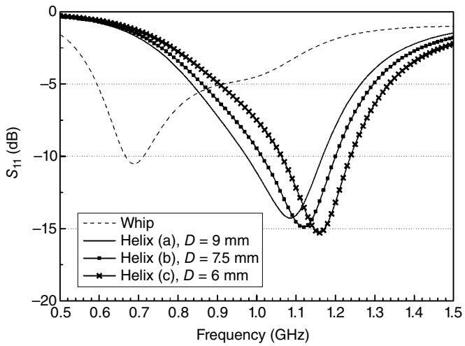
Figure 3.15 Reflection coefficients of a whip monopole and three helices, H=31.5\text{ mm} .
