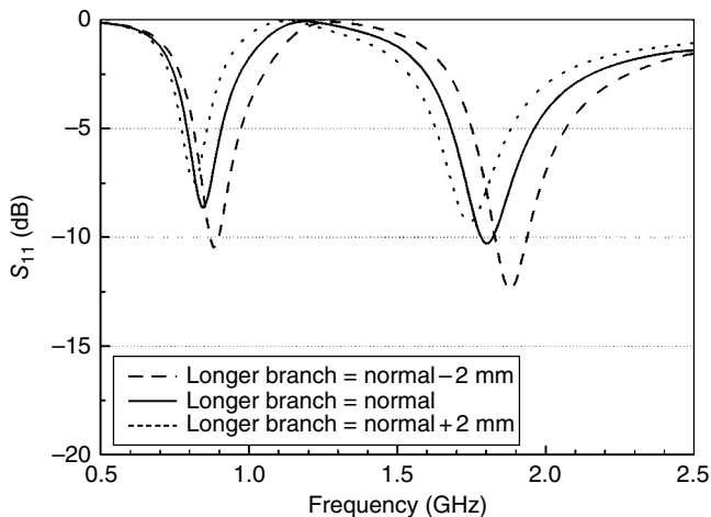
Figure 4.41 Internal folded monopole, variation in the longer branch, D=10 mm.
