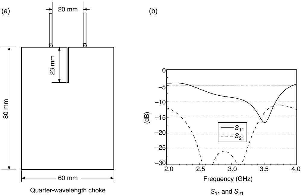
Figure 4.92 Using choke to improve isolation.
