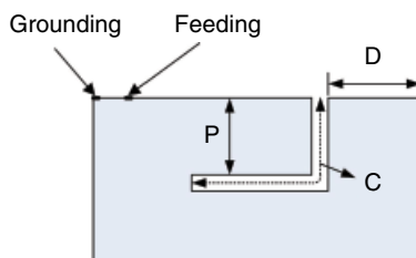
Figure 4.14 Dual-band PIFA.
