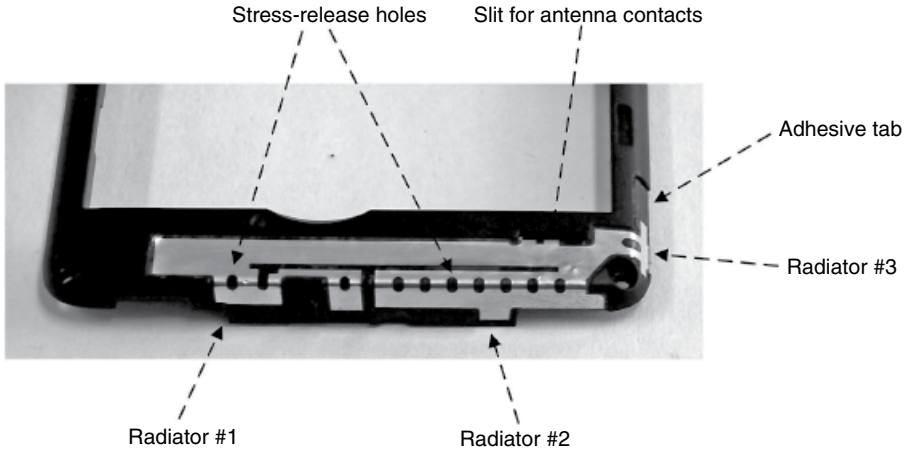
Figure 4.99 Semifinished primary antenna installed on a phone. (Source: Reproduced with permission of Xiaomi, Inc. and Shanghai Amphenol Airwave, Inc.)
