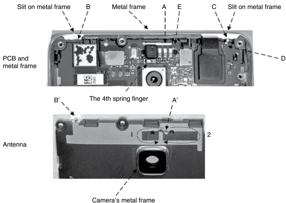
Figure 4.112 Xiaomi 4's secondary antenna. (Source: Reproduced with permission of Xiaomi, Inc.)
