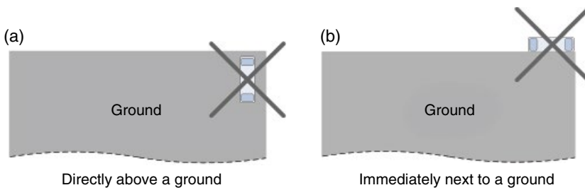
Figure 4.52 Wrong ways of placing monopole-type ceramic antennas.
