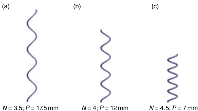
Figure 3.11 Three 90 mm-long helices with the same diameter of 6 mm.
