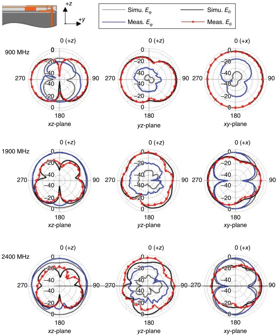
Figure 4.74 Simulated and measured radiation patterns. (Source: Deng et al. [27]. Reproduced with permission of IEEE.)
