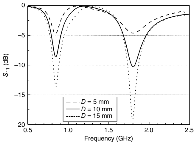
Figure 4.39 Internal folded monopole with various D .
