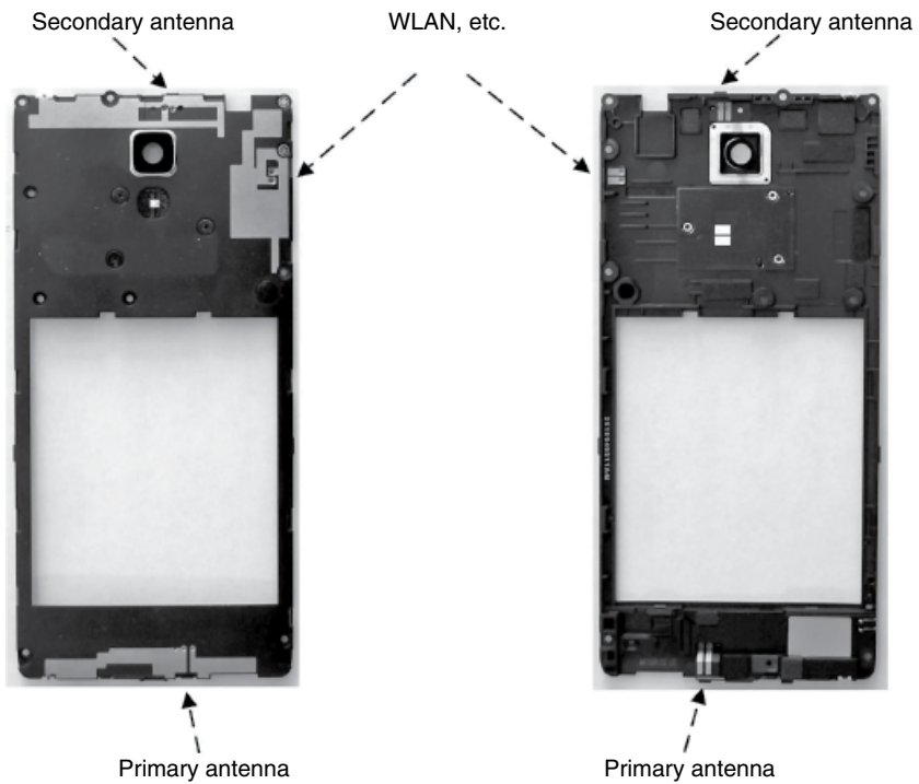
Figure 4.109 Xiaomi 4's antennas. (Source: Reproduced with permission of Xiaomi, Inc.)
