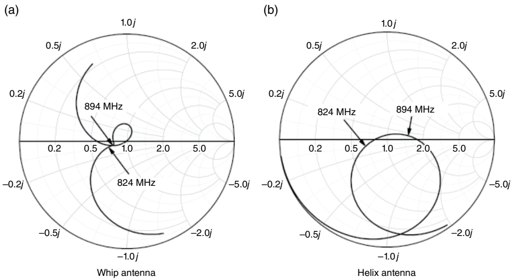
Figure 3.23 Impedances of whip and helix antennas after matching.
