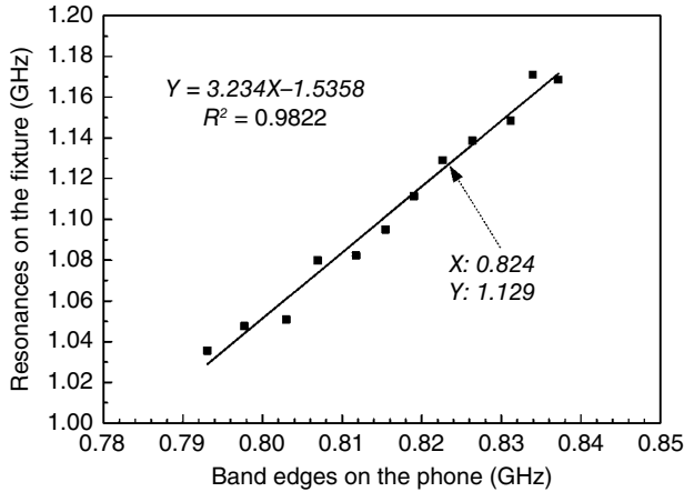
Figure 5.40 Correlation data of a real phone.
