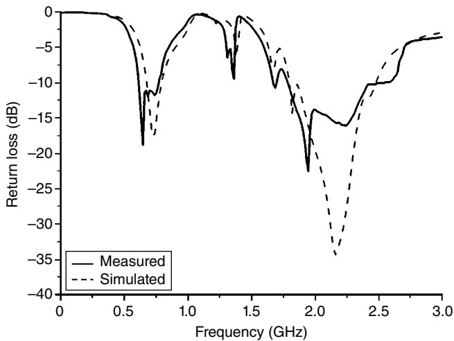
Figure 3.87 Reflection coefficients. (Source: Kim et al. [27]. Reproduced with permission of IET.)
