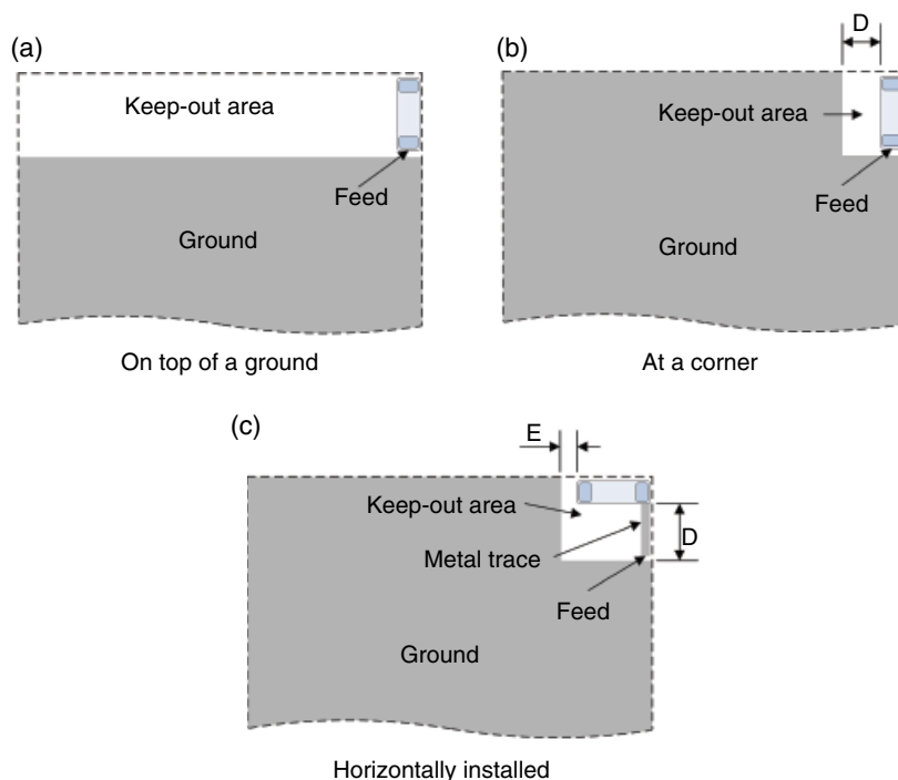
Figure 4.53 Correct ways of placing monopole-type ceramic antennas.
