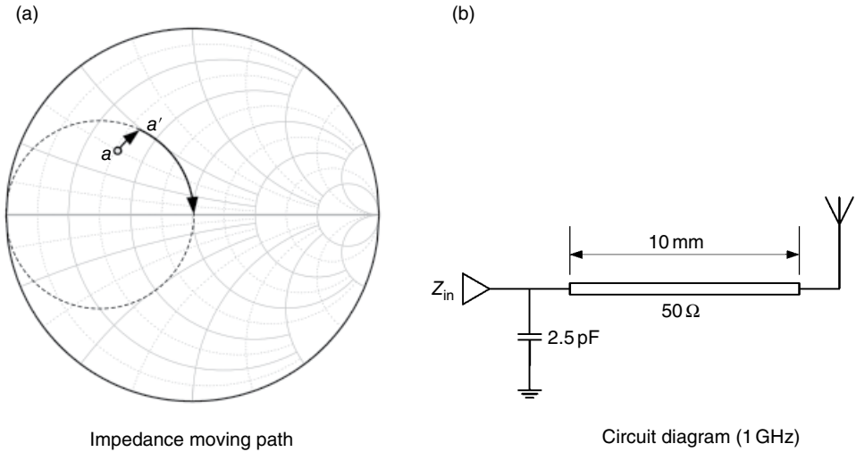
Figure 2.15 Matching with both transmission line and lumped element.
