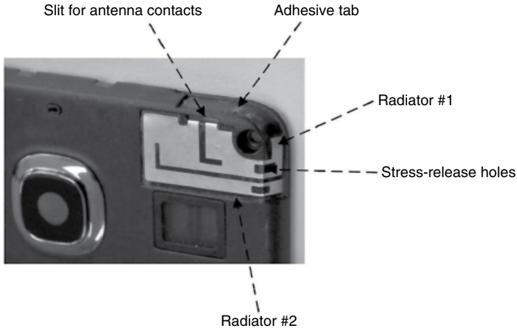
Figure 4.105 Semifinished WLAN and GPS antenna installed on a phone. (Source: Reproduced with permission of Xiaomi, Inc. and Shanghai Amphenol Airwave, Inc.)
