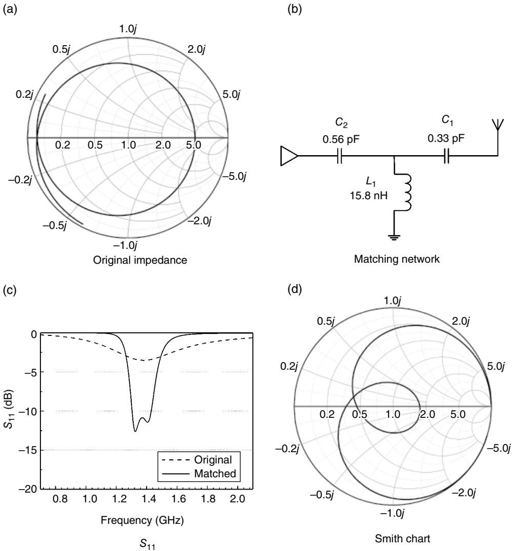
Figure 2.24 T-shaped matching circuit.
