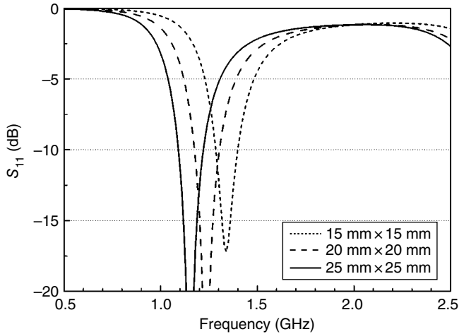
Figure 3.97 Effect of small ground, L_{\text{ant}}=70 mm.
