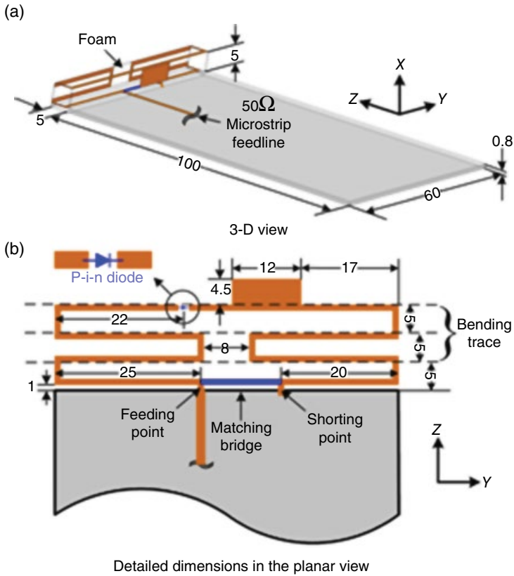
Figure 4.76 Geometry and dimensions of the proposed antenna. (Source: Li et al. [31]. Reproduced with permission of IEEE.)
