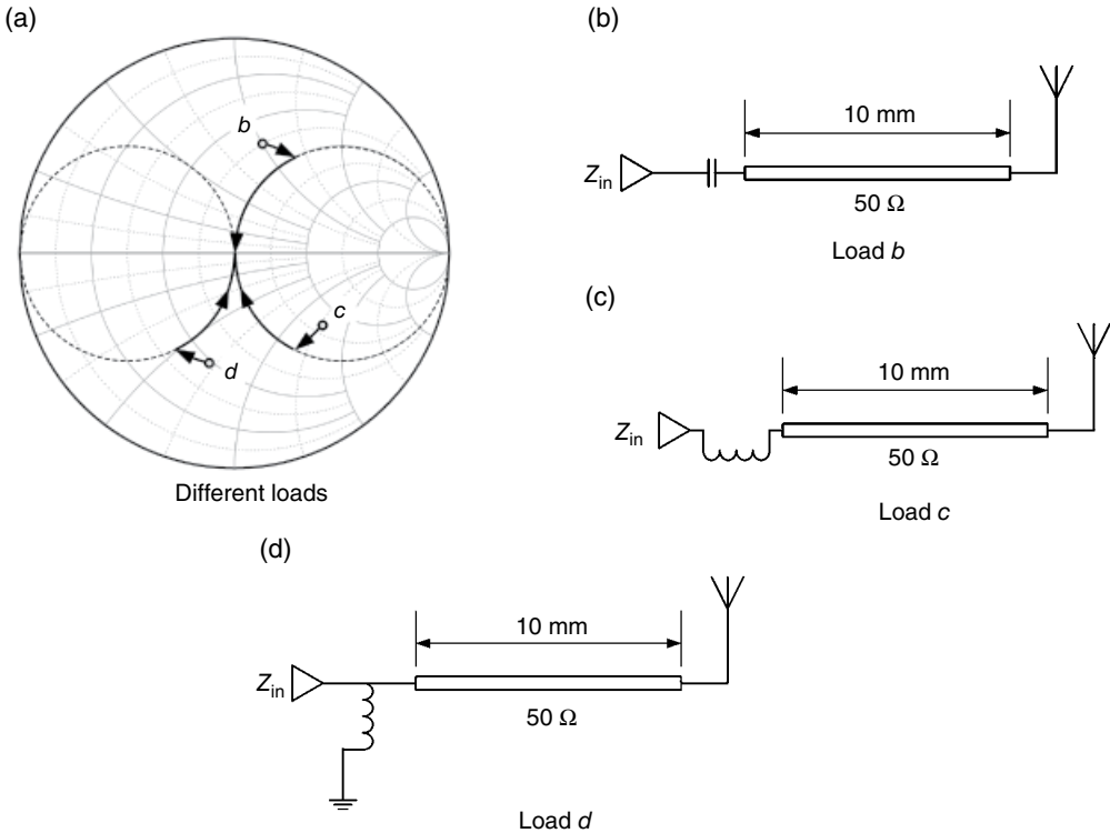
Figure 2.16 Matching circuits of load impedance b , c , and d (1 GHz).
