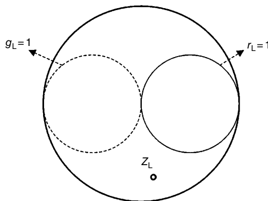
Figure 2.8 Two circles which can be matched by single components.
