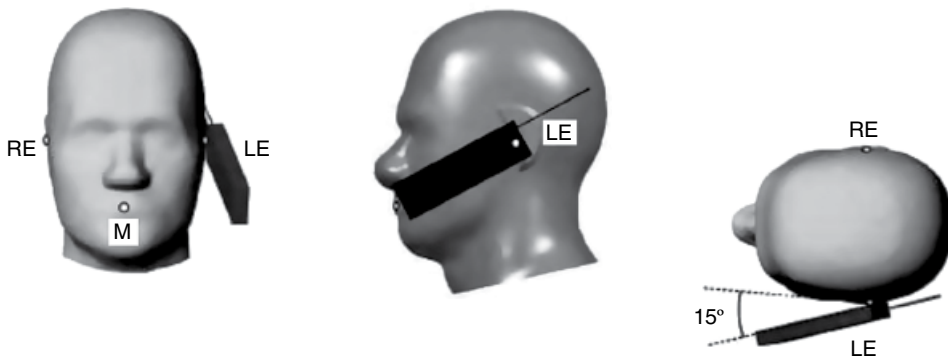
Figure 6.10 Front, side, and top views of left ear, 15° tilt position. (Source: Reproduced with permission of IEEE.)
