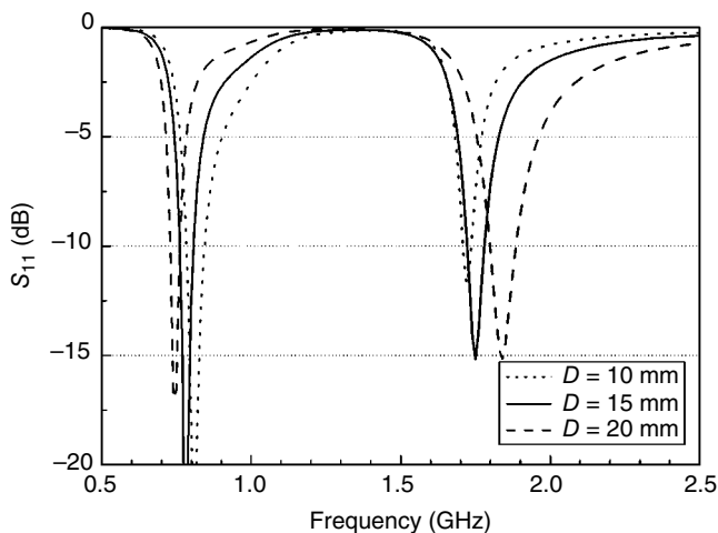
Figure 4.16 Impact of dimension D . 50\text{ mm} \times 25\text{ mm} Patch, P=15\text{ mm} , C=40\text{ mm} .
