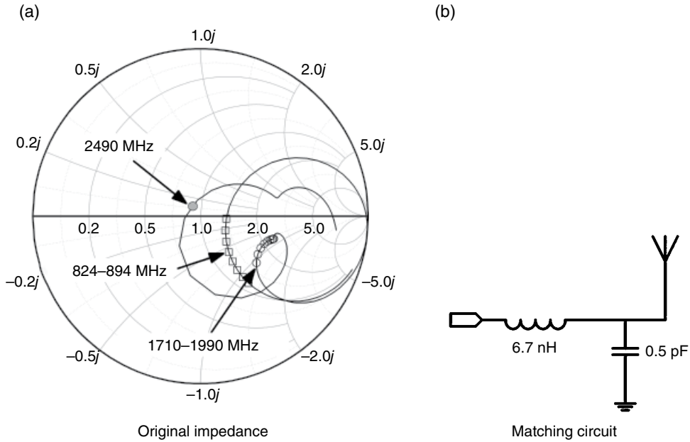
Figure 3.31 Matching a dual-branch stubby antenna.
