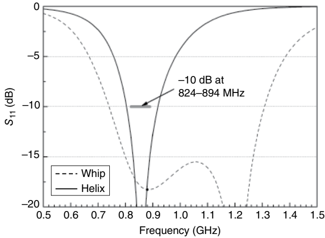
Figure 3.22 Reflection coefficients of whip and helix antennas after matching.
