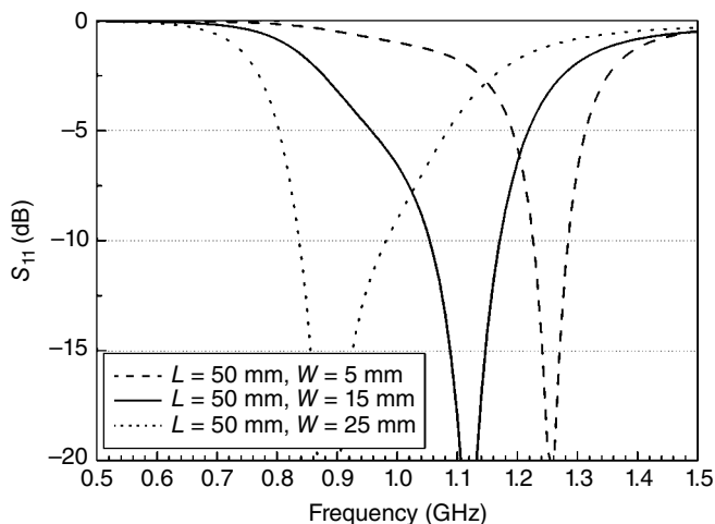
Figure 4.11 Three PIFAs with different widths H=7 mm.
