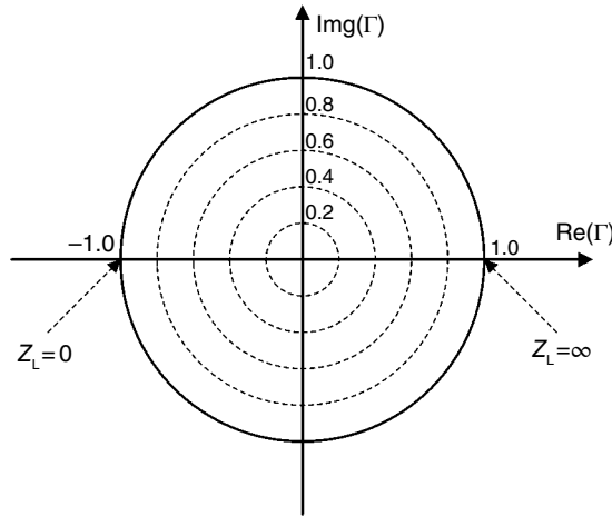
Figure 2.1 Complex plan of \Gamma .
