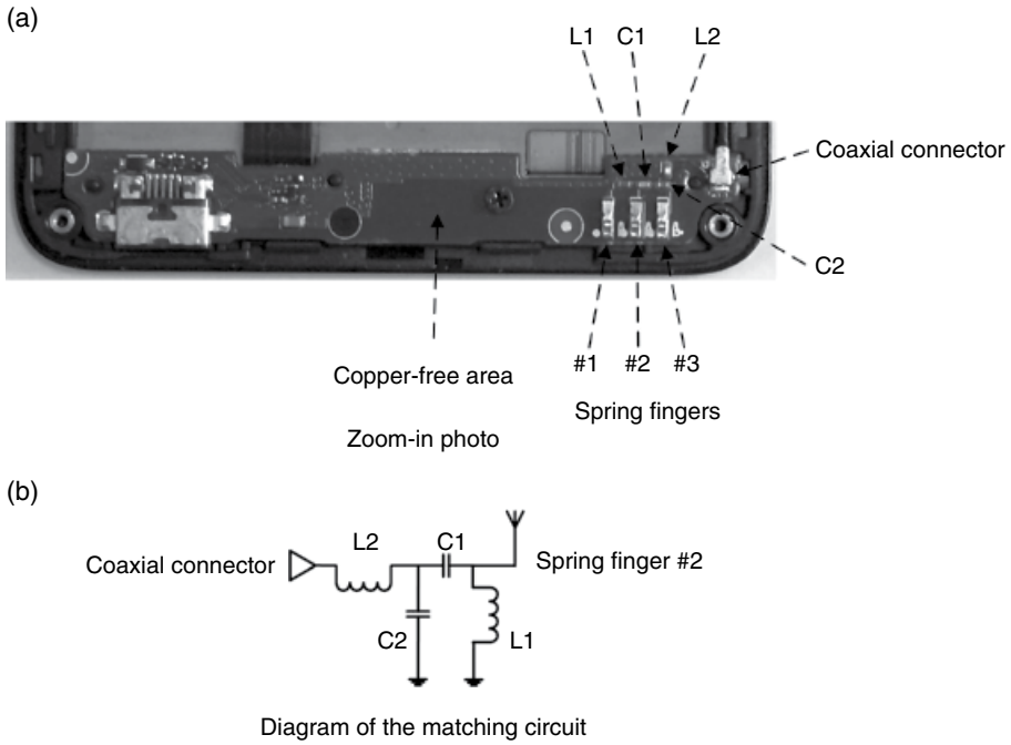
Figure 4.100 Matching circuit of the primary antenna. (Source: Reproduced with permission of Xiaomi, Inc.)
