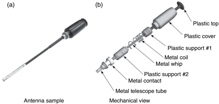
Figure 3.82 Retractable antenna. (Source: Reproduced with permission of Shanghai Amphenol Airwave.)
