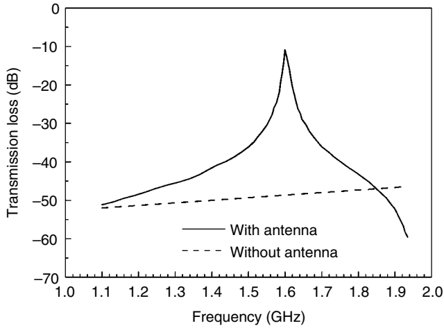
Figure 5.36 Measured result of a S_{21} setup, constructive coupling.
