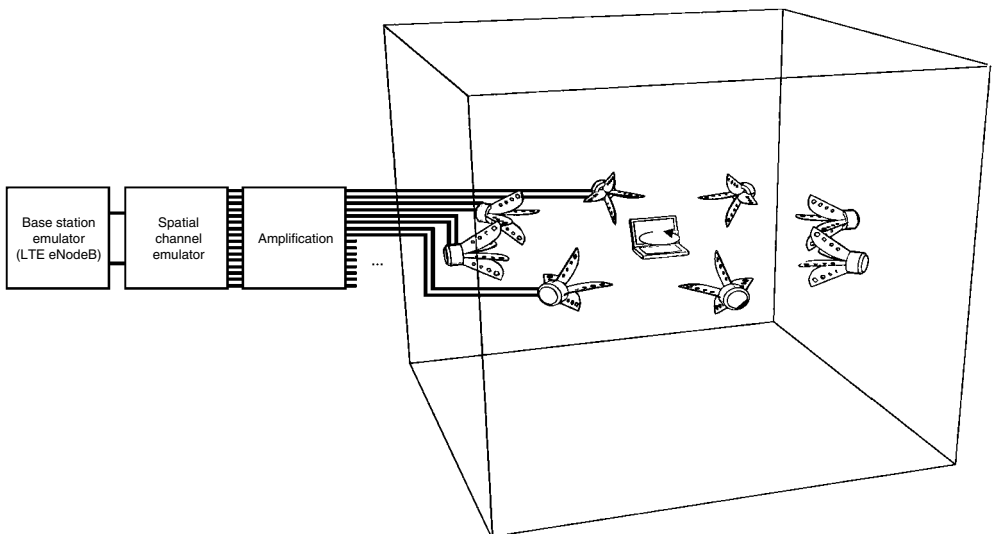
Figure 5.45 Block diagram of a typical boundary array RF environment simulation system [23]. (Source: CTIA.)
