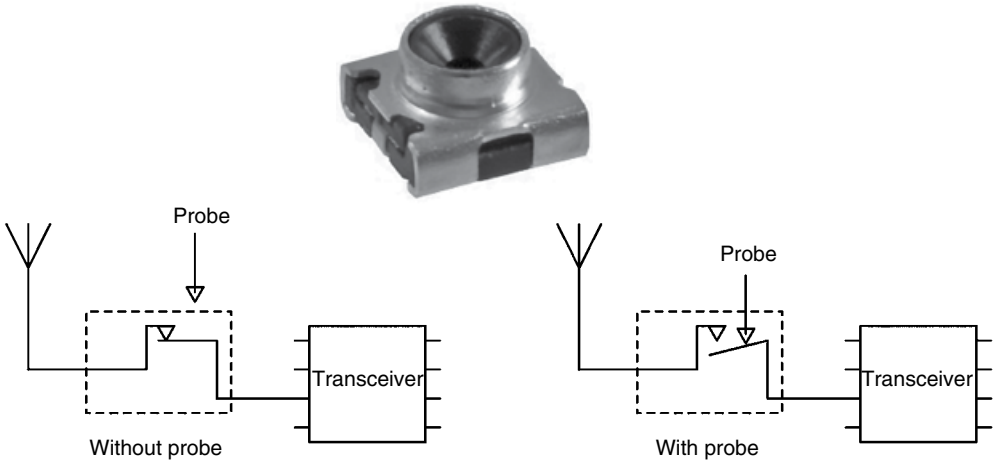
Figure 5.11 Switch connector. (Source: Murata Manufacturing Co. Ltd.)
