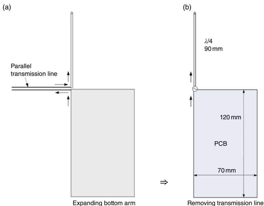
Figure 3.8 Transformation to a monopole antenna.
