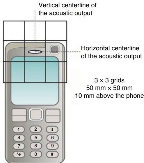
Figure 6.24 HAC measurement plane.
