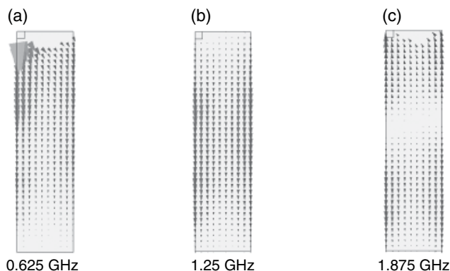
Figure 3.94 Ground's current of different modes, W=30 mm.
