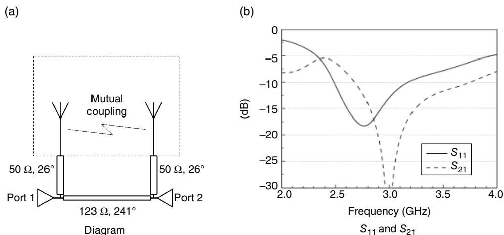
Figure 4.93 Using neutral line to improve isolation.
