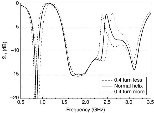
Figure 3.33 Tuning the lower resonance by adjusting the helix.
