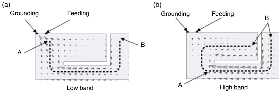
Figure 4.25 Current distributions of a “normal” PIFA.
