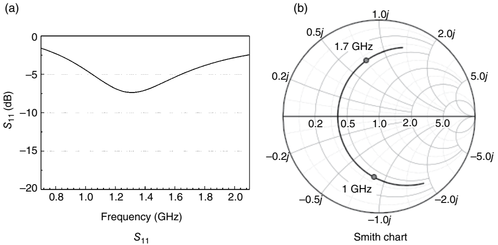
Figure 2.29 Dual-band matching Example 2.3.
