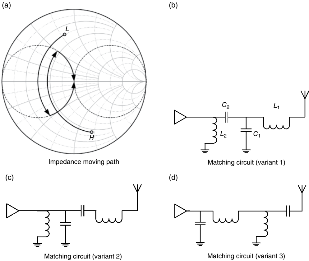
Figure 2.28 Dual-band matching Example 2.2.
