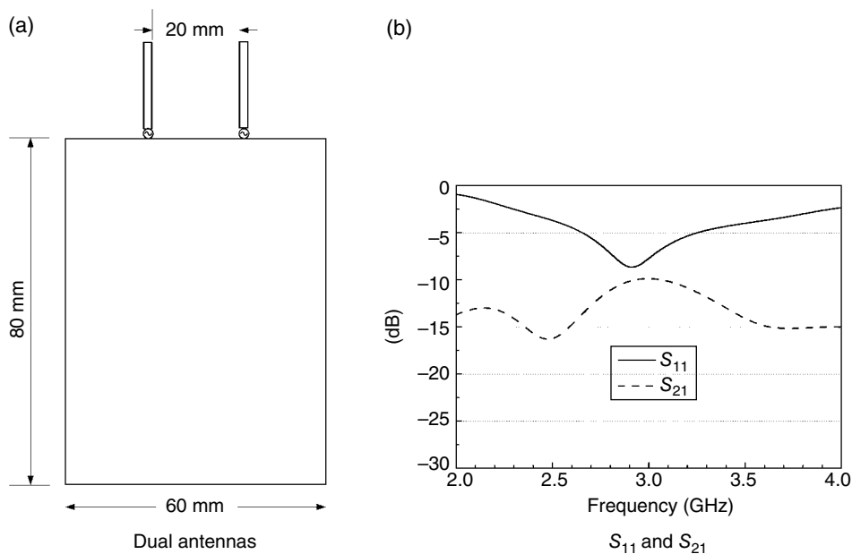
Figure 4.91 Two closely placed monopole antennas.
