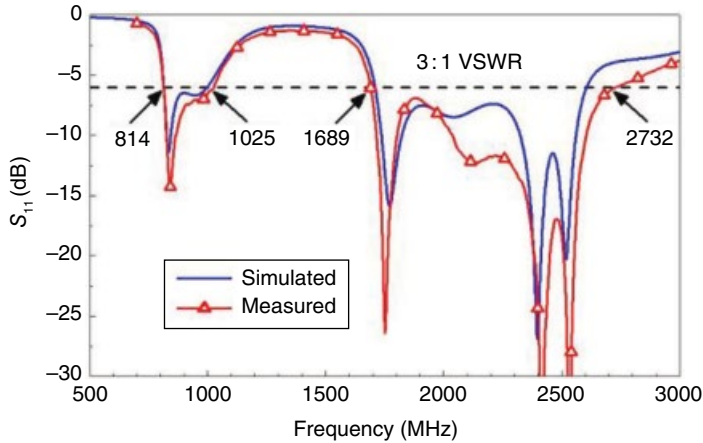
Figure 4.73 Simulated and measured S_{11} of the antenna. (Source: Deng et al. [27]. Reproduced with permission of IEEE.)
