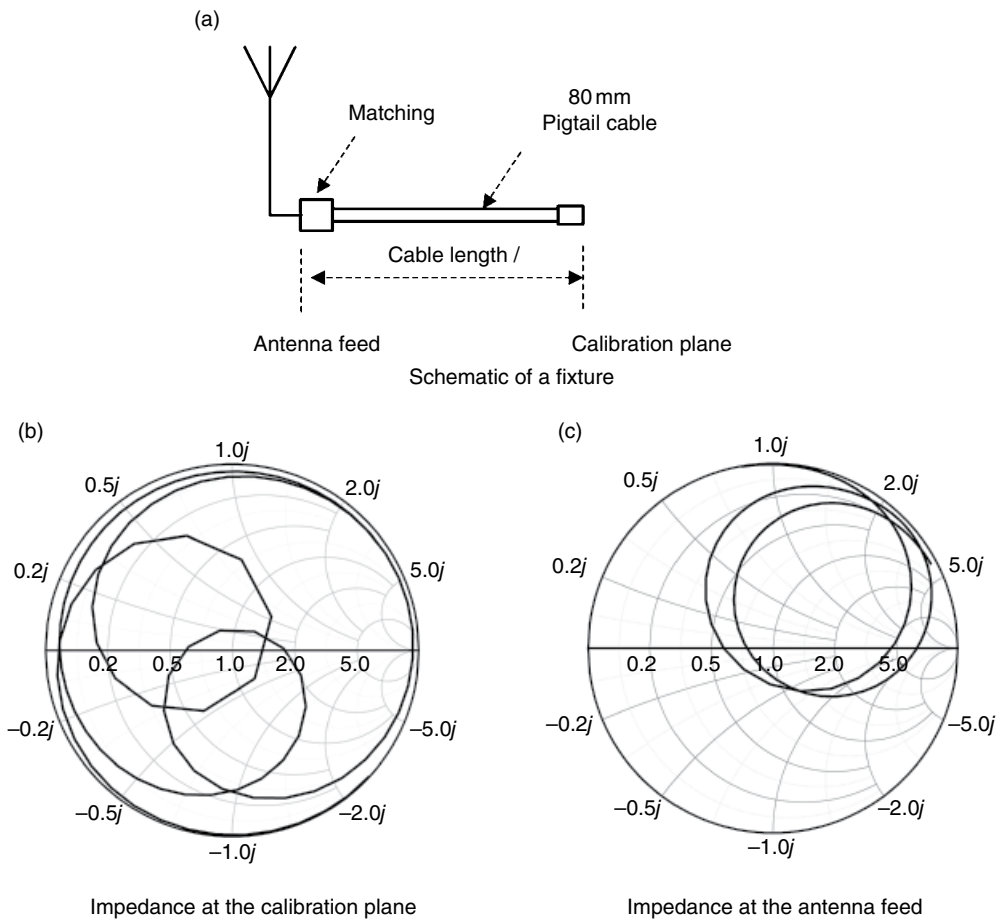
Figure 5.17 Impedance of a test fixture.
