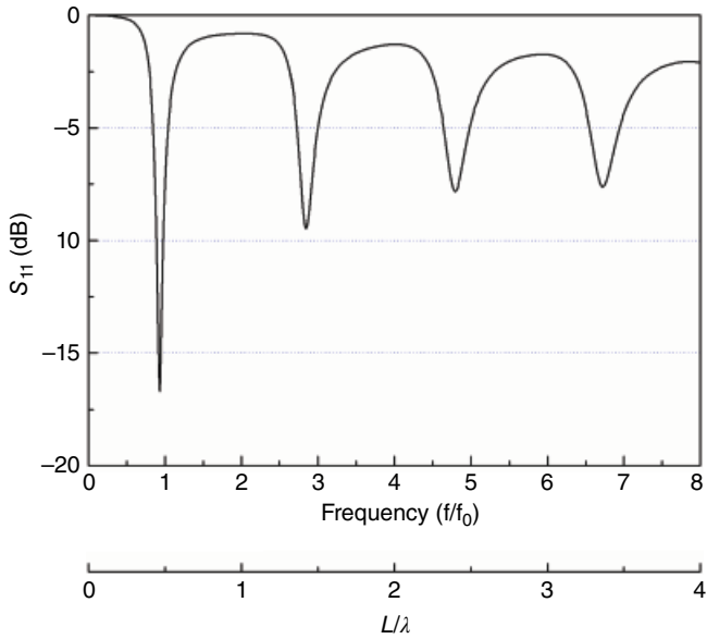
Figure 3.6 Reflection coefficient of a dipole antenna.
