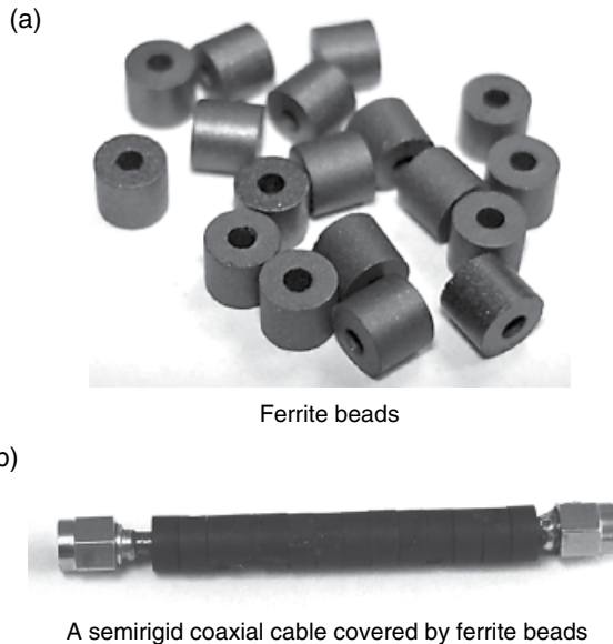
Figure 5.13 Ferrite bead choke.
