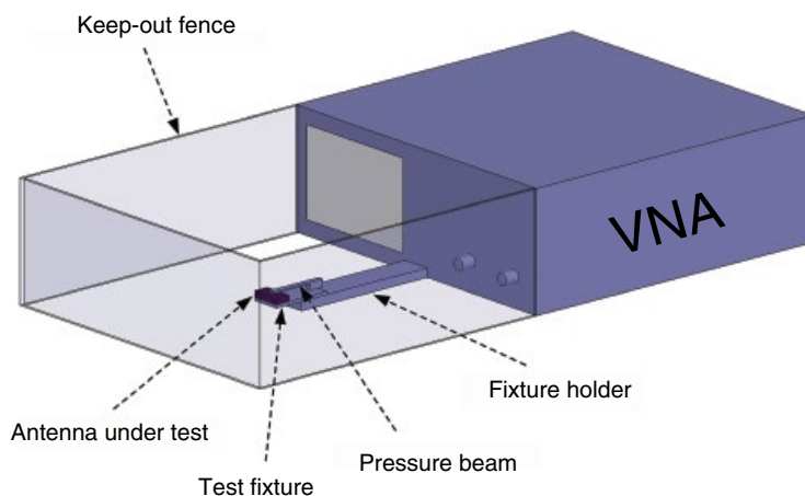
Figure 5.34 Simplified illustration of production test setup ( S_{11} type).
