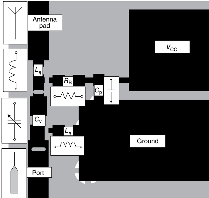
Figure 2.35 Layout of matching circuit. (Source: Li et al. [16]. Reproduced with permission of John Wiley & Sons, Inc.)
