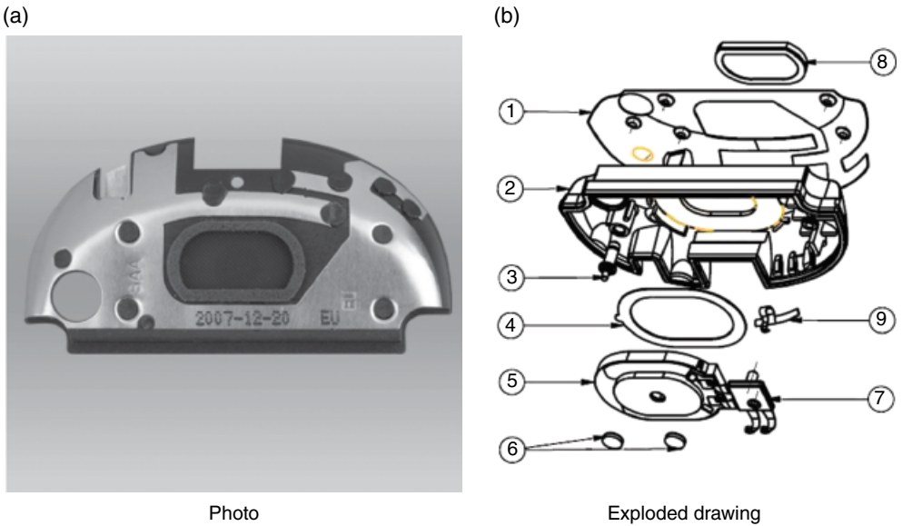
Figure 4.33 Three-dimensional metal stamping integrated antenna. (Source: Reproduced with permission of Shanghai Amphenol Airwave.)
