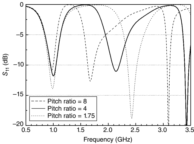
Figure 3.41 Simulation reflection coefficients.
