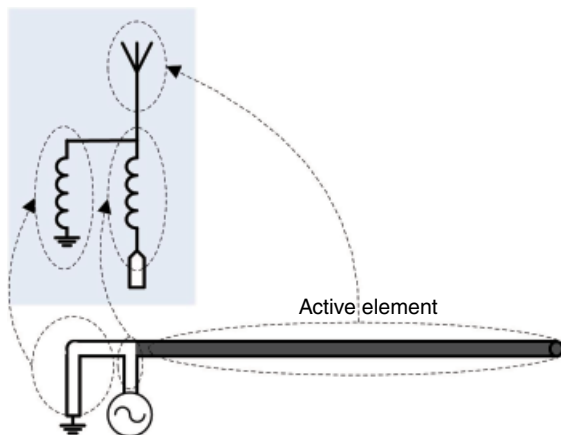
Figure 4.7 Simplified equivalent circuit of an IFA.
