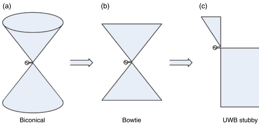
Figure 3.60 Transformation from a biconical antenna to a UWB stubby antenna.
