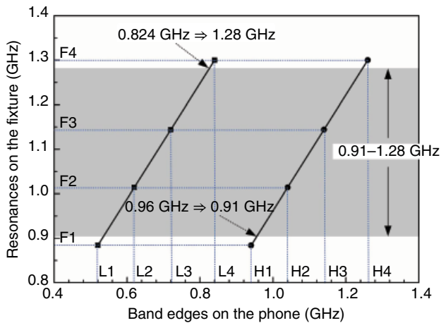
Figure 5.39 Correlations between a phone and a fixture.
