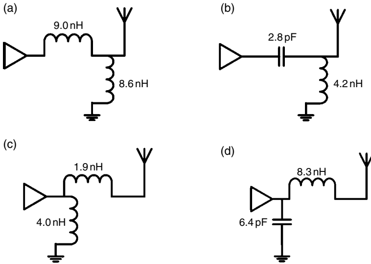
Figure 2.10 Component values of the four circuits used in Figure 2.9.
