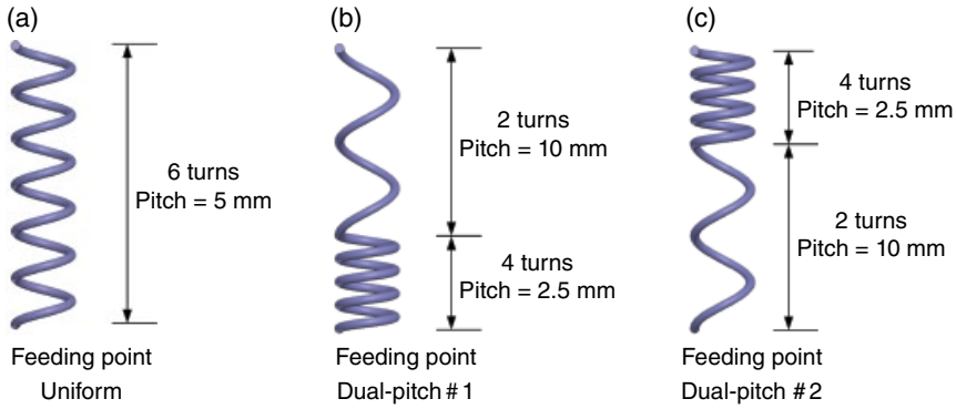
Figure 3.38 Three variants of six-turn helices.
