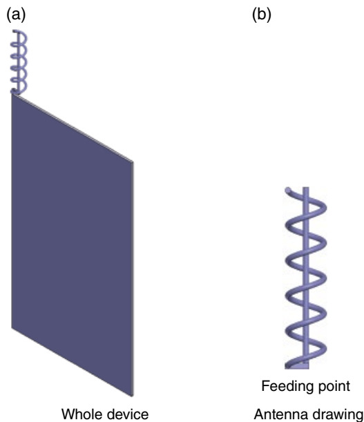
Figure 3.26 Two-branch multiband stubby antennas.
