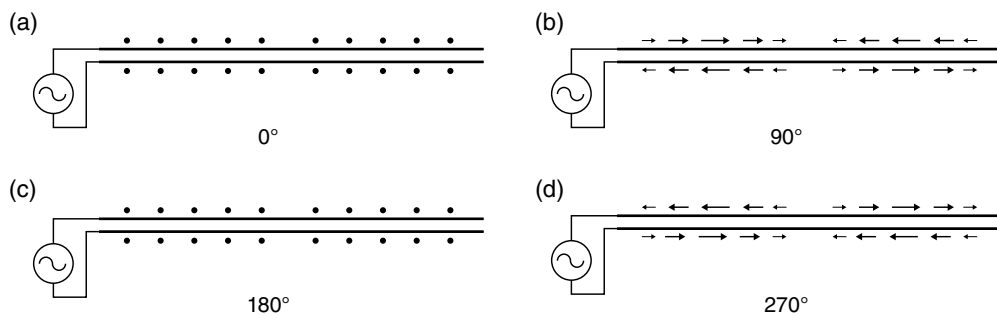
Figure 3.4 Transient current distribution of standing wave on an open-circuit transmission line.
