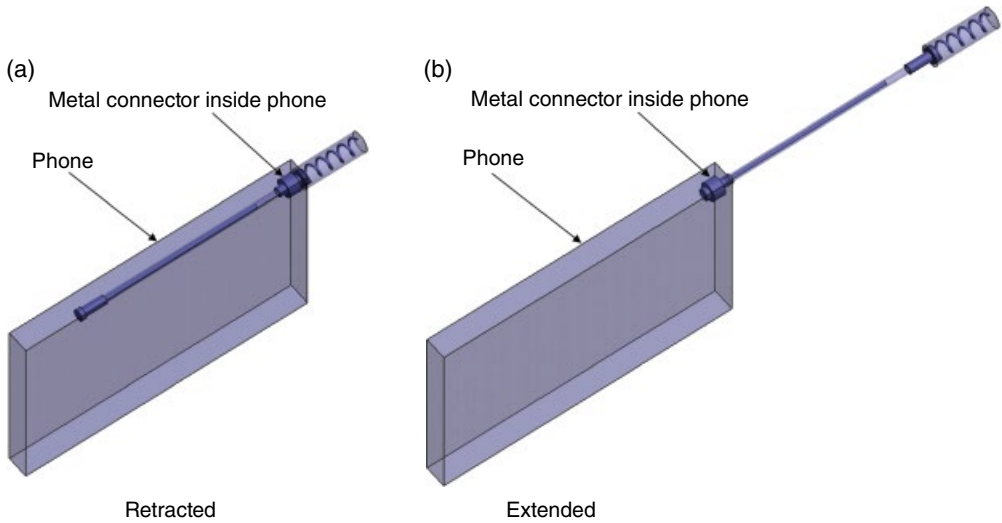
Figure 3.74 A decoupled whip-stubby antenna on a phone.
