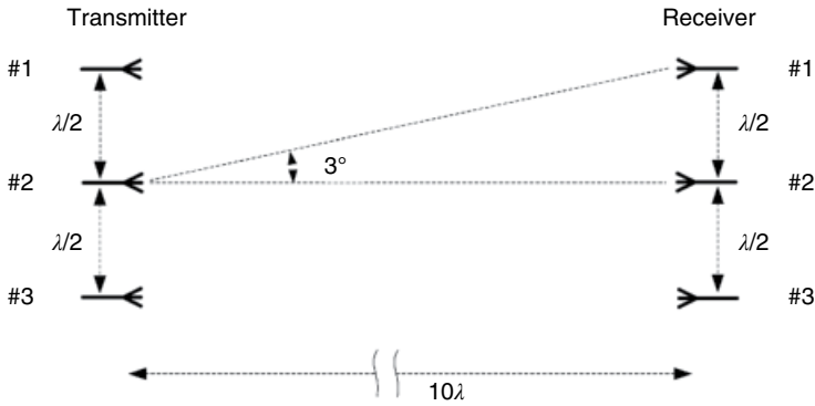
Figure 4.84 A 3x3 MIMO antenna system in free space.
