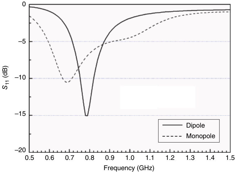
Figure 3.9 Reflection coefficients of a 180-mm-long dipole and a 90-mm-long monopole.
