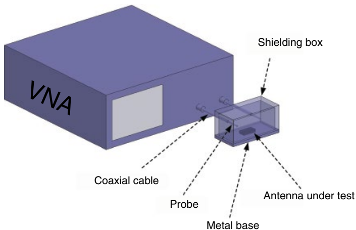
Figure 5.35 Simplified illustration of production test setup ( S_{21} type).
