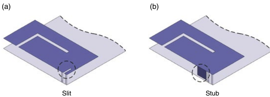
Figure 4.22 Other ways of matching.
