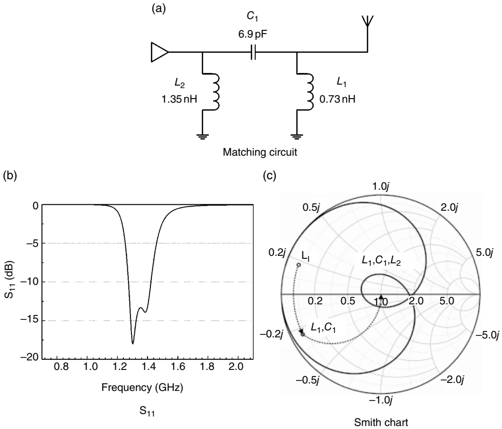
Figure 2.23 Another version of the \pi -shaped matching circuit.
