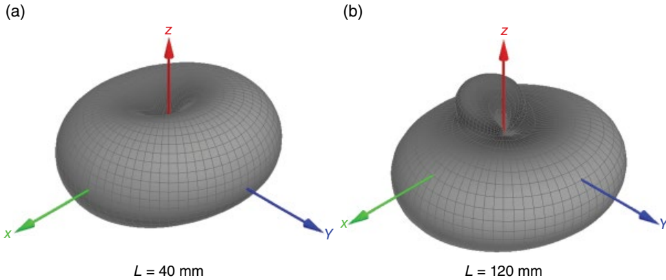
Figure 3.95 Three-dimensional radiation patterns. L_{\text{ant}}=70 mm, W=30 mm at 1.2 GHz.
