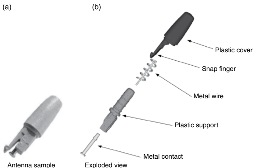
Figure 3.52 Single-branch stubby antenna. (Source: Reproduced with permission of Shanghai Amphenol Airwave.)
