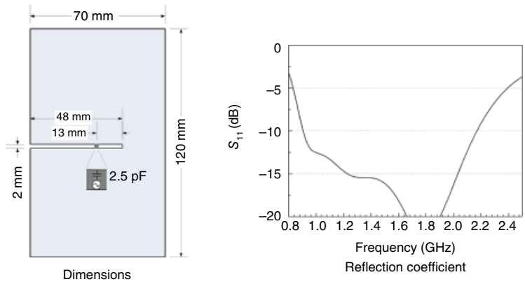
Figure 4.65 A wideband antenna which is excited by a slot.
