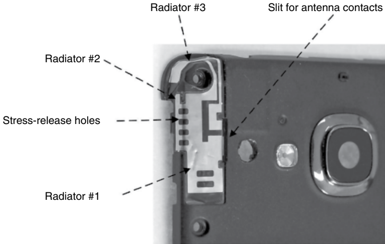
Figure 4.102 Semifinished secondary antenna installed on a phone. (Source: Reproduced with permission of Xiaomi, Inc. and Shanghai Amphenol Airwave, Inc.)
