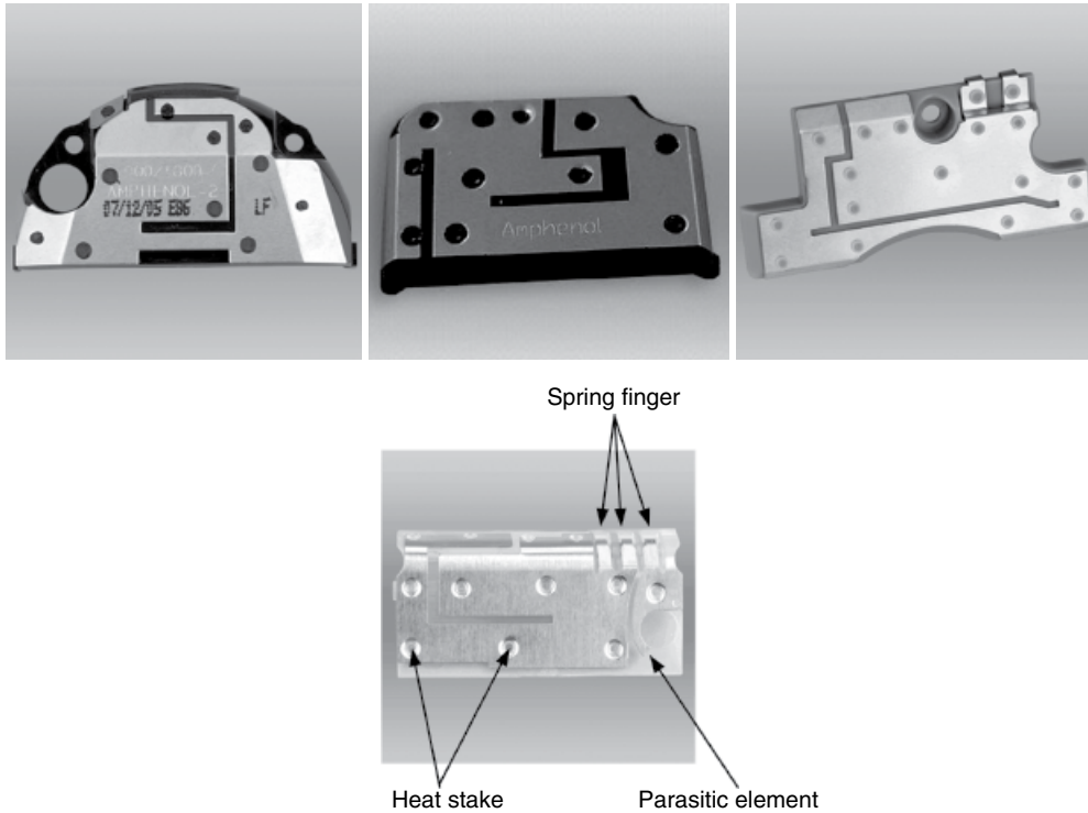
Figure 4.31 Metal stamping technology. (Source: Reproduced with permission of Shanghai Amphenol Airwave.)
