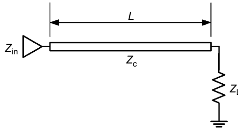
Figure 2.13 Load impedance connected by a segment of transmission line.
