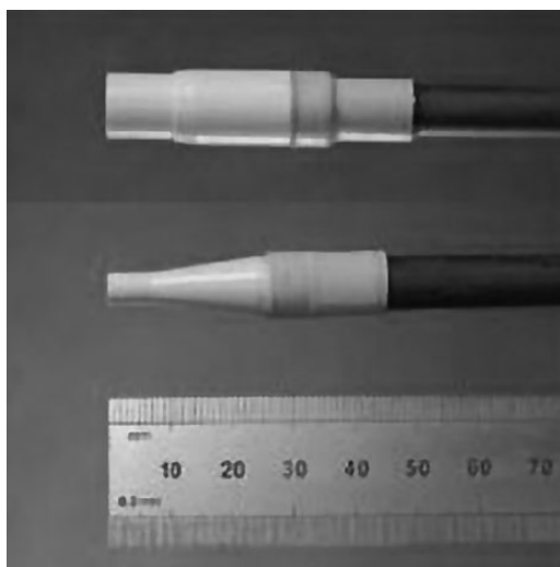
Figure 6.23 H -field and E -field probes. (Source: IndexSAR Ltd.)
