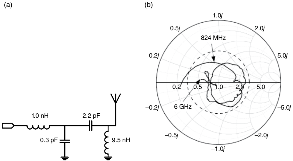
Figure 3.68 Matched UWB stubby. (a) Matching circuit. (b) Measured impedance.
