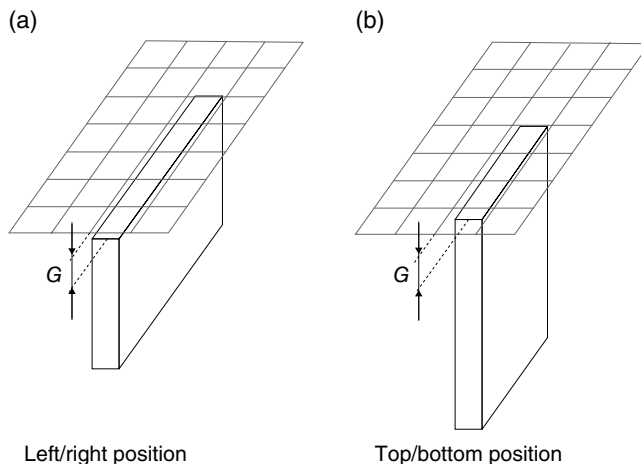
Figure 6.21 SAR distribution of an IFA.
