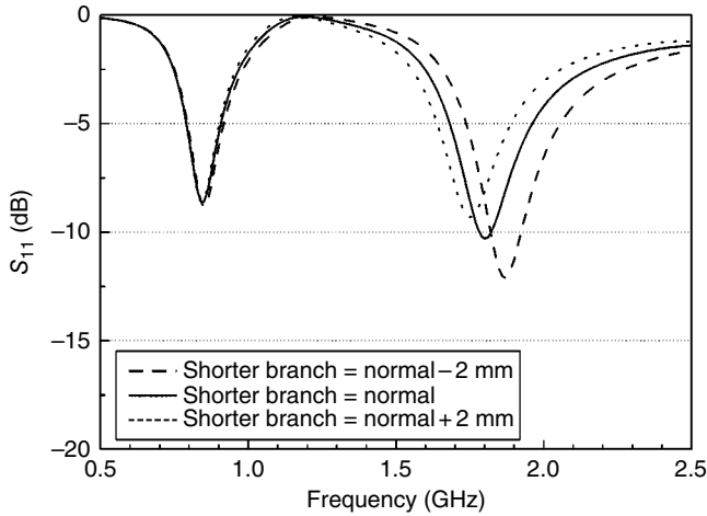
Figure 4.40 Internal folded monopole, variation in the shorter branch, D=10 mm.
