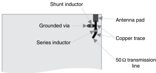
Figure 2.11 Layout of Figure 2.10a on a printed circuit board.
