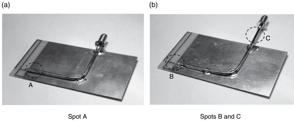
Figure 5.10 A fixture with improper details.
