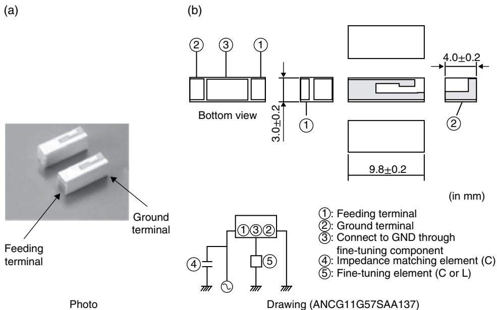
Figure 4.55 IFA ceramic GPS antenna. (Source: Murata Manufacturing Co. Ltd.)
