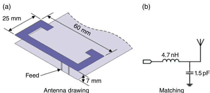
Figure 4.27 A large PIFA.
