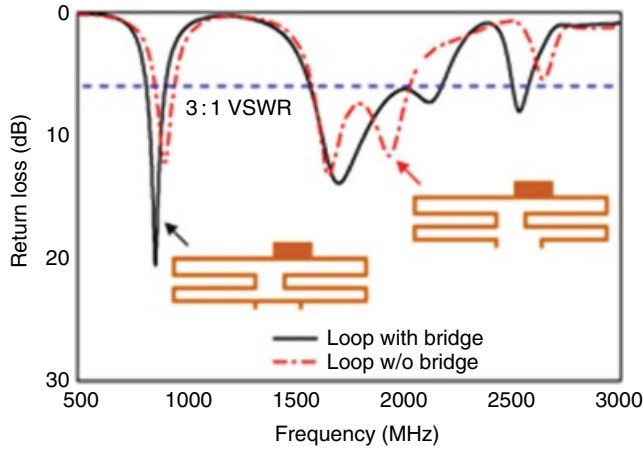
Figure 4.78 Simulated return loss of loop mode of the proposed antenna with or without the matching bridge. (Source: Li et al. [31]. Reproduced with permission of IEEE.)
