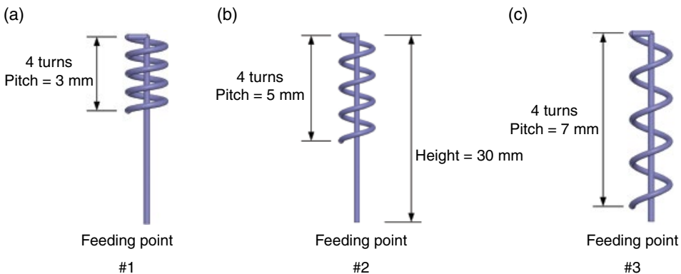
Figure 3.48 Three variants of helix-loaded whips.
