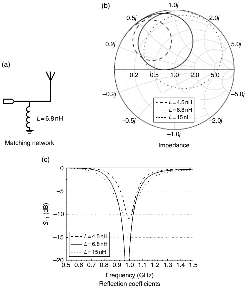
Figure 4.4 Using a shunt inductor to match the antenna with G = 6 \text{ mm} .
