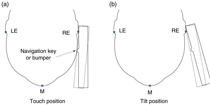
Figure 6.14 Extruded navigation key or bumper.
