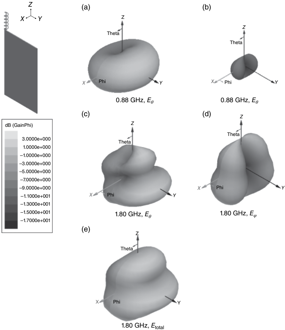
Figure 3.28 Radiation patterns of a two-branch stubby antenna.
