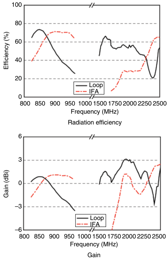
Figure 4.82 Measured results of loop and IFA modes of the proposed antenna. (Source: Li et al. [31]. Reproduced with permission of IEEE.)
