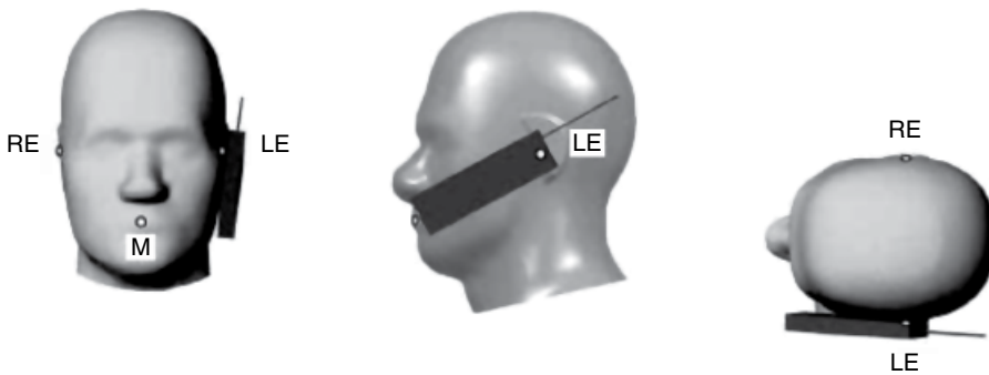
Figure 6.9 Front, side, and top views of left ear, check/touch position (IEEE [3]). M, mouth; RE, right ear; LE, left ear. (Source: Reproduced with permission of IEEE.)
