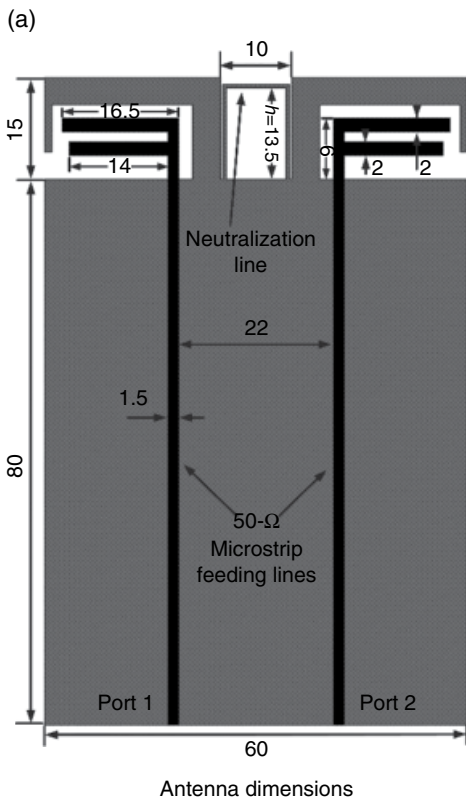
Figure 4.94 A wideband dual antenna. (Source: Wang and Du [42]. Reproduced with permission of IEEE.)
