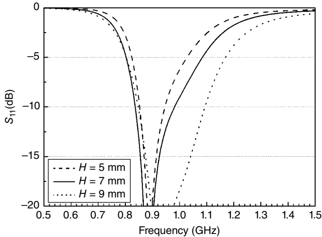
Figure 4.13 PIFA's bandwidth vs. height. L=50\text{ mm}, W=25\text{ mm} .
