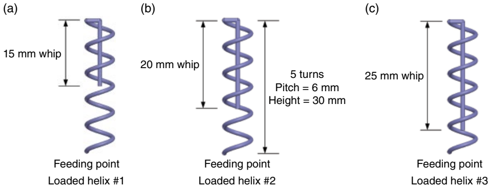
Figure 3.53 Three variants of whip-loaded helices.
