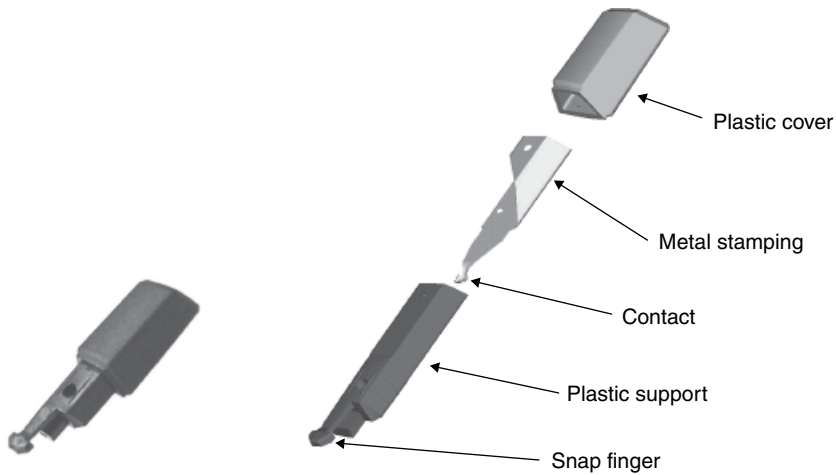
Figure 3.72 Production UWB stubby antenna. (Source: Reproduced with permission of Shanghai Amphenol Airwave.)
