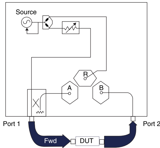
Figure 5.2 Schematic of a simplified VNA. (Source: Reproduced with permission of Agilent Technologies.)
