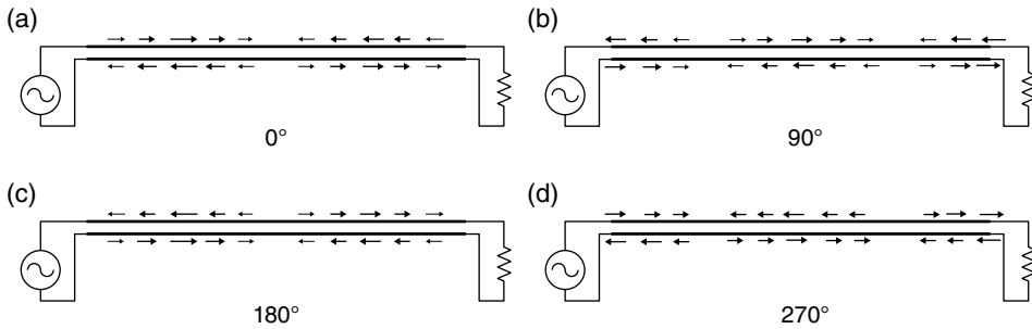
Figure 3.3 Transient current distribution of a traveling wave on a terminated transmission line.
