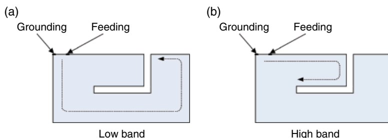
Figure 4.15 Decisive paths of different bands.
