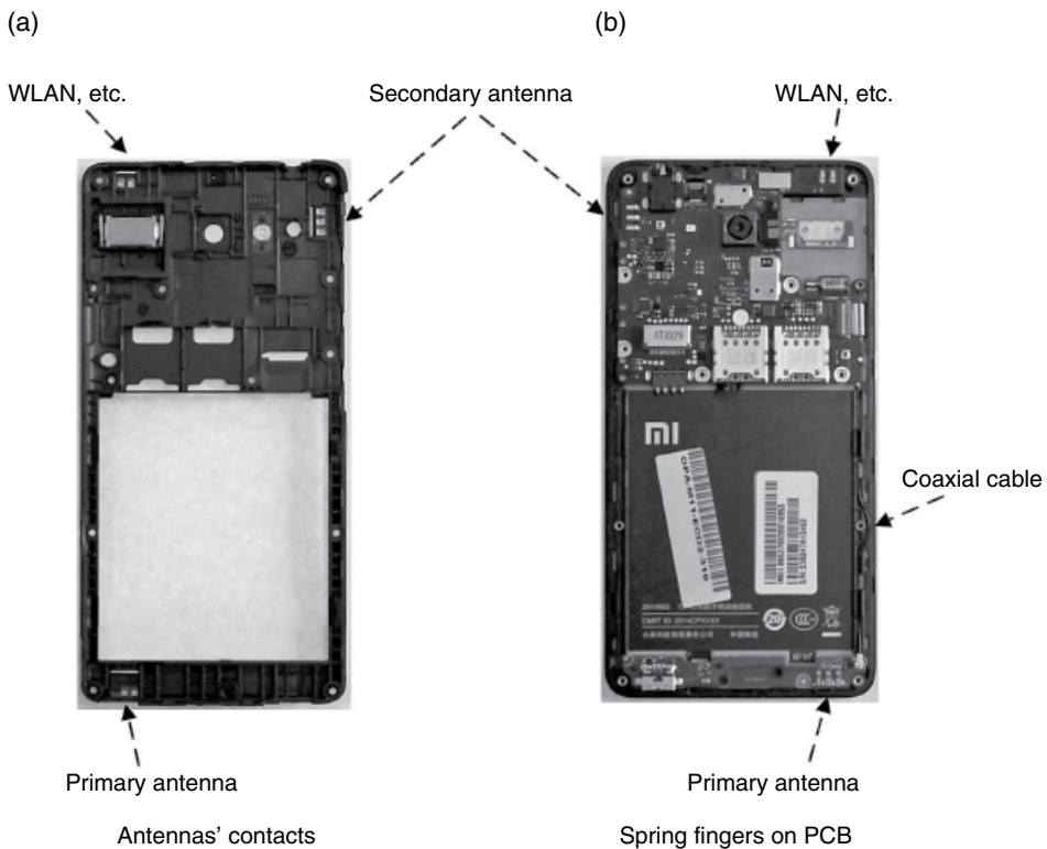
Figure 4.97 Antennas' contacts on the back and spring fingers on PCB. (Source: Reproduced with permission of Xiaomi, Inc.)
