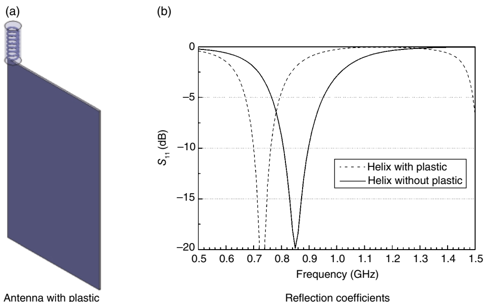
Figure 3.25 Comparison between antennas with and without plastic.
