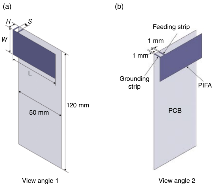
Figure 4.10 Planar inverted-F antenna (PIFA).
