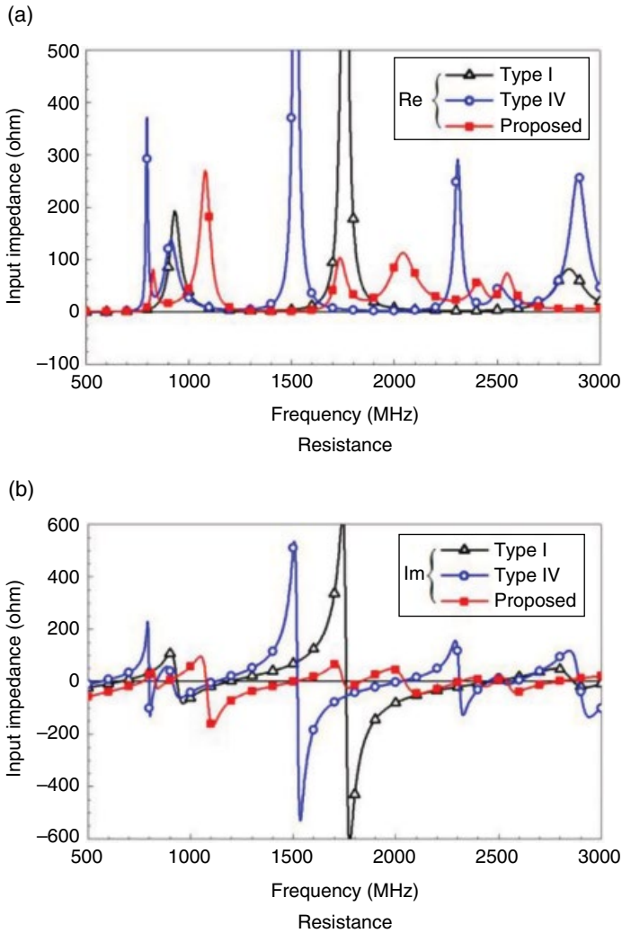
Figure 4.70 Simulated input impedance of the antenna. (Source: Deng et al. [27]. Reproduced with permission of IEEE.)
