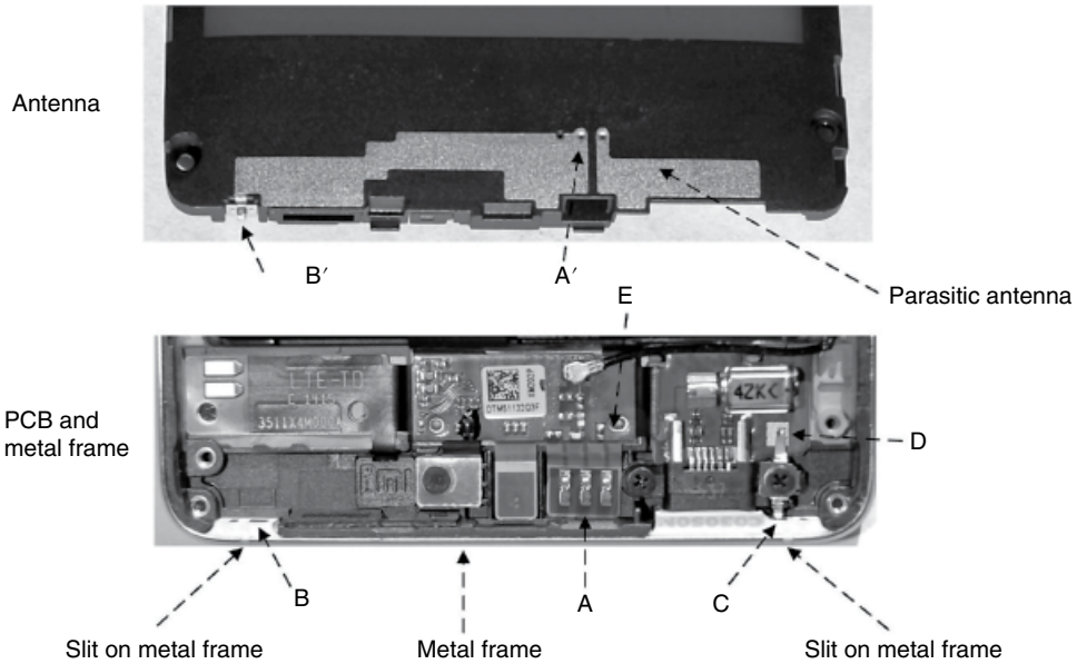
Figure 4.111 Xiaomi 4's primary antenna. (Source: Reproduced with permission of Xiaomi, Inc.)
