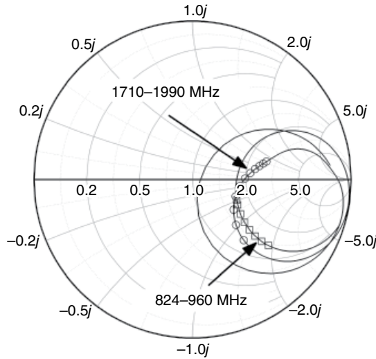
Figure 3.44 Impedance of the original Figure 3.40a antenna.
