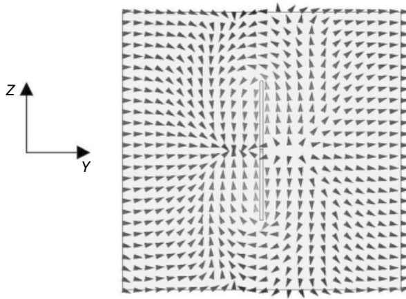
Figure 4.61 Instantaneous current distribution on a finite ground.
