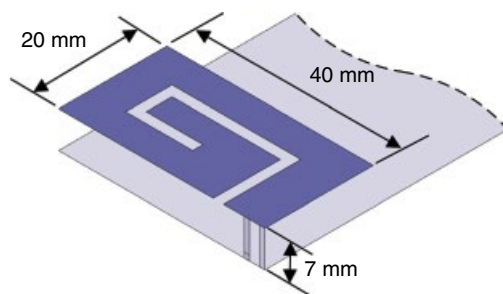
Figure 4.23 A small PIFA.
