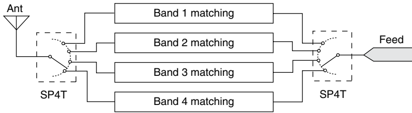
Figure 2.38 Reconfigurable matching circuits with four positions: SP4T architecture.
