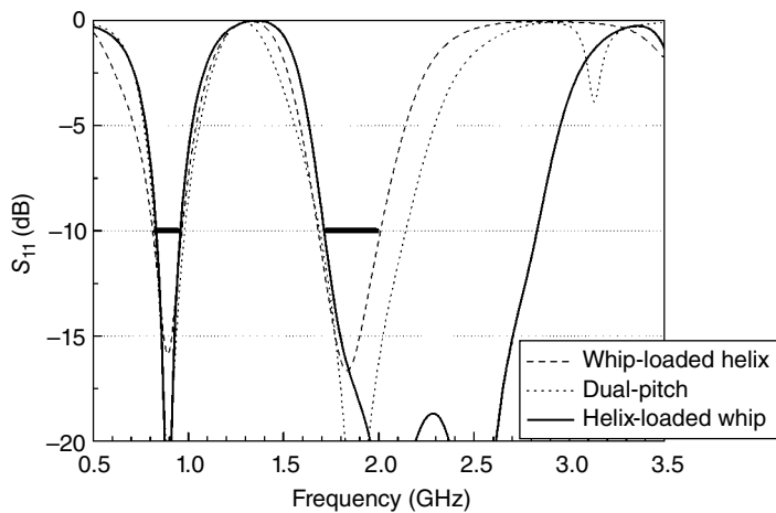
Figure 3.57 Comparison among three single-branch multiband antennas.
