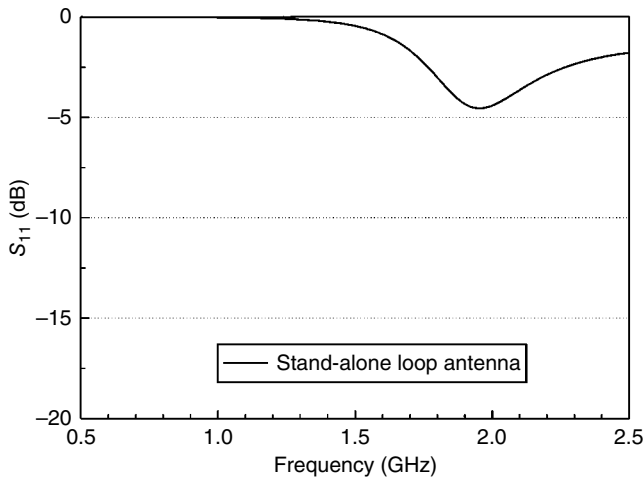
Figure 4.44 Reflection coefficient of a stand-alone loop antenna.
