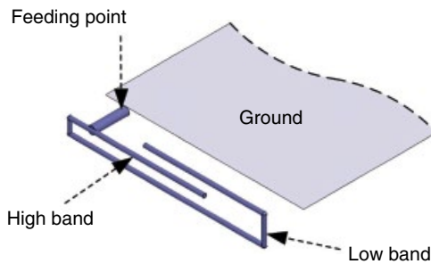
Figure 4.37 Internal folded monopole antenna.
