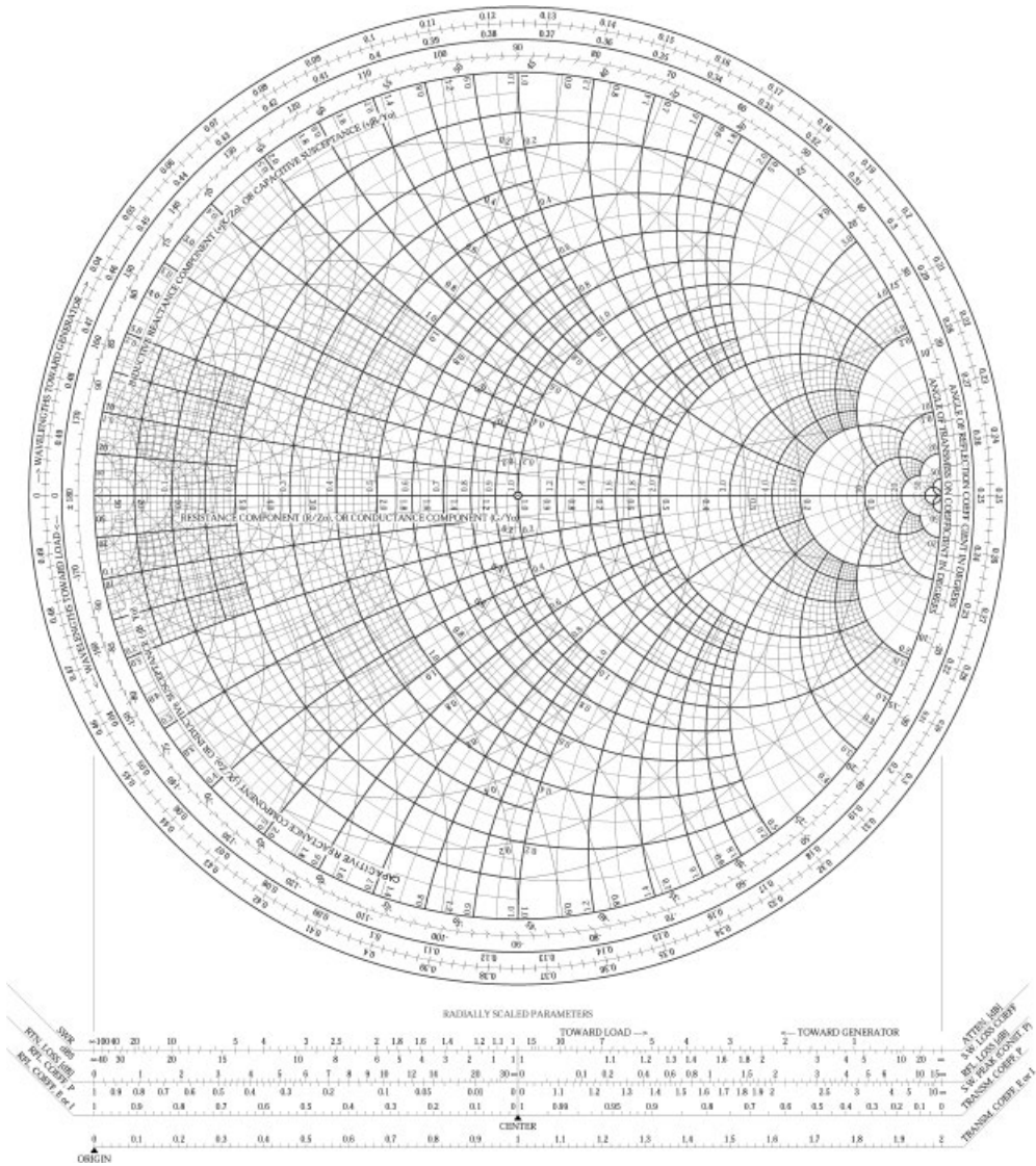
Figure 2.4 The normalized impedance and admittance Smith charts (ZY Smith chart). (Source: Reproduced from J. Colvin, “Color,” Smith Chart Form ZY-01-N , University of Florida, 1997.)
