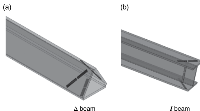
Figure 6.4 Configurations of orthogonal short dipoles.
