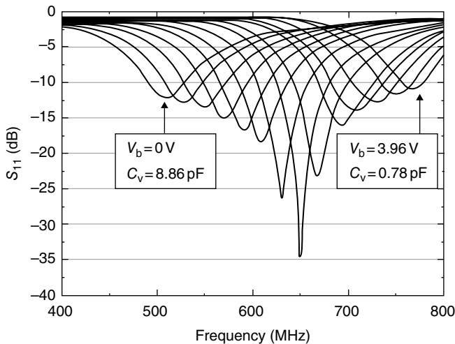
Figure 2.36 Measured S_{11} . (Source: Li et al. [16]. Reproduced with permission of John Wiley & Sons, Inc.)
