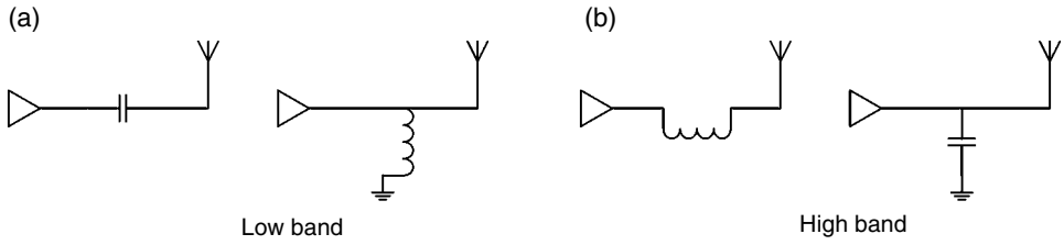
Figure 2.26 Matching components for low band and high band, respectively.
