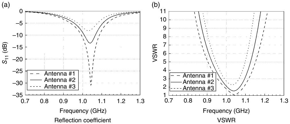
Figure 5.3 Return loss vs. VSWR.
