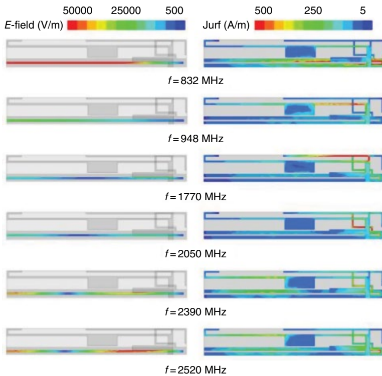
Figure 4.71 Simulated distribution of the electric field in the open slot and the surface current of the antenna. (Source: Deng et al. [27]. Reproduced with permission of IEEE.)
