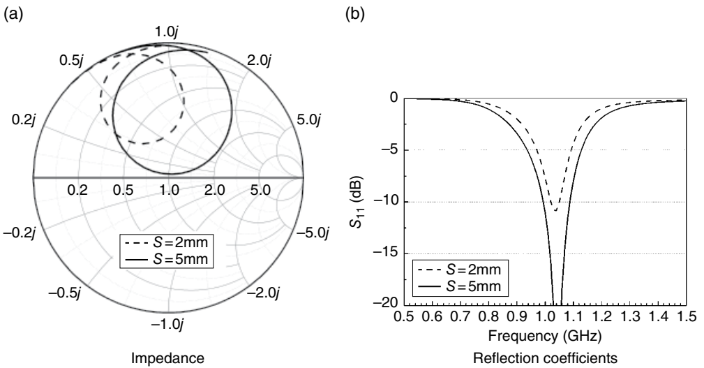
Figure 4.6 Impact of separation S on an IFA.
