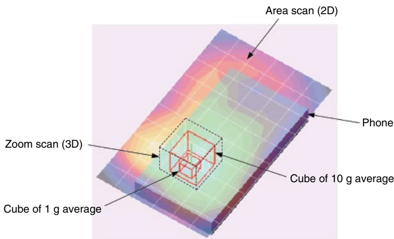
Figure 6.7 Cube of 1 and 10 g average on a body phantom.
