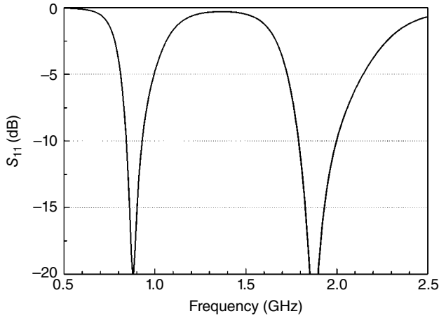
Figure 4.28 Reflection coefficient of the large PIFA.
