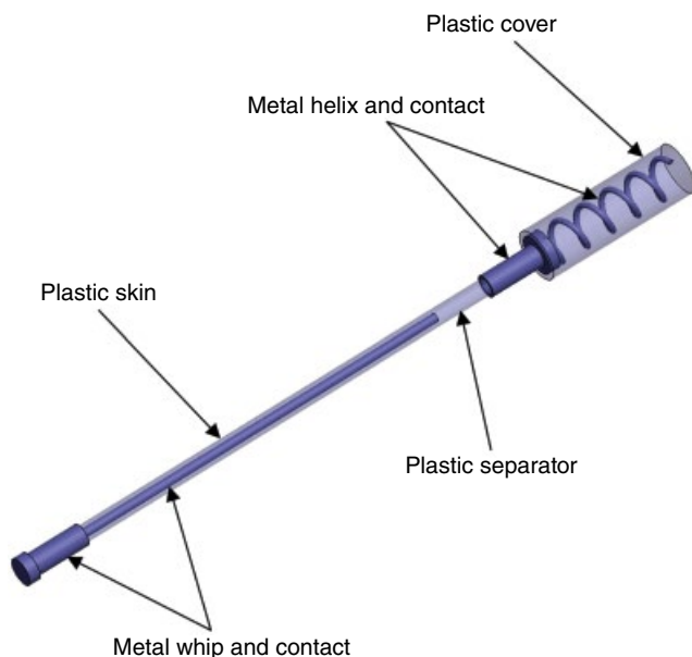
Figure 3.73 Decoupled whip–stubby antenna.
