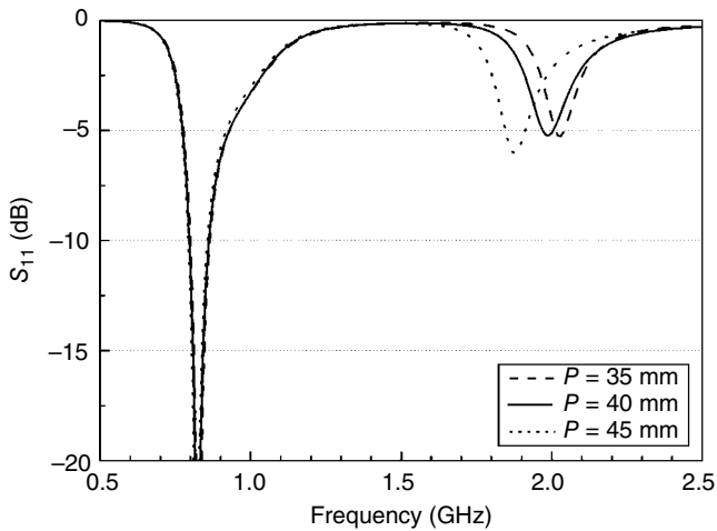
Figure 4.18 Impact of dimension P . 50\text{ mm} \times 25\text{ mm} Patch, C = 35\text{ mm} , D = 10\text{ mm} .
