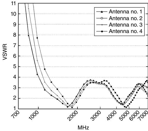
Figure 3.63 VSWR versus antenna variants shown in Figure 3.62 W=8 mm, H=5 mm, L=30 mm, C-clip height=3 mm, and \theta=30^\circ .
