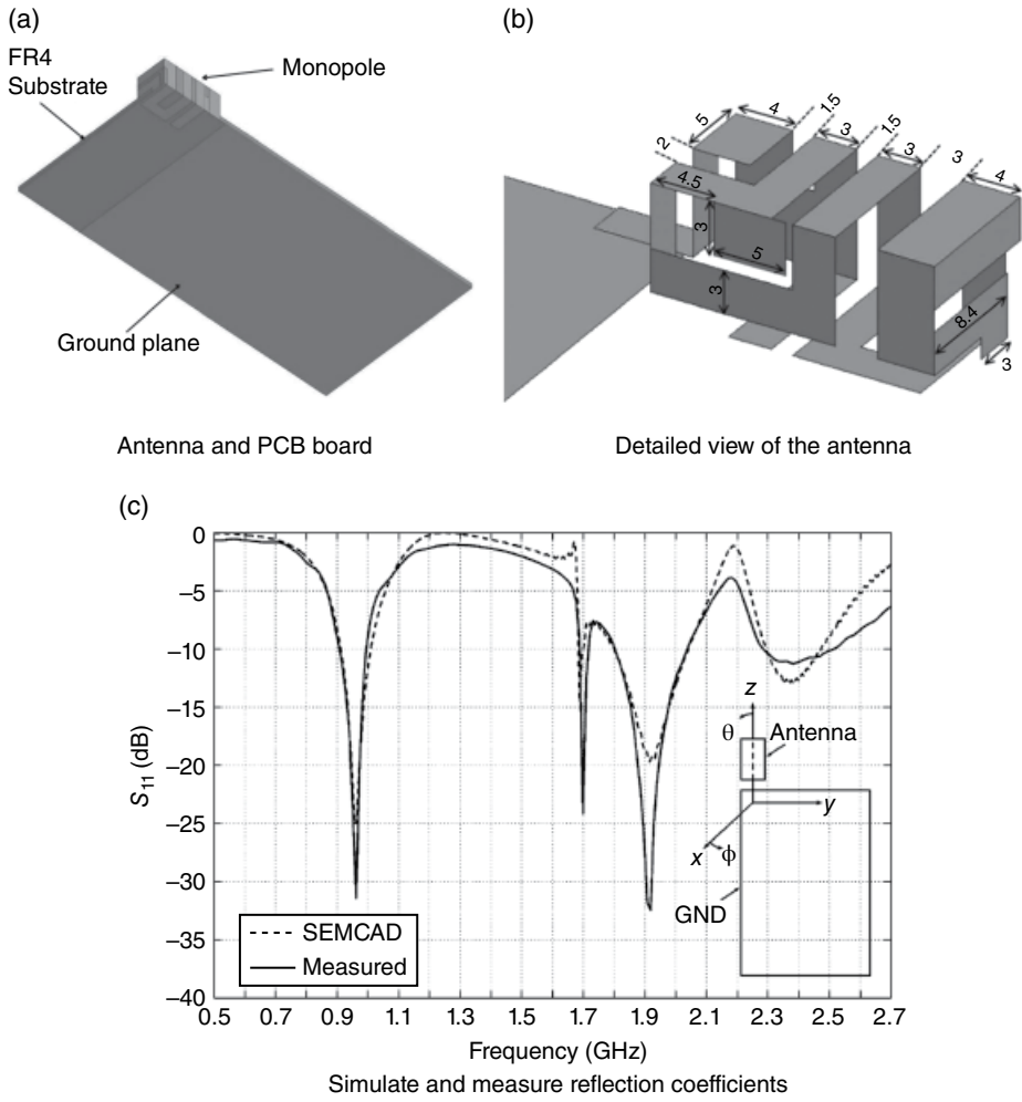
Figure 3.90 A three-dimensional multiband flex antenna. (Source: Kanj and Ali [28]. Reproduced with permission of IEEE.)
