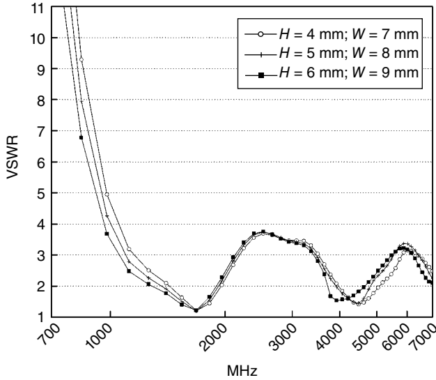
Figure 3.65 VSWR versus antenna width and height L=30 mm, C-clip height=3 mm, and \theta=30^\circ . (Source: Zhang et al. [24]. Reproduced with permission of IEEE.)
