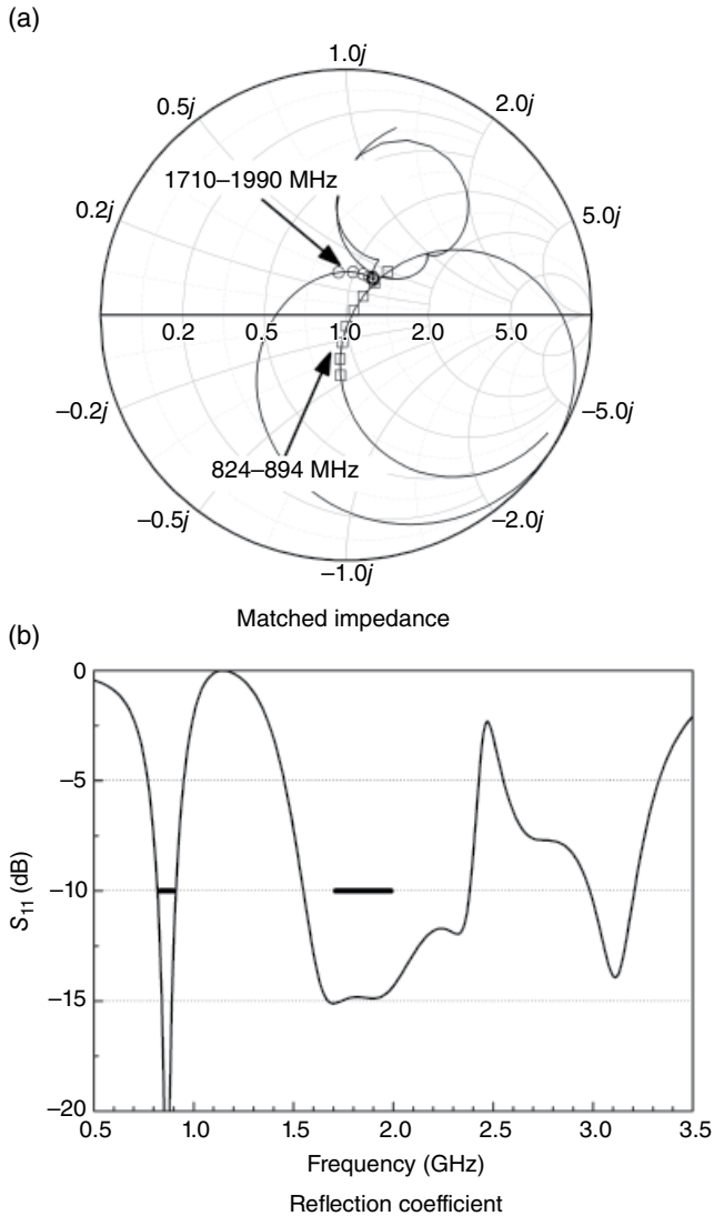
Figure 3.32 Matched dual-branch stubby antenna.
