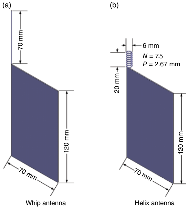
Figure 3.18 Dimensions of two antennas designed to cover 824–894 MHz.
