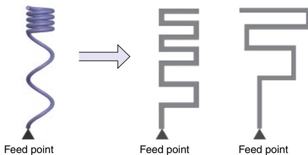
Figure 3.89 Variants of multi-pitch-type meander line antennas.
