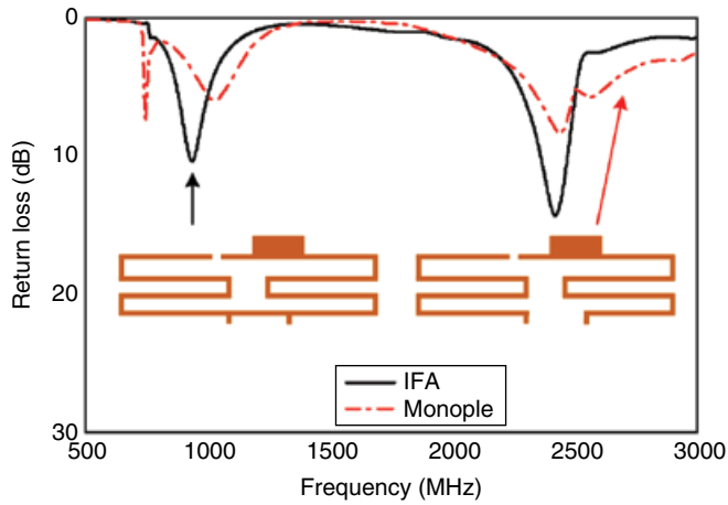
Figure 4.80 Simulated return loss of IFA mode of the proposed antenna with or without the matching bridge. (Source: Li et al. [31]. Reproduced with permission of IEEE.)
