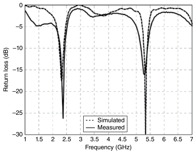
Figure 3.85 Reflection coefficients. (Source: Khaleghi [26]. Reproduced with permission of IEEE.)
