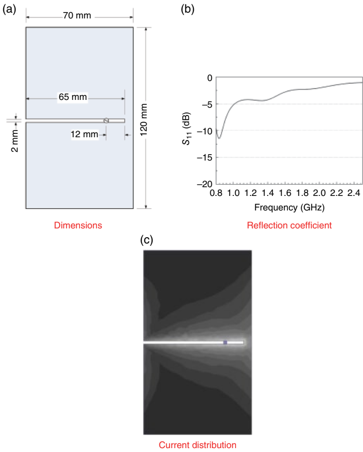
Figure 4.64 A quarter-wavelength slot in the middle.
