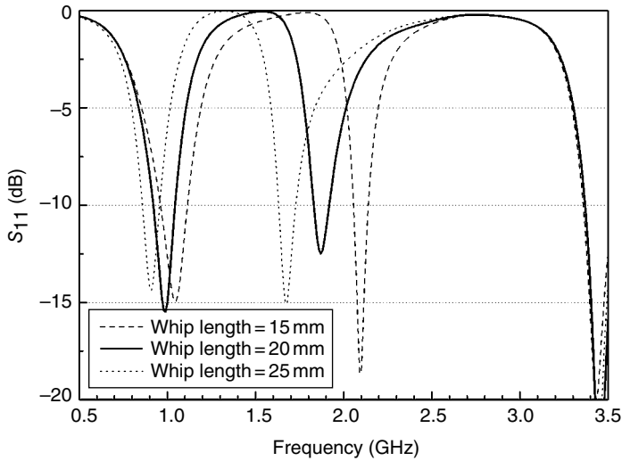
Figure 3.54 Simulated reflection coefficients.
