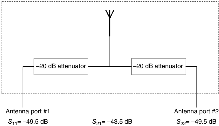
Figure 4.90 A “perfect” dual-port MIMO antenna.
