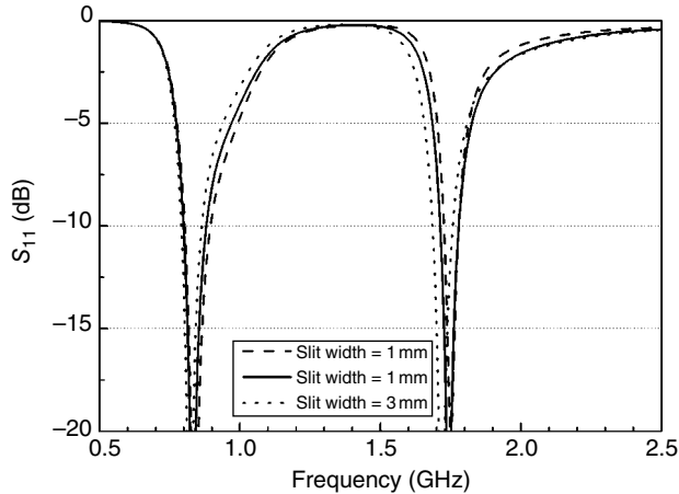
Figure 4.20 Bandwidth trade-off between low and high bands.
