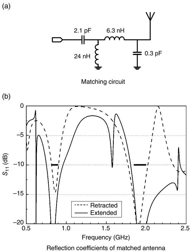
Figure 3.81 Matching both retracted and extended positions.
