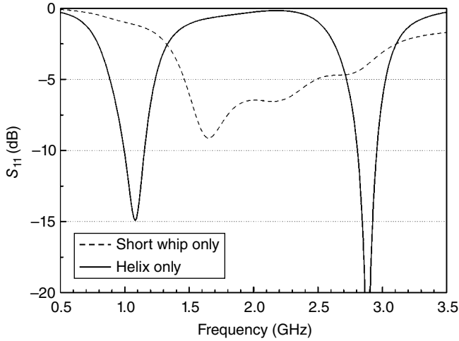
Figure 3.29 Reflection coefficients of a whip-only antenna and a helix-only antenna.
