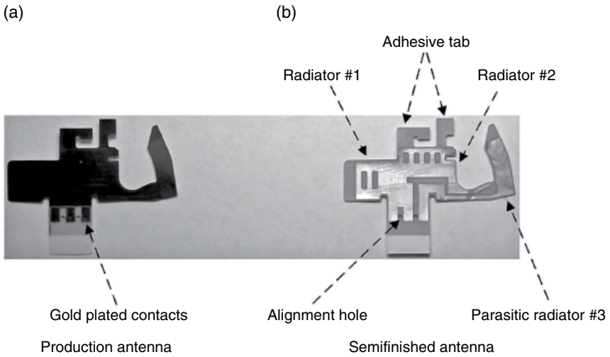
Figure 4.101 Hongmi 2A's secondary antenna. (Source: Reproduced with permission of Xiaomi, Inc. and Shanghai Amphenol Airwave, Inc.)
