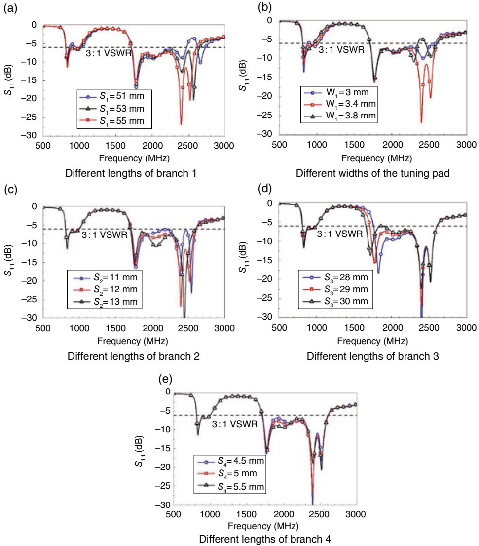
Figure 4.72 Parametric studies. (Source: Deng et al. [27]. Reproduced with permission of IEEE.)
