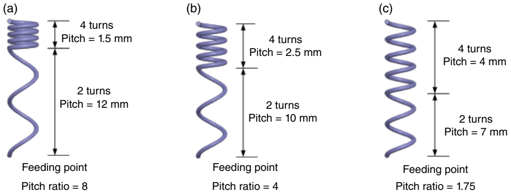
Figure 3.40 Effect of different pitches.
