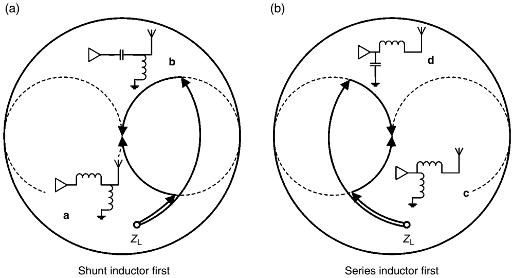
Figure 2.9 Four matching options of single load impedance.
