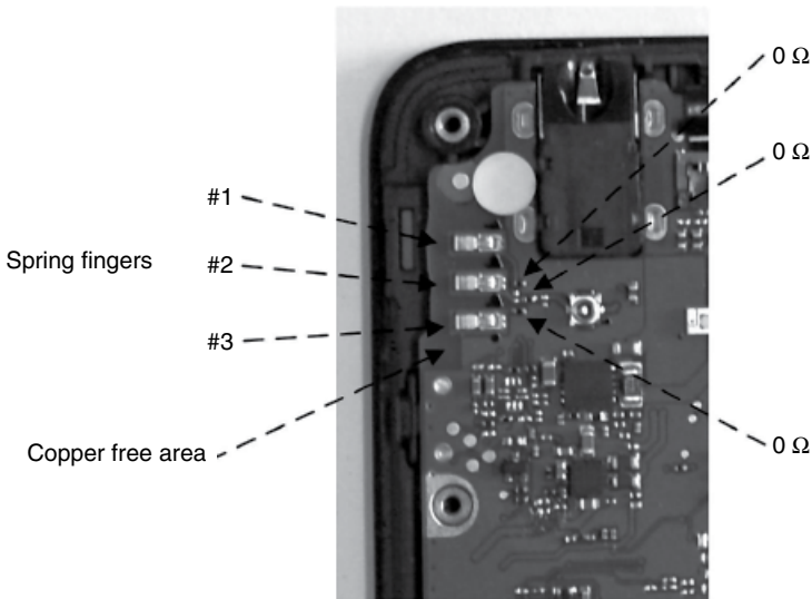
Figure 4.103 Matching circuit of the secondary antenna. (Source: Reproduced with permission of Xiaomi, Inc.)
