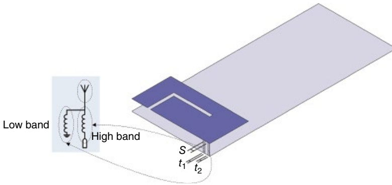
Figure 4.21 Equivalent circuit of feeding and grounding strips.
