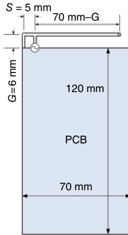
Figure 4.5 Inverted-F antenna (IFA).
