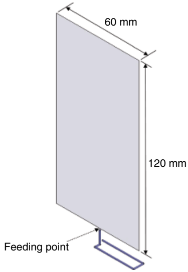
Figure 4.48 Bottom-installed monopole antenna.
