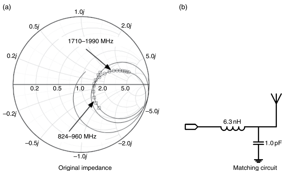
Figure 3.55 Matching a whip-loaded helix.
