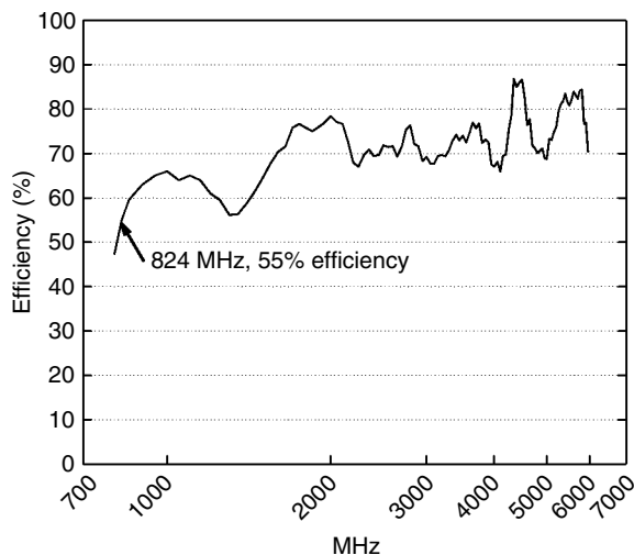
Figure 3.70 Measured efficiency data of the prototype antenna with matching network. (Source: Zhang et al. [24]. Reproduced with permission of IEEE.)
