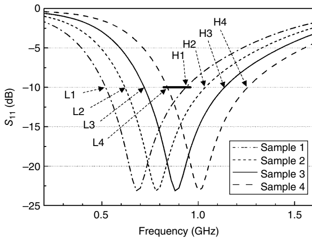
Figure 5.37 Antennas’ response measured on a phone.
