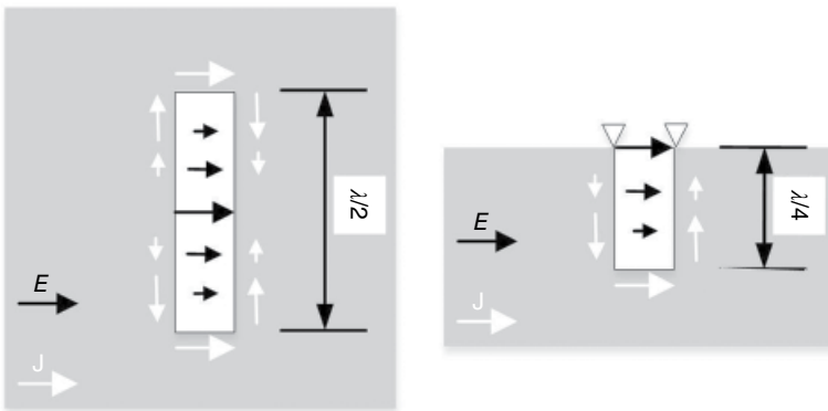
Figure 4.62 Different modes of a slot antenna
