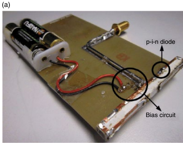
Photo of the proposed antenna with bias circuit
