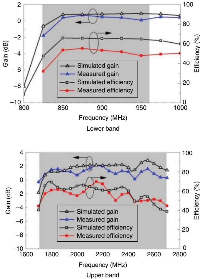
Figure 4.75 Simulated and measured gain and efficiency. (Source: Deng et al. [27]. Reproduced with permission of IEEE.)
