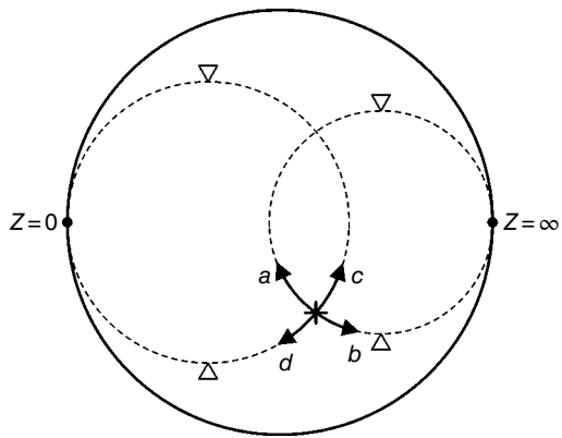
Figure 2.6 Always two circles running through a given impedance on the Smith chart.
