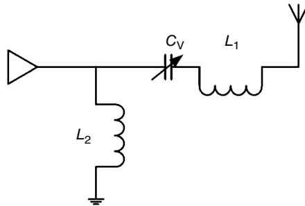
Figure 2.33 Diagram of matching circuit.
