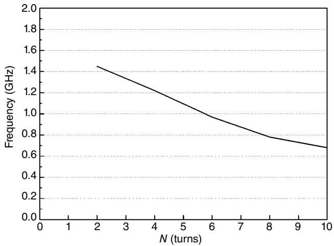
Figure 3.16 Resonant frequency versus number of turns, H=31.5\text{ mm} and D=6\text{ mm} .
