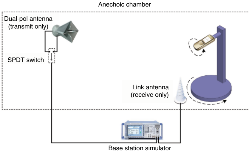
Figure 5.30 Simplified block diagram of a TIS test setup.
