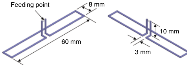
Figure 4.43 Oblique views of a loop antenna.
