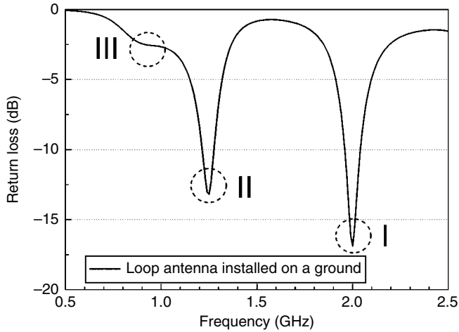
Figure 4.47 Reflection coefficient of a bottom-installed loop antenna.
