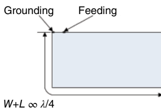
Figure 4.12 Estimating the resonant frequency of a PIFA.
