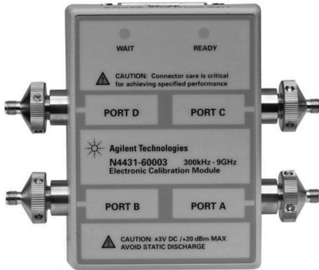
Figure 5.16 E-Cal Module N4431-60003. (Source: Reproduced with permission of Agilent Technologies.)
