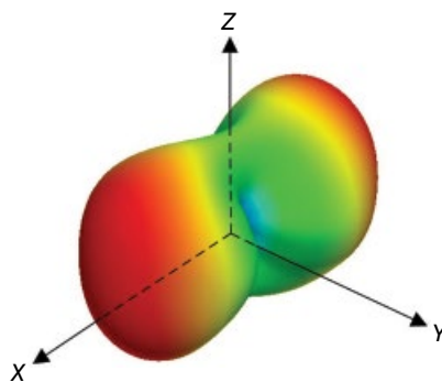
Radiation pattern
