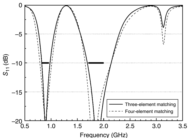
Figure 3.47 Simulated reflection coefficients of the matched Figure 3.40a antenna.
