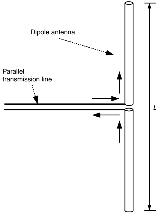
Figure 3.5 Dipole antenna.
