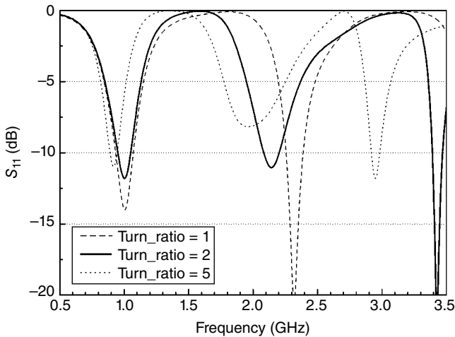
Figure 3.43 Simulated reflection coefficients.
