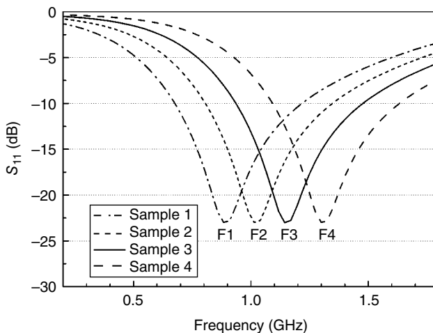
Figure 5.38 Antennas' response measured on an S_{11} fixture.
