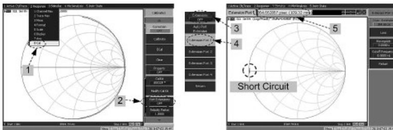
Figure 5.18 Port extension interface.
