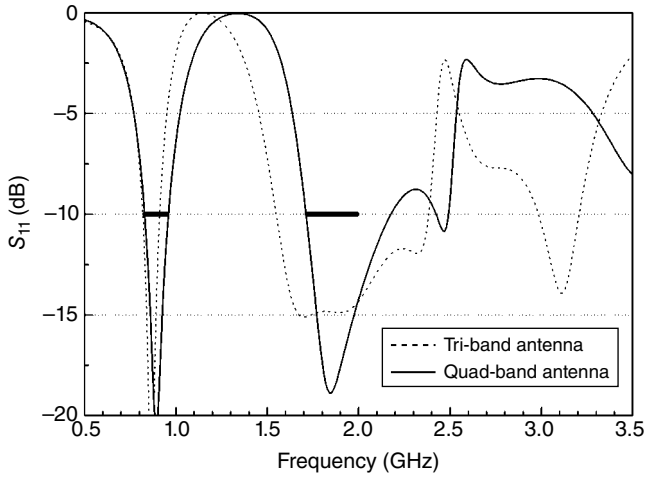
Figure 3.35 Reflection coefficient of the quad-band antenna.
