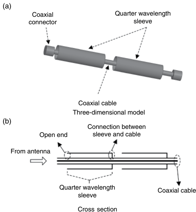
Figure 5.12 Sleeve choke.
