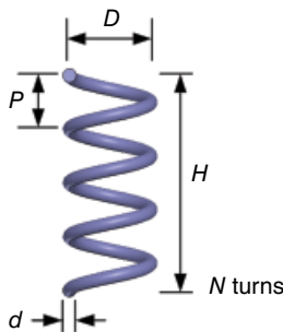
Figure 3.10 Critical dimensions of a helix.
