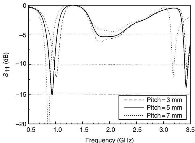
Figure 3.49 Simulated reflection coefficients.
