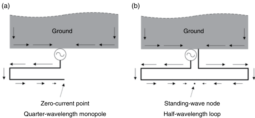
Figure 4.50 Current distributions of a monopole and a loop.
