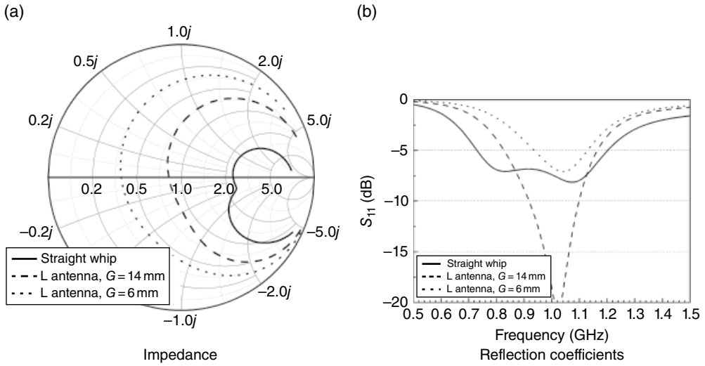
Figure 4.3 Impact of separation G on an L-shaped antenna.
