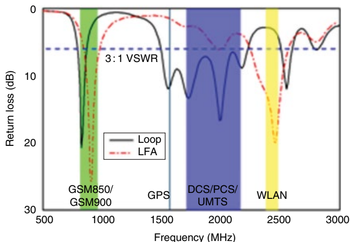
Figure 4.77 Measured return loss of loop and IFA modes of the proposed antenna. (Source: Li et al. [31]. Reproduced with permission of IEEE.)
