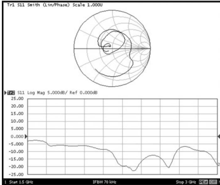
Figure 5.4 Displaying both the VSWR and the Smith chart on a VNA.
