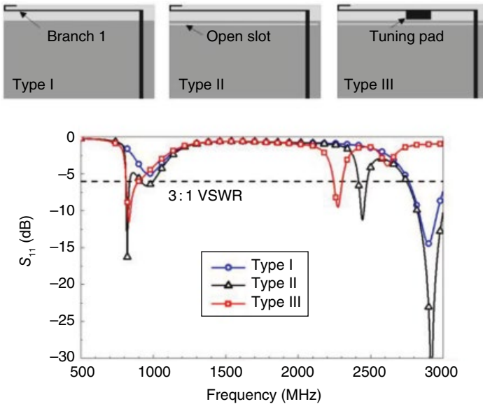
Figure 4.68 Comparison of simulated S_{11} for different antenna types. Type I: only branch 1, Type II: Type I+ open slot, and Type III: Type II+ tuning pad. (Source: Deng et al. [27]. Reproduced with permission of IEEE.)
