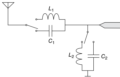
Figure 2.40 Reconfigurable matching circuit with four states: SPDT architecture.
