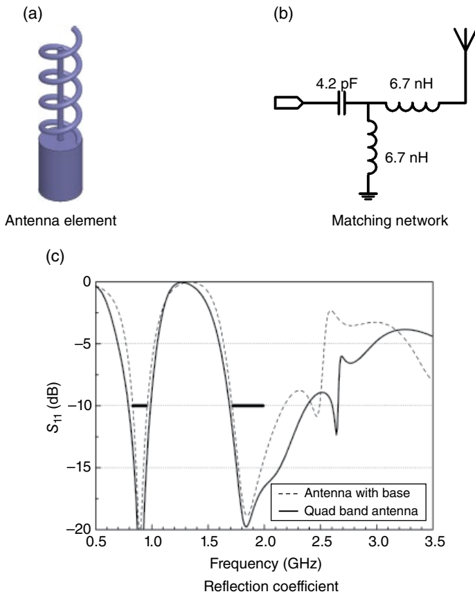
Figure 3.36 Antenna with a metal base.
