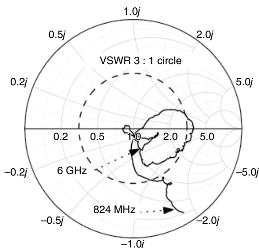
Figure 3.67 Measured impedance of the prototype antenna without matching.
