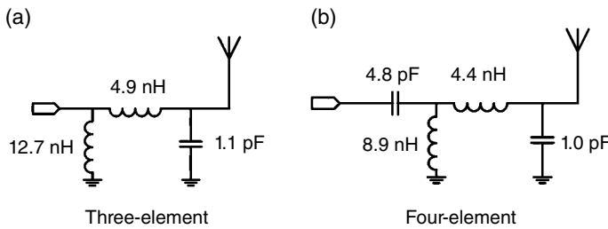
Figure 3.45 Matching circuits for the Figure 3.40a antenna.
