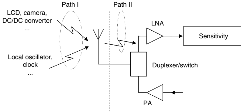
Figure 5.31 Some causes of desense.
