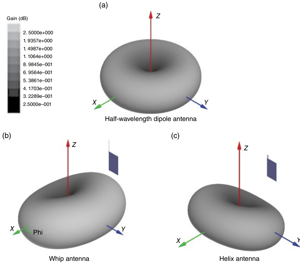
Figure 3.24 Three-dimensional radiation patterns at 850 MHz.
