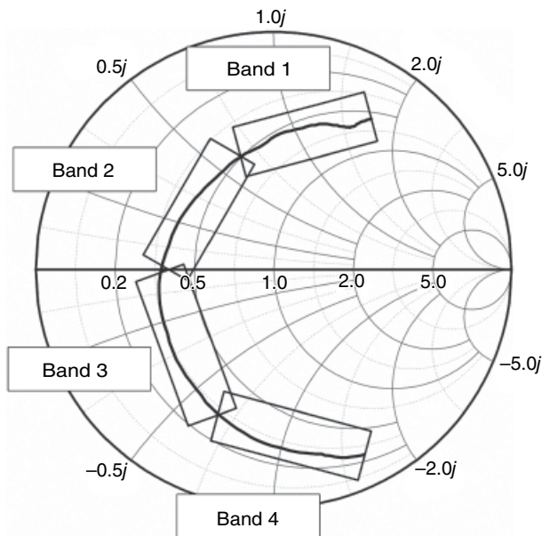
Figure 2.37 Dividing the impedance curve into four regions.
