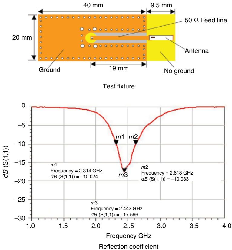
Figure 4.54 Performance of Johanson Technology 2450AT43A100. (Source: Reproduced with permission of Johanson Technology.)
