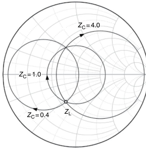
Figure 2.14 The impedance's moving path on the transmission lines.
