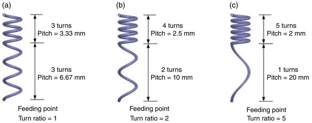
Figure 3.42 Effect of different turns on small pitch portion.
