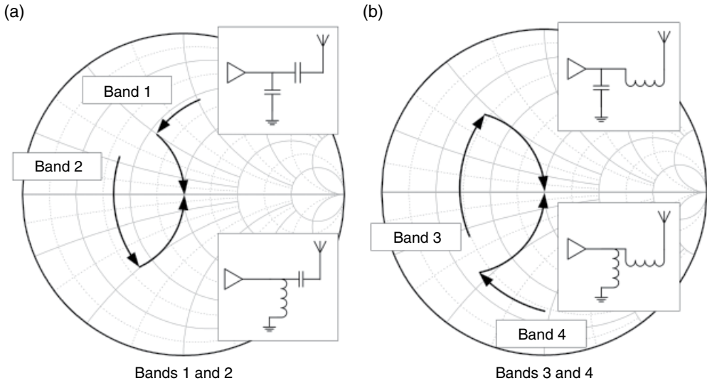
Figure 2.39 Corresponding matching circuits of four regions.
