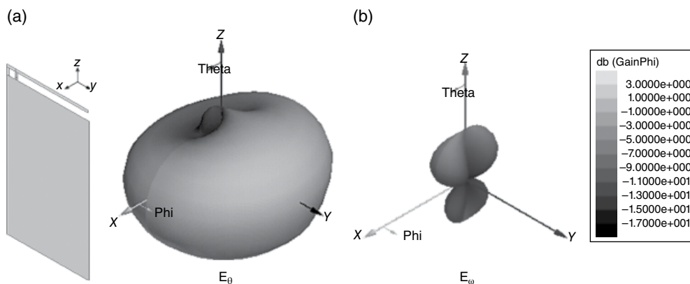
Figure 4.9 Three-dimensional radiation patterns, IFA, S=5 mm, 1.05 GHz.
