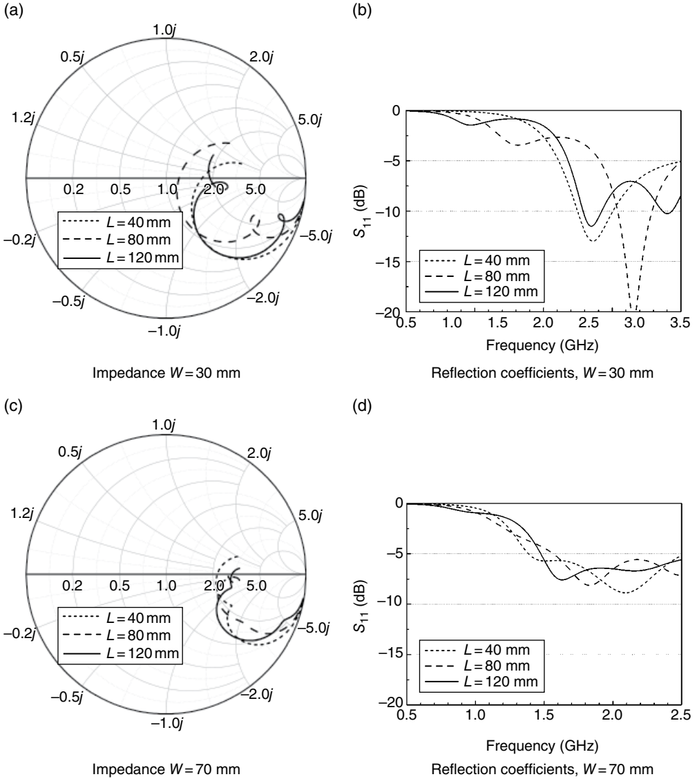
Figure 3.96 Effect of ground width and length, L_{ant} = 30 mm.
