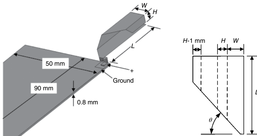
Figure 3.61 Mechanical drawing. (Source: Zhang et al. [24]. Reproduced with permission of IEEE.)
