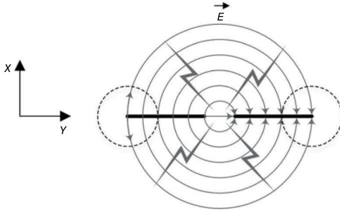
Figure 4.60 Explanation of the radiation null along the Y-axis.
