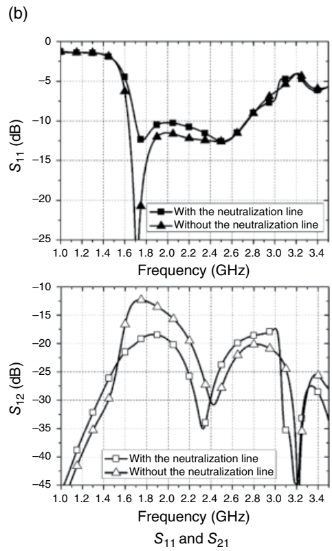
Figure 4.94 A wideband dual antenna. (Source: Wang and Du [42]. Reproduced with permission of IEEE.)
