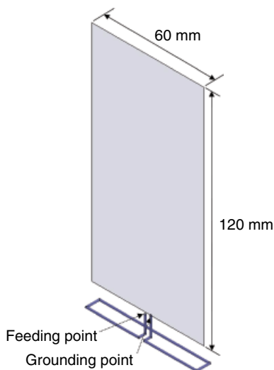
Figure 4.46 Bottom-installed loop antenna.
