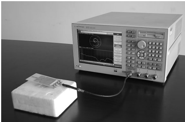
Figure 5.5 A fixture connected to a VNA.
