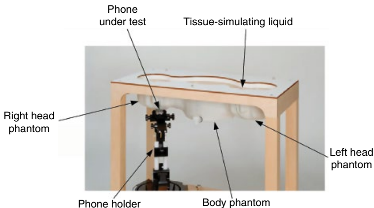
Figure 6.1 Phantom used in SAR measurements (Twin SAM). (Source: Reproduced with permission of Schmid & Partner Engineering AG.)
