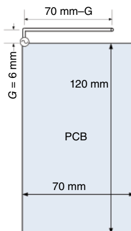
Figure 4.2 L-shaped antenna.
