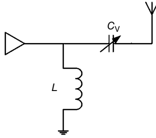
Figure 2.32 Matching circuit of the original antenna.
