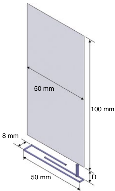
Figure 4.38 Dimensions of a sample internal monopole antenna.
