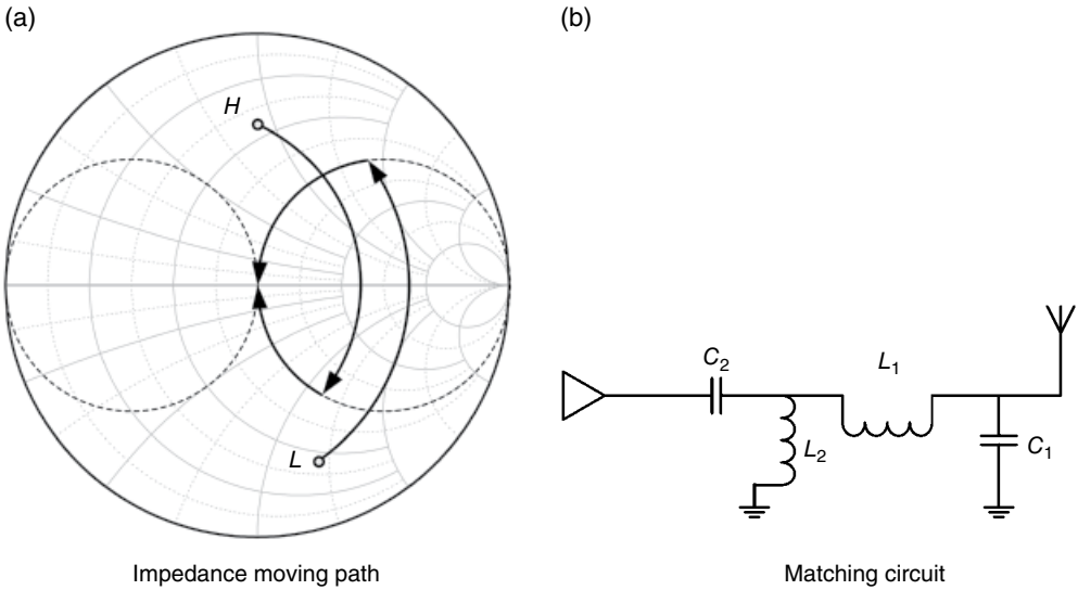
Figure 2.27 Dual-band matching Example 2.1.
