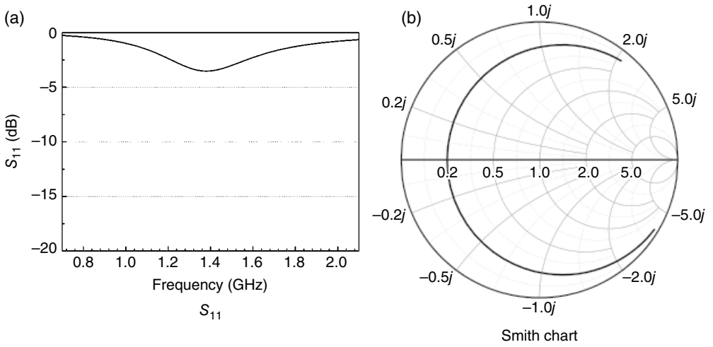
Figure 2.19 Original antenna impedance before matching.
