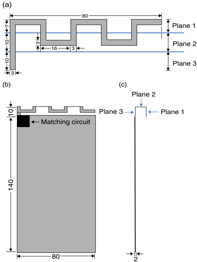
Figure 2.34 Geometry of meander line antenna: (a) antenna element, (b) front view, and (c) side view. (Source: Li et al. [16]. Reproduced with permission of John Wiley & Sons, Inc.)
