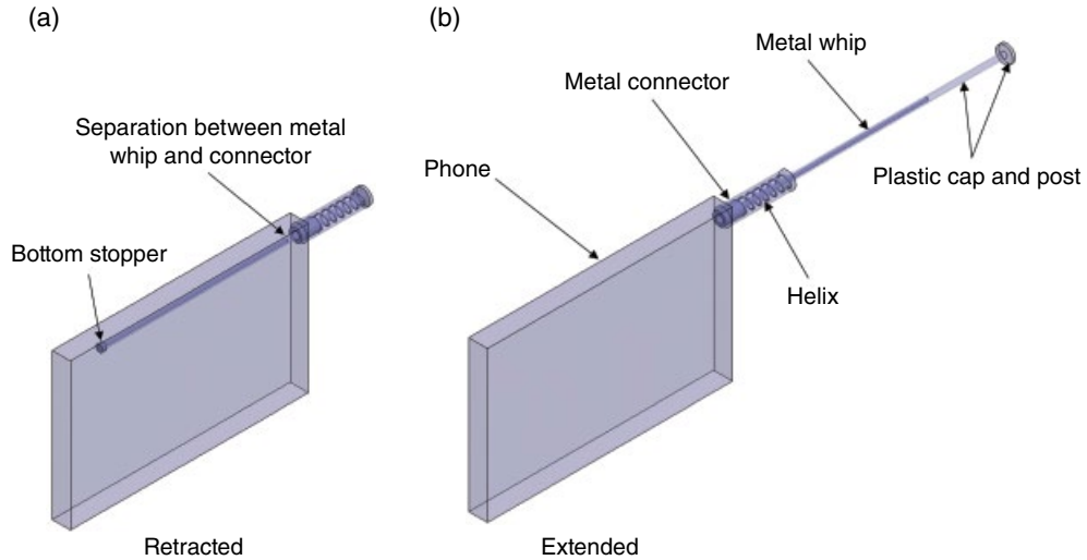
Figure 3.77 A semi-decoupled whip–stubby antenna on a phone.
