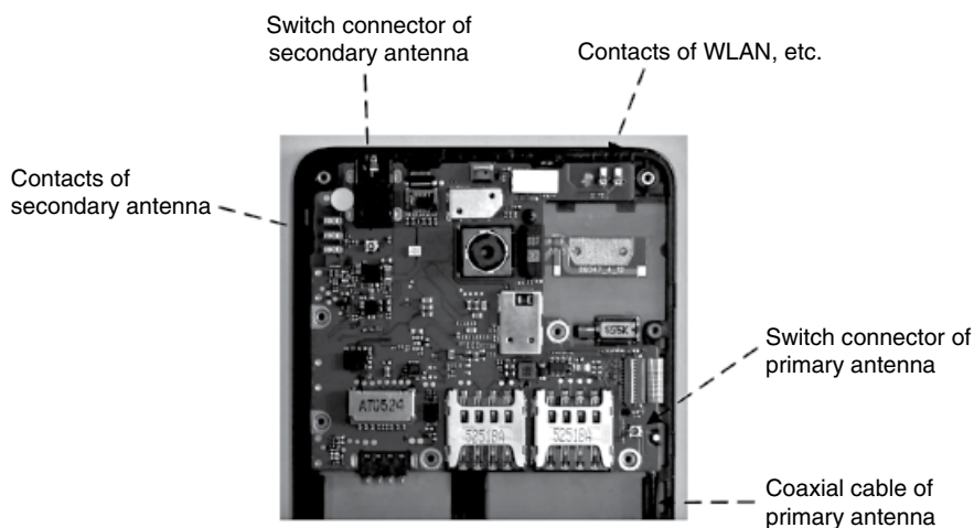
Figure 4.107 Switch connectors on the PCB. (Source: Reproduced with permission of Xiaomi, Inc.)
