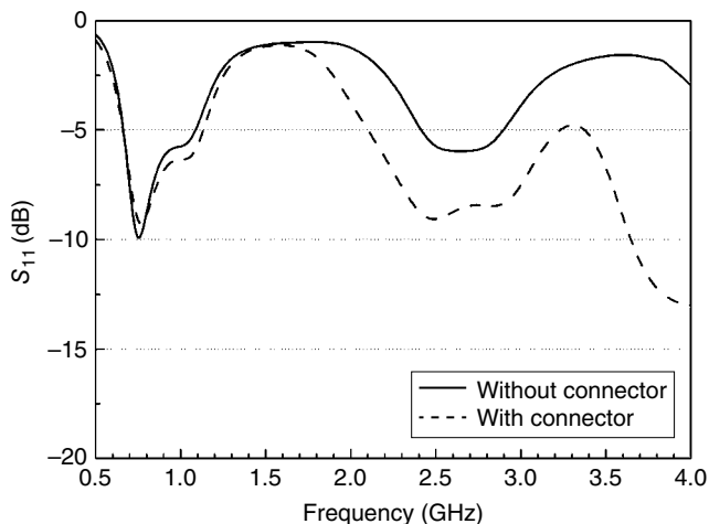
Figure 3.76 Metal connector's impact on whip antennas.
