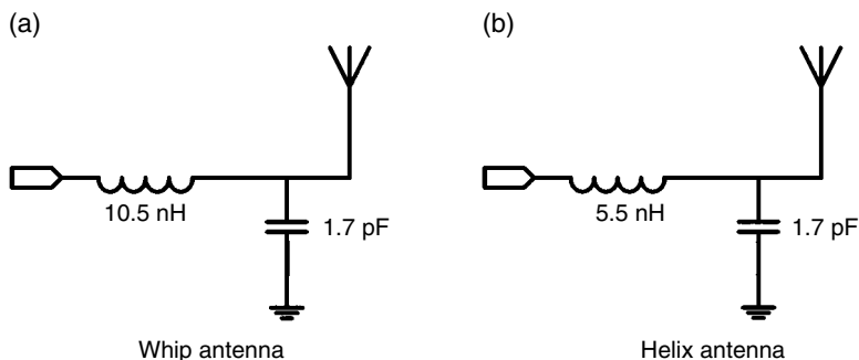
Figure 3.21 Matching circuits of whip and helix antennas.
