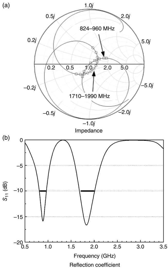
Figure 3.56 Matched whip-loaded helix antenna.
