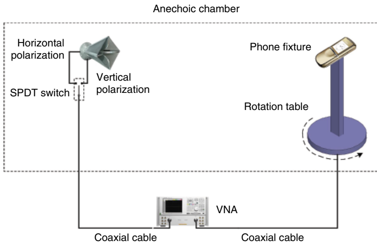
Figure 5.22 Simplified block diagram of a 2D test setup.
