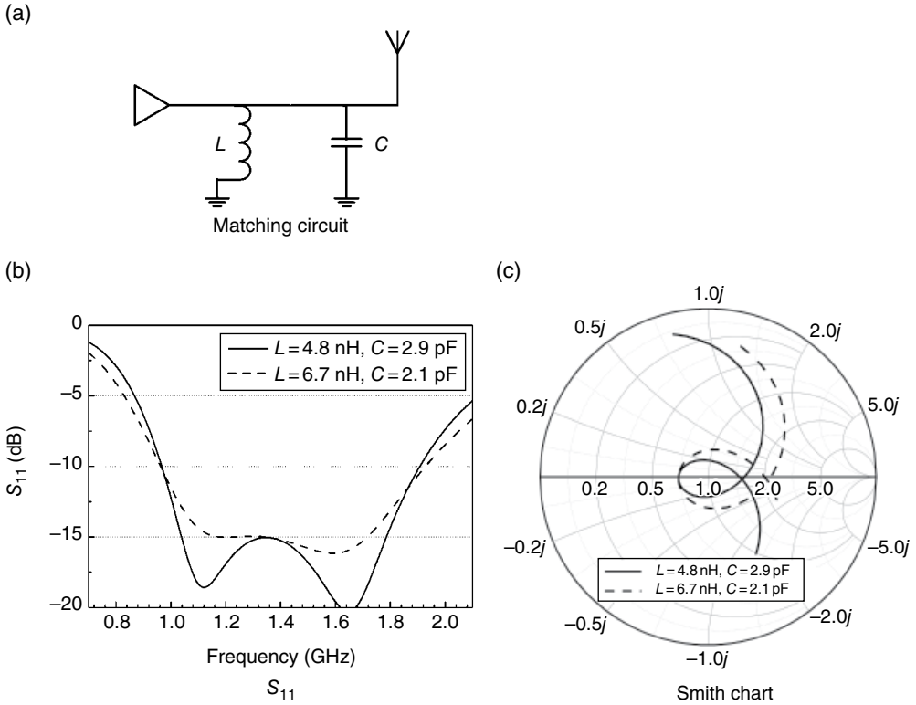
Figure 2.18 Shunt LC resonator as a matching circuit.
