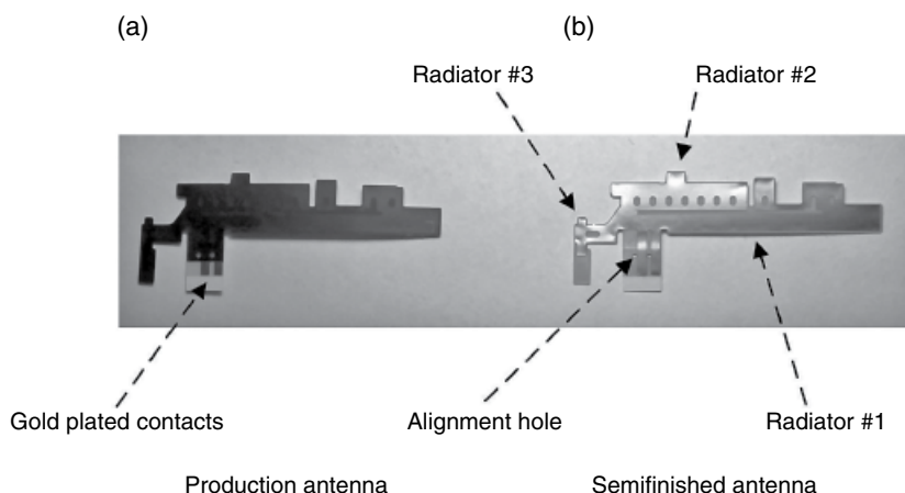
Figure 4.98 Hongmi 2A's primary antenna. (Source: Reproduced with permission of Xiaomi, Inc. and Shanghai Amphenol Airwave, Inc.)
