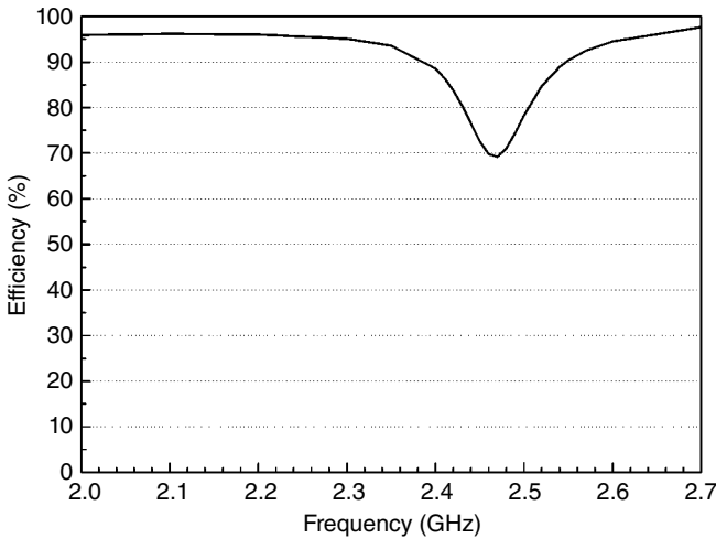
Figure 3.30 Antenna radiation efficiency.
