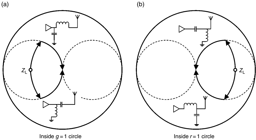
Figure 2.12 Two matching options of single load impedance.
