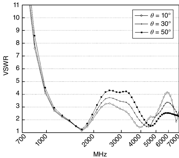
Figure 3.64 Antenna VSWR versus different taper angle W=8 mm, H=5 mm, L=30 mm, and C-clip height=3 mm. (Source: Zhang et al. [24]. Reproduced with permission of IEEE.)
