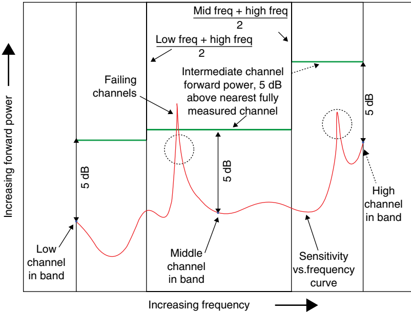
Figure 5.33 Illustration of intermediate channel test. (Source: CTIA.)
