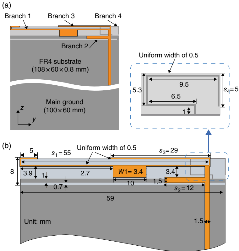
Figure 4.67 Geometry and dimensions of the antenna. (Source: Deng et al. [27]. Reproduced with permission of IEEE.)
