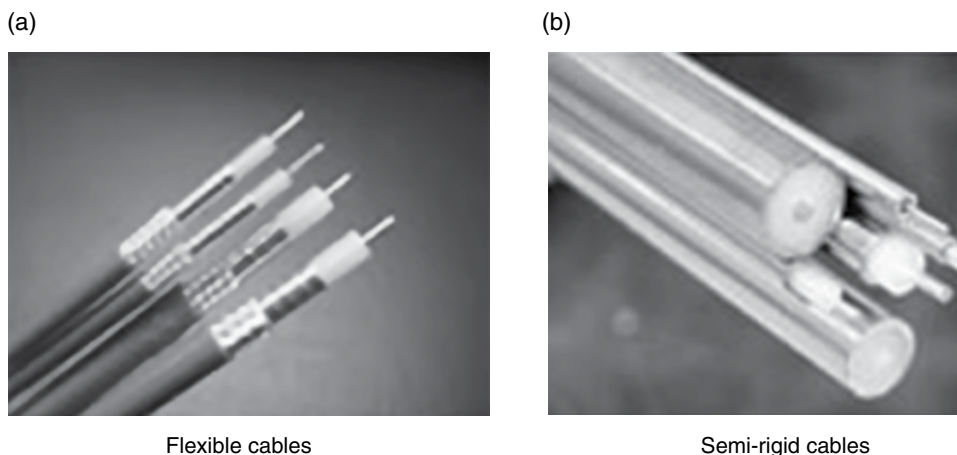
Figure 5.7 Coaxial cables.
