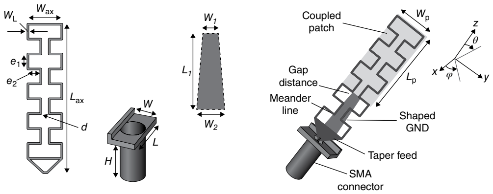
Figure 3.84 Dual-band antenna for WLAN application. (Source: Khaleghi [26]. Reproduced with permission of IEEE.)
