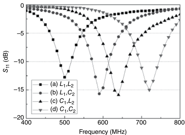
Figure 2.41 Simulated S_{11} .
