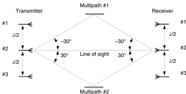
Figure 4.86 MIMO system in a multipath environment.
