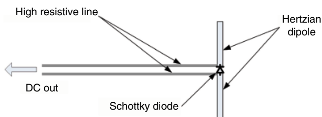
Figure 6.5 Sensor made of Schottky diode.
