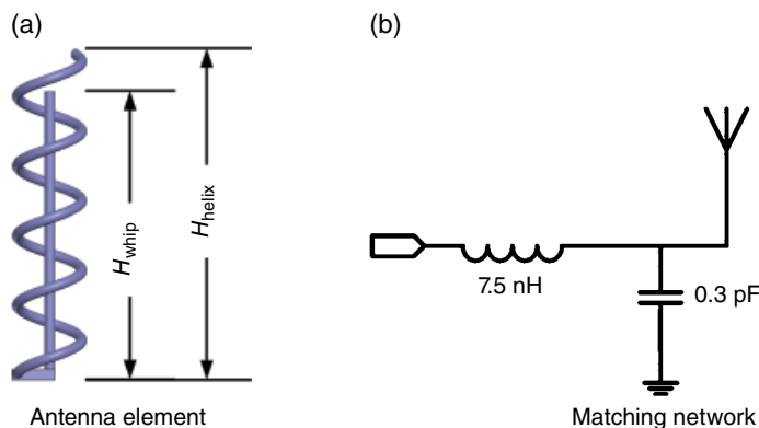
Figure 3.34 Quad-band antenna and its matching network.
