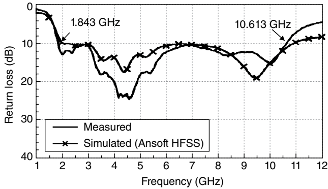
Figure 3.59 Measured and simulated return loss. (Source: Wong and Chien [19]. Reproduced with permission of IEEE.)
