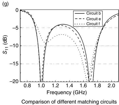
Figure 2.30 Selection of matching circuits.
