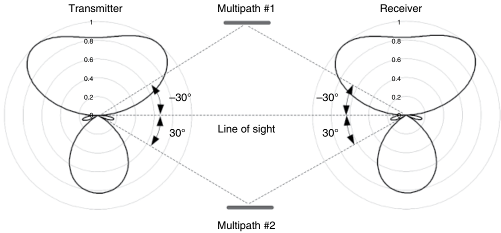
Figure 4.87 Nulled patterns corresponding to the multipath 1.
