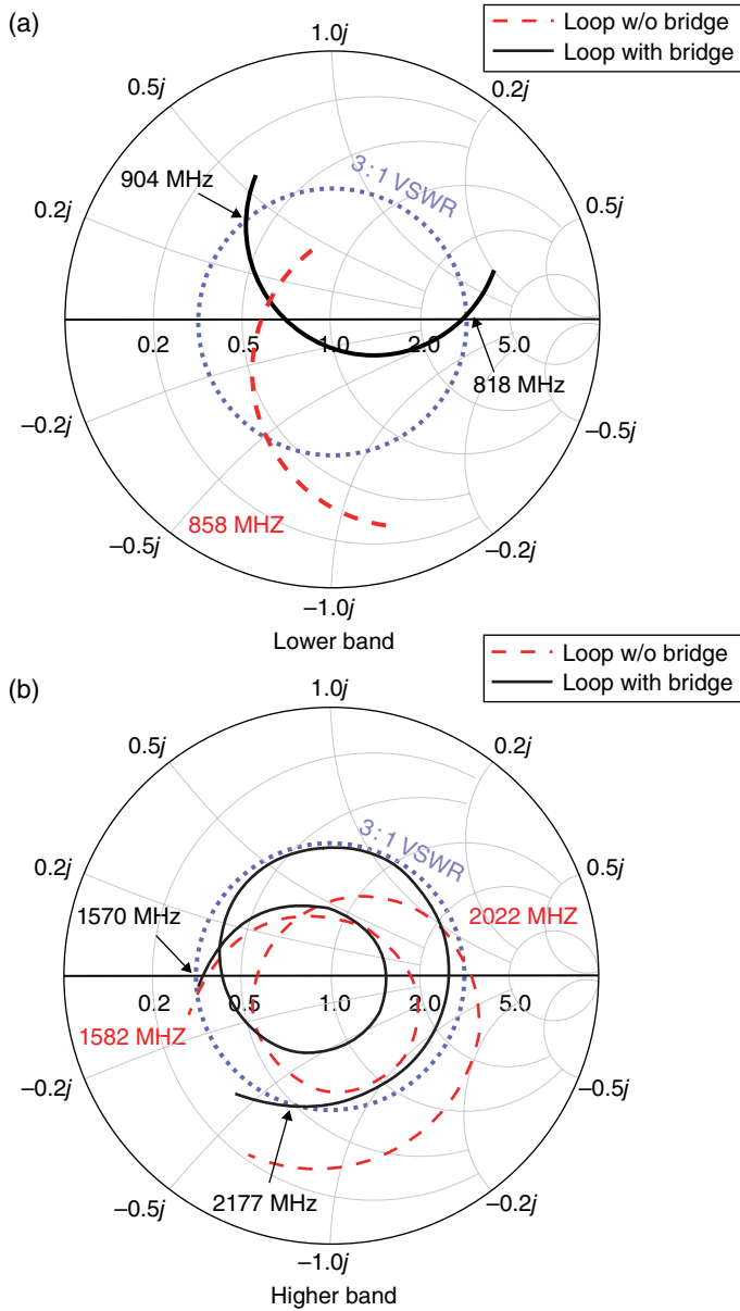
Figure 4.79 Smith chart of the loop mode with or without the matching bridge. (Source: Li et al. [31]. Reproduced with permission of IEEE.)
