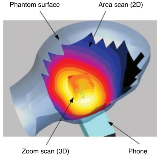
Figure 6.6 Area and zoom scanning on a left head phantom.
