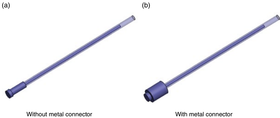
Figure 3.75 Two different whip antennas.
