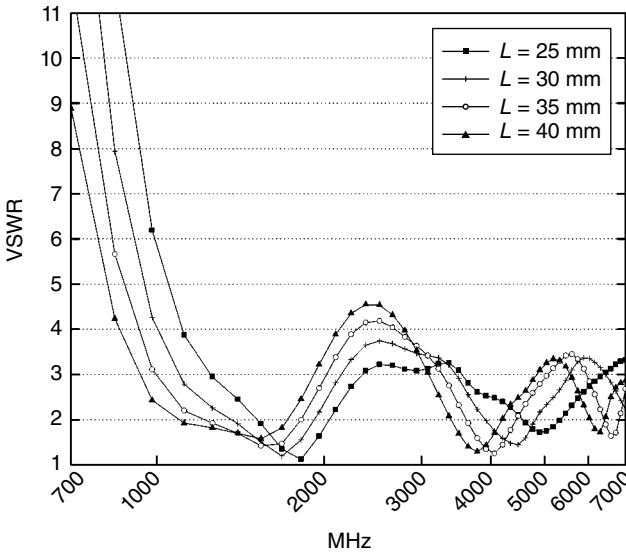
Figure 3.66 VSWR versus antenna length W=8 mm, H=5 mm, C-clip height=3 mm, and \theta=30^\circ . (Source: Zhang et al. [24]. Reproduced with permission of IEEE.)
