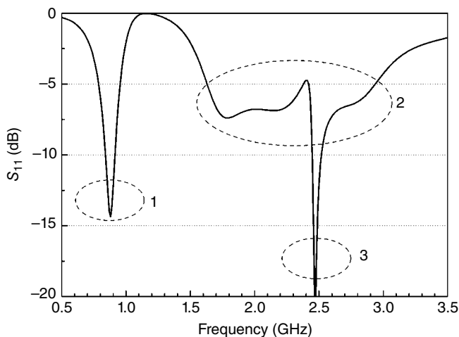
Figure 3.27 Reflection coefficient of a two-branch stubby antenna.
