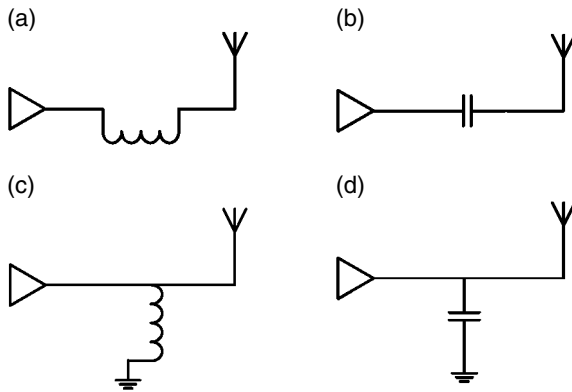
(a) Series inductor (b) Series capacitor (c) Shunt inductor (d) Shunt capacitor
