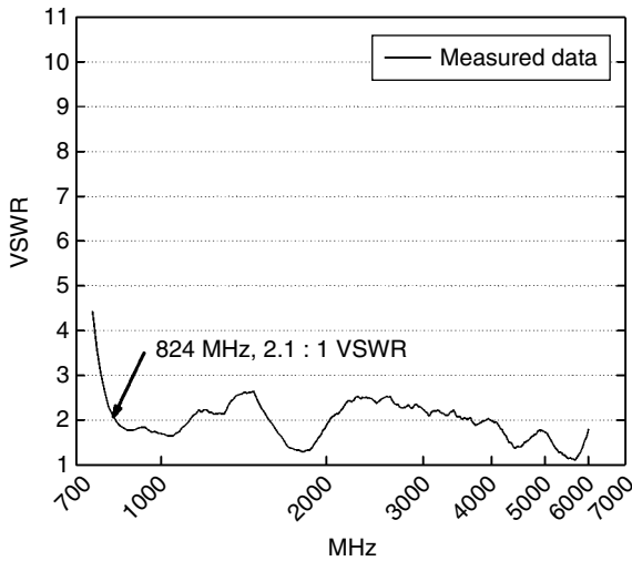
Figure 3.69 Measured VSWR data of the prototype antenna with matching network. (Source: Zhang et al. [24]. Reproduced with permission of IEEE.)
