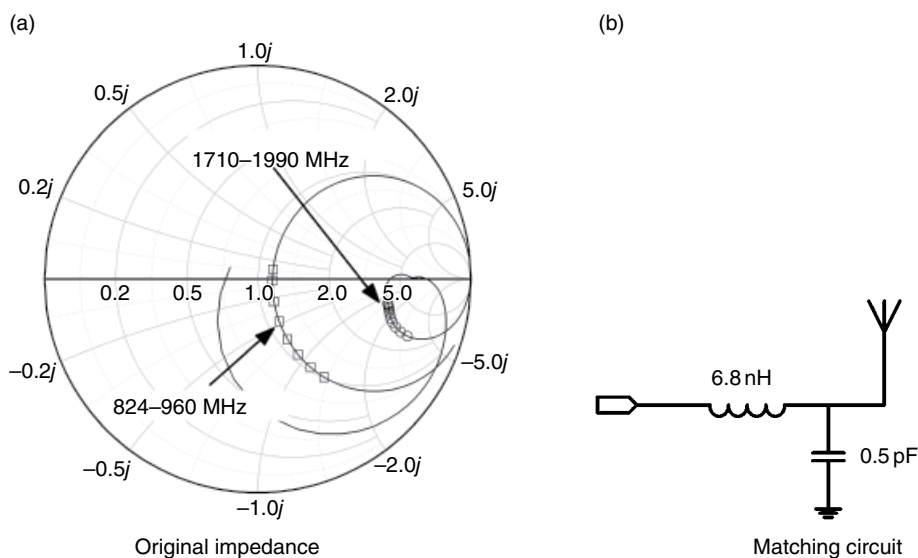
Figure 3.50 Matching a helix-loaded whip.
