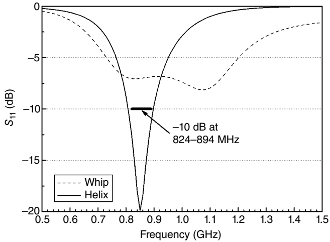
Figure 3.19 Original reflection coefficients of whip and helix antennas.
