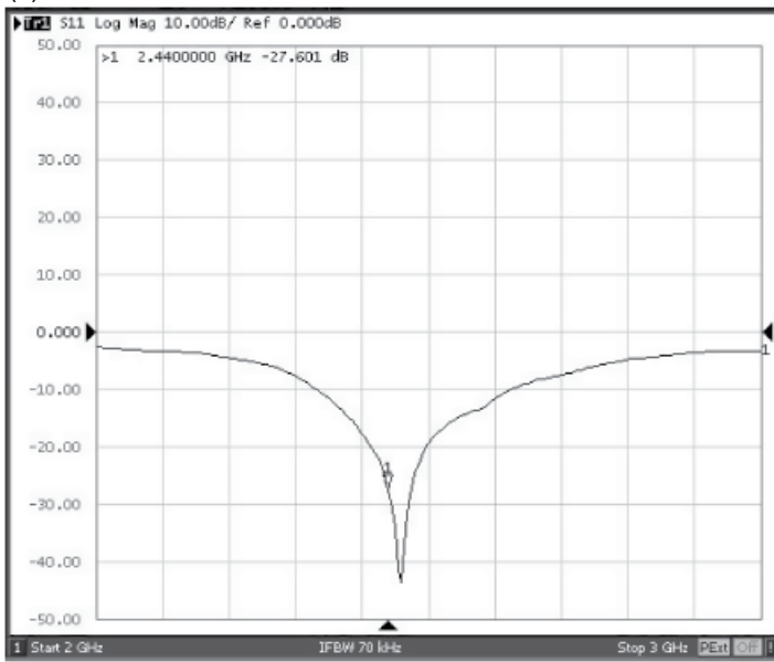
Figure 1.22 Making antenna smaller.
