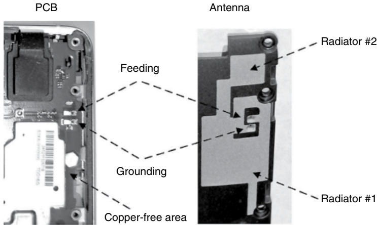
Figure 4.113 Xiaomi 4's WLAN, etc. antenna. (Source: Reproduced with permission of Xiaomi, Inc.)
