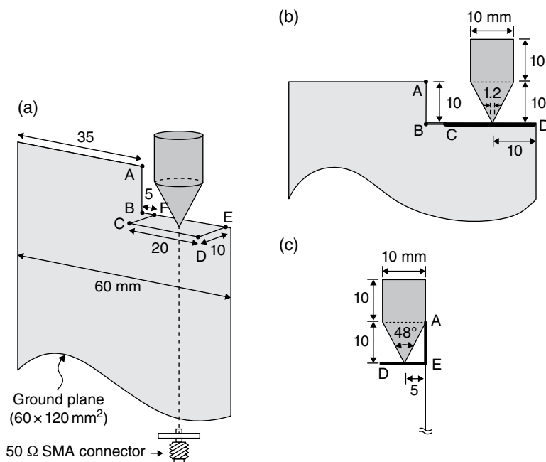
Figure 3.58 Wideband cylindrical monopole antenna. (a) Geometry of the proposed wideband cylindrical monopole antenna. (b) Front view. (c) Side view. (Source: Wong and Chien [19]. Reproduced with permission of IEEE.)
