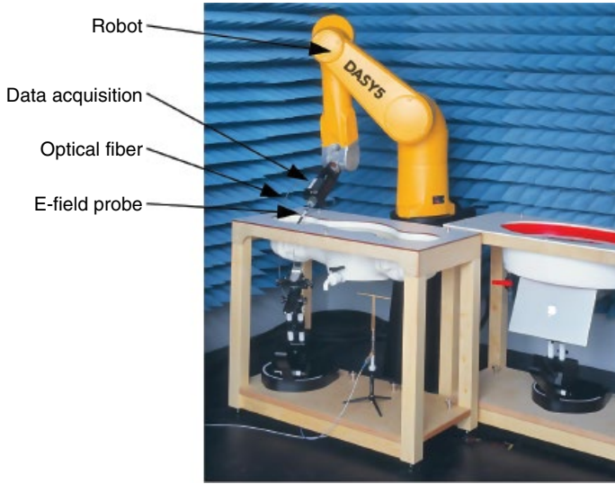
Figure 6.3 Robot and E -field probe. (Source: Reproduced with permission of Schmid & Partner Engineering AG)
