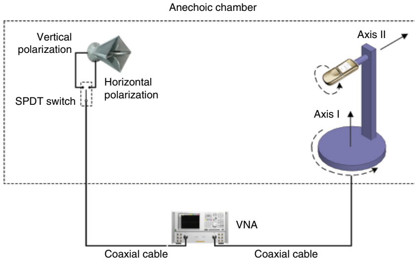
Figure 5.23 Simplified block diagram of a 3D test setup.
