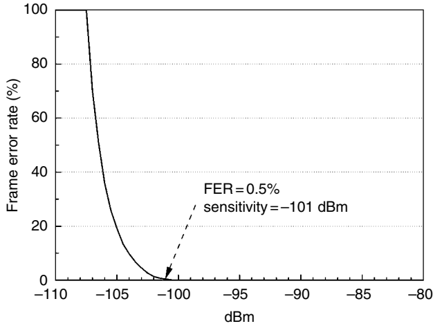
Figure 5.29 FER vs. signal power.
