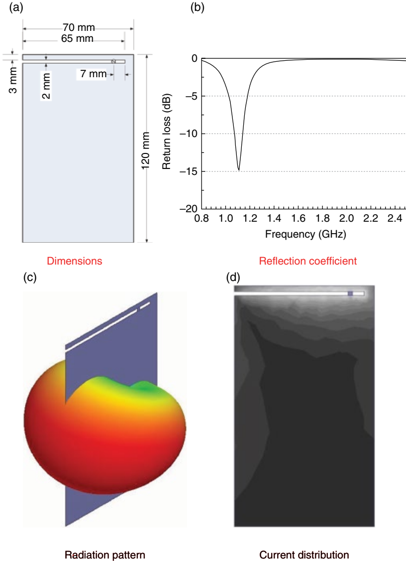
Figure 4.63 A quarter-wavelength slot on the top.
