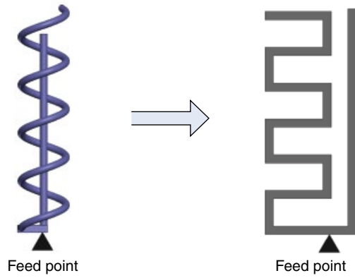
Figure 3.83 Multiple branch meander line antennas.
