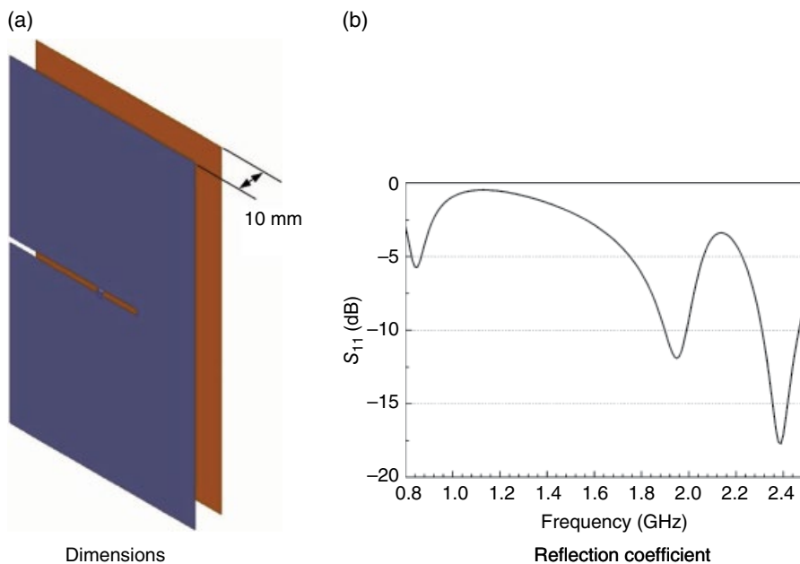
Figure 4.66 Impact of LCD screen shield.
