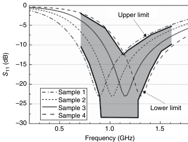
Figure 5.41 Set pass/fail region with upper and lower limits.
