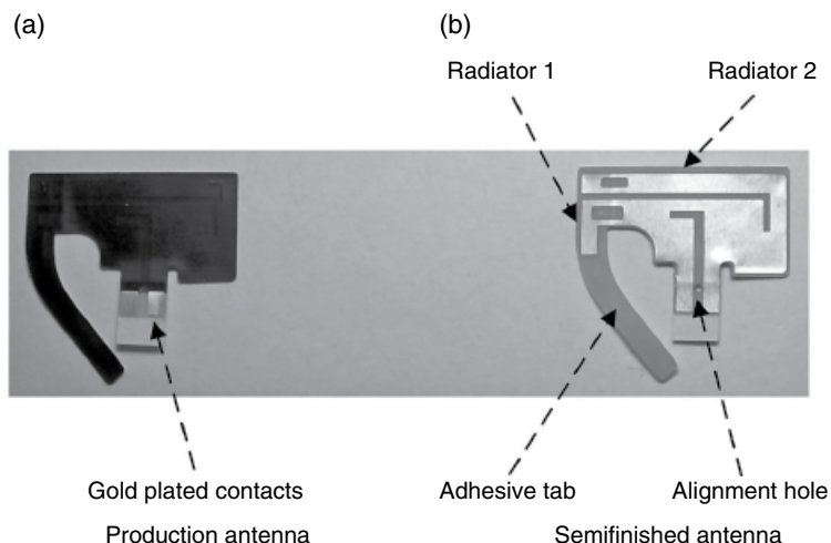
Figure 4.104 Hongmi 2A's WLAN and GPS antenna. (Source: Reproduced with permission of Xiaomi, Inc. and Shanghai Amphenol Airwave, Inc.)
