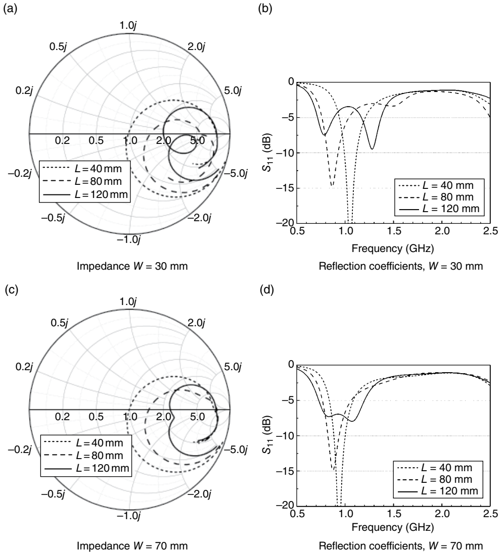
Figure 3.93 Effect of ground width and length, L_{ant} = 70 mm.
