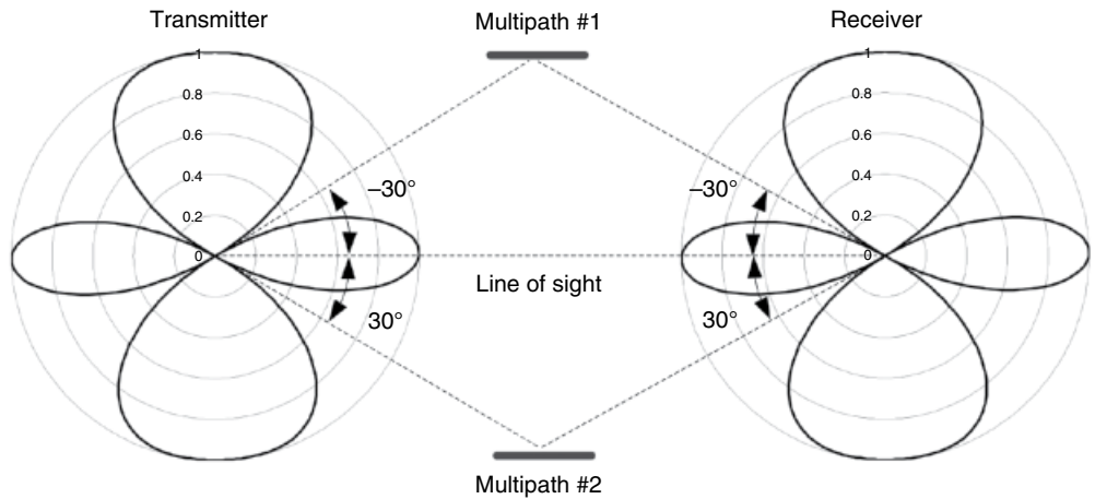
Figure 4.88 Nulled patterns corresponding to the LOS path.
