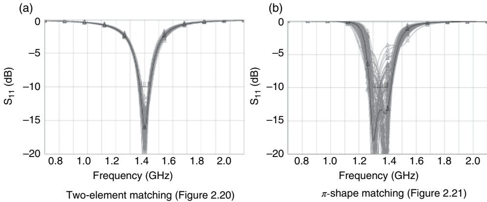
Figure 2.25 Tolerance analysis (5% of component value).
