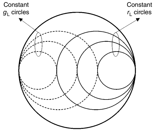
Figure 2.5 Simplified ZY Smith chart for lumped-element-only matching.
