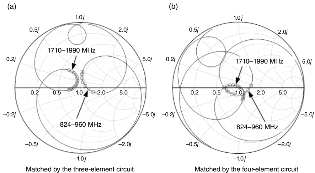
Figure 3.46 Impedance of the matched Figure 3.40a antenna.
