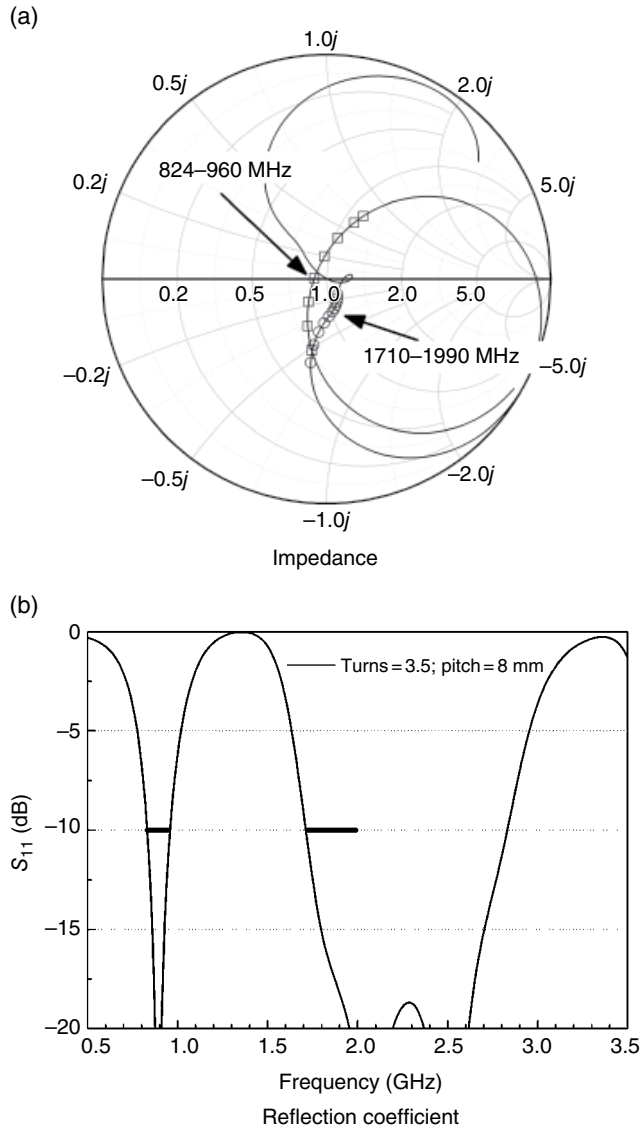
Figure 3.51 Matched helix-loaded whip antenna.
