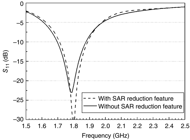
Figure 6.19 Impact of SAR reduction feature on reflection coefficient.
