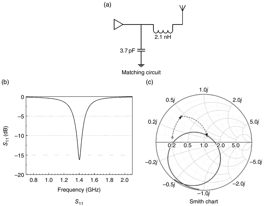
Figure 2.20 Two-element matching circuit.
