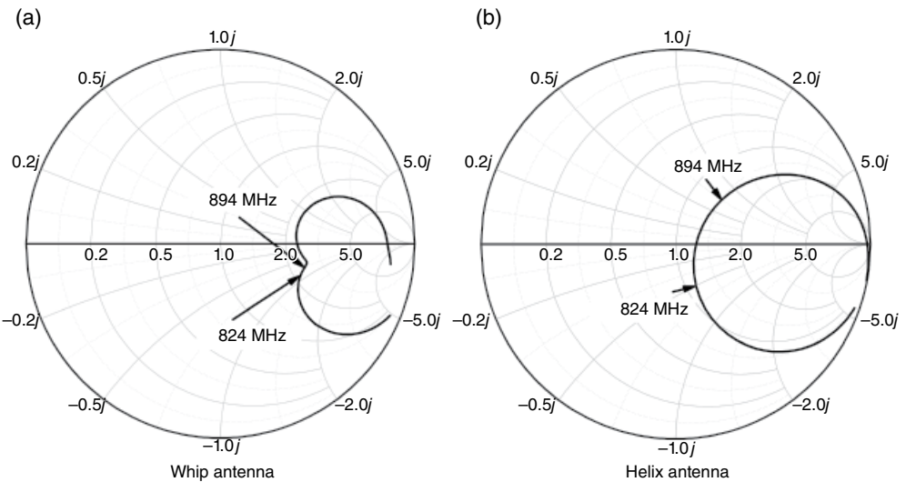
Figure 3.20 Impedances of whip and helix antennas.
