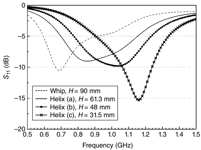
Figure 3.13 Reflection coefficients of a whip monopole and three helices, D=6 mm.
