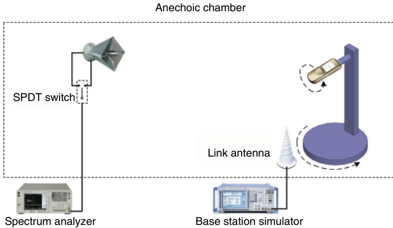
Figure 5.28 Simplified block diagram of a TRP test setup.
