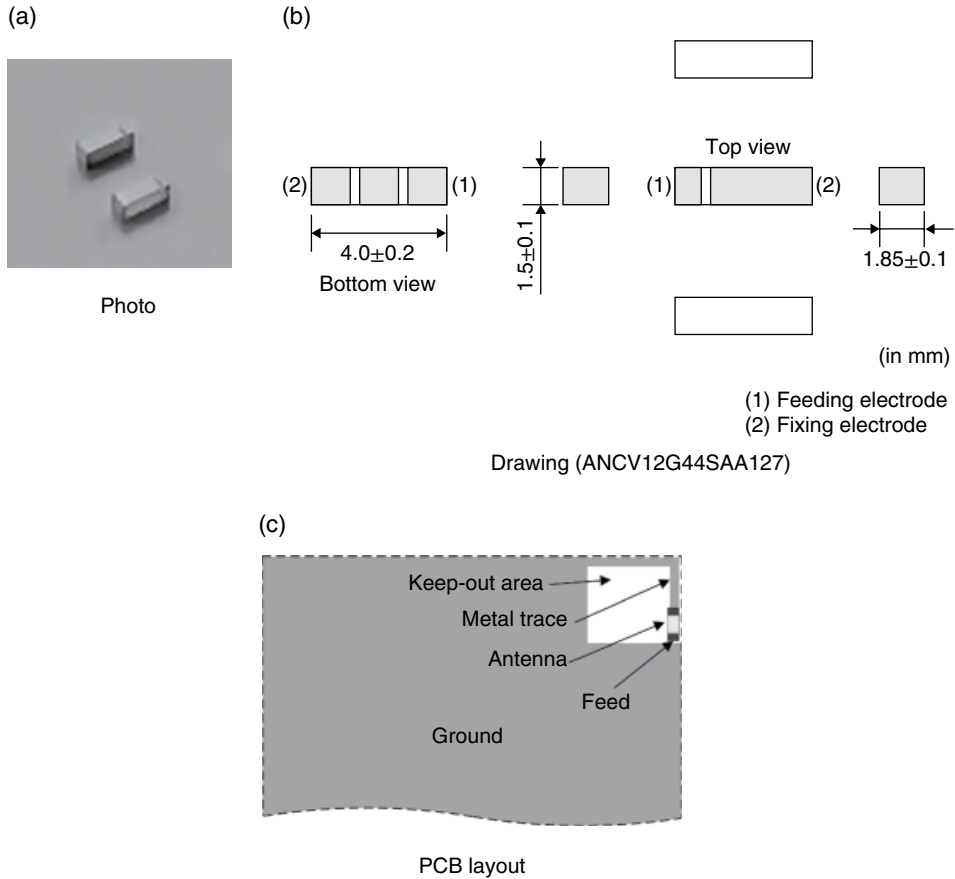
Figure 4.56 Loop ceramic WLAN antenna. (Source: Murata Manufacturing Co. Ltd.)
