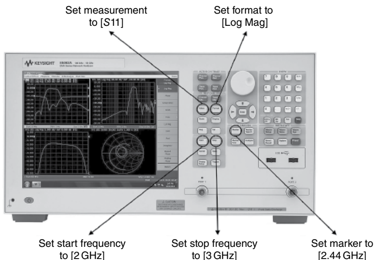
Figure 1.14 Network analyzer.
