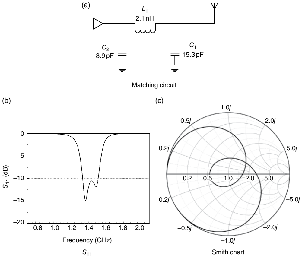
Figure 2.21 \pi -shaped matching circuit.
