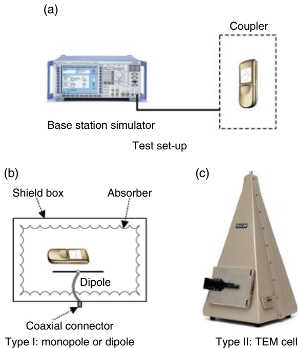
Figure 5.43 Radiating test on a production line. (Source: Reproduced with permission of TESCOM.)
