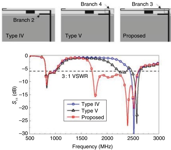
Figure 4.69 Comparison of simulated S_{11} for different antenna types. Type IV: Type III+branch 2, Type V: Type IV+branch 4, proposed: Type V+ branch 3. (Source: Deng et al. [27]. Reproduced with permission of IEEE.)
