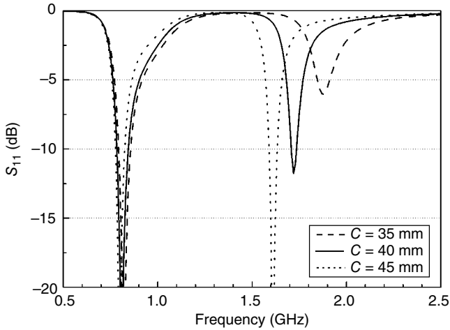
Figure 4.17 Impact of dimension C . 50\text{ mm} \times 25\text{ mm} Patch, P = 15\text{ mm} , D = 10\text{ mm} .
