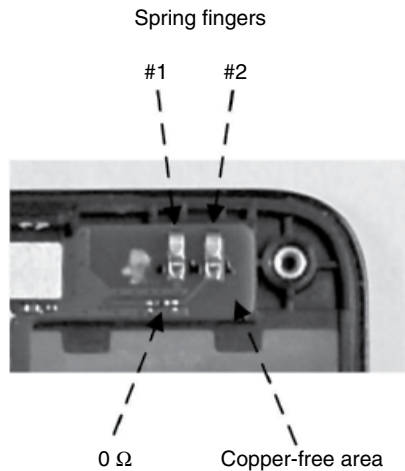
Figure 4.106 Matching circuit of the WLAN and GPS antenna. (Source: Reproduced with permission of Xiaomi, Inc.)
