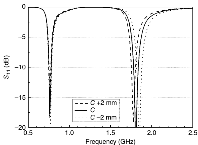
Figure 4.24 A small PIFA: slot length variations.
