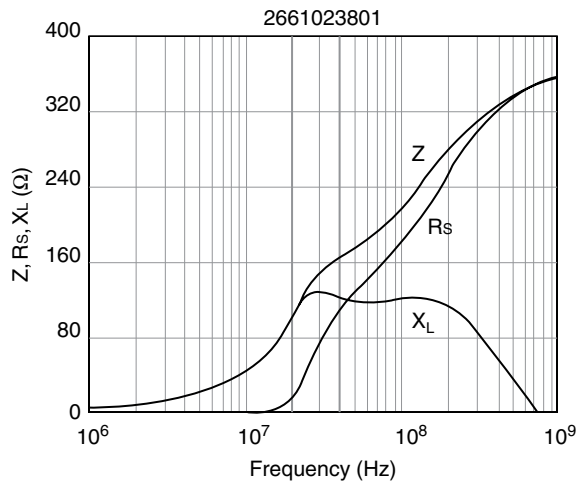
Figure 5.14 Impedance, reactance, and resistance vs. frequency (EMI Core 2661023801). (Source: Fair-Rite Products, Corp.)
