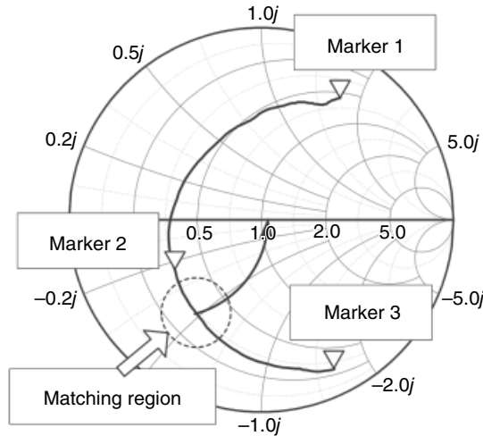
Figure 2.31 Impedance curve of the original antenna.
