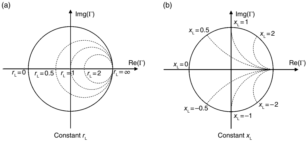
Figure 2.2 Family of curves of constant r_L and x_L .
