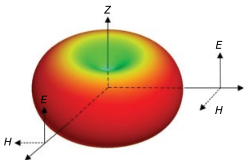
Dipole antenna
