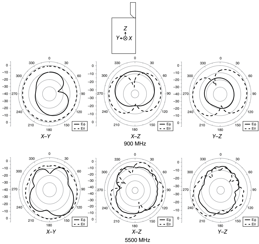
Figure 3.71 Measured antenna patterns. (Source: Zhang et al. [24]. Reproduced with permission of IEEE.)
