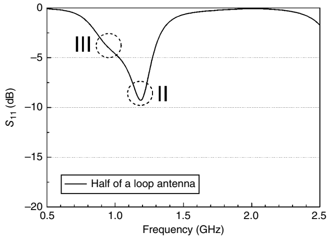
Figure 4.49 Reflection coefficient of a bottom-installed monopole antenna.
