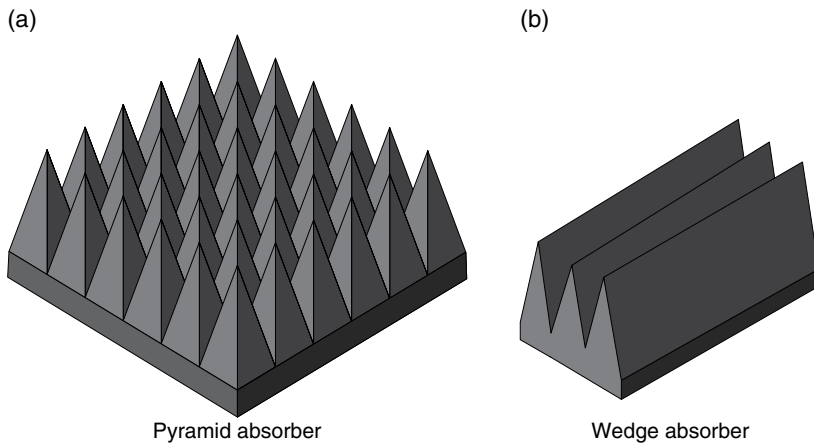
Figure 5.20 Radiation absorbent material. (Source: Reproduced with permission of Microwave Vision.)
