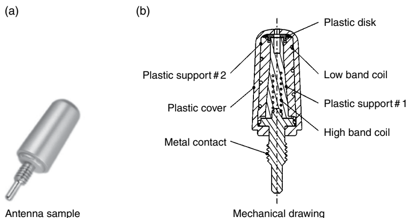
Figure 3.37 Dual-coil helix antenna. (Source: Reproduced with permission of Shanghai Amphenol Airwave.)
