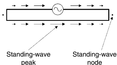
Figure 4.45 Current distribution of a one-wavelength stand-alone loop antenna.
