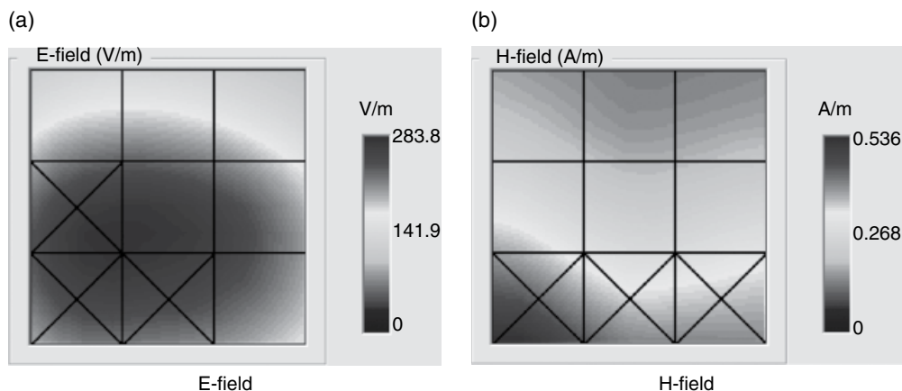
Figure 6.26 Measurement result of a sample phone (at CDMA 850, Channel 384).
