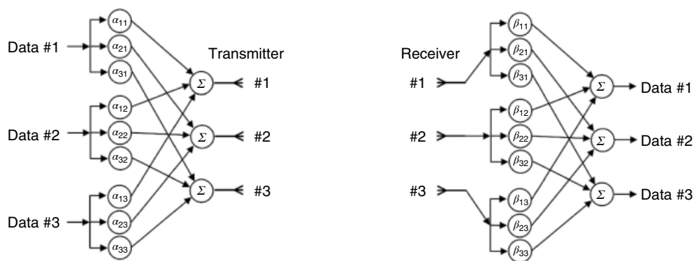
Figure 4.89 Explain MIMO system through the view of phased array.
