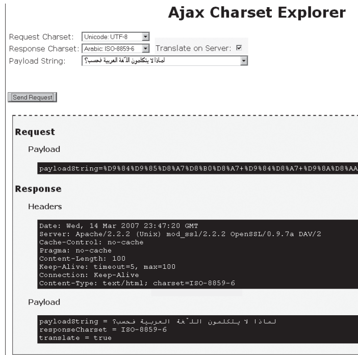
FIGURE 4-2 Character sets working correctly
