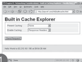
FIGURE 6-20 Caching and Ajax can coexist
