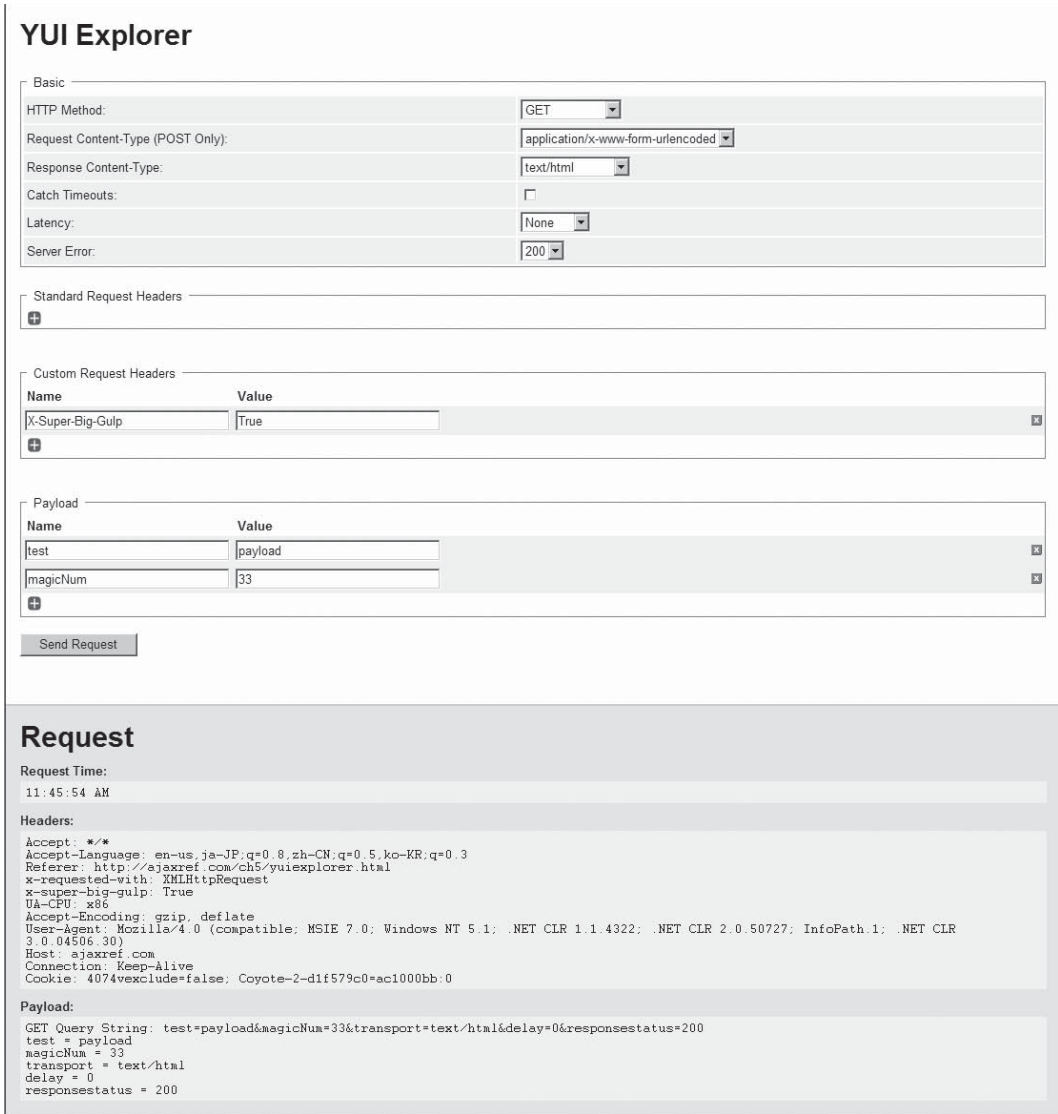
FIGURE 5-2 YUI version of Ajax request explorer
