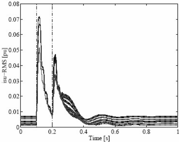
Figure 14. Subterranean lines currents (three-phase fault)
