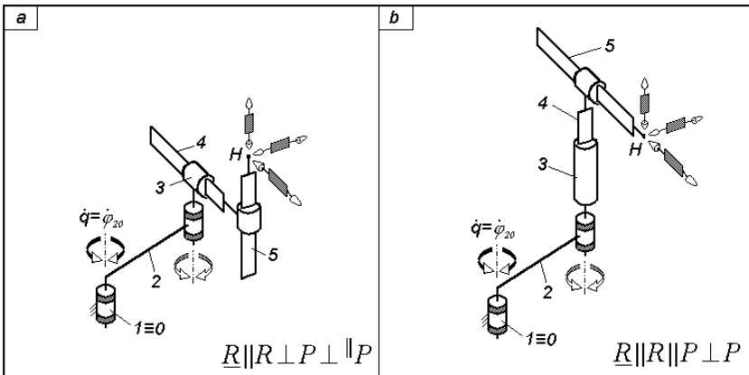
Figure 5. Elementary legs without idle mobilities ( M_A = S_{nA/1}^A = 4 )
