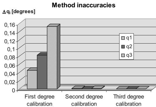
Figure 5. The inaccuracies of the calibration models.
