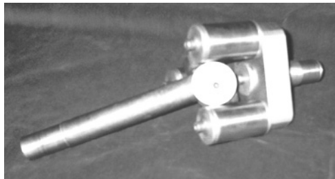
Figure 9. Cylinder/cylinder contacts
