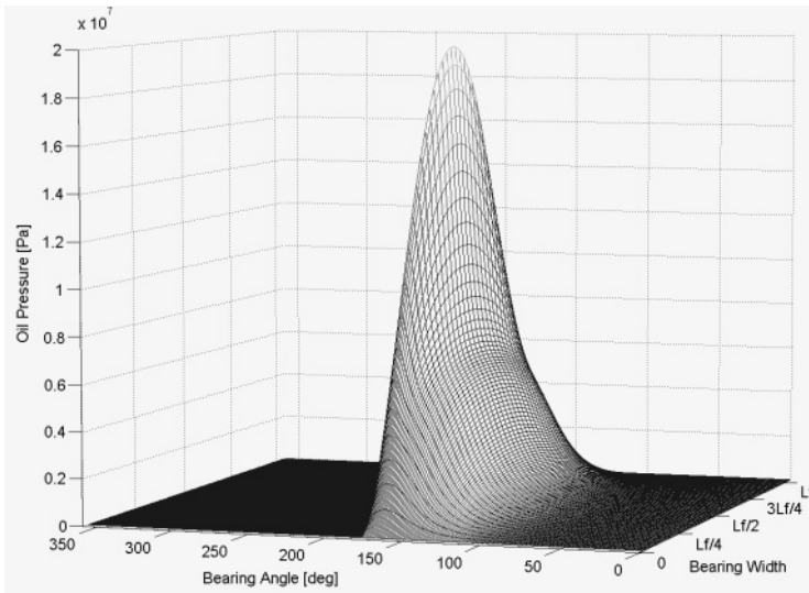
Figure 15. Pressure at 320 deg and 3000 rpm
