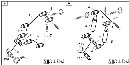
Figure 15. Complex legs with trimobile planar loops without idle mobilities ( M_A = S_{nA/1}^A = 5 )
