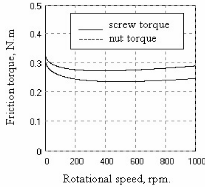
Figure 5. Total friction torque acting on the screw and on the nut
