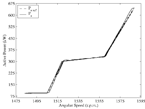
Figure 19. \omega_m versus P_s curve
