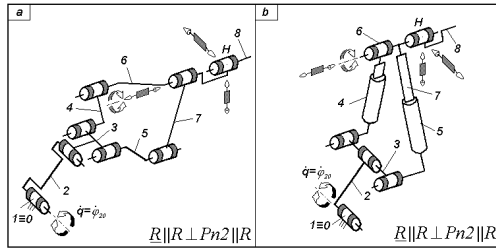
Figure 13. Complex legs with bimobile planar loops without idle mobilities ( M_A = S_{nA/1}^A = 5 )
