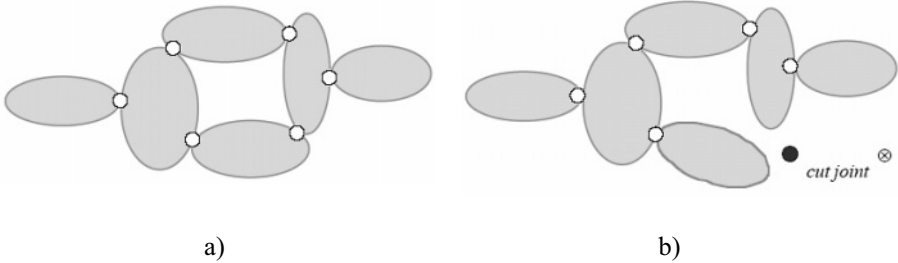
Figure 21. A closed-chain system and its reduced open-chain system.
