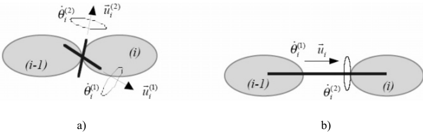
Figure 17. Joint velocities: a) universal; and b) cylindrical.
