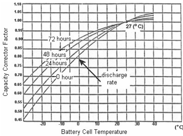
Figure 18. Capacity correction factor of a Pb battery versus battery cell temperature (°C) and the discharge rate.
