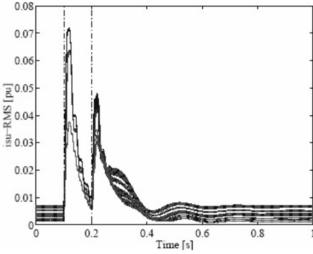
Figure 13. Subterranean lines currents (two-phase fault)
