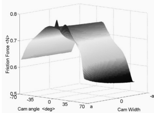
Figure 11. Cam-tappet friction force at 1200 rpm (engine speed)
