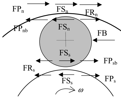
Figure 2. The forces acting on the ball and on the two races in a ball-screw system
