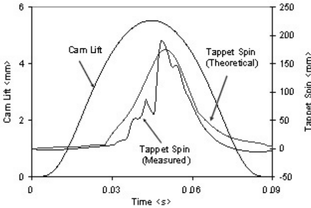
Figure 12. Tappet spin
