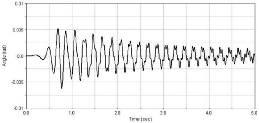
Figure 6. Angular deformation of torsion spring
