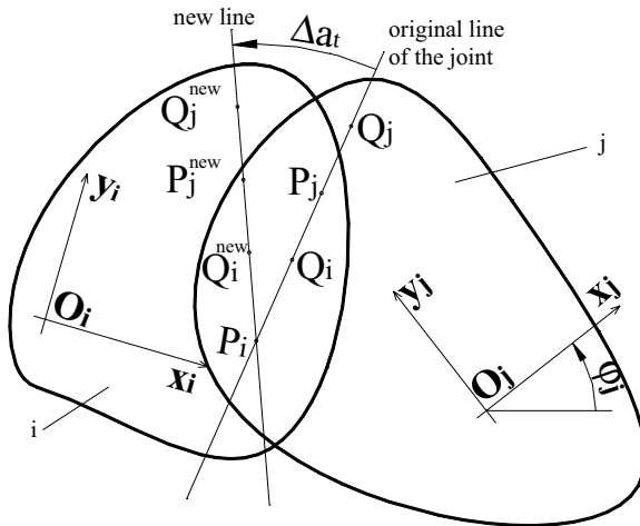
Figure 2. Modification of a translational joint
