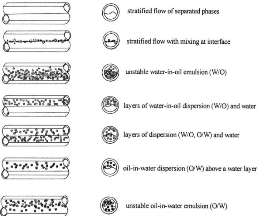
Figure 2. Oil-water mixture flow systems representation (according Nadler and Mewes): stratified flow of the two phases, stratified flow with two-interface mixture, unstable water in oil emulsion flow type, stratified water flow and emulsion of water in oil, stratified water flow, emulsion of oil in water and emulsion of water in oil, stratified water flow and oil in water emulsion, unstable oil in water emulsion type flow.
