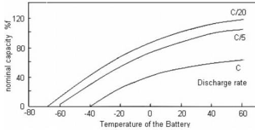
Figure 17. Impact of temperature and of discharge rate to the energy delivered (the case of a PV-acid battery).
