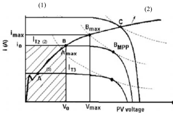
Figure 1. The characteristic I, V of a PV system (1) and the characteristic I, V of a motor (2).
