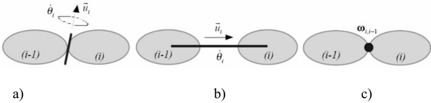
Figure 16. Joint velocities: a) revolute; b) prismatic; and c) spherical.
