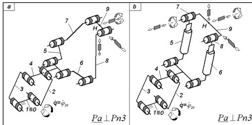
Figure 14. Complex legs with trimobile planar loops without idle mobilities ( M_A = S_{nA/1}^A = 4 )
