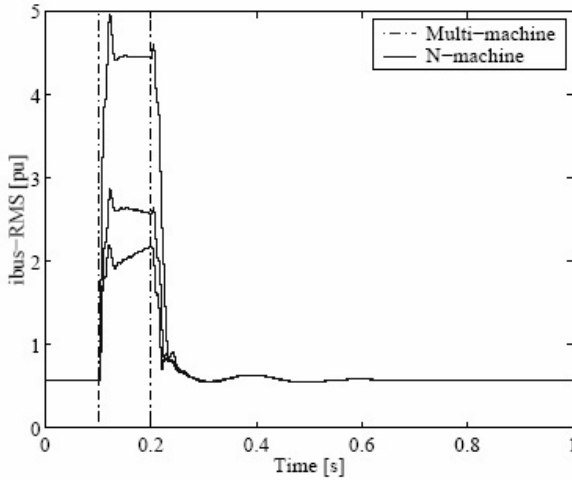
Figure 7. Currents in the infinite busbar (single-phase fault)
