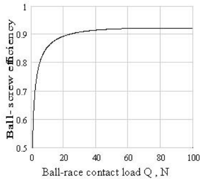
Figure 9. Variation of the ball screw efficiency with ball-race contact load
