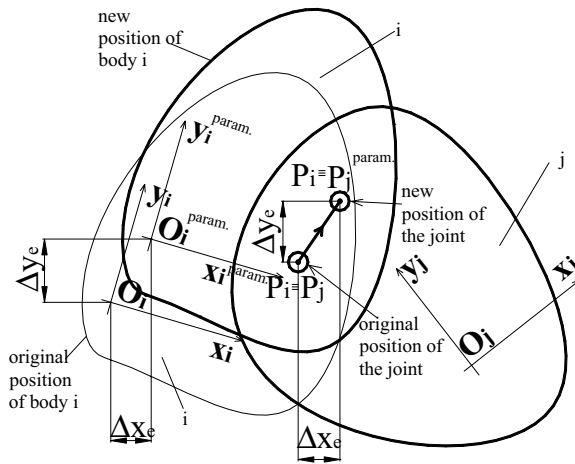
Figure 3. Modification of a body's position
