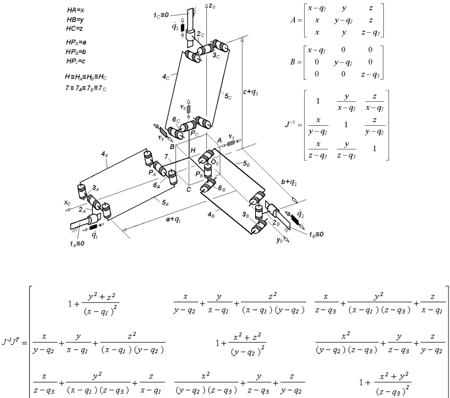
Figure 1. Orthoglide - a TPM-CM (3- PRPaR ) with three coupled motions
