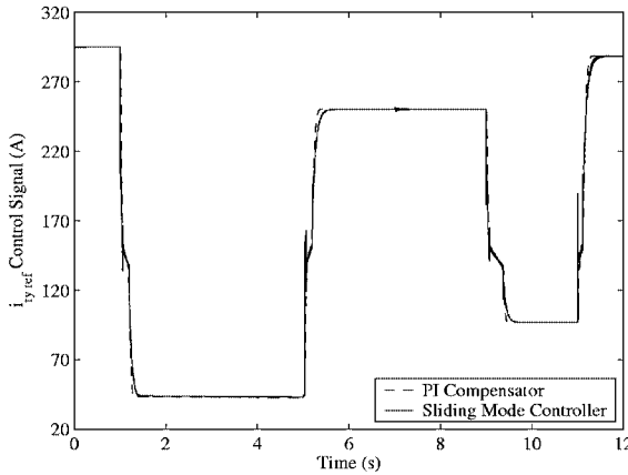
Figure 20. i_{ry \text{ ref}} control signal in both tests
