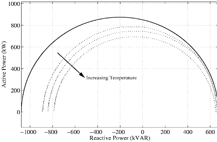
Figure 3. P/Q curves for the generator + inverter
