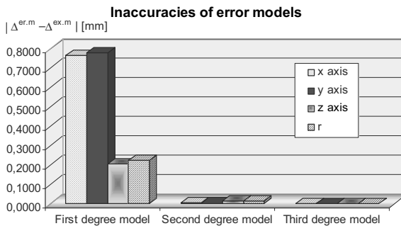
Figure 4. The inaccuracies of error models ( \Delta^{er.m} —errors established with error models, \Delta^{ex.m} —errors established with exact models).
