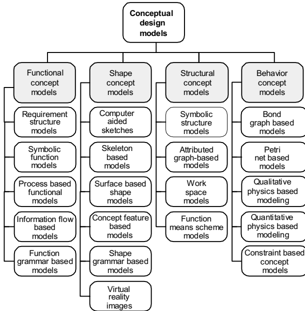
Figure 1. Taxonomy of virtual conceptual models
