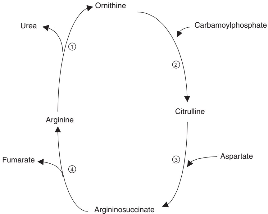
Fig. 4.2. The urea cycle. Key to enzymes: 1, arginase; 2, ornithine transcarbamoylase; 3, argininosuccinate synthetase; 4, argininosuccinase.
