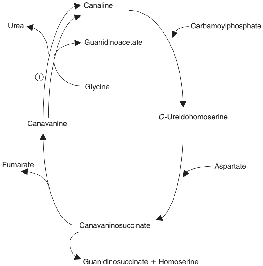
Fig. 4.4. Mammalian metabolism of canavanine. Enzymes: analogous to those involved in the urea cycle; thus 1, arginase. (Adapted from D'Mello, 1991.)
