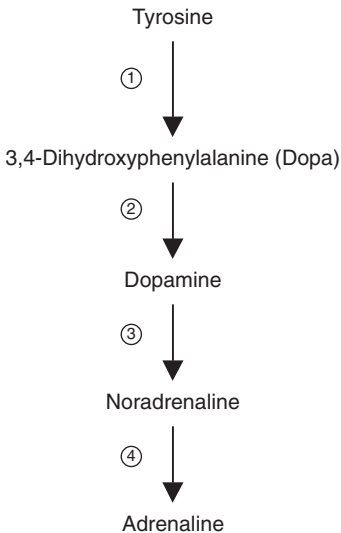
Fig. 4.10. Synthesis of noradrenaline and adrenaline from tyrosine. Enzymes: 1, tyrosine hydroxylase; 2, aromatic decarboxylase; 3, dopamine- \beta -hydroxylase; 4, transmethylease.
