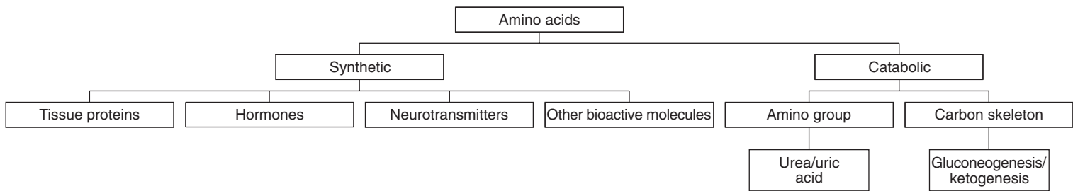
Fig. 4.1. Overview of pathways in amino acid metabolism in animals.
