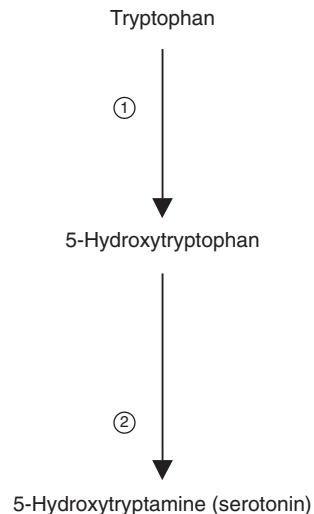
Fig. 4.11. Synthesis of 5-hydroxytryptamine from tryptophan. Enzymes: 1, tryptophan 5-monoxygenase; 2, 5-hydroxytryptophan decarboxylase.
