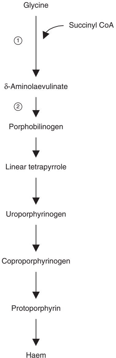
Fig. 4.9. Biosynthesis of haem from glycine. Enzymes: 1, \delta -aminolaevulinate synthetase; 2, \delta -aminolaevulinate dehydrase.
