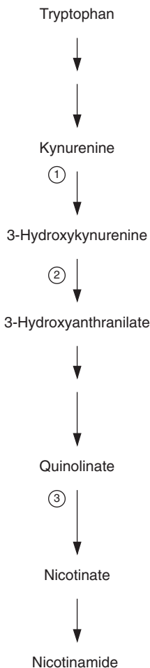
Fig 4.12. Biosynthesis of nicotinamide from tryptophan. Enzymes: 1, kynurenine 3-oxygenase; 2, kynureninase; 3, quinolinolate transphosphoribosylase.
