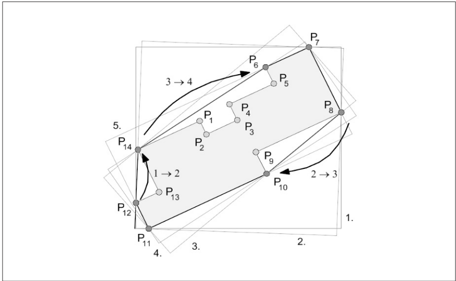
Fig. 8.4. A construction of the smallest area enclosing rectangle using rotating calipers (phases are numbered). Changes of the point V_j to its successor V_j are marked with arrows.
