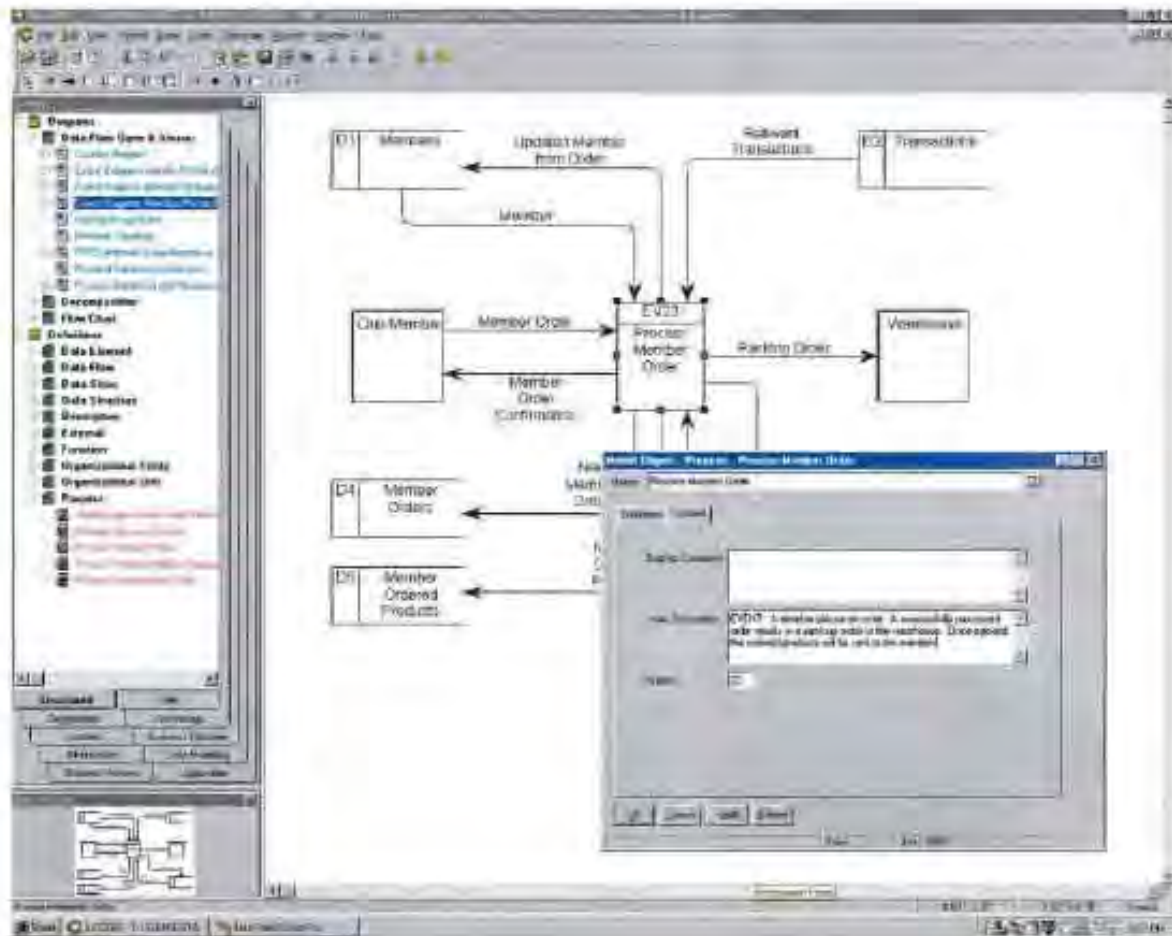
FIGURE 9-14 CASE for Process Modeling (using System Architect 2001 by Popkin Software & Systems)
