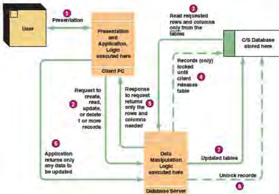
FIGURE 13-8 Client/Server System: Distributed Data (Two Tiers)
