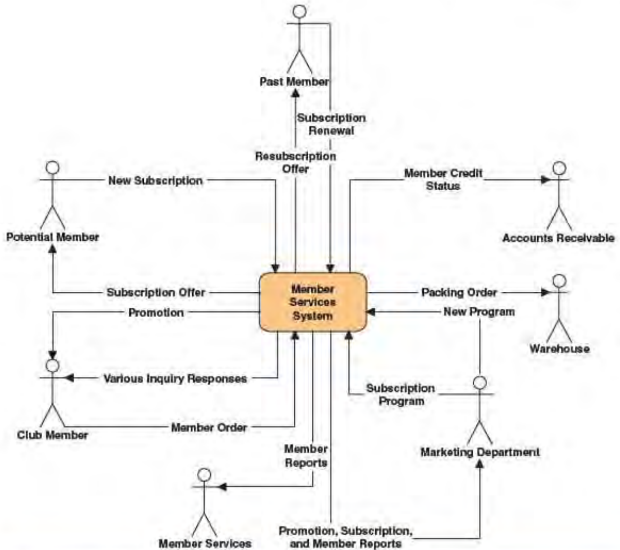
FIGURE 5-11 Context Diagram
