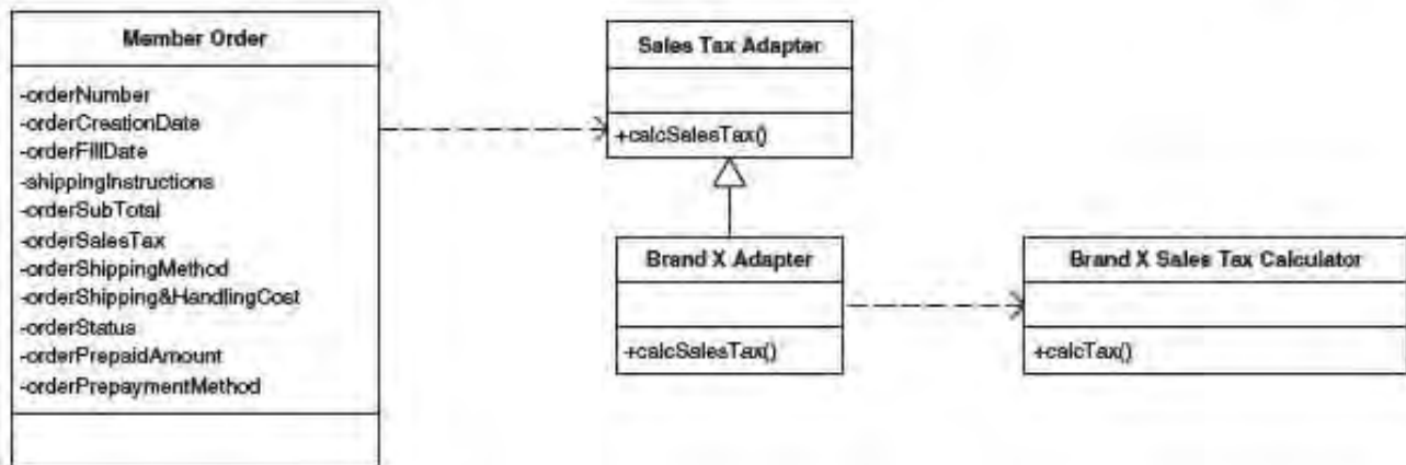
FIGURE 18-21 Adapter Pattern
