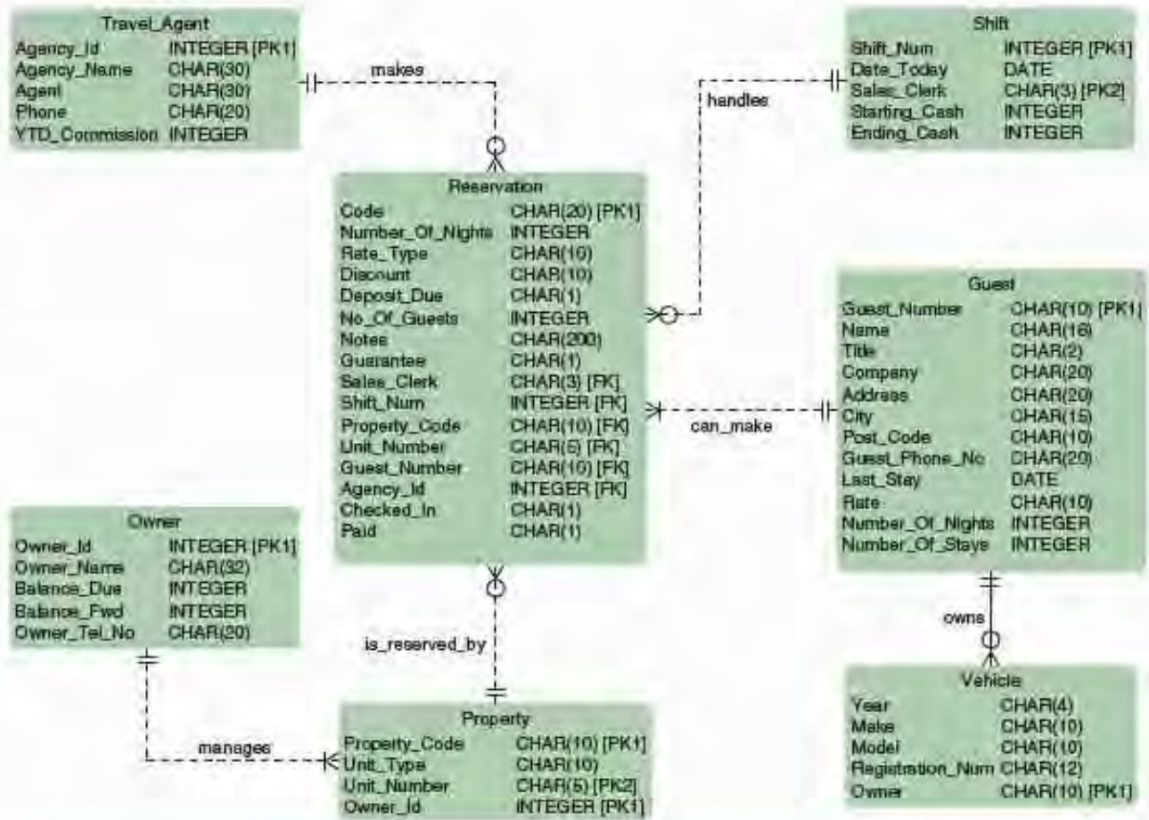
FIGURE 12-2 Sample Information Engineering Physical Entity Relationship Diagram
