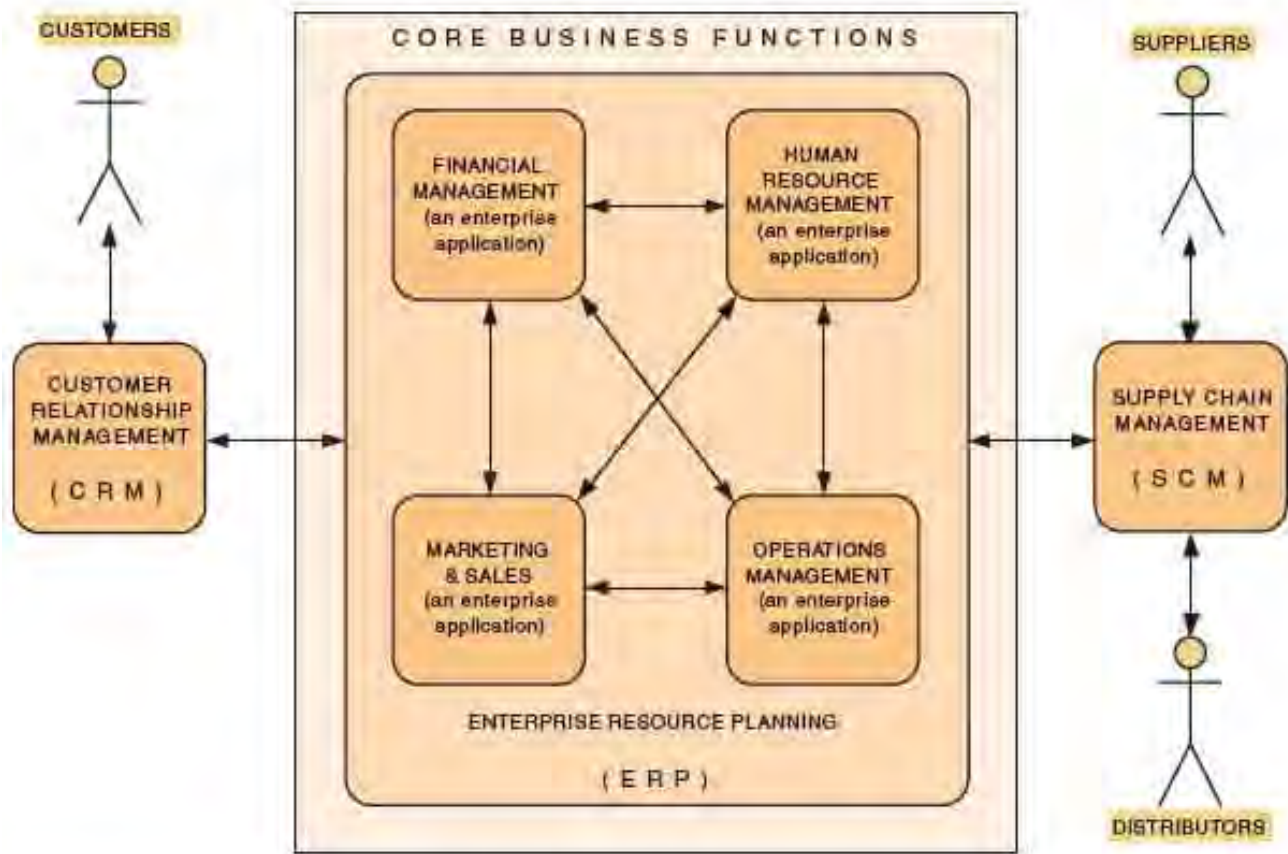
FIGURE 1-9 Enterprise Applications
