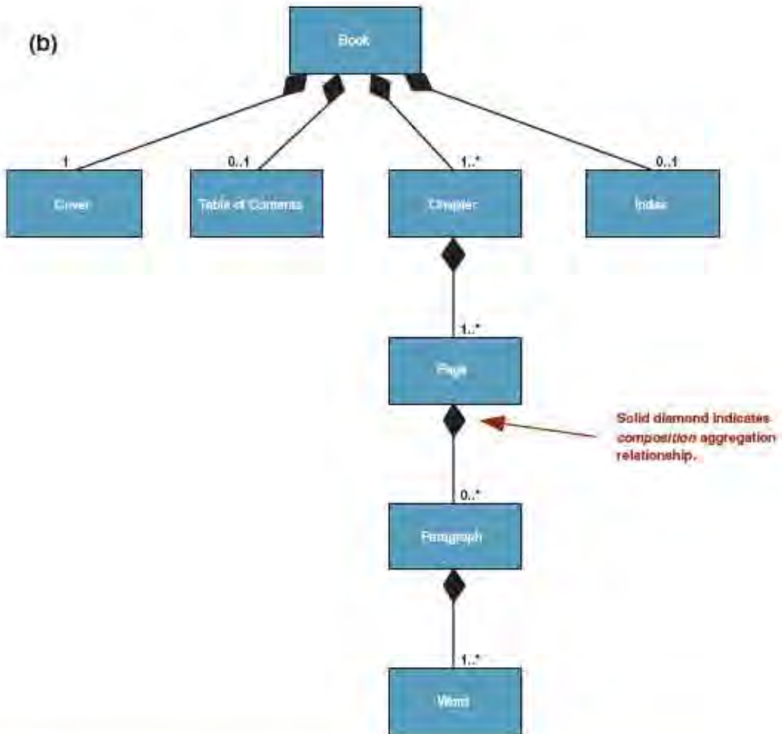
FIGURE 10-6 Aggregation Relationships
