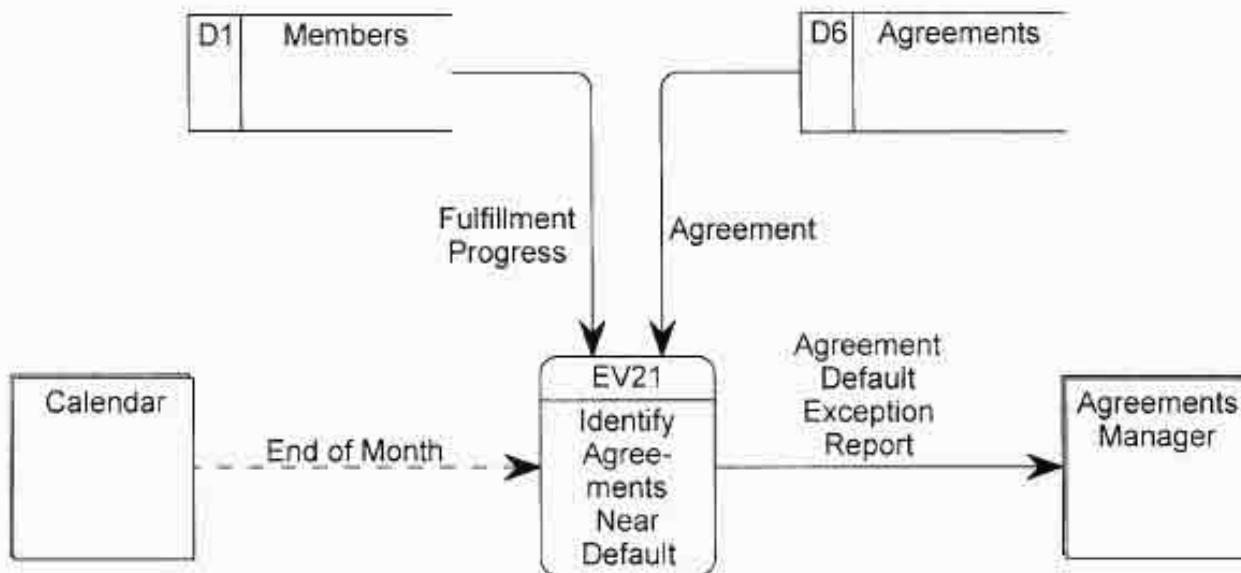
FIGURE 9-21 A Temporal Event Diagram (created with System Architect 2001 )
