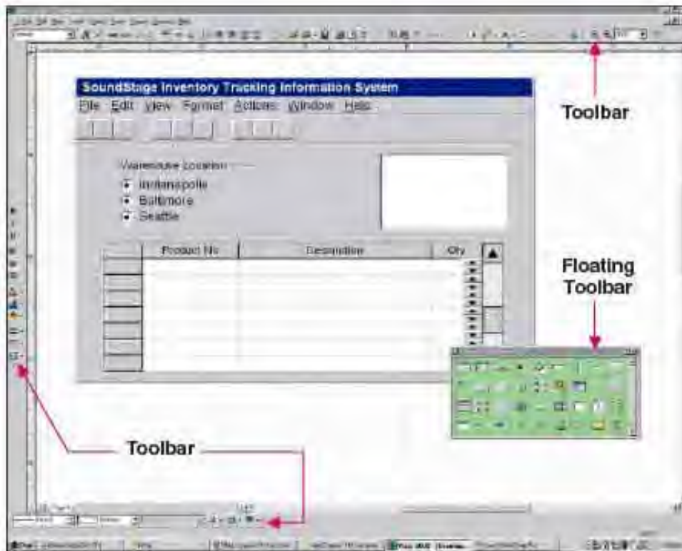
FIGURE 17-5 Toolbars
