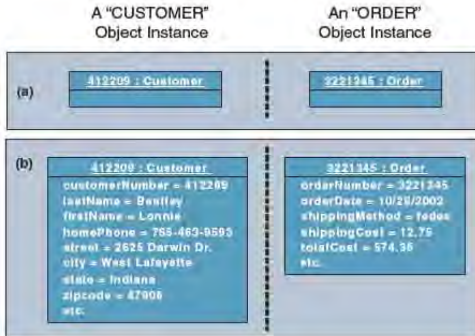
FIGURE 10-1 Object Instances
