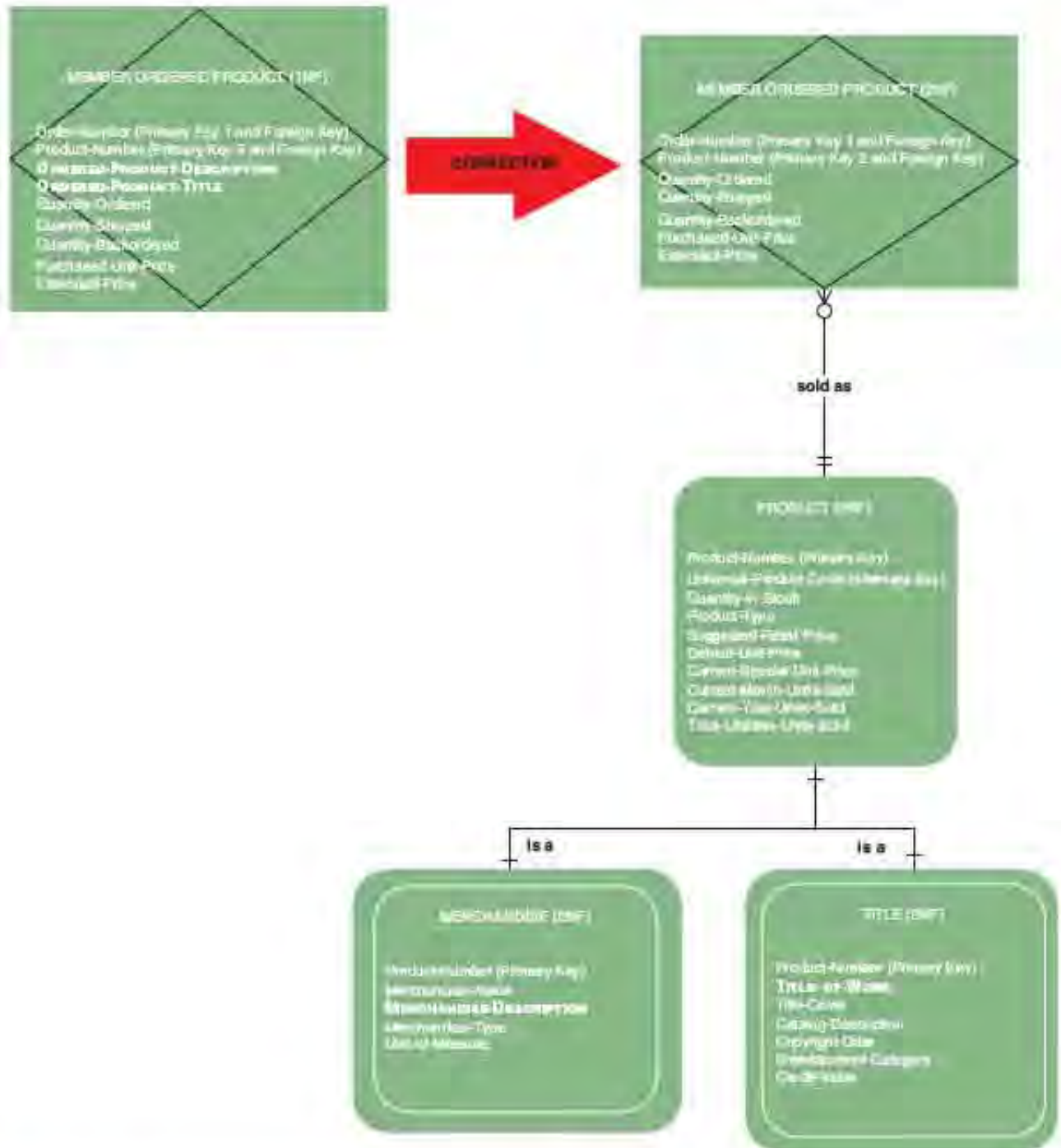
FIGURE 8-19 Second Normal Form (2NF)
