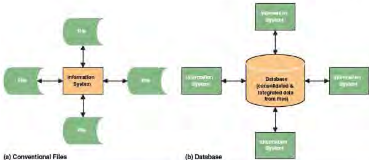
FIGURE 14-1 Conventional Files versus the Database
