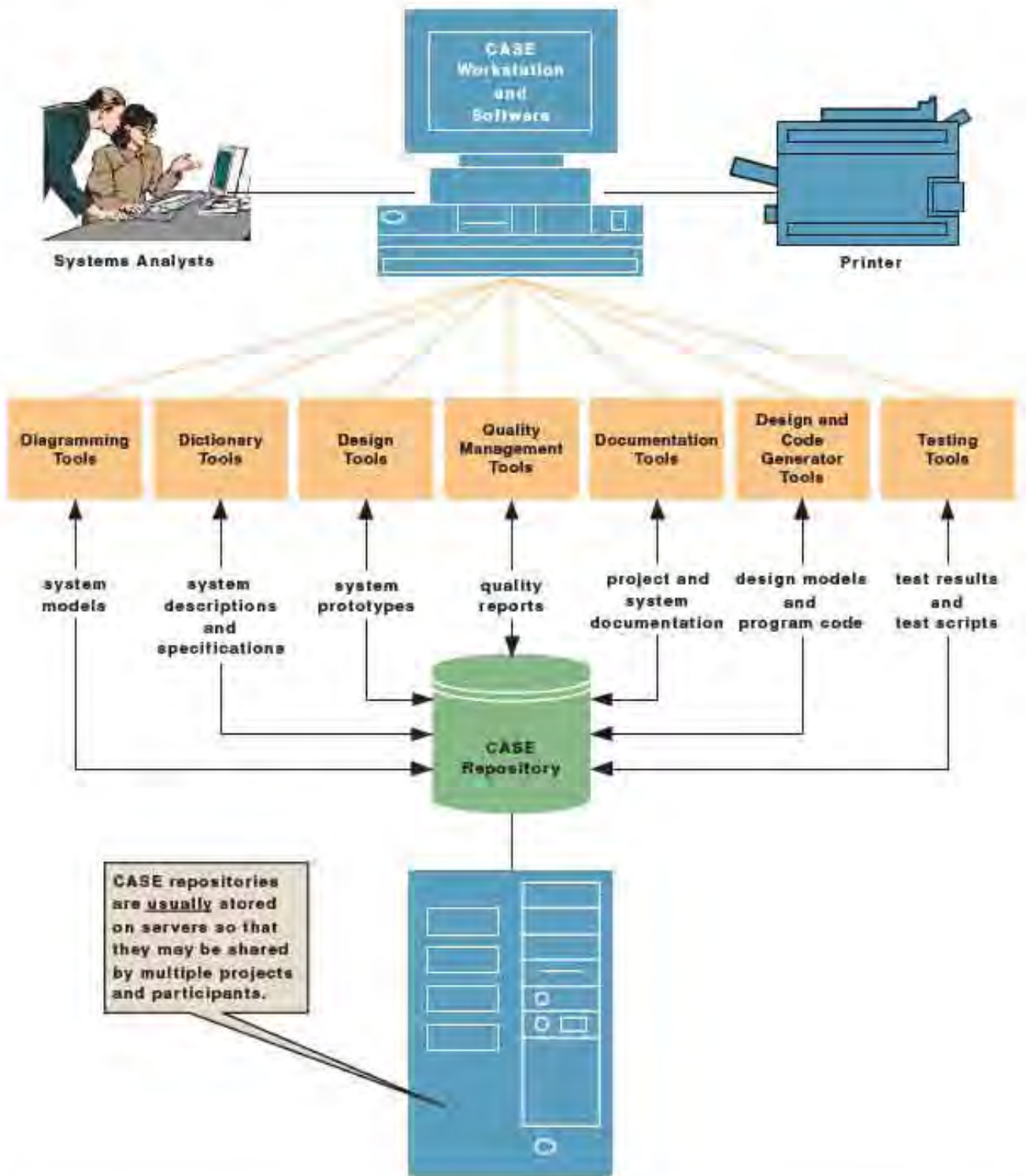
FIGURE 3-16 CASE Tool Architecture
