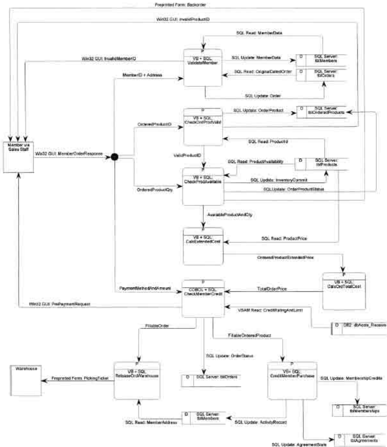
FIGURE 13-13 A Physical DFD for an Event
