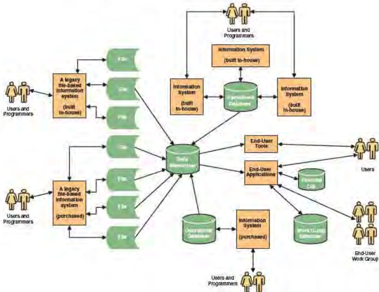
FIGURE 14-2 A Typical, Modern Data Architecture
