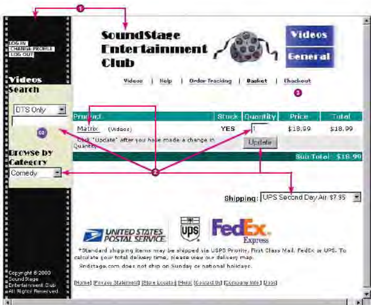
FIGURE 16-12 Input Prototype for Web Shopping Cart
