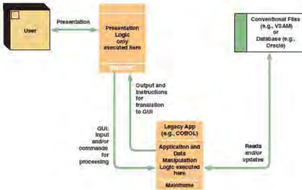
FIGURE 13-7 Client/Server System: Distributed Presentation
