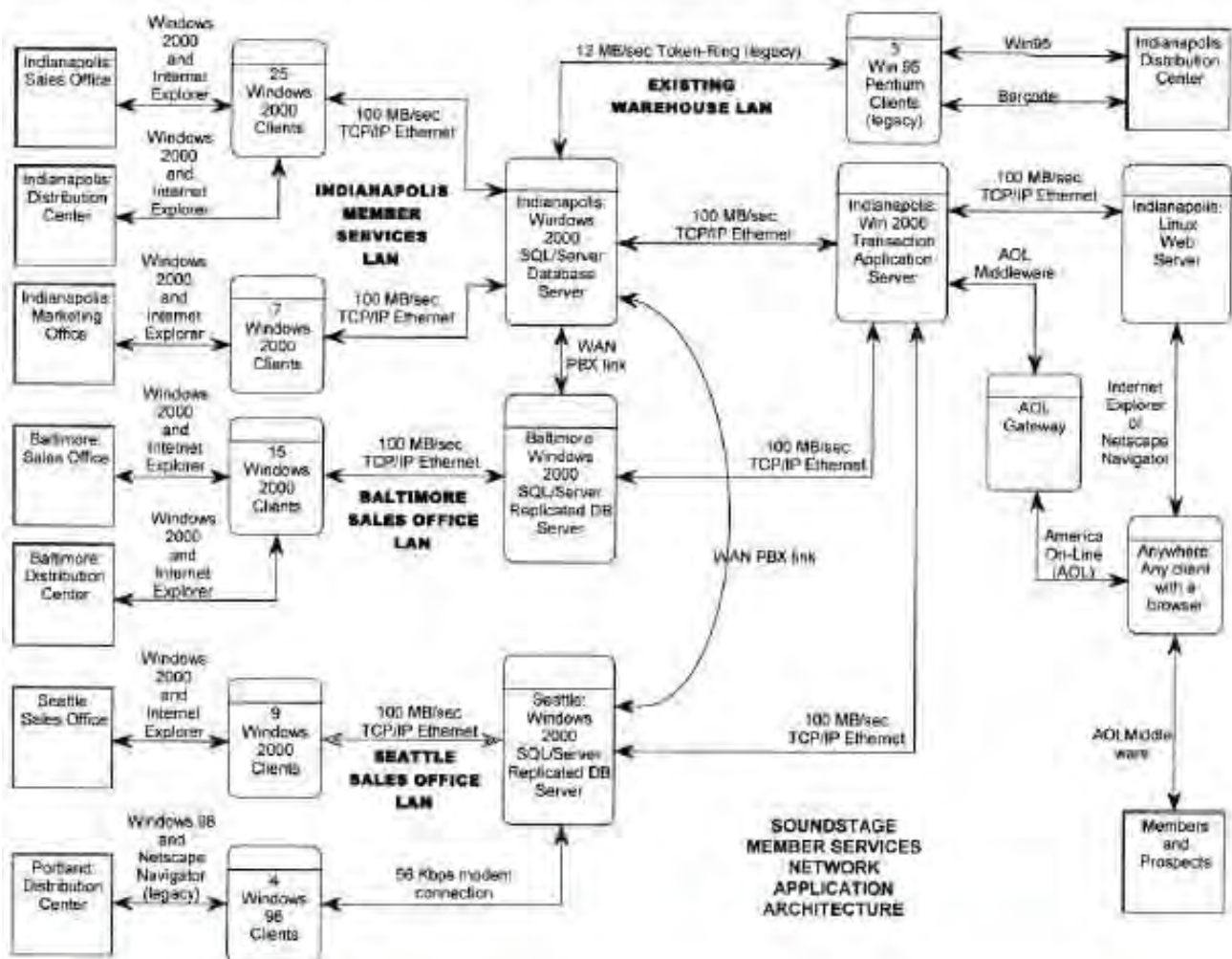
FIGURE 13-11 Network Architecture DFD
