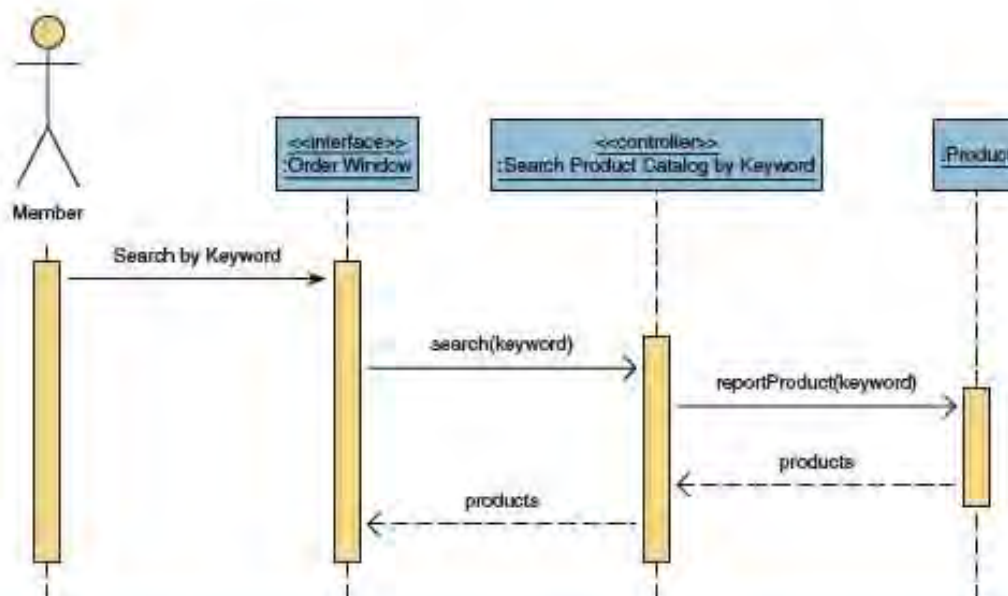
FIGURE 18-13 Sequence Diagram for Search Product Catalog by Keyword Use Case
