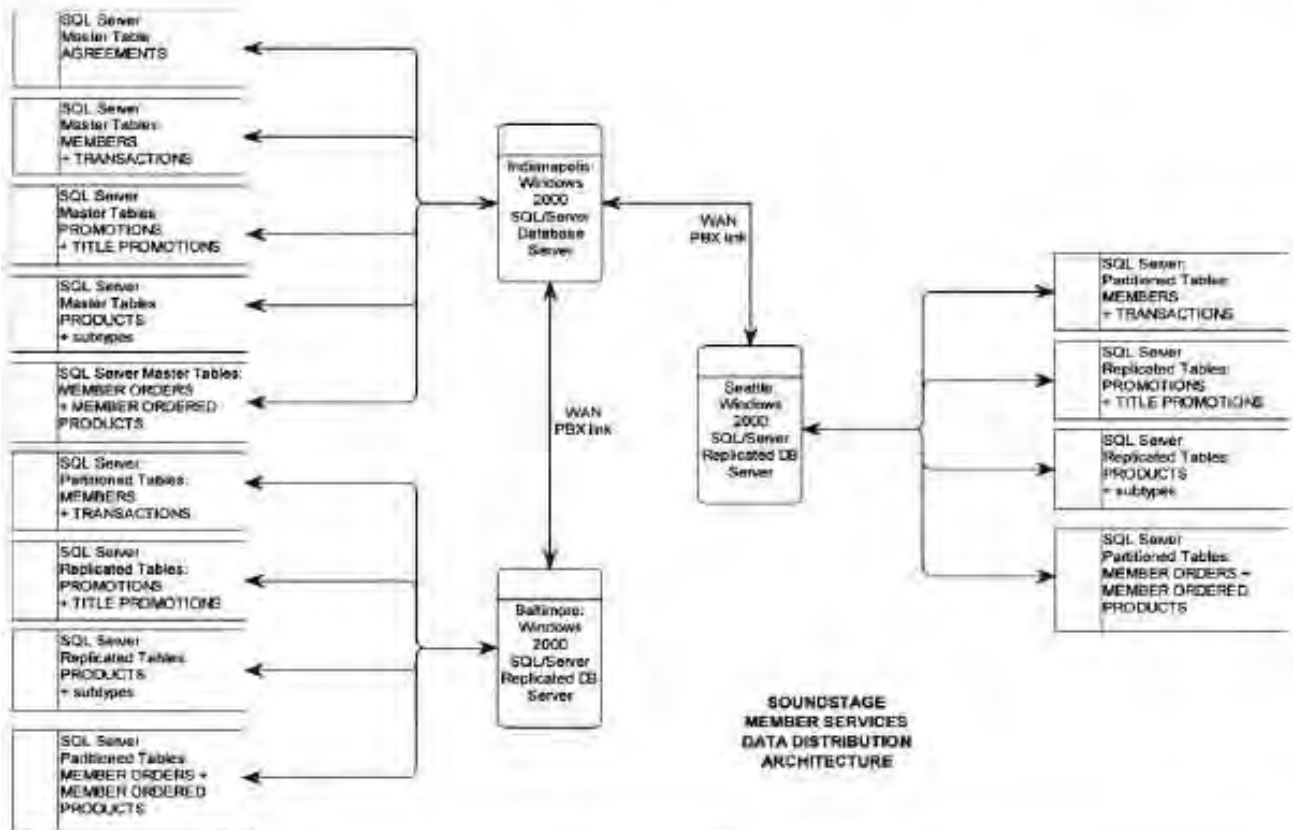
FIGURE 13-12 Data Distribution and Technology Assignments for SoundStage
