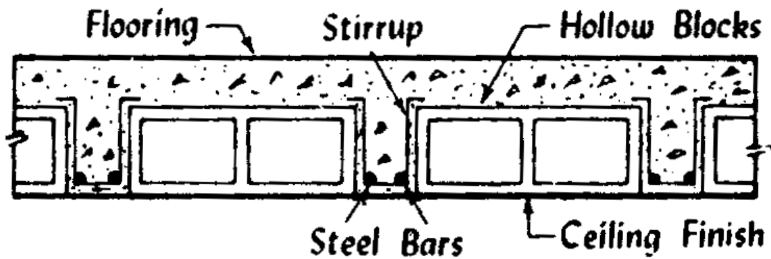
Fig 12.10 Hallow Block and Rib floor
