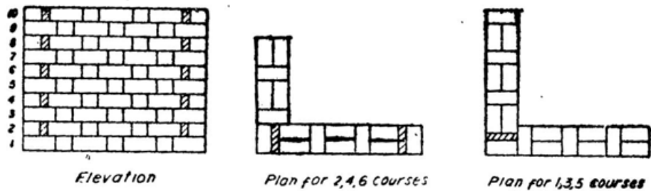
One-brick wall double flemish bond.
