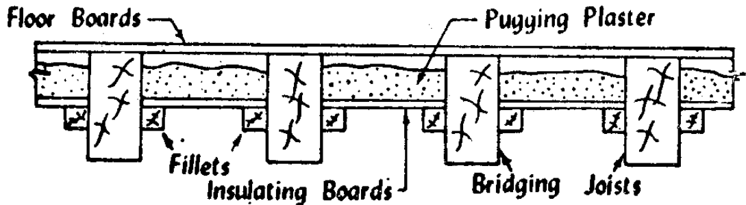
Fig 12.1 Pugging
