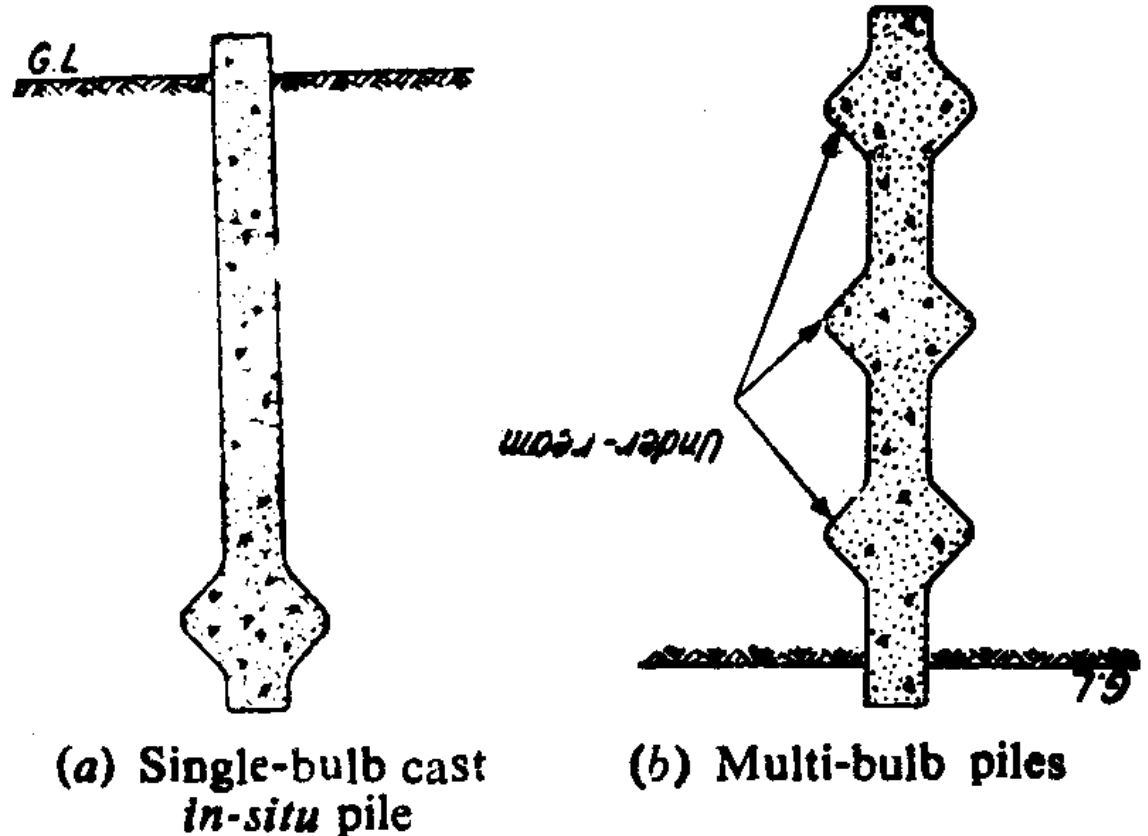
Fig 10.14 Under-reamed Piles
