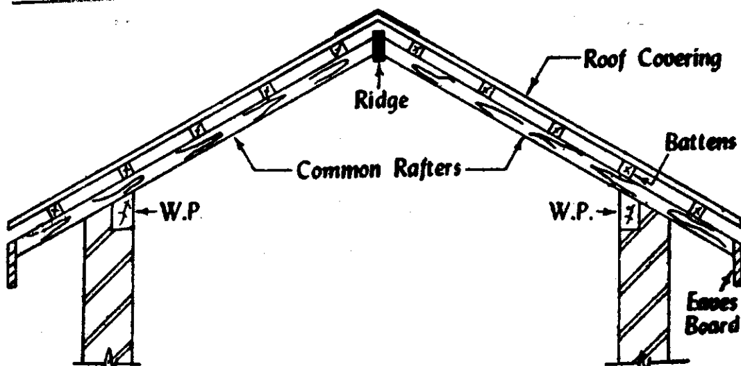
Fig 13.4 Couple roof
