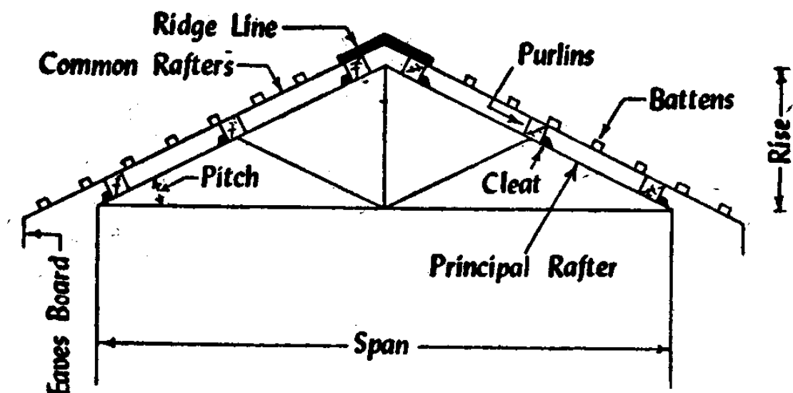
Fig 13.2 Truss
