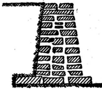
Fig 11.10 Dry Rubble Masonry
