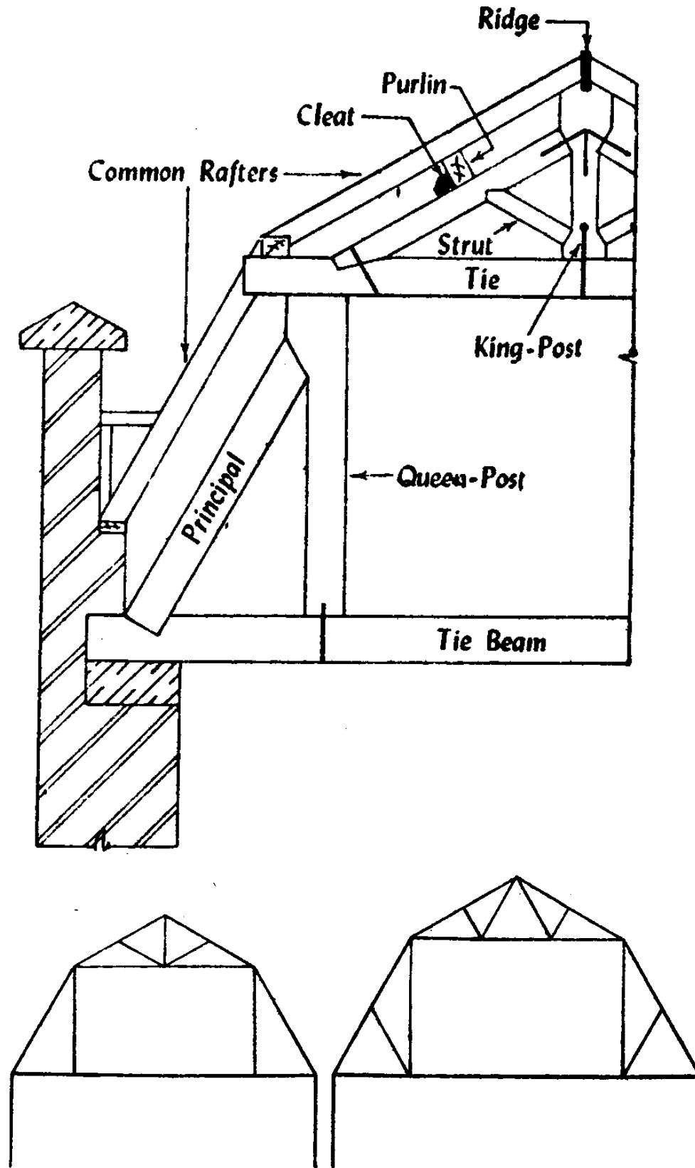
Fig 13.10 Mansard truss
