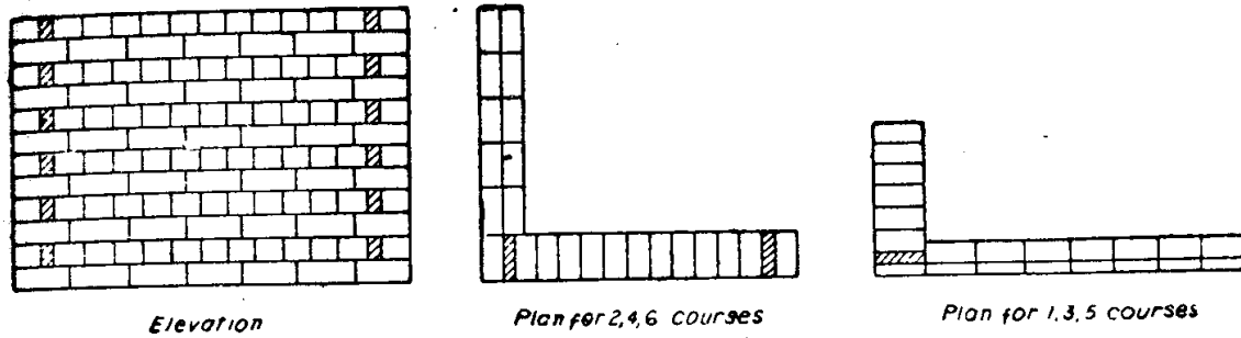
One-brick wall English bond
