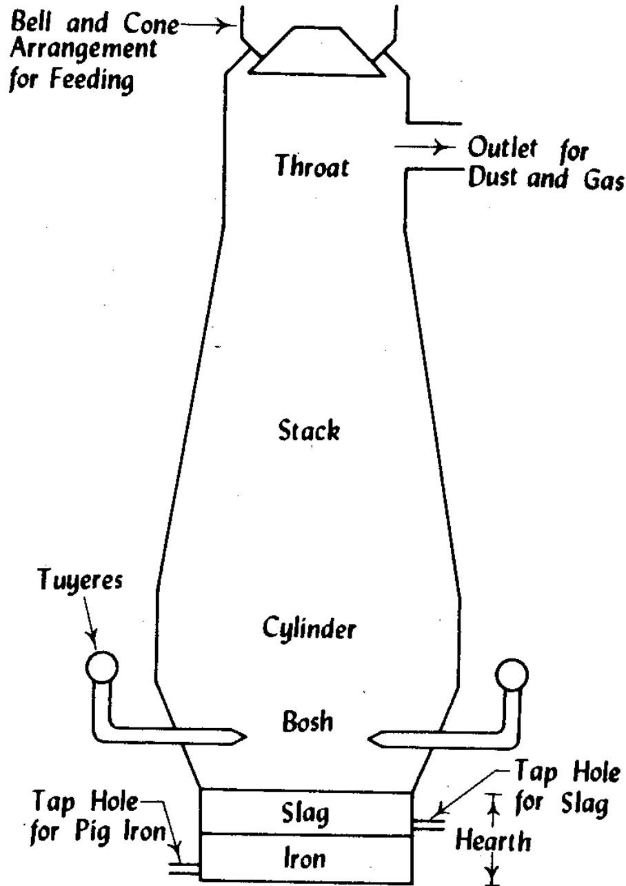
Fig 8.1 Blast Furnace
