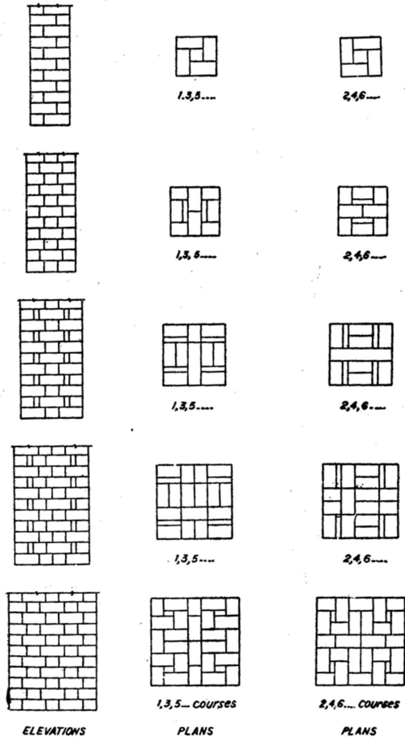
Fig 11.27 Columns in Double Flemish bond
