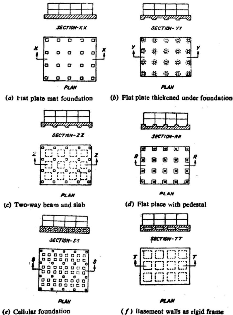
Fig 10.10 Different types of Raft Foundations
