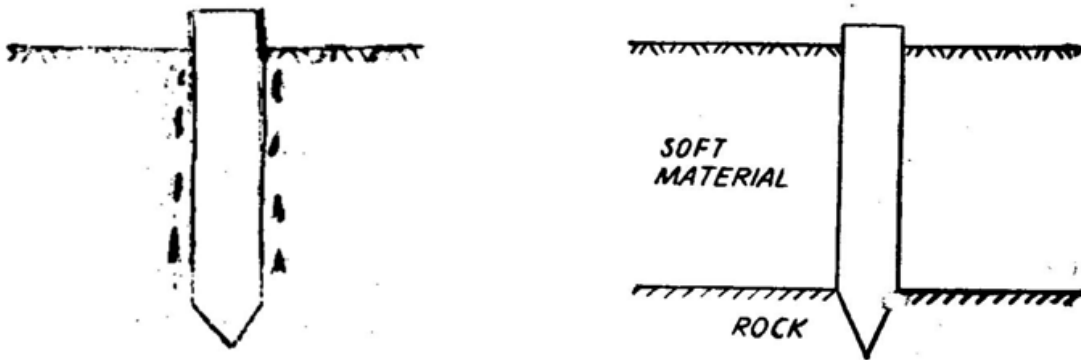
Fig 10.11 Friction pile & Bearing Pile
