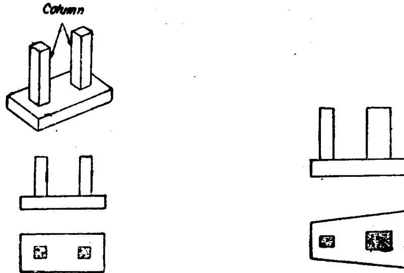
(b) Trapezoidal combined footing.
