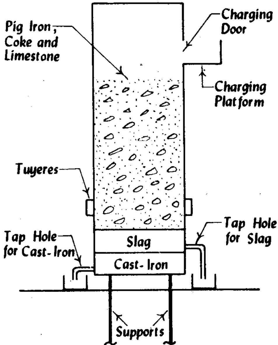
Fig 8.2 Cupola Furnace
