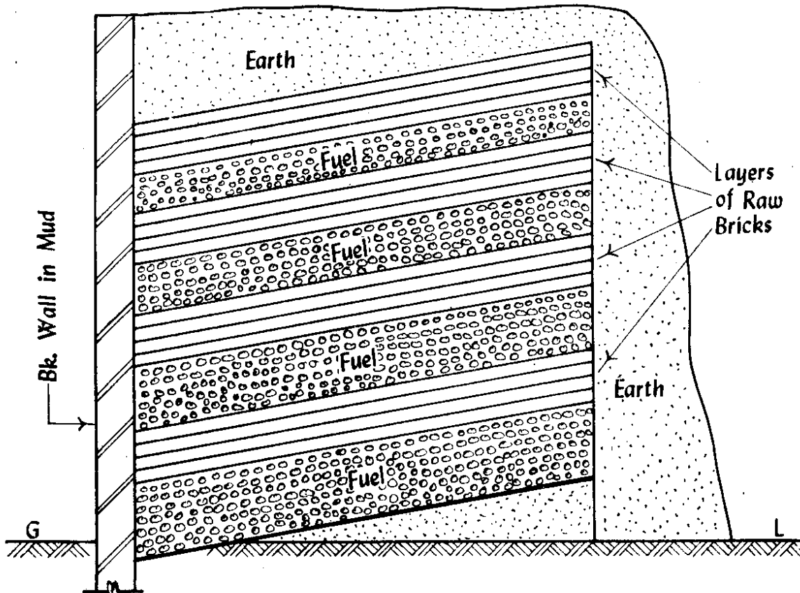
Fig 2.3 Clamp
