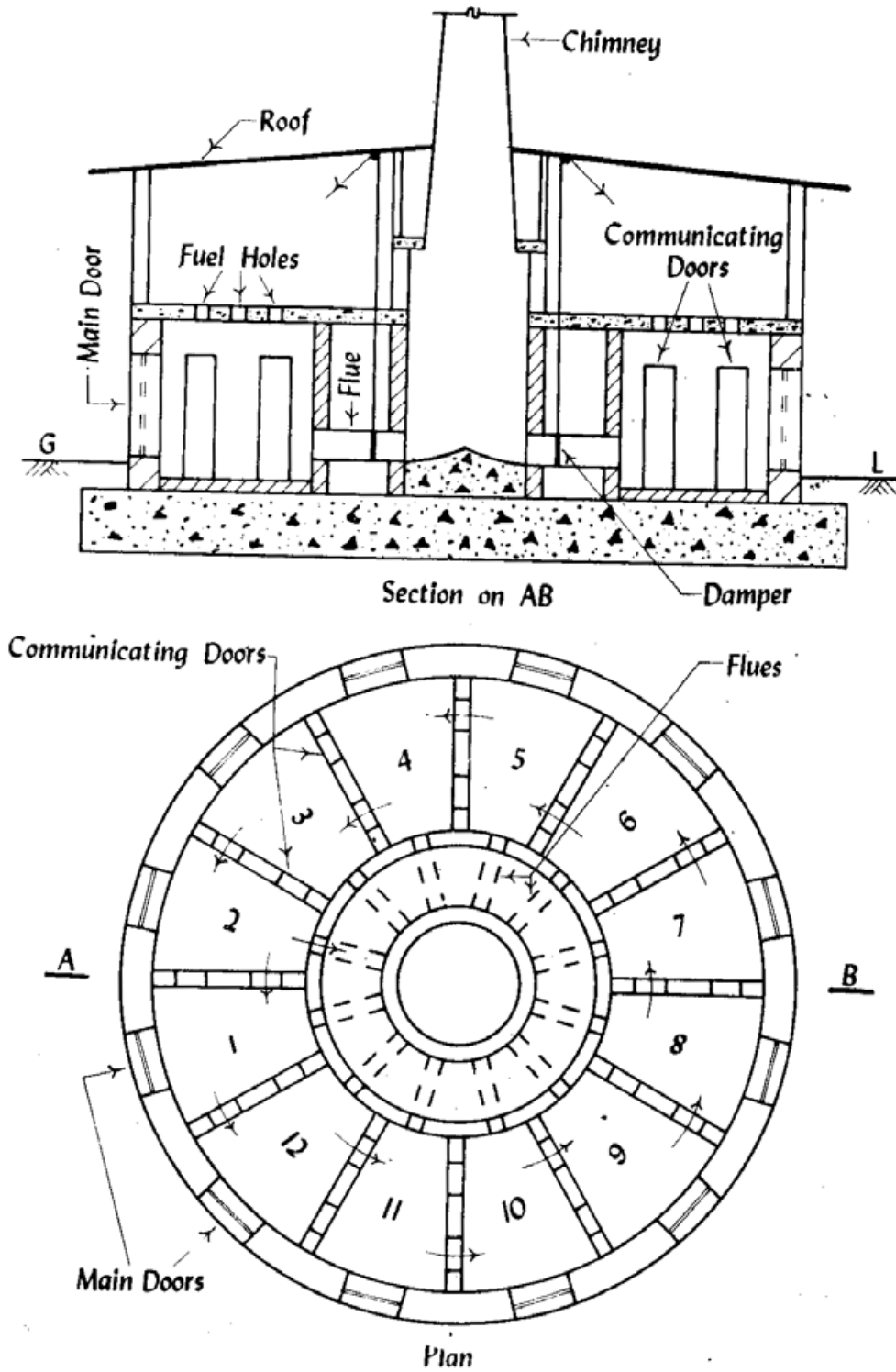
Fig 2.6 Hoffman's kiln
