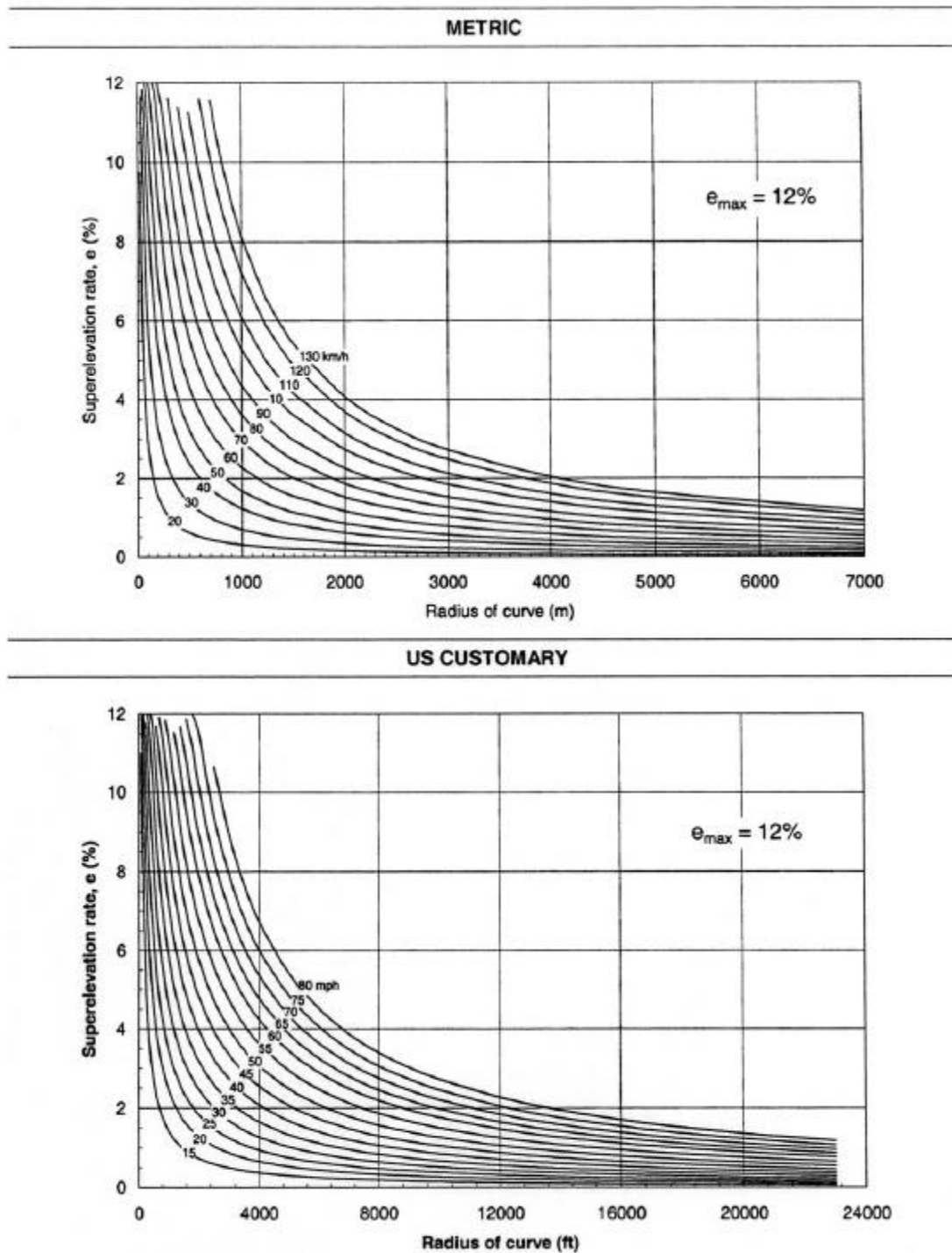
Exhibit 3-20. Design Superlevation Rates for Maximum Superlevation Rate of 12 Percent
