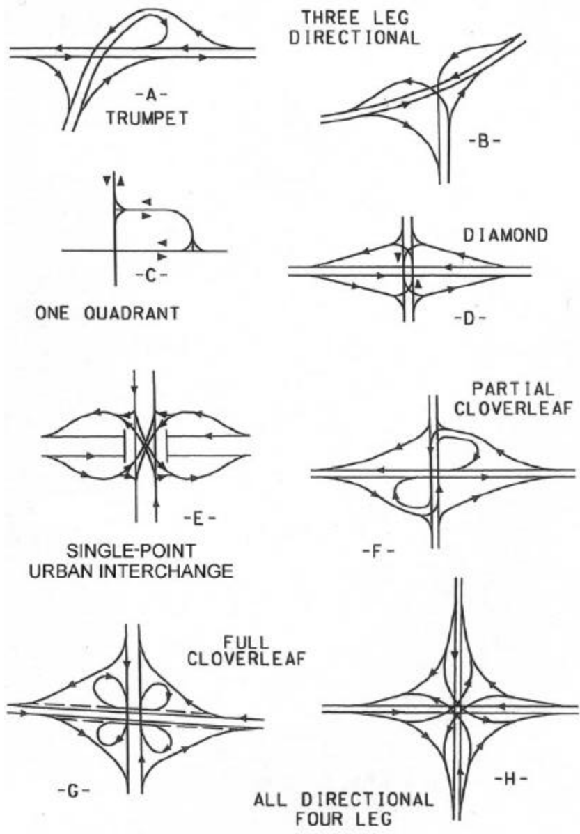
Exhibit 10-1. Interchange Configurations
