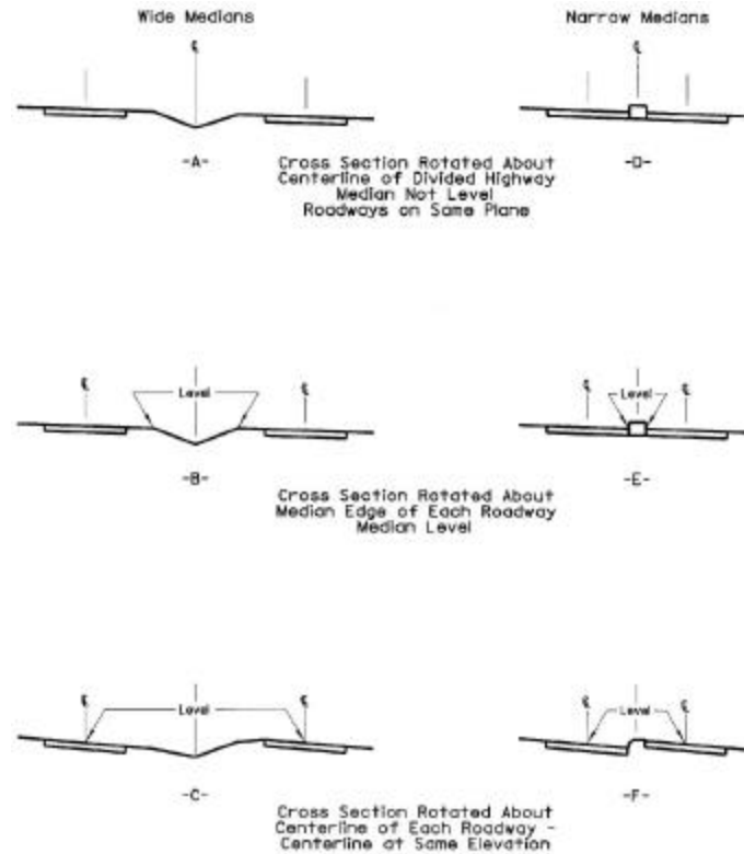
Exhibit 7-6. Methods of Attaining Superelevation on Divided Arterials
