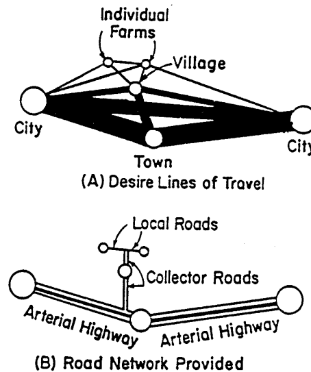
Exhibit 1-2. Channelization of Trips
