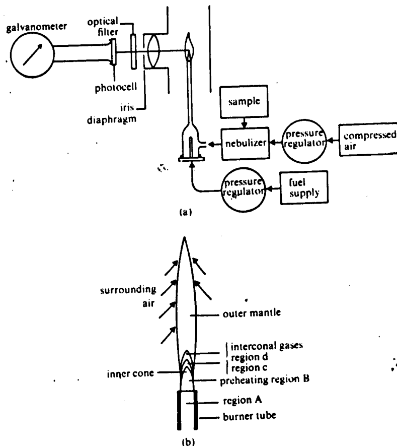
Figure 8.17. (a) Schematic diagram of a flame photometer. (b) Structure of a flame
