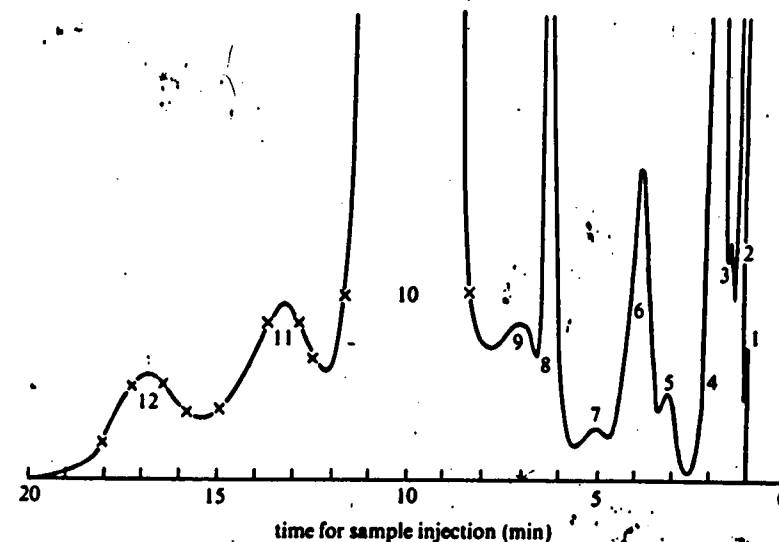
Figure 12.5. Gas chromatogram of the products obtained from n -hexane when passed over a \text{SiO}_2/\text{Pt} catalyst at 450^\circ\text{C} . (Column: 2 m, Apiezon 'L' on 100 to 120 mesh Diatomite 'C'; Carrier gas, helium, 45\text{ cm}^3\text{ min}^{-1} ; Temperature 30^\circ\text{C} ) X = typical sampling points
