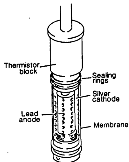
Figure 6.14. Construction of an EIL temperature compensated oxygen electrode (from EIL advertising material)
