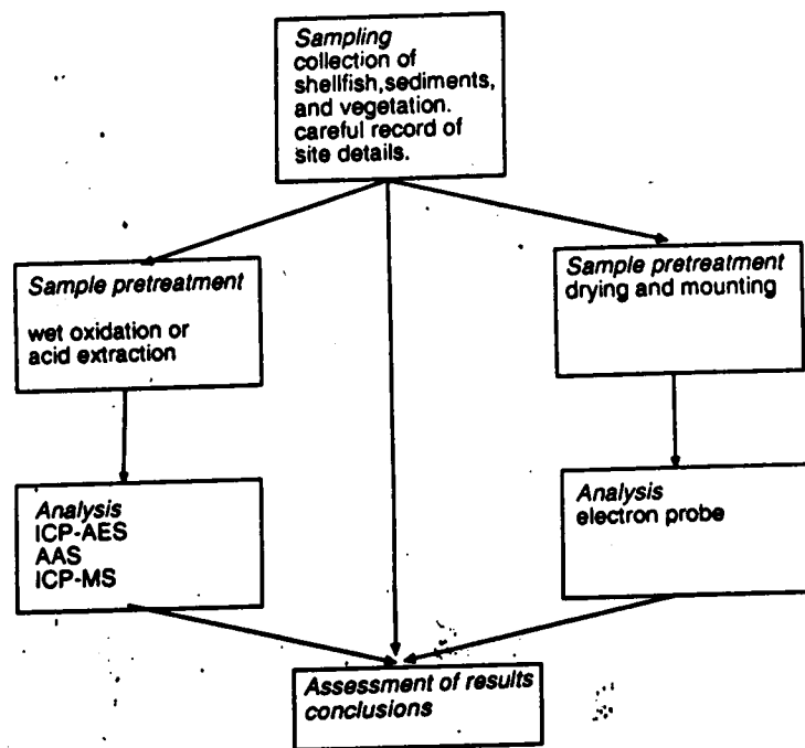
Figure 12.4. Outline analysis of shellfish for heavy metal pollutants
