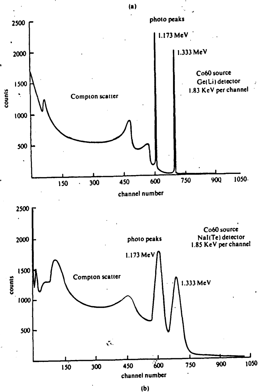
Figure 10.11. (a) \gamma -spectrum of ^{60}\text{Co} obtained by a Ge(Li) detector. (b) \gamma -spectrum of ^{60}\text{Co} obtained by a NaI(Tl) crystal detector
