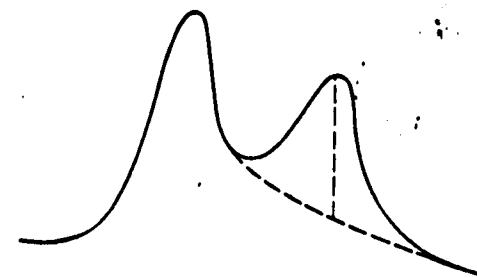
Figure 9.25. Construction of a baseline for quantitative analysis
