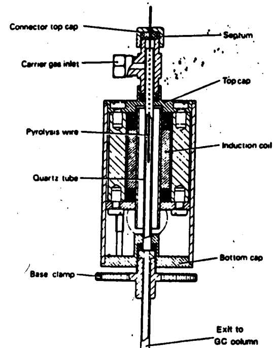
Figure 11.25. A Curie-point pyrolyser. Reprinted from Irwin, Analytical Pyrolysis , Marcel Dekker Inc. NY (1982)
