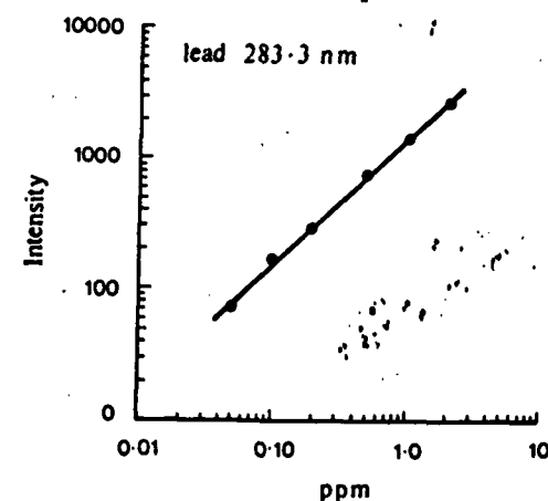
Figure 8.12. Calibration curve for ICP determination of lead in sea water showing the wide linear range
