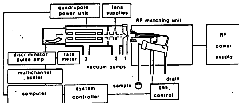
Figure 8.14. Schematic diagram of a typical ICP-MS system. In some systems the multichannel scaler may be omitted
