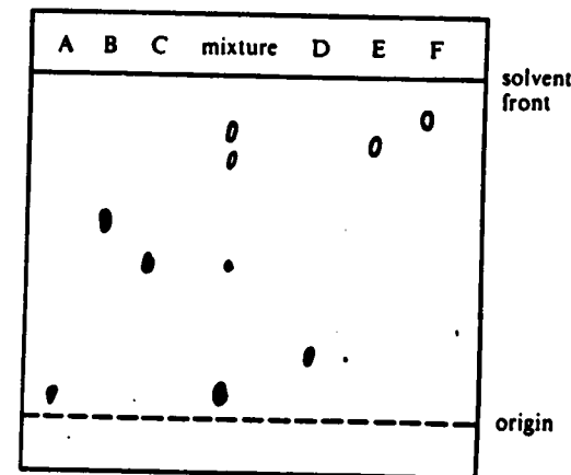
Figure 4.41. Thin-layer chromatogram
