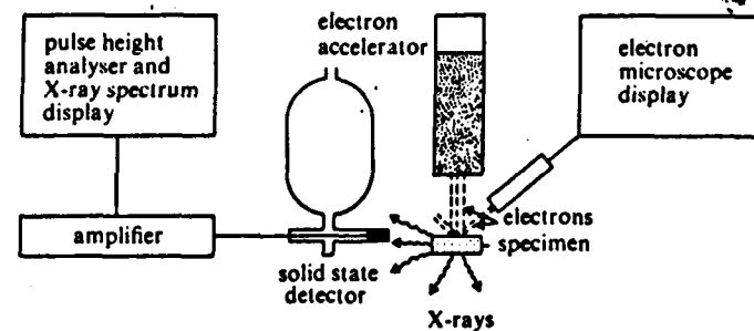
Figure 8.36. Schematic layout of an electron microscope—electron probe analyser
