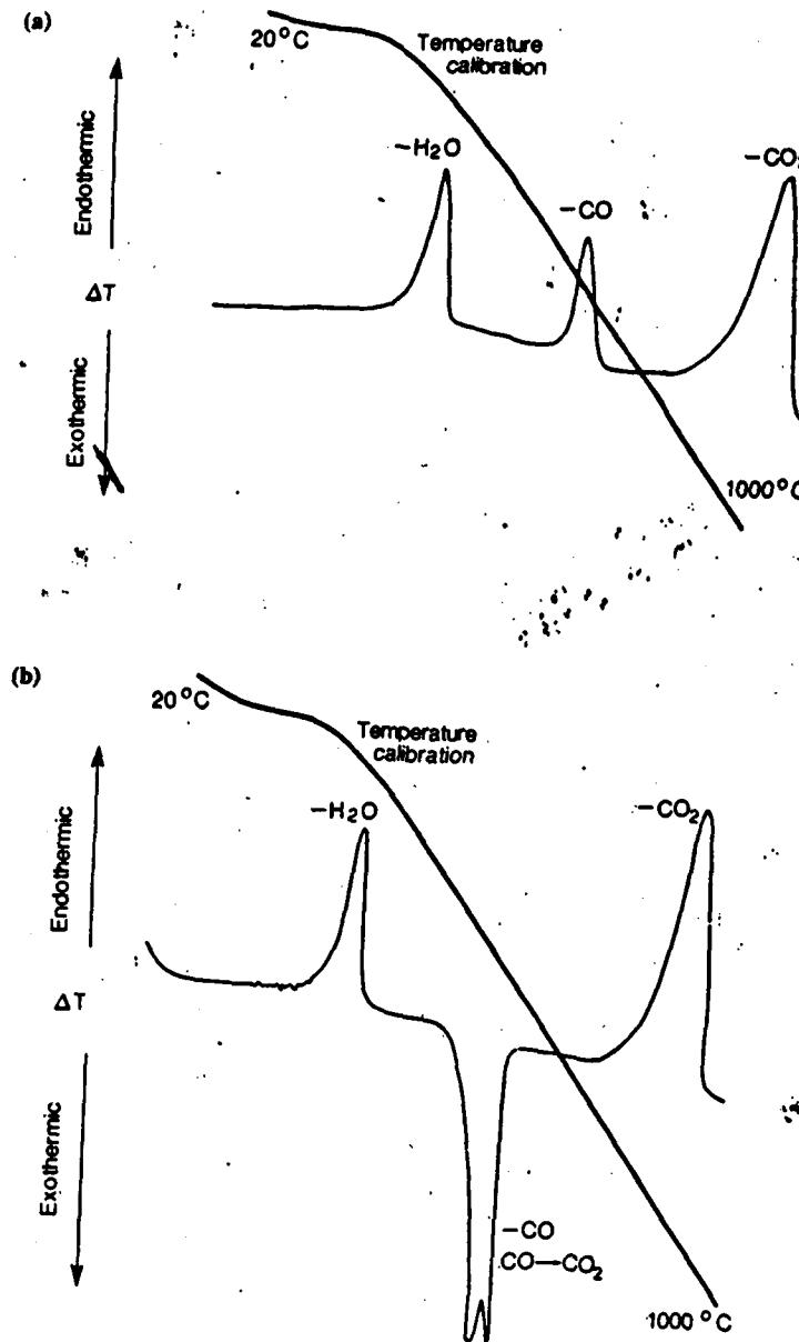
Figure 11.9: DTA study of calcium oxalate \text{CaC}_2\text{O}_4 \cdot \text{H}_2\text{O} showing the effect of changing the atmosphere from (a) nitrogen to (b) air
