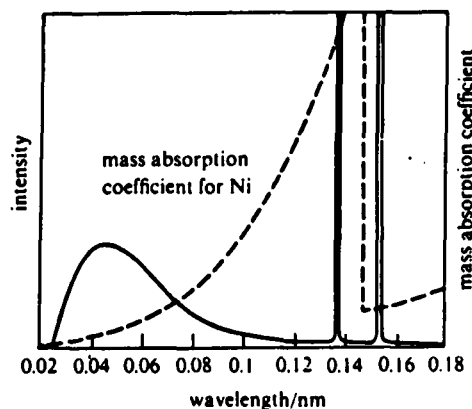
Figure 8.37. Primary X-ray spectrum for Cu with the absorption edge of a nickel filter superimposed showing how it may be used to isolate the long wavelength emission peak
