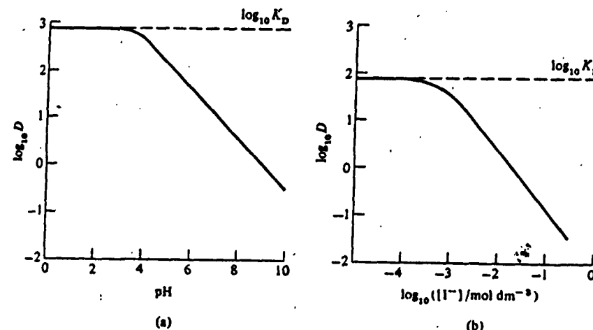
Figure 4.1. The effect of pH and complex formation on extracting species. (a) \log_{10} D against pH for the extraction of benzoic acid, K_a = 6.3 \times 10^{-5} mol dm ^{-3} . (b) \log_{10} D against \log_{10} [I^-]/\text{mol dm}^{-3} for the extraction of I_2 .
