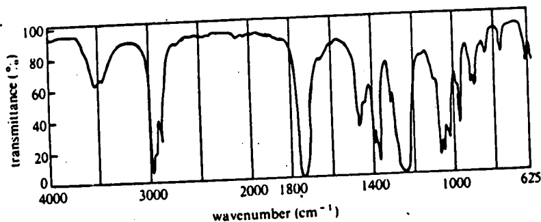
Figure 9.23. Infrared spectrum of n -propyl acetate
