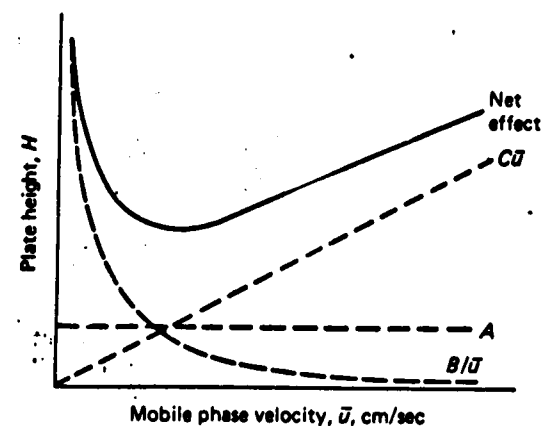
Figure 4.10. Efficiency as a function of mobile phase velocity and the effect of each term in equation 4.45
