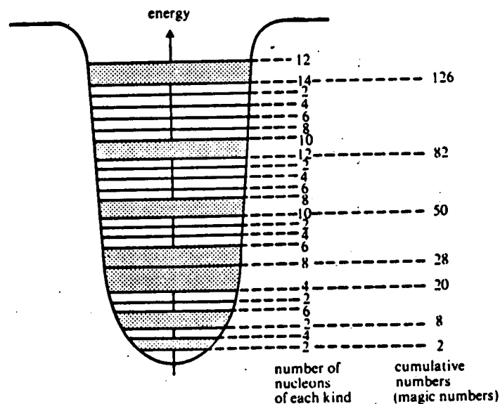
Figure 10.1. Representation of nuclear energy levels showing the energy levels of nucleons and the 'magic numbers' corresponding to filled shells. Shaded areas represent the gaps between the shells
