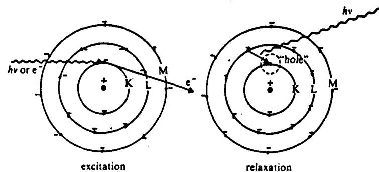
Figure 8.30. Schematic representation of an X-ray fluorescence process
