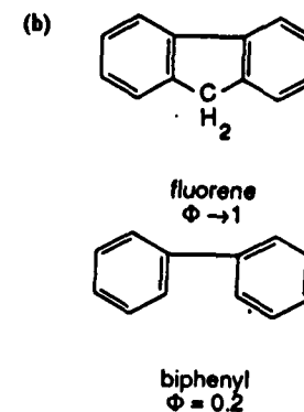
Figure 9.11(b). Effect of structural rigidity on quantum yield, \Phi_f
