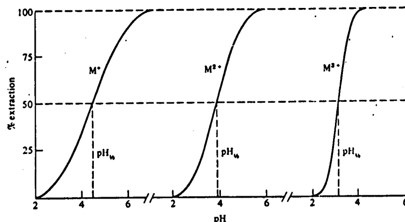
Figure 4.2. Extraction as a function of pH for metals of different formal valencies. (Note: the position of each curve along the pH abscissa is not significant)
