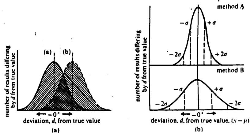
Figure 2.2. Normal error curves. (a) Curve (a) shows a normal distribution about the true value. Curve (b) shows the effect of a determinate error on the normal distribution. (b) Curves showing the results of the analysis of a sample by two methods of differing precision. Method A is the more precise, or reliable
