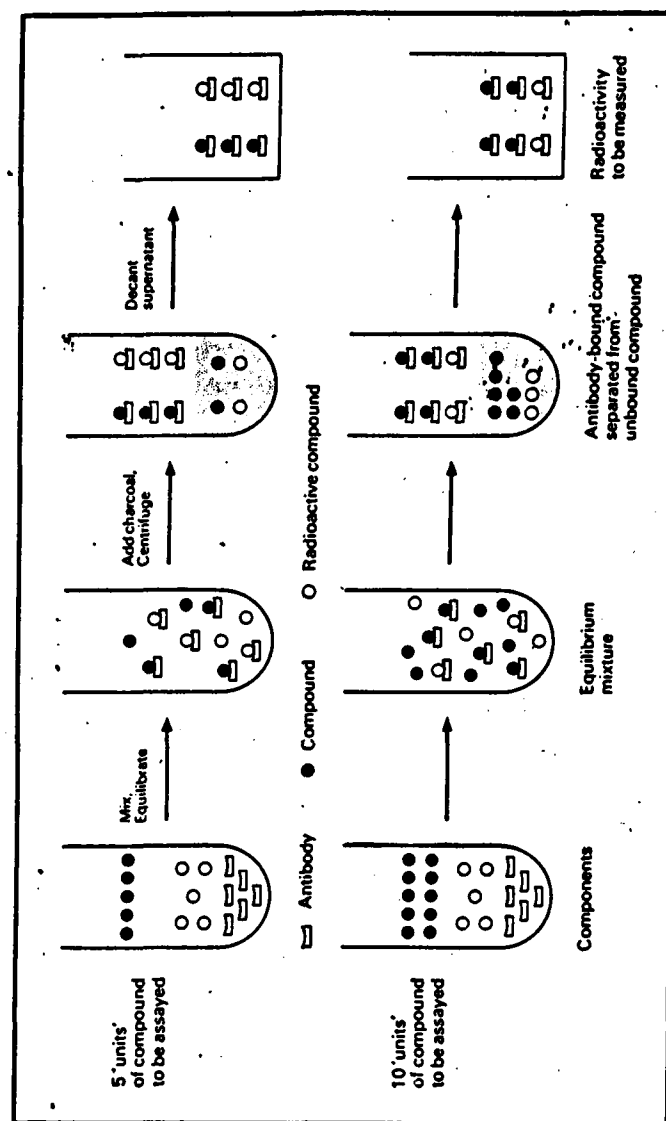
Figure 10.16. The principle of radioimmunoassay. In this example charcoal is used to adsorb the unbound compound and the amount of radioactive compound bound to antibody is measured.
