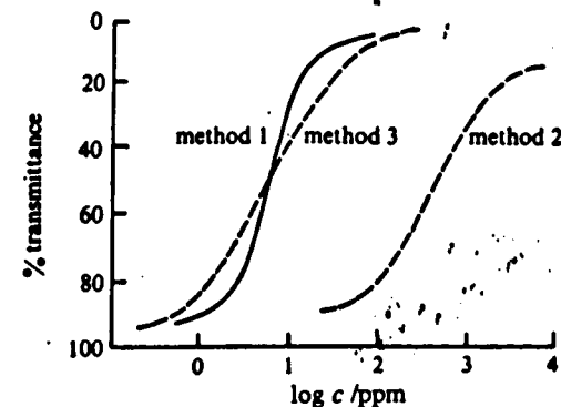
Figure 9.10. Ringbom calibration curves
