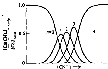
Figure 3.2. The relation between solution composition and the amount of cyanide added in the \text{Cd}^{2+} + \text{CN}^- system.
