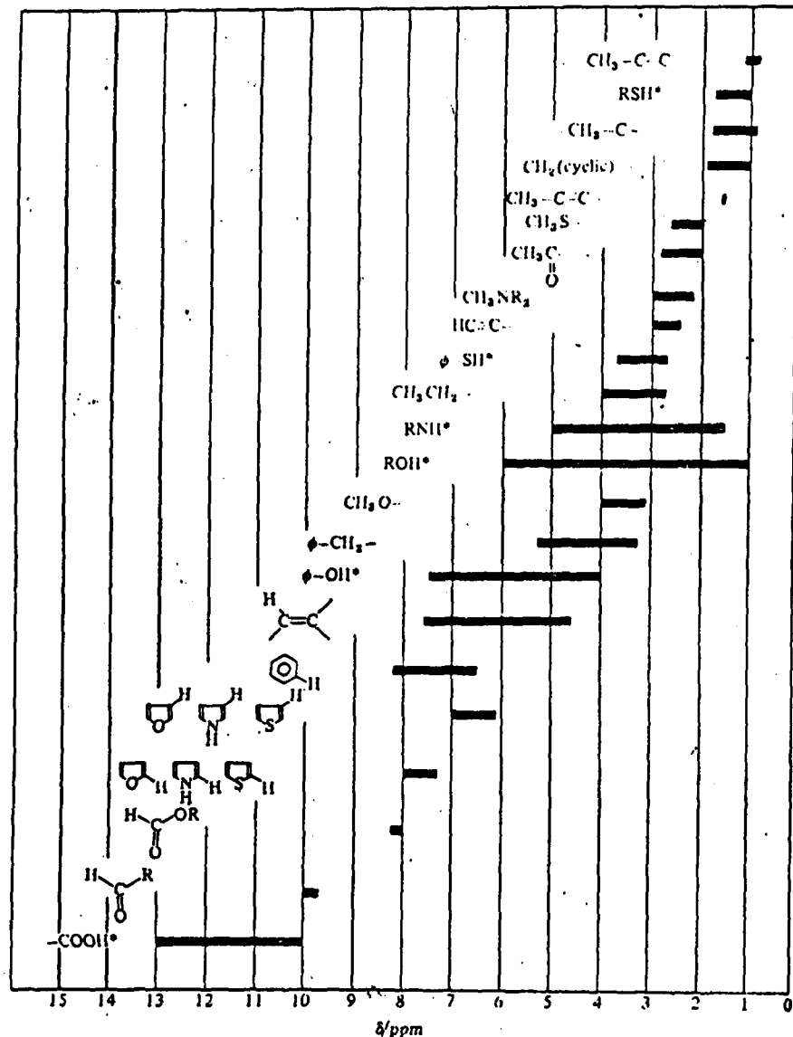
Figure 9.29. Approximate chemical shifts for protons in various functional groups relative to TMS.
