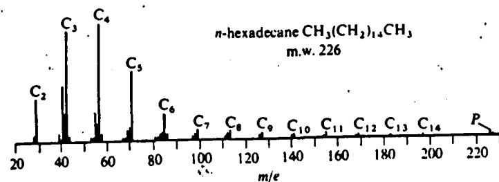
Figure 9.51. Mass spectrum of n -hexadecane
