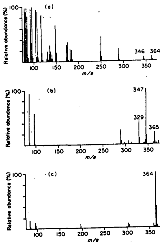
Figure 9.52. Mass spectra of tetrahydrocortisone. (a) E.I.; (b) C.I.; (c) F.I.
