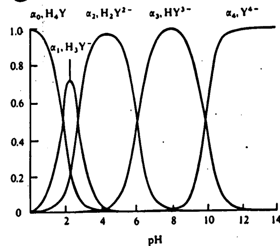
Figure 5.5. The variation of \alpha values with pH for EDTA species
