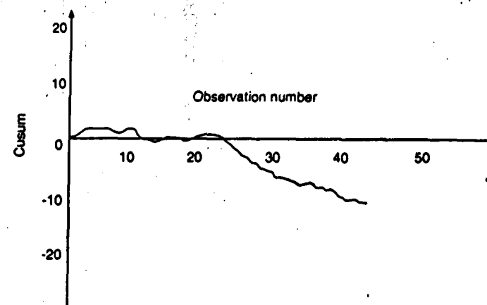
Figure 2.6. A typical cusum plot showing a lack of control with a negative deviation developing after 20 observations
