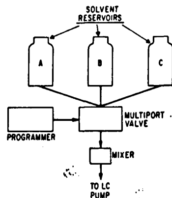
Figure 4.26(c). A low-pressure gradient former with three solvents
