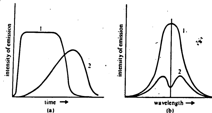
Figure 8.5. (a) Variations of line intensity during burning of sample; element 1 is more volatile than 2. (b) energy-wavelength profile and self-absorption
