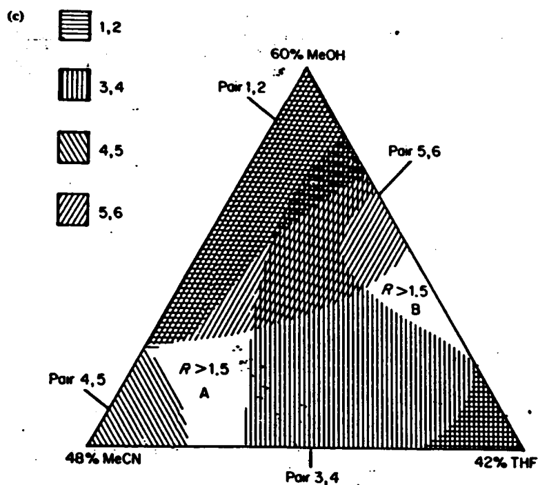
Figure 4.35. (a) Simplex lattice design for reversed-phase chromatographic optimization showing relative proportions of each solvent to be used. (b) Individual resolution maps for the five pairs of solutes in a 6-component test mixture. (c) Overlapping resolution map (ORM) for the 6-component test mixture.
