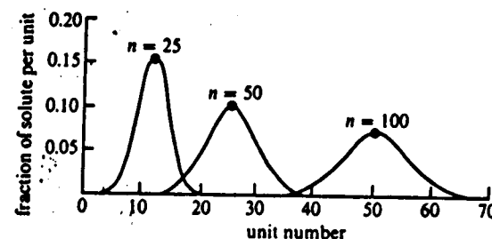
Figure 4.6. Effect of the number n of equilibrations on solute distributions for a distribution ratio D = 1
