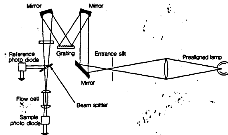
Figure 4.28. Variable-wavelength detector, showing deuterium lamp, optical path, reference photodiode and monochromator
