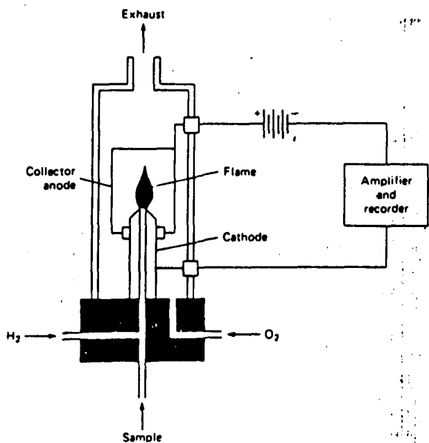
Figure 4.16. Flame ionization detector (fid)
