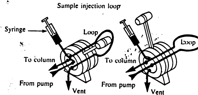
Figure 4.27. Valve injector with external loop
