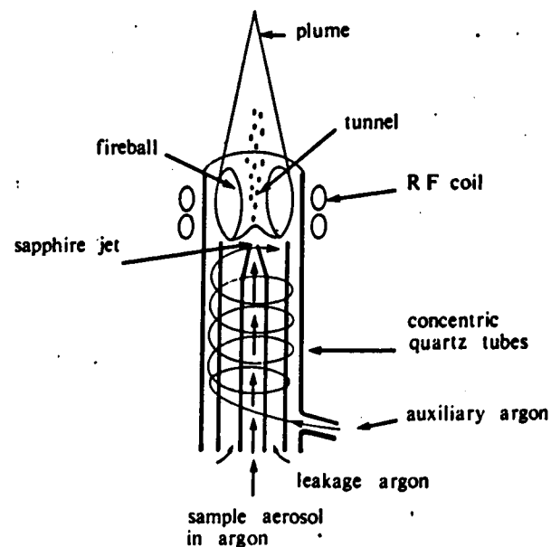
Figure 8.11. ICP torch
