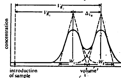
Figure 4.11. Resolution of adjacent peaks
