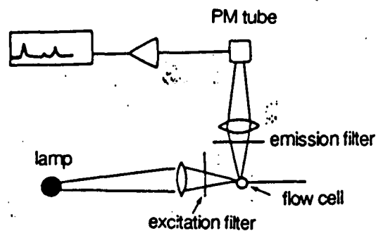
Figure 4.30. Schematic diagram of a simple dual-filter fluorimeter. Excitation using a xenon lamp. Filters used to select the wavelength in both the excitation and emission beams
