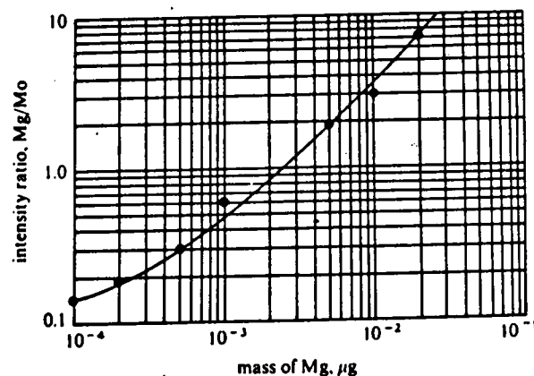
Figure 8.6. Working curve for the analysis of magnesium with molybdenum as internal standard
