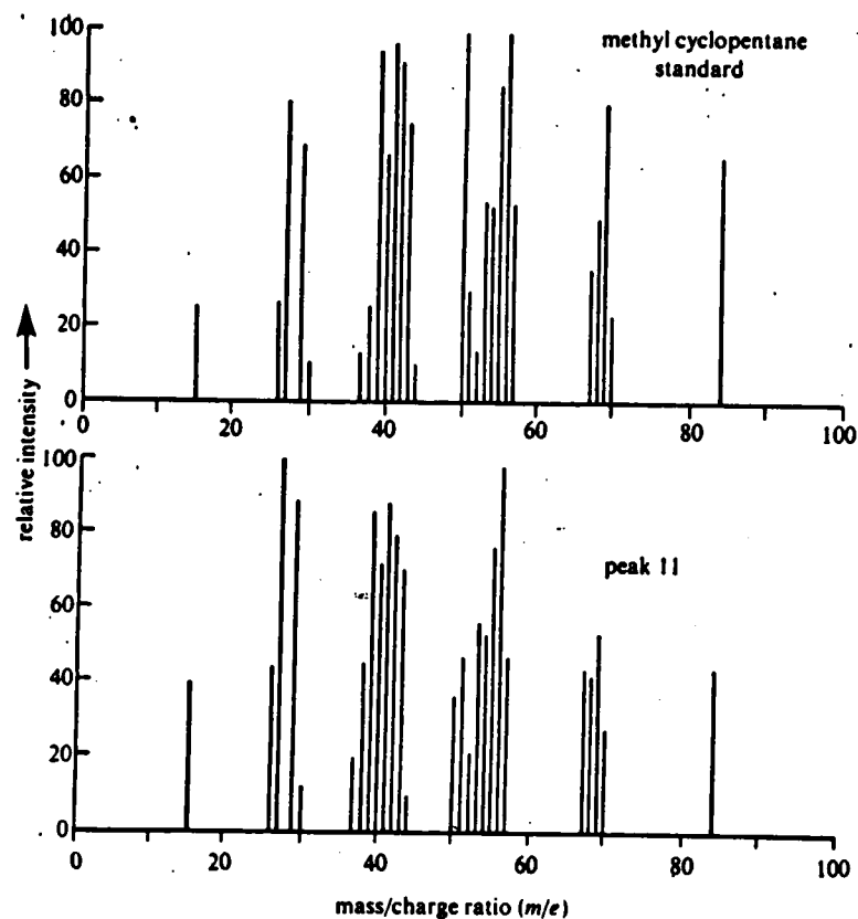
Figure 12.6(a). Mass spectrometric confirmation of peak 11 as methyl cyclopentane
