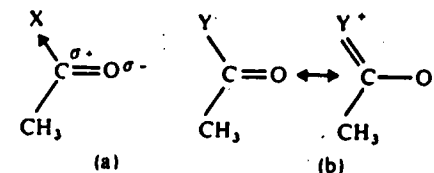
Figure 9.15. Effect of substituents of the carbonyl bond. (a) Inductive effect. X = H, OH, OR, halogen. (b) Resonance effect, Y = \text{NH}_2 , NHR, \text{NR}_2 , phenyl
