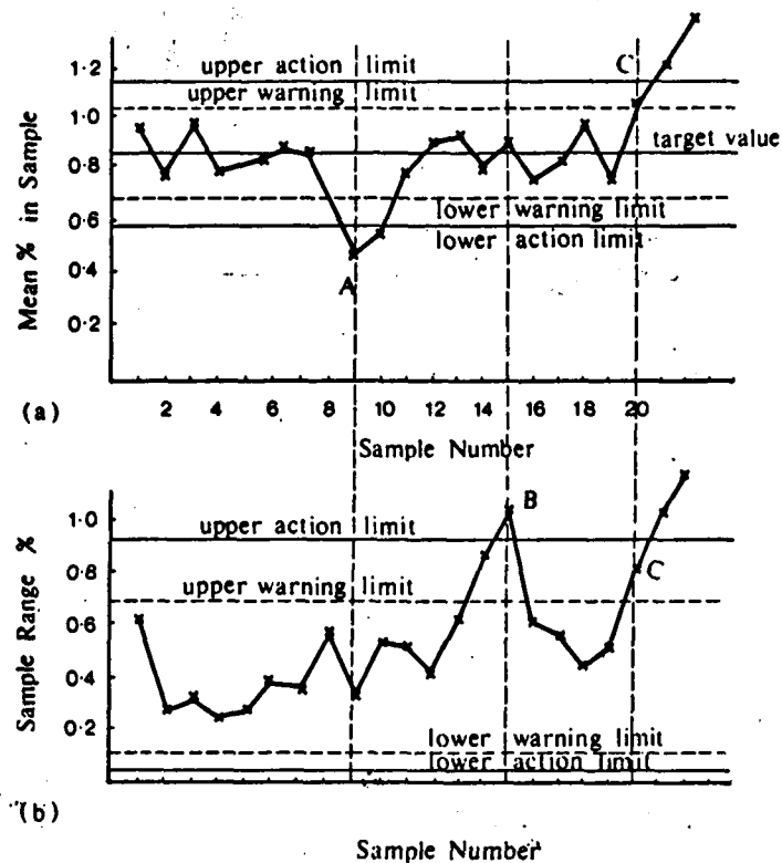
Figure 2.5. A typical pair of Shewhart charts. (a) Averages chart and (b) ranges chart. Point A shows a lack of control of averages only, point B of ranges only and point C of both together
