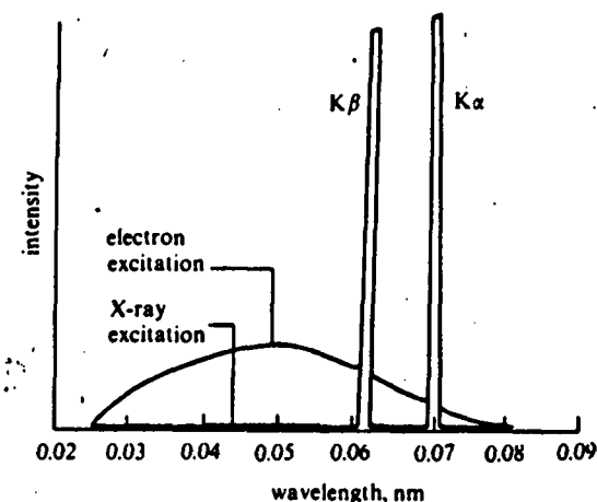
Figure 8.27. Spectra of X-rays emitted from a molybdenum target as a result of electron (25 keV) and X-ray (35 keV) bombardment
