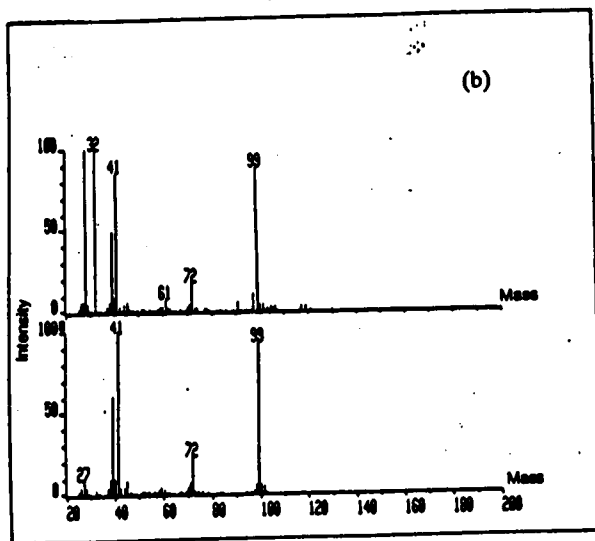
Figure 11.21. (a) Pyrogram of polystyrene cement. (b) Mass spectrum of peak 36 from polystyrene cement and its first library fit: 3-isothiocyanatopropene
