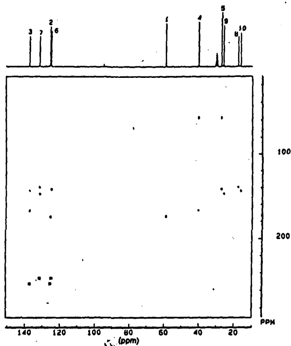
Figure 9.46. The INADEQUATE spectrum of geraniol in \text{CD}_3\text{COCD}_3 at 75.6 MHz for ^{13}\text{C}
