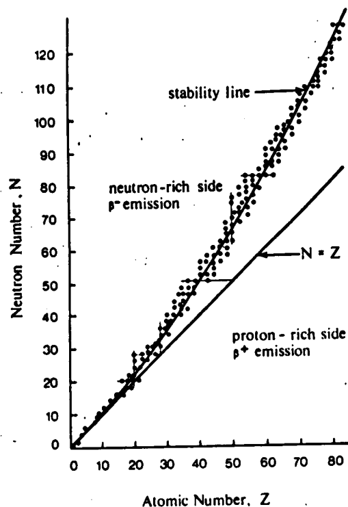
Figure 10.2. Stable nuclides and the stability line
