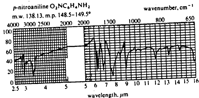
Figure 9.24. Infrared spectrum of p -nitroaniline
