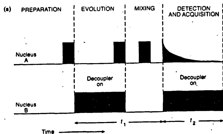
Figure 9.41(a). Generalized multipulse sequence for 1-D or 2-D nmr
