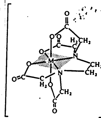
Figure 5.4. A proposed structure for a metal-EDTA chelate showing its octahedral geometry
