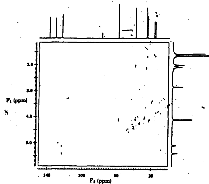
Figure 9.45. The HETCOR spectrum of geraniol, in \text{CDCl}_3 , at 500 MHz for ^1\text{H} and 125.7 for ^{13}\text{C}
