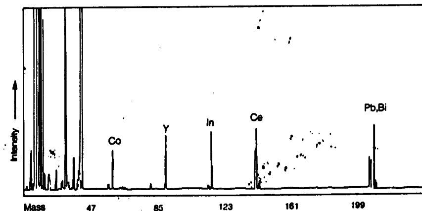
Figure 8.13. ICP-MS spectrum of Be, Al, Co, Y, In, Ce, Pb, Bi and U ( 100 \text{ mg dm}^{-3} ) (courtesy of Dr K. Jarvis, Plasma Mass Spectrometry Laboratory, Royal Holloway College)
