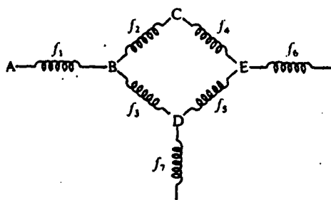
Figure 9.14. Classical analogy of polyatomic molecule
