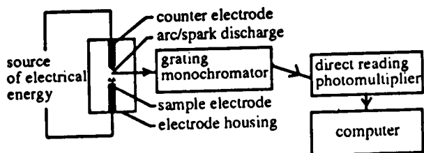
Figure 8.3. Schematic diagram of an emission spectrometer
