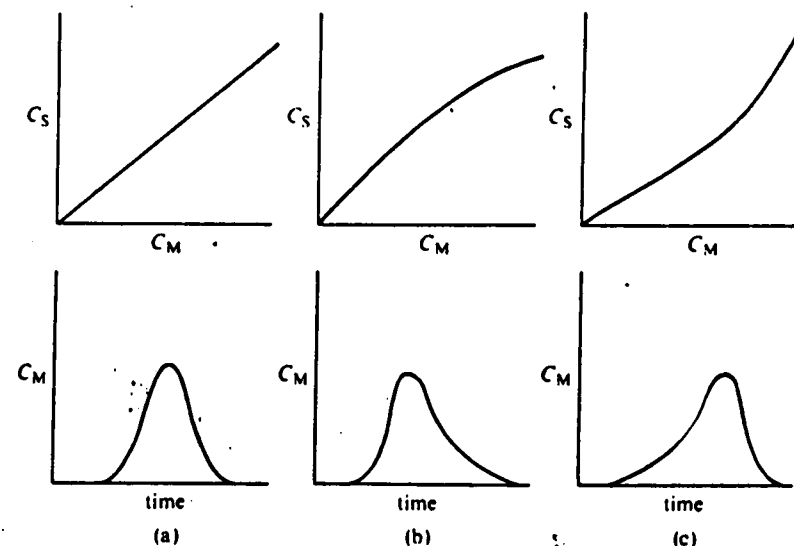
Figure 4.8. Sorption isotherms and concentration profiles. (a) Linear isotherm; Gaussian profile. (b) Curved isotherm; 'tailing'. (c) Curved isotherm; 'fronting'
