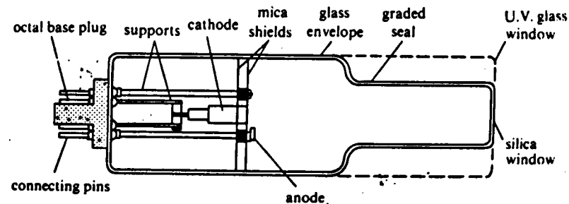
Figure 8.24. Diagram of hollow-cathode lamp
