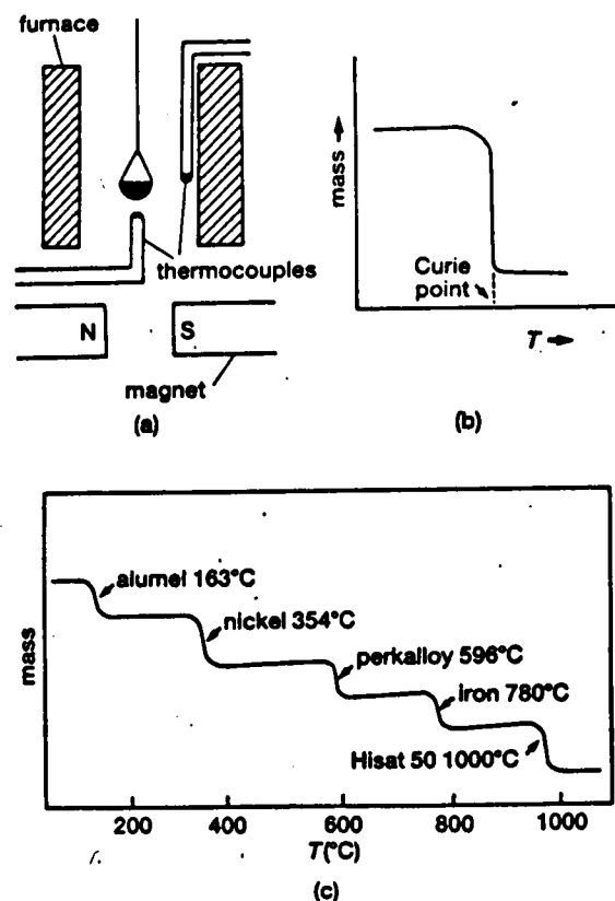
Figure 11.4. Curie-point method of temperature calibration
