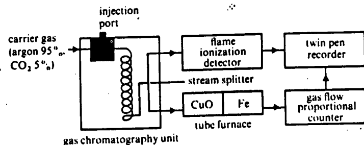
Figure 10.9. Layout of a radio-gas chromatograph
