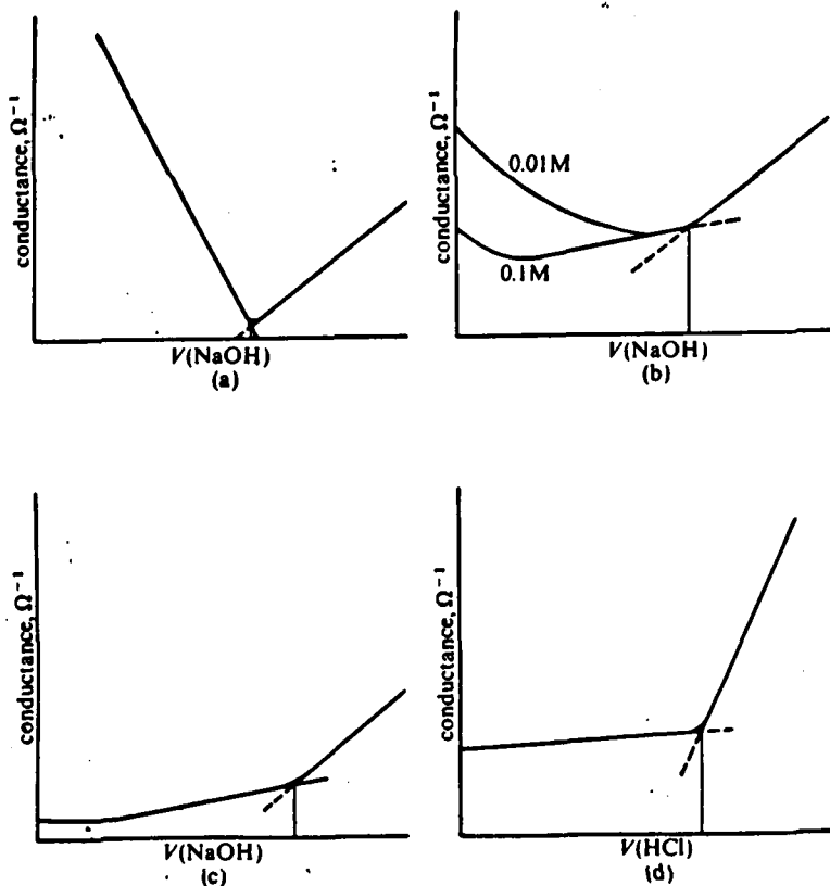
Figure 6.19. Conductometric titration curves (a) Titration of strong acid with NaOH. (b) Titration of acetic acid, K_a = 1.75 \times 10^{-5} \text{ mol dm}^{-3} with NaOH. (c) Titration of boric acid K_a = 6 \times 10^{-10} \text{ mol dm}^{-3} with NaOH. (d) Titration of sodium acetate with HCl
