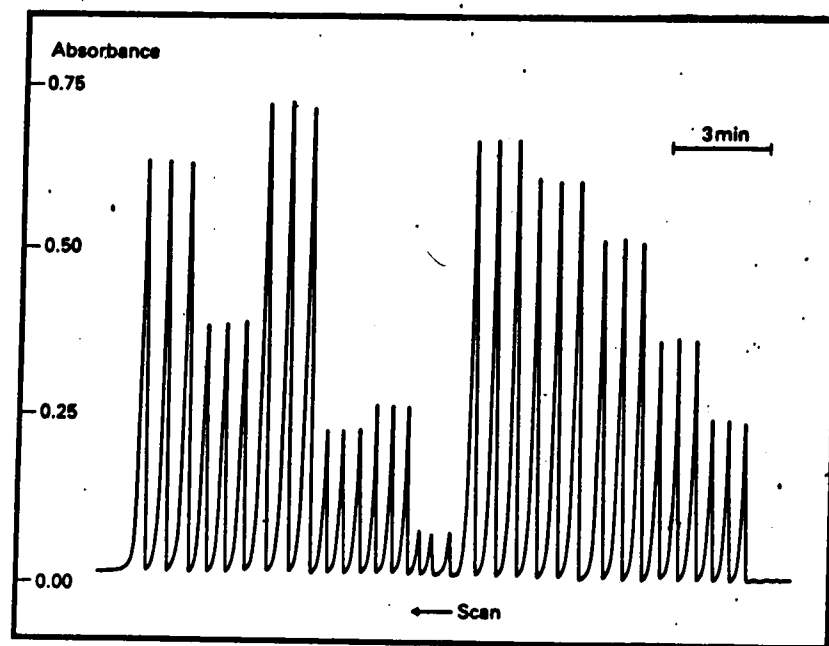
Figure 12.9. Continuous-flow enzymatic determination of ethanol in beverages. To the right is a series of six standards (0–0.4%) followed by six samples—orange juice (1 and 10% v/v), bottled beer (1 and 10% v/v), red wine (1% v/v) and liqueur (1% v/v), all analysed in triplicate (from P. J. Worsfold, Chemistry in Britain , December, 1988)
