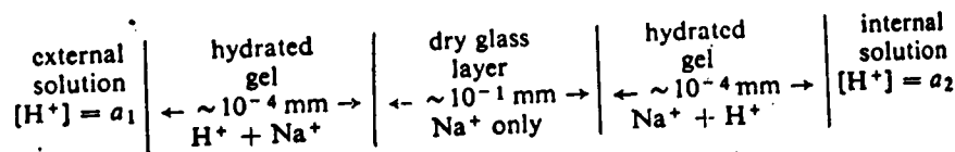
Figure 6.3. Cross-section of a glass membrane
