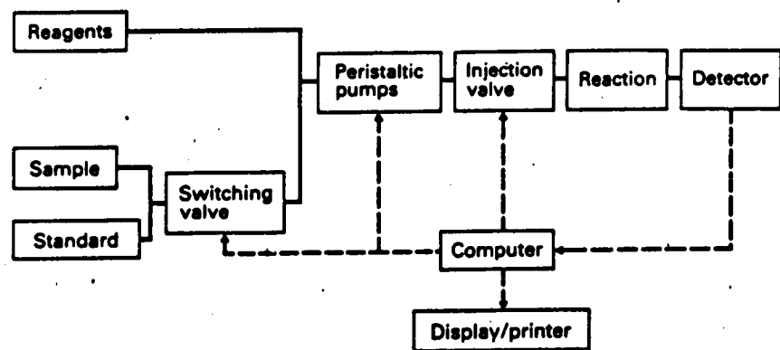
Figure 12.10. Block diagram of a remote spectrophotometric, flow injection based monitor for the determination of nitrate in river water. Reduction to nitrate by copperized cadmium followed by colour development with sulphanilimide and N-1-naphthylmethylenediamine dihydrochloride (from P. J. Worsfold, Chemistry in Britain , December, 1988)
