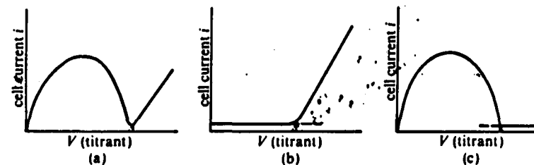
Figure 6.16. Bi-amperometric titration curves. (a) Both electrode reactions reversible, e.g. \text{Fe}^{2+} against \text{Ce}^{4+} . (b) Only titrant reaction is reversible, e.g. \text{AsO}_3^{3-} against \text{I}_2 . (c) Only substance titrated is reversible, e.g. \text{I}_2 against \text{Na}_2\text{S}_2\text{O}_3
