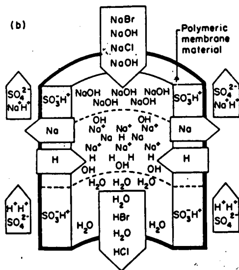
Figure 4.38. (a) Configuration of ion chromatograph with ion-exchange separation column and conductometric detector. (b) Ion chromatography suppressor fibre exchanging hydrogen ions for sodium ions during an anion separation. The halide ions remain as the mineral acids
