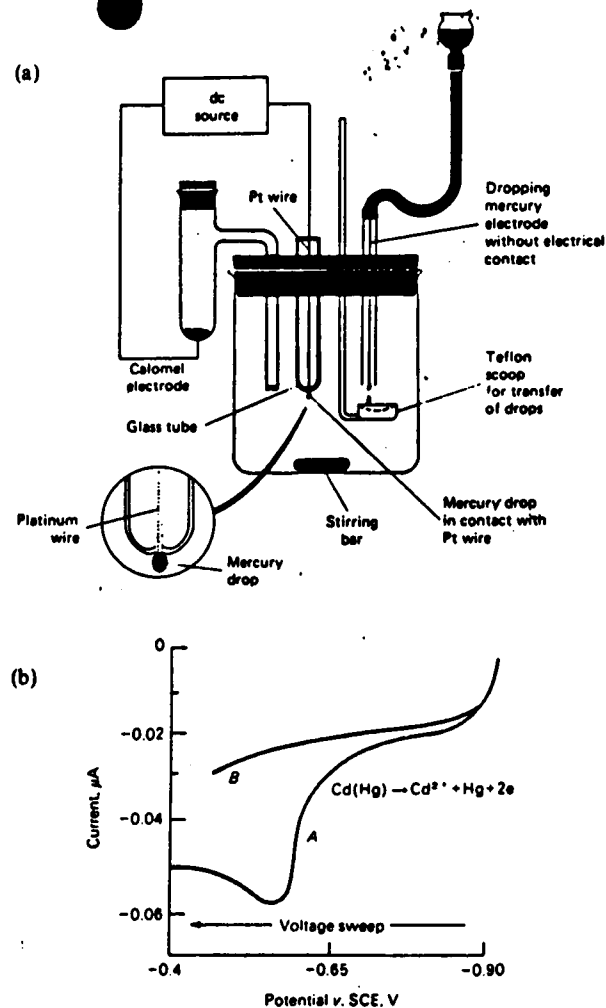
Figure 6.13. (a) Apparatus for stripping analysis. (b) Curve A: Current-voltage curve for anodic stripping of cadmium. Curve B: Residual current curve for blank. Reprinted with permission and adapted from R. D. DeMars and I. Shair, Anal. Chem. 29, 1825 (1957). Copyright by the American Chemical Society
