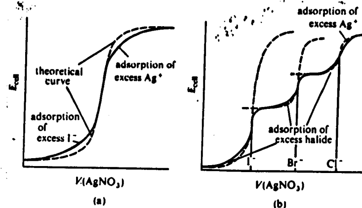
Figure 6.8. Titration of halides with silver nitrate. (a) Titration of iodide with AgNO_3 . (b) Titration of a mixture of chloride, bromide and iodide with AgNO_3
