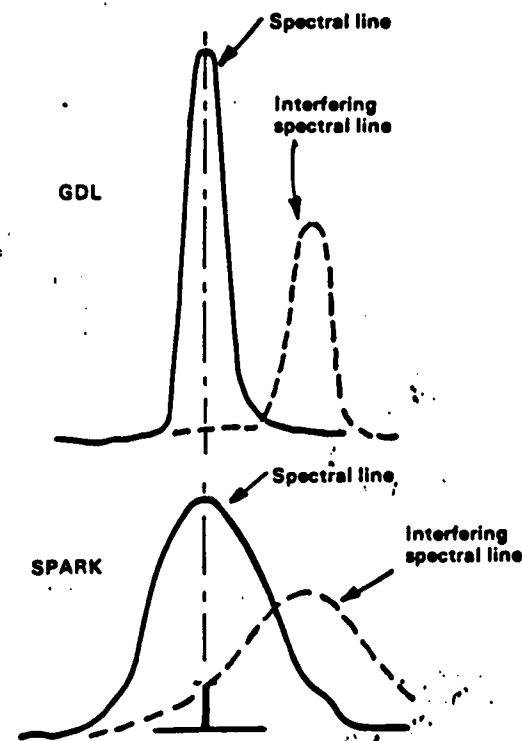
Figure 8.9. Comparison of spectral characteristics of GDL and spark emission signals (with permission from Jobin-Yvon)
