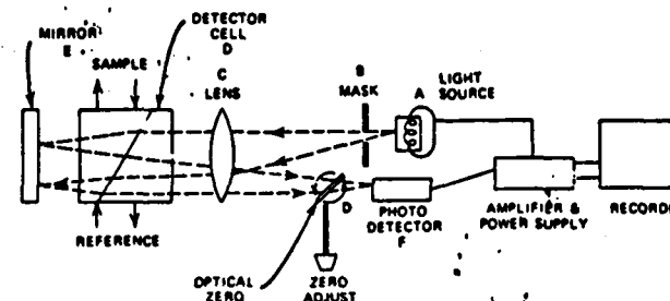
Figure 4.31. Refractive index (RI) detector
