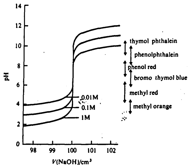
Figure 5.1. The effect of concentration on titration curves and indicators for a strong acid (HCl) and a strong base (NaOH). 100 \text{ cm}^3 of HCl is being titrated with NaOH of the same molarity in each case
