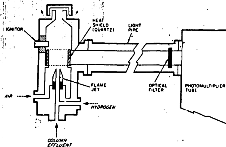
Figure 4.18. Schematic cross-section of a flame photometric detector (fpd)
