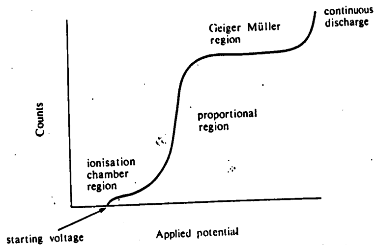
Figure 10.8. Characteristic curve for a gas ionization detector
