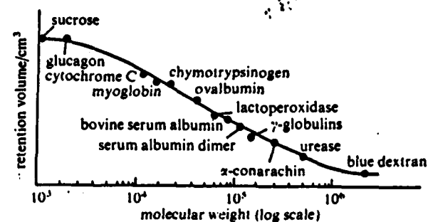
Figure 4.43. Relation between molecular weight and retention volume for proteins at pH = 7.5 (Sephadex G-200 column)
