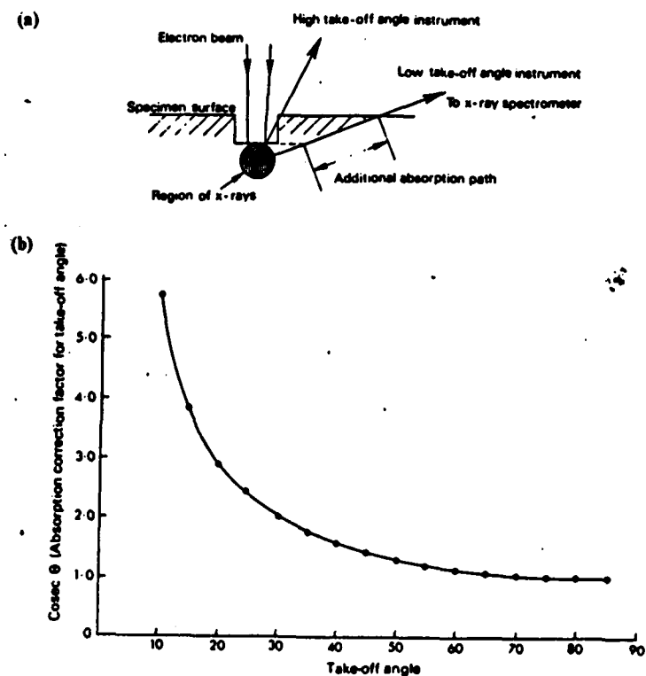
Figure 8.29. (a) Diagram showing the additional absorption path that X-rays must take when operation is at a low take-off angle, as compared to operation at a high take-off angle. (b) Relationship between absorption correction factor and take-off angle
