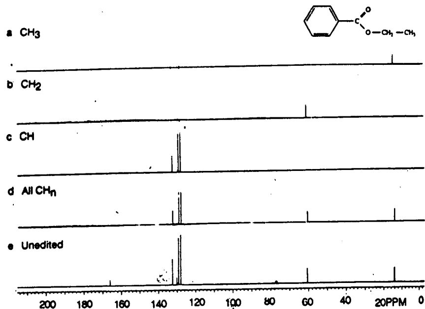
Figure 9.42. DEPT results for ethyl benzoate. (a)–(c): CH 3 , CH 2 , and CH subspectra. (d) Subspectrum of all protonated carbons. (e) Unedited spectrum. 16 fids were accumulated for each \theta value
