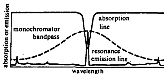
Figure 8.21. Profiles of an absorption line, an emission line from a sharp line source and the bandpass of a monochromator
