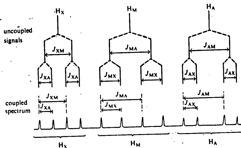
Figure 9.34. Splitting diagram for an AMX system
