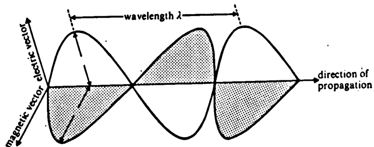
Figure 7.1. Wave representation of electromagnetic radiation
