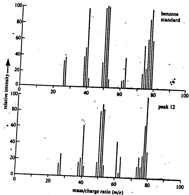
Figure 12.6(b). Mass spectrometric confirmation of peak 12 as benzene
