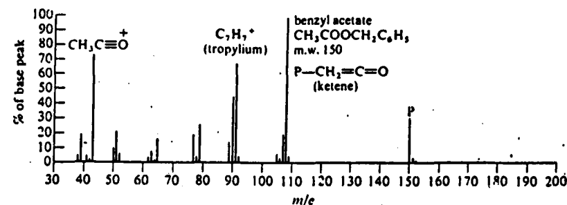
Figure 9.54. Mass spectrum of benzyl acetate
