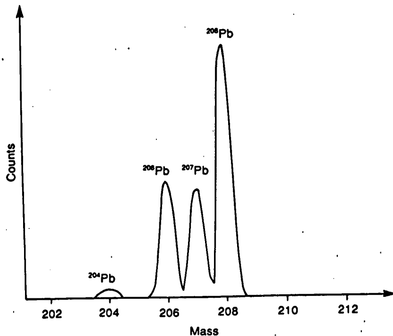
Figure 8.16. ICP-MS spectrum showing the naturally occurring isotopes of lead
