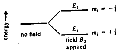
Figure 9.27. Nuclear spin energy levels for a proton or carbon-13, I = \frac{1}{2}
