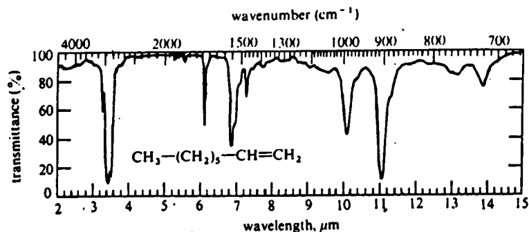
Figure 9.19. Infrared spectrum of 1-octene
