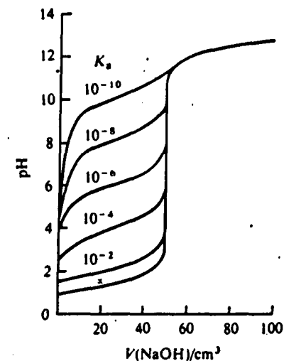
Figure 5.2. The effect of K_a on the titration curves for weak acids with a strong base. 50 \text{ cm}^3 of 0.1 \text{ M} acid is being titrated with 0.1 \text{ M} NaOH in each case
