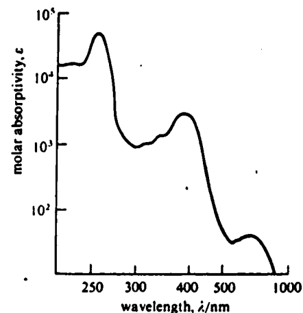
Figure 9.6. uv/visible absorption spectrum of bis(8-hydroxyquinoline)Cu(II)
