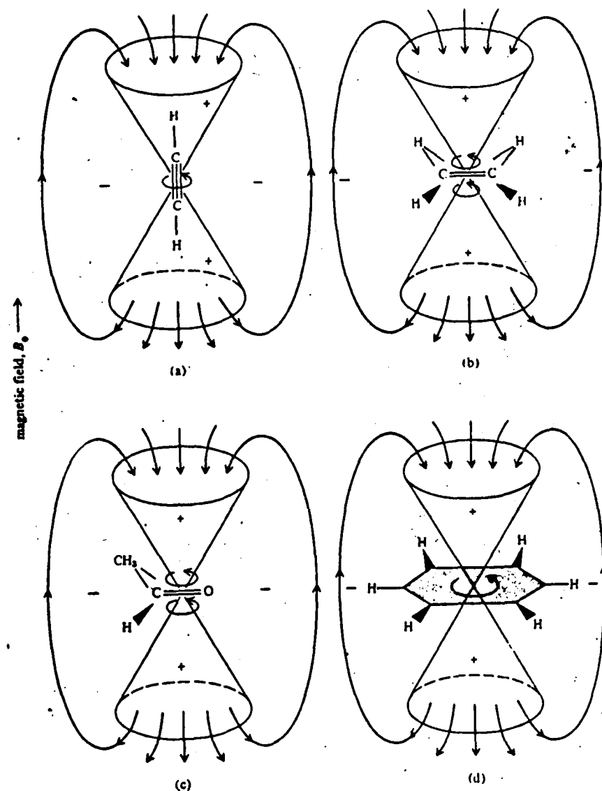
Figure 9.30. Anisotropic shielding in unsaturated groups. (Shielding zones +; deshielding zones -). (a) Acetylene. (b) Ethylene. (c) Acetaldehyde. (d) Benzene
