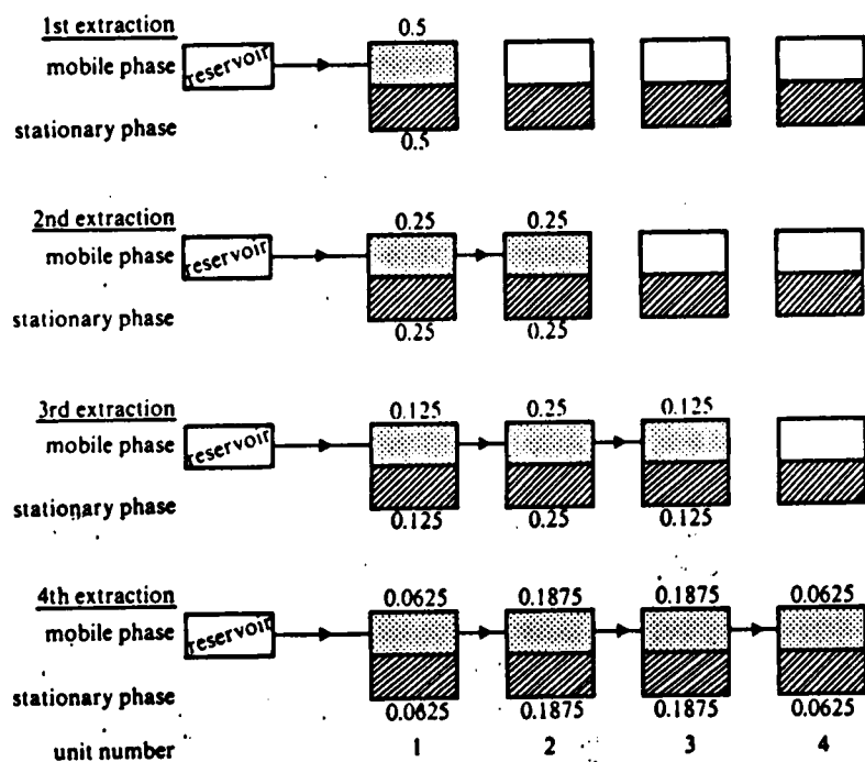
Figure 4.5. Extraction scheme for a single solute by Craig counter-current distribution. (Figures represent the proportions in each phase for D = 1 and equal volumes. Only the first four extractions are shown)
