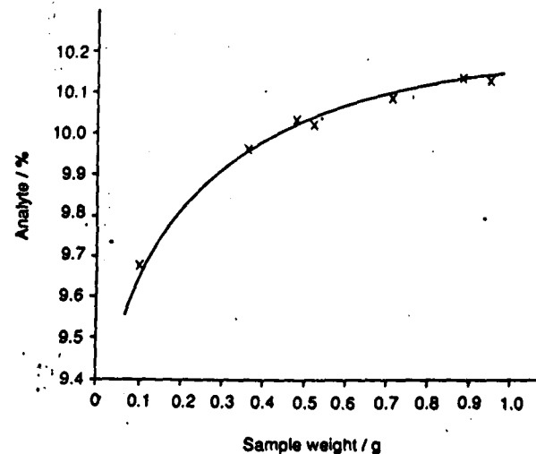
Figure 2.3. Plot of analyte content against sample weight to investigate a determinate error
