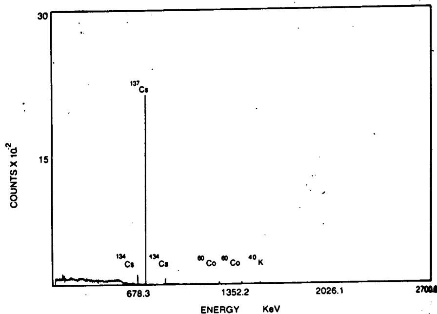
Figure 10.18. \gamma -Ray spectrum of a soil sample from Belarus showing the identification of ^{134}\text{Cs} and ^{137}\text{Cs} fallout from the Chernobyl accident
