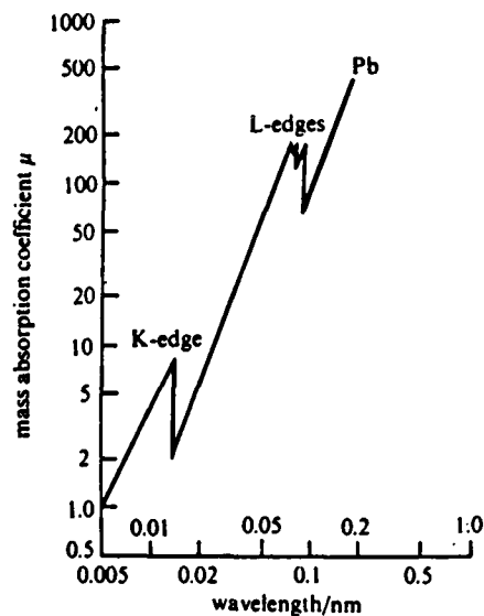
Figure 8.33. Log-log plot of mass absorption coefficient against wavelength for lead showing K and L absorption edges
