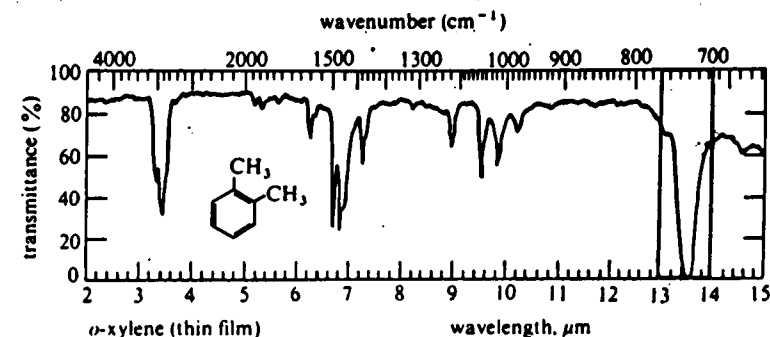
Figure 9.18. Infrared spectrum of 1,2-dimethylbenzene
