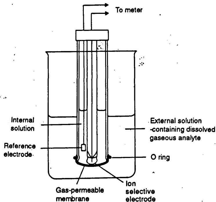
Figure 6.5. Schematic diagram of a gas-sensing electrode. Selective ion electrode is shown as a glass electrode. The reference electrode is an Ag-AgCl electrode. Other electrode combinations are possible
