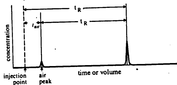
Figure 4.21. Measurement of adjusted retention time, t'_R
