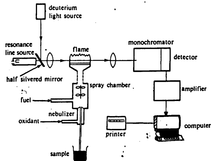
Figure 8.22. Practical system for flame atomic absorption spectrometry including a deuterium background corrector
