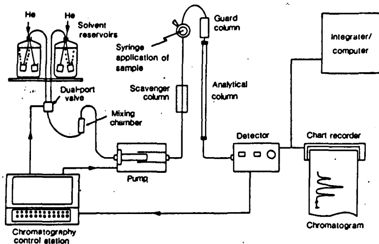
Figure 4.25. Schematic diagram of a binary (2-solvent) hplc system
