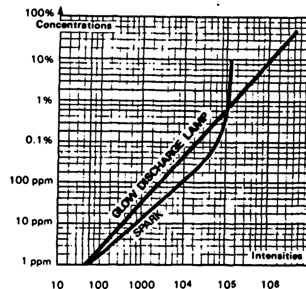
Figure 8.7. Typical GDL and spark emission calibration curves contrasting range and linearity (with permission from Jobin-Yvon)
