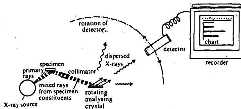
Figure 8.35. Schematic layout of a dispersive X-ray fluorescence spectrometer
