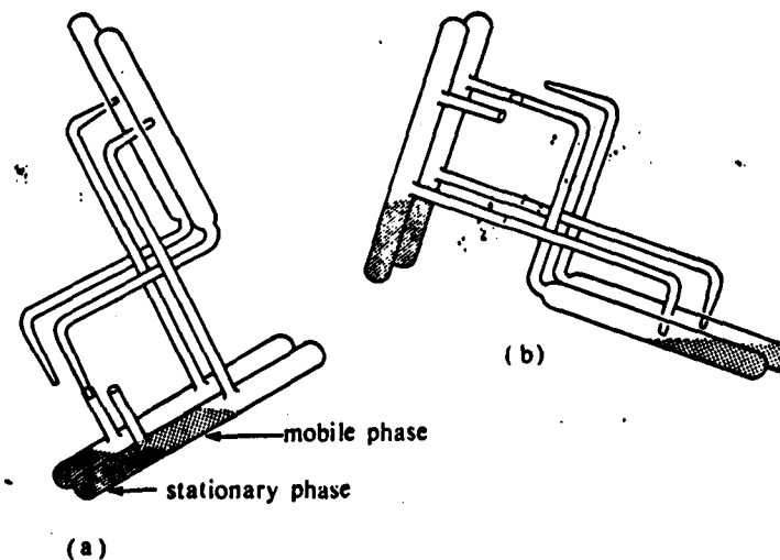
Figure 4.4. Two interlocking glass units for Craig counter-current distribution. (a) Position during extraction. (b) Position during transfer. (Note: by returning the apparatus from (b) to (a) the transfer is completed. The mobile phase moves on to the next unit and is replaced by a fresh portion)
