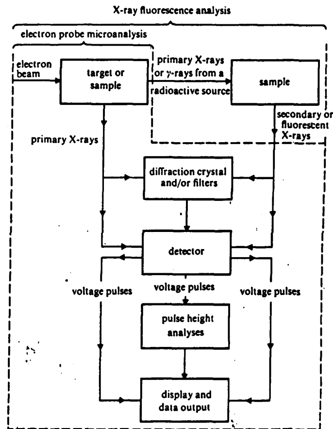
Figure 8.32. Schematic representation of X-ray emission spectrometry
