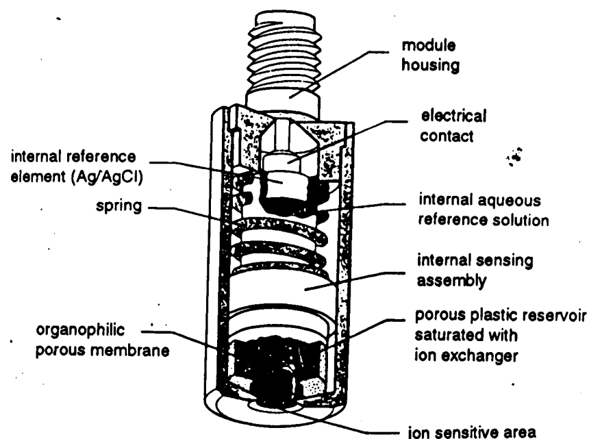
Figure 6.4. Calcium sensitive ion-exchange membrane electrode
