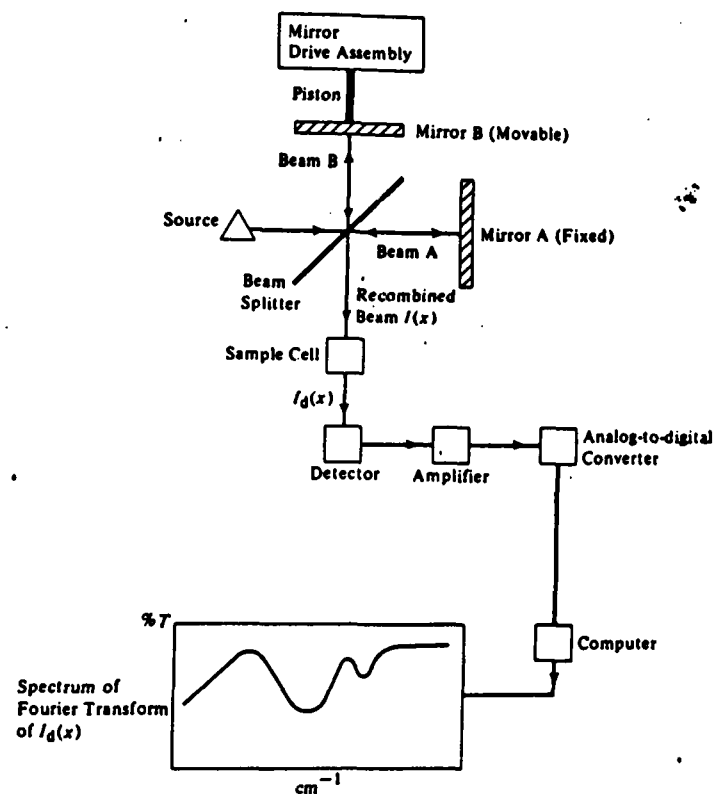
Figure 7.8. Interferometer and associated electronics
