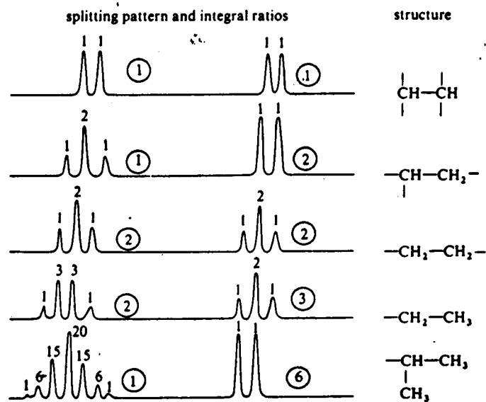
Figure 9.32. First order splitting patterns for some common molecular structures. (Numbers in circles represent relative total areas of the multiplets)
