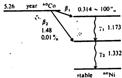
Figure 10.4. Decay scheme for ^{60}\text{Co}
