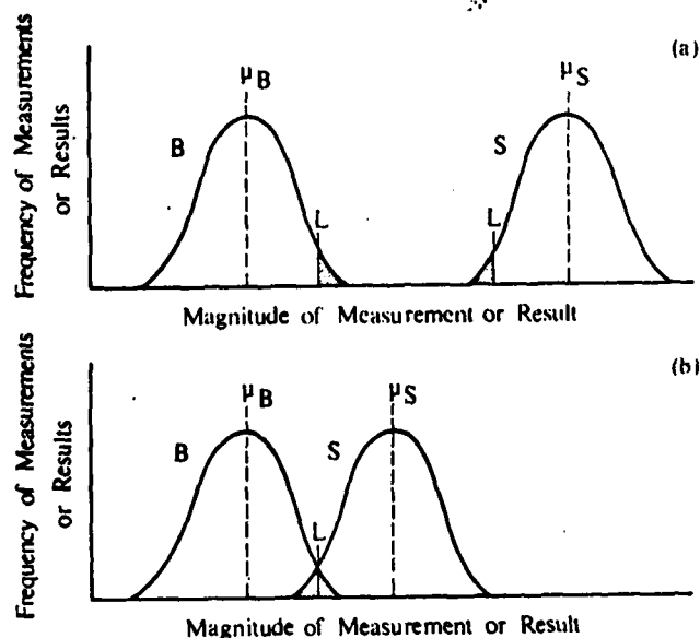
Figure 2.4. Normal error curves for blank B and sample S measurements
