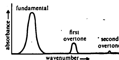
Figure 9.13. Infrared spectrum of a diatomic molecule in solution
