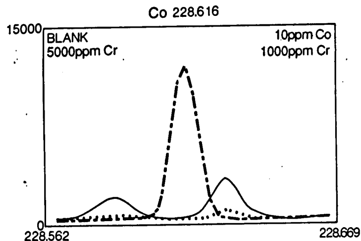
Figure 8.4. Wavelength characterization scan (from ARL laboratories). Key: — 5000 ppm Cr; --- 1000 ppm Cr; - · - · - 10 ppm Co.
