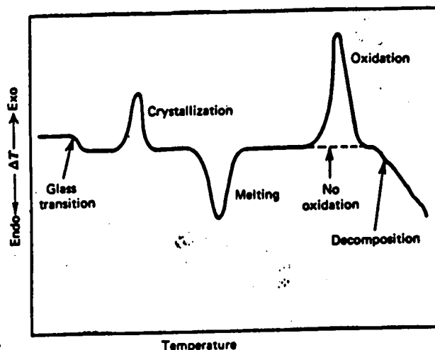
Figure 11.13. Schematic DTA curve of a typical polymer. Note: glass transitions reflect a heat capacity change but none H = 0 . Thus they are seen as 'steps' on the baseline rather than peaks
