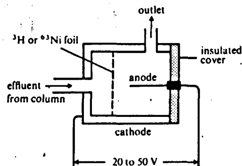
Figure 4.17. Electron capture detector (ecd)
