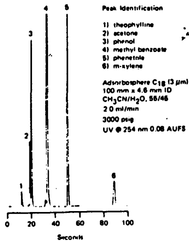
Figure 4.40. Examples of separation by hplc and ic
