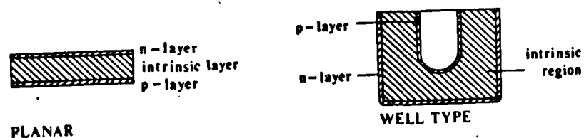
Figure 10.13. Cross-sections through typical lithium drift radiation detectors
