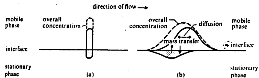
Figure 4.9. Effects of diffusion and mass transfer on peak width. (a) Concentration profiles of a solute at the beginning of a separation. (b) Concentration profiles of a solute after passing some distance through the system.
