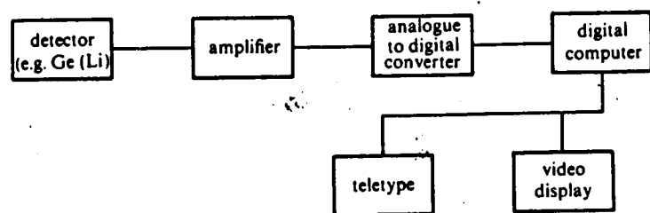
Figure 10.15. Layout of a nuclear spectrometer with a computer to provide pulse height analysis
