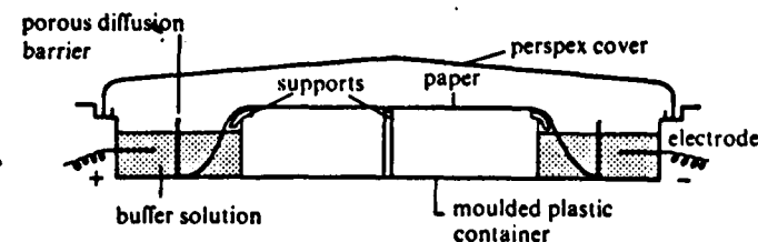
Figure 4.44. Apparatus for paper electrophoresis
