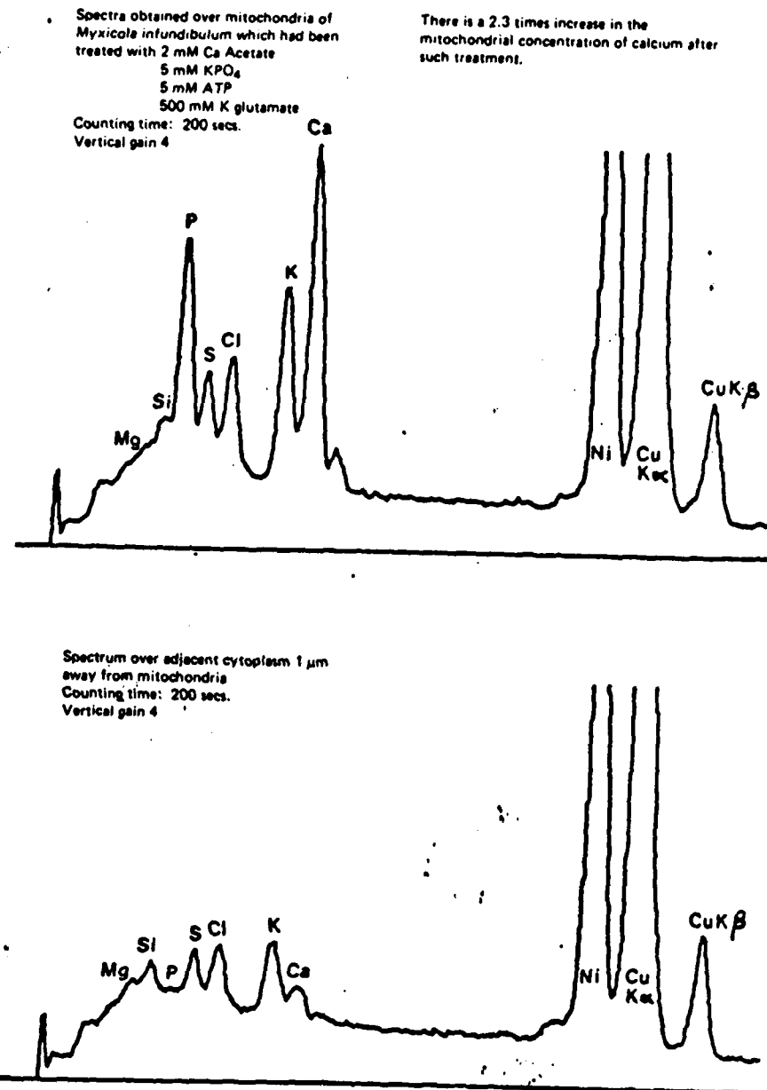
Figure 8.40. Electron probe—SEM X-ray spectra demonstrating the ability of the technique to distinguish between targets in close juxtaposition
