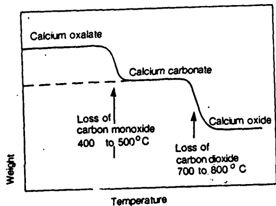
Figure 11.1. TG curve for calcium oxalate
