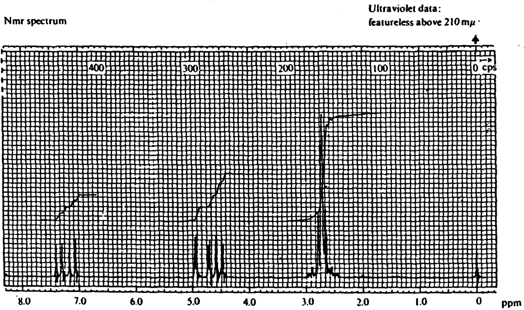
Figure 9.48. Pmr spectrum of divinyl- \beta - \beta '-thiodipropionate, conditions as figure 9.47
