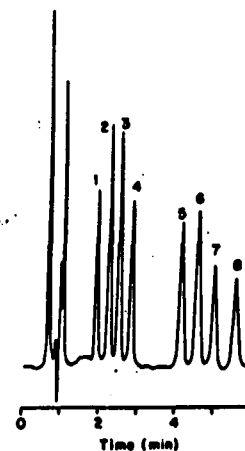
Separation of tricyclic antidepressants on a cyano-bonded silica column. Column Supelcoil LC-PCN, 5 µm, 150 mm x 4.6 mm. Eluent acetonitrile-methanol-0.01 M K 2 HPO 4 buffer, pH 7.0, 60:15:25 at 2 ml min -1 . Ultraviolet spectrophotometric detection at 215 nm. Peaks: 1, trimipramine (internal standard); 2, doxepin; 3, amitriptyline; 4, imipramine; 5, desmethyldoxepin; 6, nortriptyline; 7, desipramine; 8, protriptyline (internal standard). (Reproduced with permission of Supelco, Inc., Bellefonte, PA 16823.)
