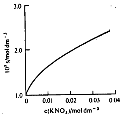
Figure 5.7. The effect of ionic strength on the solubility s of \text{BaSO}_4
