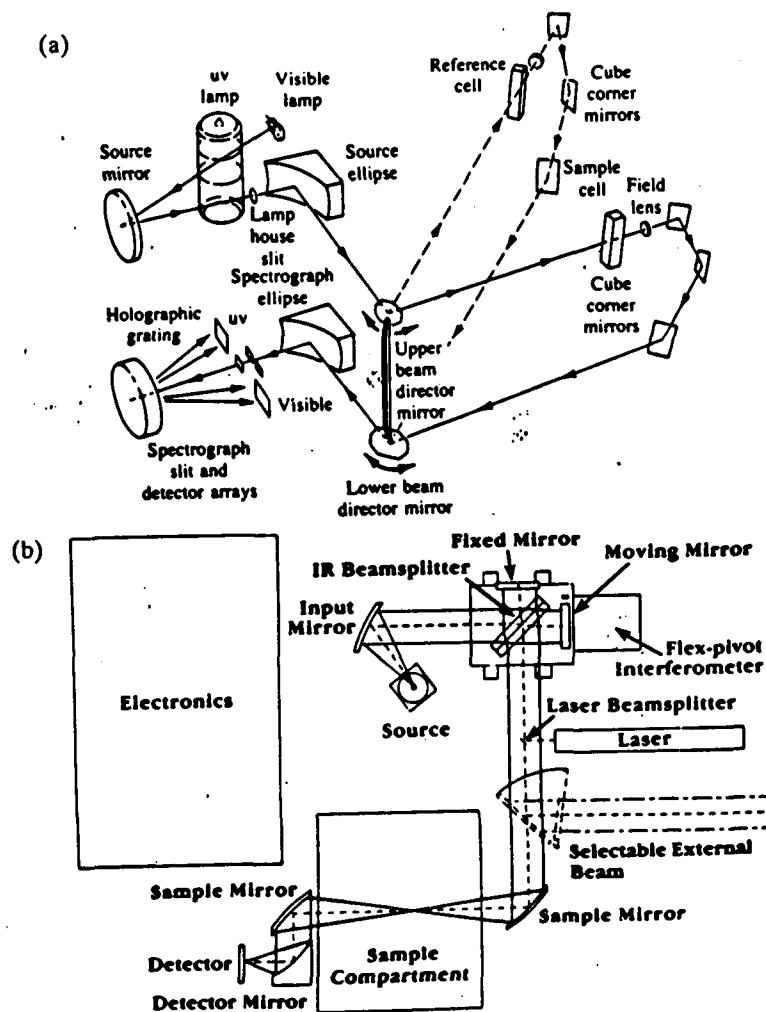
Figure 9.2. (a) UV/visible diode array spectrometer (Hewlett-Packard HP8450A) using the reversed-optics configuration (courtesy of Hewlett-Packard). (b) Fourier-transform IR spectrometer (Nicolet brochure)
