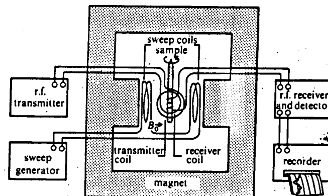
Figure 9.26. Schematic diagram of a continuous wave nmr spectrometer
