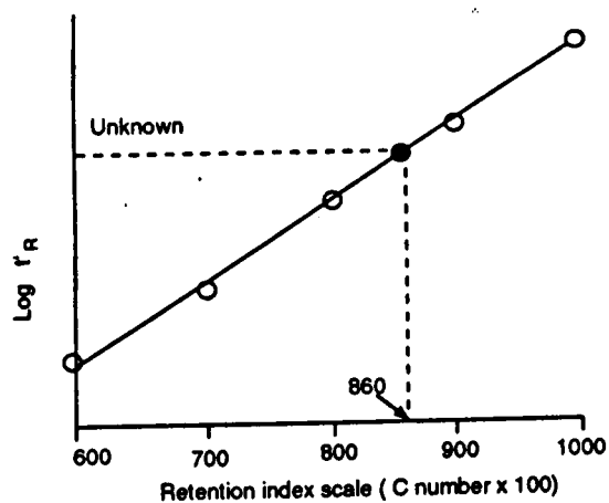
Figure 4.22. Graph of log adjusted retention times on n -alkanes compared to carbon number. The open circles show log retention times of n -alkane standards. The retention of an unknown (full circle) can be determined from the graph as shown
