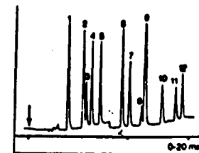
Ion-pair chromatographic separation of morphine and homologues. Column LiChrosorb RP Select B, 250 mm x 4.6 mm. Eluent: (a) methanol-0.05 M phosphate buffer, pH 3.5, 60:40 without ion-pair reagent; (b) as (a) plus 0.05 M dodecylsulfonic acid sodium salt as ion-pair counter-ion. Peaks: 1, morphine; 2, methylmorphine; 3, ethylmorphine. (Reproduced by permission of Merck, Darmstadt.)
