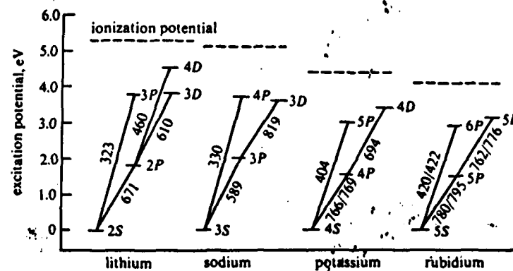
Figure 8.18. Energy level diagrams for the easily excited atomic lines of lithium, sodium, potassium and rubidium. Wavelengths are given in nanometres for the spectral lines produced by transitions between the different levels. The ionization potential is indicated by the dashed line above the respective diagrams
