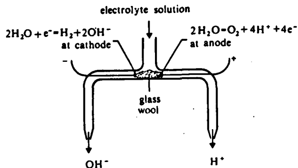
Figure 6.18. Device for external generation of H^+ and OH^-
