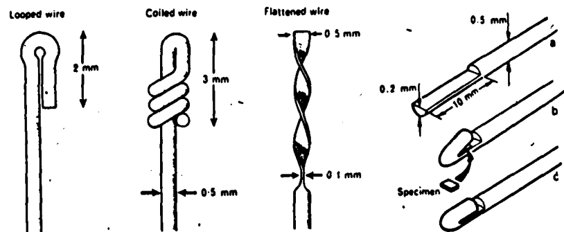
Figure 11.26. Various pyrolysis wire configurations. Reprinted from Irwin, Analytical Pyrolysis , Marcel Dekker Inc. NY (1982)
