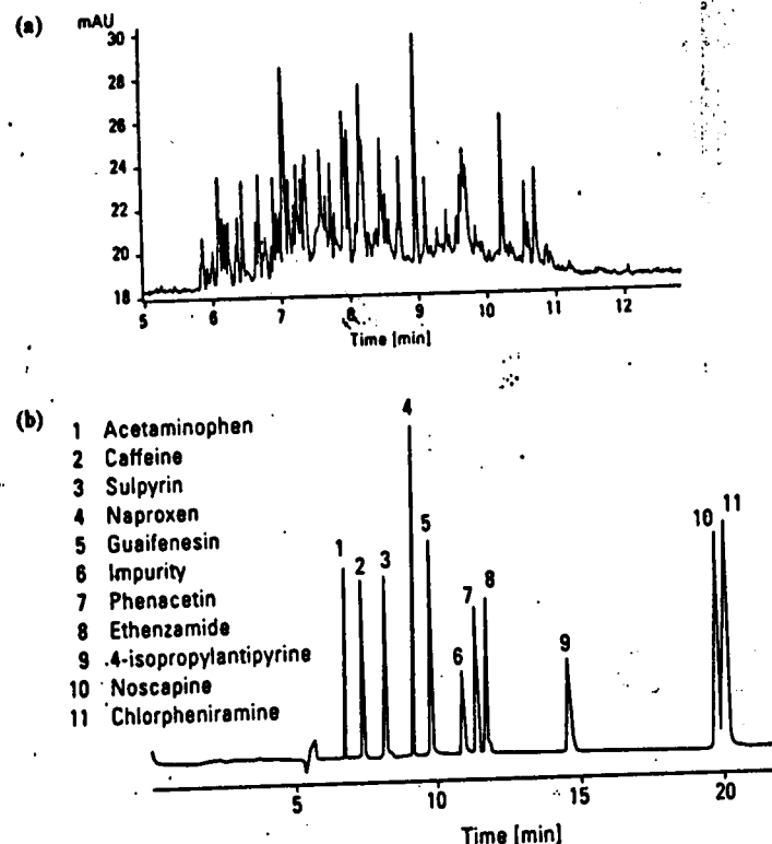
Figure 4.48. Some examples of separations by hpce. (a) CZE BSA peptide map. Conditions: 20 mM phosphate, pH 7, V = 25 kV, i = 16 \mu\text{A} , l = 50 cm, \text{id} = 50 \mu\text{m} with 3X extended pathlength detection cell, \lambda = 200 nm. (b) MECC separation of cold-relief medicine constituents. Conditions: 20 mM phosphate-borate, 100 mM SDS, pH 9, V = 20 kV, L = 65 cm, \text{i.d.} = 50 \mu\text{m} , \lambda = 210 nm. (c) CGE of 1 kbp ladder using minimally crosslinked polyacrylamide. Conditions: Bis-crosslinked polyacrylamide (3%T, 0.5%C), 100 mM Tris-borate, pH 8.3, E = 250 V/cm, i = 12.5 \mu\text{A} , l = 30 cm, L = 40 cm, \text{i.d.} = 75 \mu\text{m} , \lambda = 260 nm, polyacrylamide coated capillary. (d) CIEF of standard protein mixture. Polyacrylamide coated capillary
