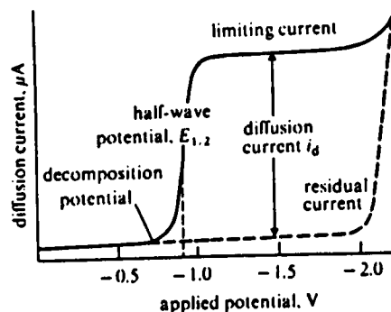
Figure 6.9. Polarographic wave or polarogram
