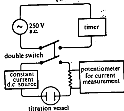
Figure 6.17. Circuit diagram for coulometric titrations
