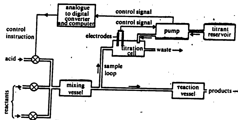
Figure 12.11. Schematic diagram of an analyser/controller for an acid catalysed reaction
