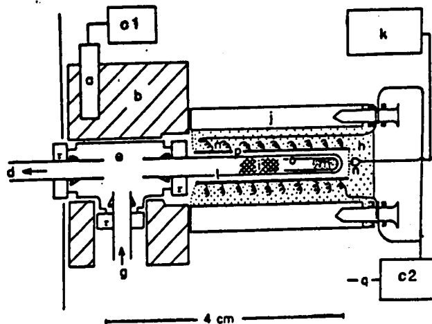
Figure 11.23. Controlled furnace-type pyrolyser: a, heater; b, Al block; c, variable transformer; d, gas outlet to column; e, Swagelok union; f, column oven; g, gas inlet; h, cement; i, glass wool plug; j, insulating block; k, pyrometer; l, stainless steel chamber; m, sample; n, heater thermocouple; o, pyrolysis tube; p, ceramic tube; q, line voltage. Reprinted from Irwin, Analytical Pyrolysis , Marcel Dekker Inc. NY (1982)
