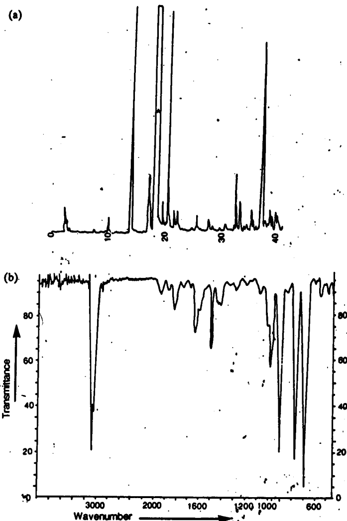
Figure 11.12. (a) Py-GC trace for polystyrene. (b) FTIR spectrum of 'peak A' identifying it as styrene (courtesy of P. J. Haines, Kingston University)
