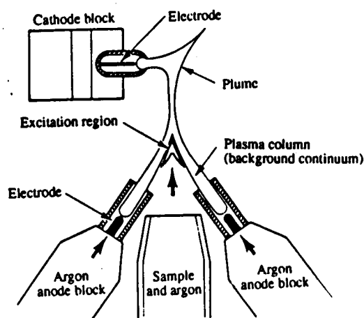
Figure 8.10. dc plasma jet
