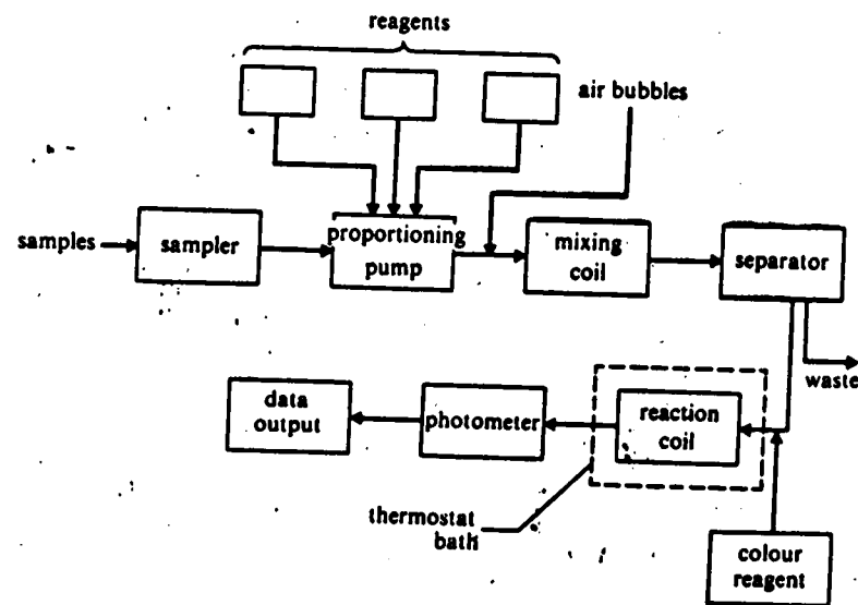
Figure 12.7. Schematic representation of an automated colorimetric analysis
