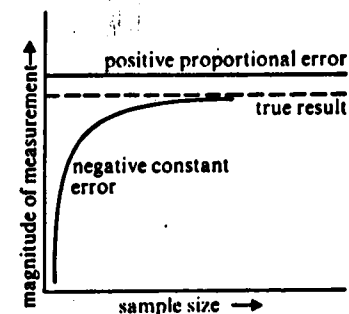
Figure 2.1. The effects of constant and proportional errors on a measurement of concentration
