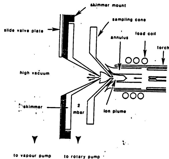
Figure 8.15. Cross-section of typical ICP ion source showing plasma torch and ion extraction interface. Extraction and skimmer sizes are slightly exaggerated for clarity
