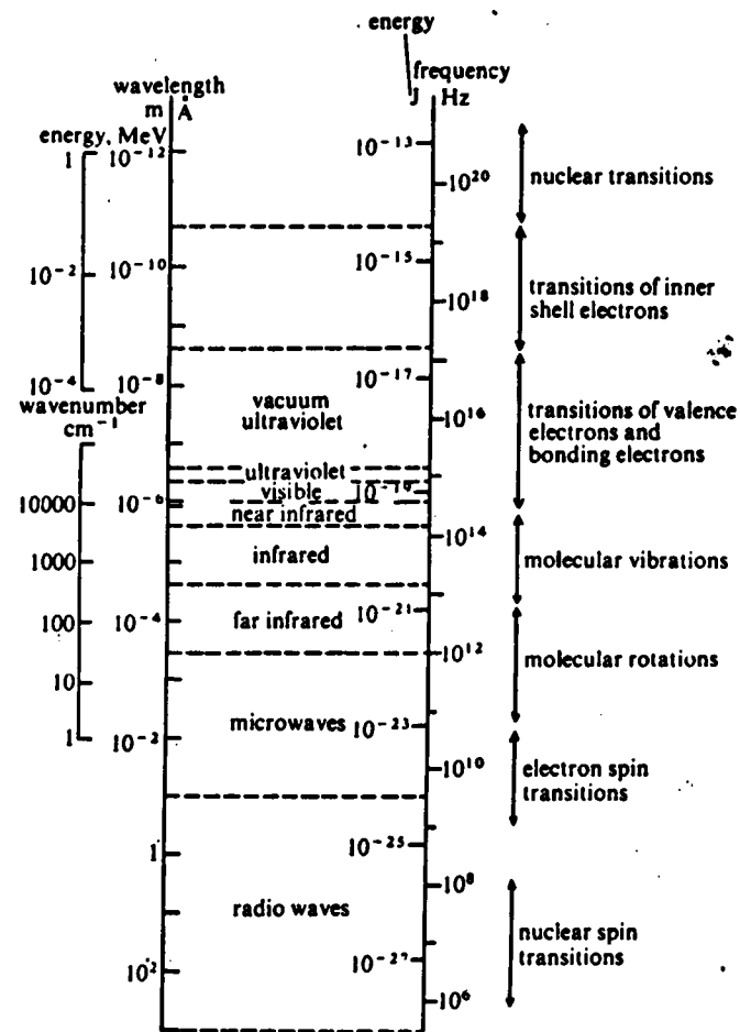
Figure 7.2. The electromagnetic spectrum
