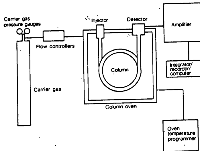
Figure 4.13. Schematic diagram of a gas chromatograph (from R. M. Smith, Gas and Liquid Chromatography in Analytical Chemistry , Wiley, 1988)
