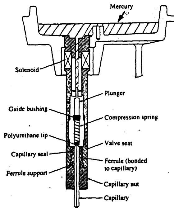
Figure 6.10. Dropping mercury electrode
