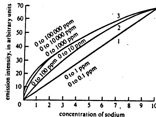
Figure 8.20. Emission intensity of sodium in the acetylene-oxygen flame at 589 nm showing the effect of self-absorption on calibration curves
