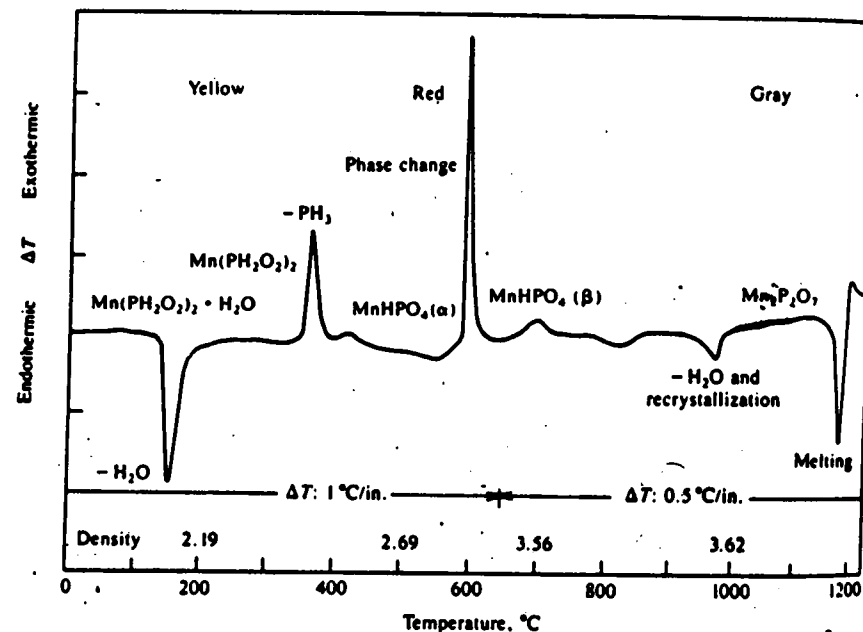
Figure 11.11. DTA curve for \text{Mn}(\text{PH}_2\text{O}_2)\cdot\text{H}_2\text{O}
