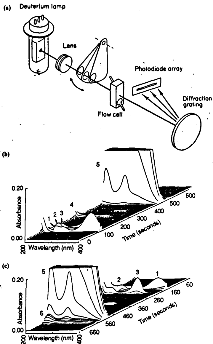
Figure 4.29. (a) Optical path in a UV photodiode array detector. (b and c). Three-dimensional display from UV diode array detector; azathioprine and impurities separated by reversed-phase (RP) HPLC with HP 1040A detector coupled to an HP 85 microcomputer: (b) isometric projection of data showing components 1-5; (c) reversed projection of data showing components 1-6. Key: (1) 1-methyl-4-nitro-5-hydroxyimidazole; (2) 1-methyl-4-nitro-5-thioimidazole; (3) 6-mercaptopurine; (4) 1-methyl-4-nitro-5-chloroimidazole; (5) azathioprine; (6) process impurity
