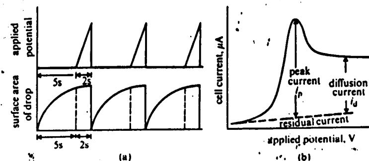
Figure 6.11. Oscillographic polarography. (a) Variation of drop area and applied potential with time. (b) Oscillographic display of a polarogram
