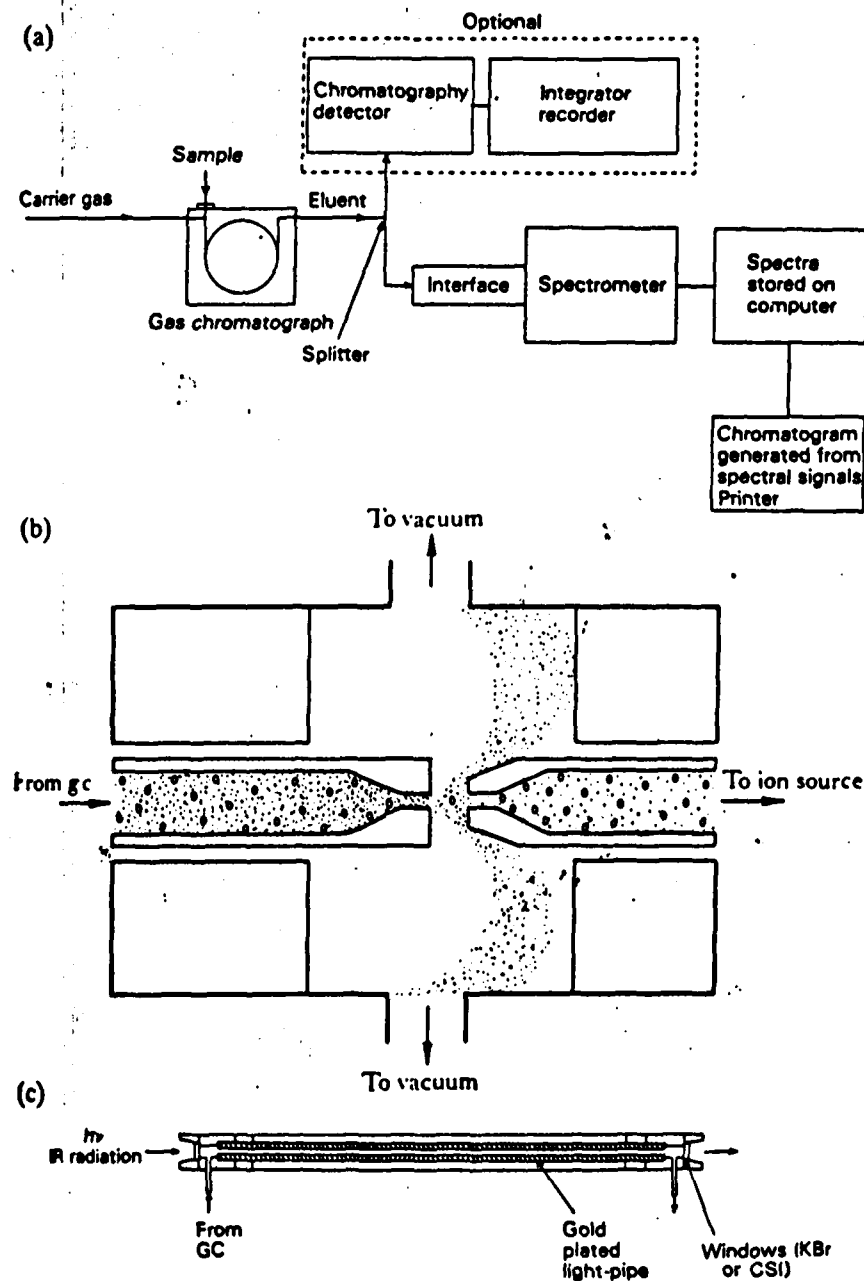
Figure 4.24. (a) GC-spectrometer system. (b) Jet-orifice separator for GC-MS. (c) Flow-through light pipe cell for GC-IR
