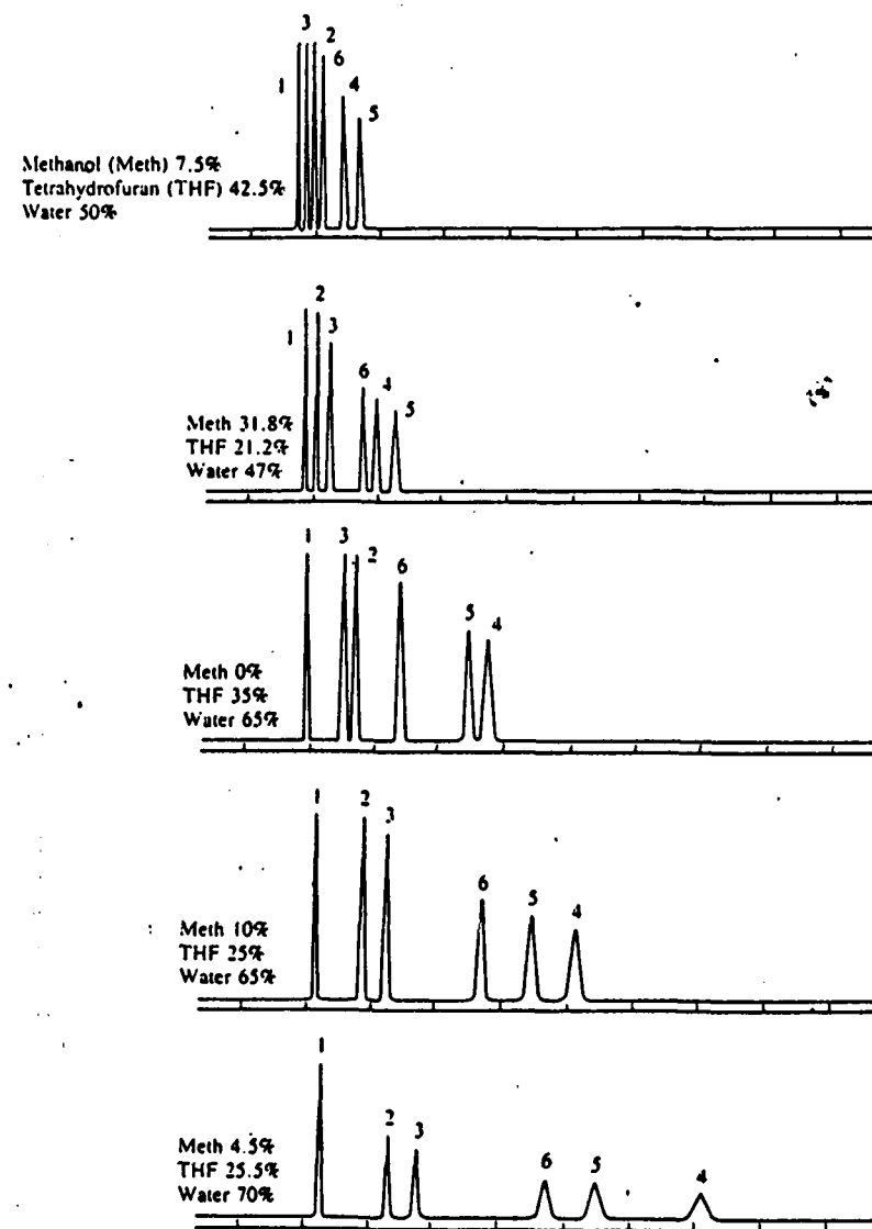
Figure 4.34. Optimizing an hplc separation using five ternary mobile phases. Peaks: (1) benzyl alcohol, (2) phenol, (3) 3-phenylpropanol, (4) 2,4-dimethylphenol, (5) benzene, and (6) diethyl o -phthalate. (After R. D. Conlon, 'The Perkin-Elmer Solvent Optimization System,' Instrumentation Research , p. 95 (March 1985). Courtesy of Instrumentation Research.)
