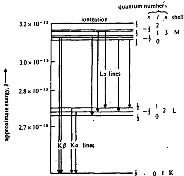
Figure 8.31. X-ray transitions in the molybdenum atom. Lines are designated by the letter referring to the lower quantum group and \alpha where \Delta n = -1 and \beta where \Delta n = -2
