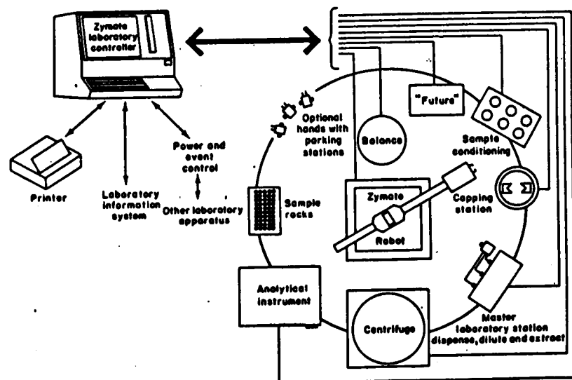
Figure 12.12. Robot arm system for sample preparation with different workstations (reproduced by permission of Zymark Corporation)
