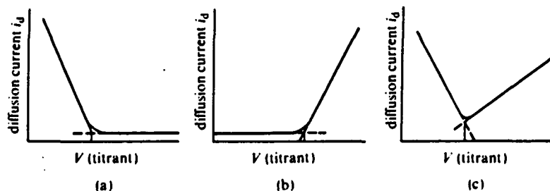
Figure 6.15. Amperometric titration curves. (a) Only substance titrated is reducible, e.g. \text{Pb}^{2+} against \text{SO}_4^{2-} , \text{Ag}^+ against halide. (b) Only titrant is reducible, e.g. \text{SO}_4^{2-} against \text{Pb}^{2+} , \text{Na}_2\text{S}_2\text{O}_3 against \text{I}_2 . (c) Both reducible, e.g. \text{Pb}^{2+} against \text{CrO}_4^{2-} , \text{Cu}^{2+} against \alpha -benzoin oxime
