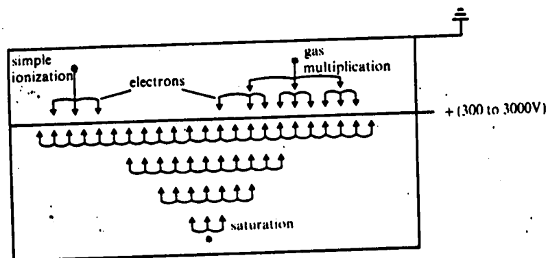
Figure 10.7. Radiation induced ionization in an argon filled detector
