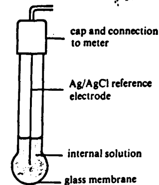
Figure 6.2. Glass electrode
