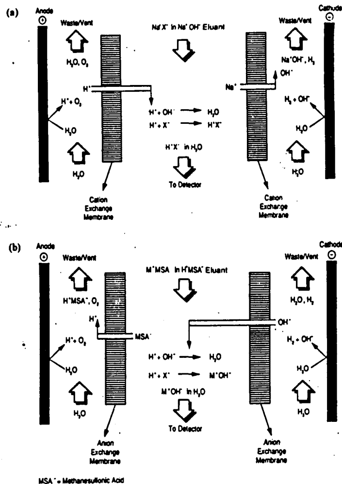
Figure 4.39. Self-regenerating suppressor cartridge incorporating an electrolysis cell. (a) For anionic analytes. (b) For cationic analytes
