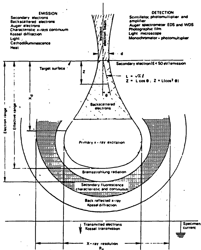
Figure 8.28. Diagram showing the effects of the interaction of an electron beam with a solid specimen.
