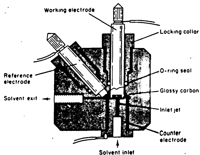
Figure 4.32. 'Wall-jet' amperometric detector
