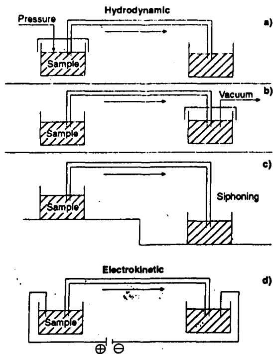
Figure 4.47. Methods of sample injection for capillary electrophoresis
