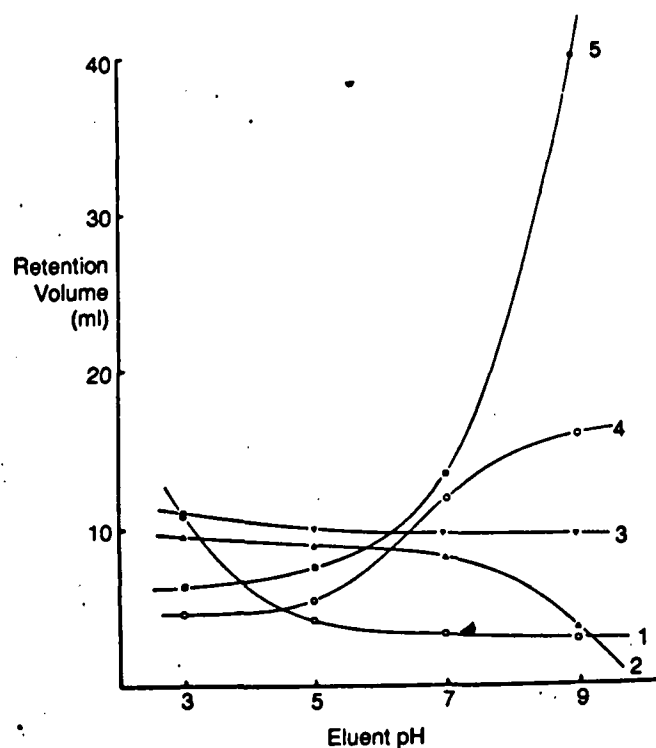
Figure 4.37. Effect of eluent pH on selectivity in reverse-phase BPC. Column, 30 \times 0.4 cm, \mu -Bondapak-C 18 , 10 \mu\text{m} ; mobile phase, 0.025 \text{ M NaH}_2\text{PO}_4 - \text{Na}_2\text{HPO}_4 with 40% v methanol; flowrate, 2 ml/min; temp., ambient; detector, UV, 220 nm; samples, 1-10 \mu\text{g} . (1) Salicylic acid; (2) phenobarbitone; (3) phenacetin; (4) nicotine; (5) methylamphetamine
