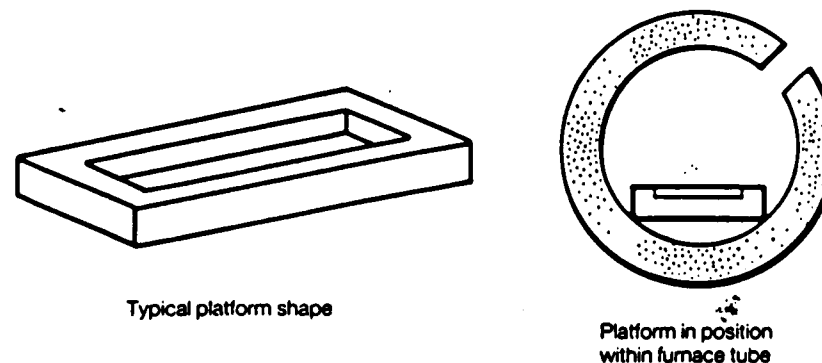
Figure 8.26. Platform shape and orientation within a furnace tube
