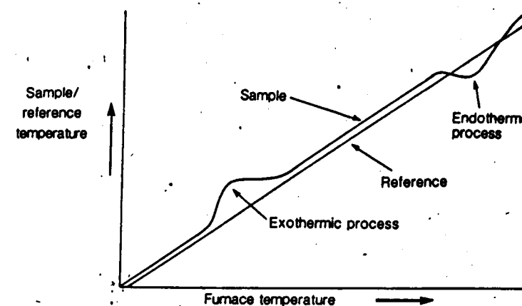
Figure 11.7. Schematic representation of the variation of sample and reference temperature in DTA
