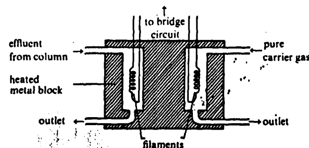
Figure 4.15. Thermal conductivity detector (tcd)
