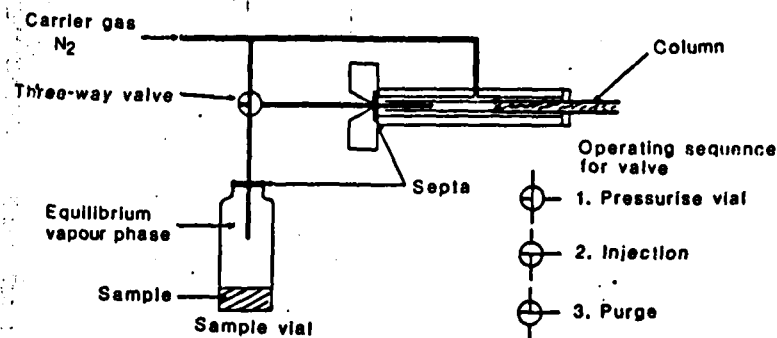
Figure 4.20. Headspace sample injection system (positioned in a heated oven)
