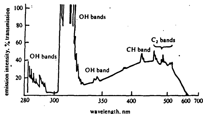
Figure 8.19. Flame background spectrum of an acetylene-oxygen flame containing an organic aerosol
