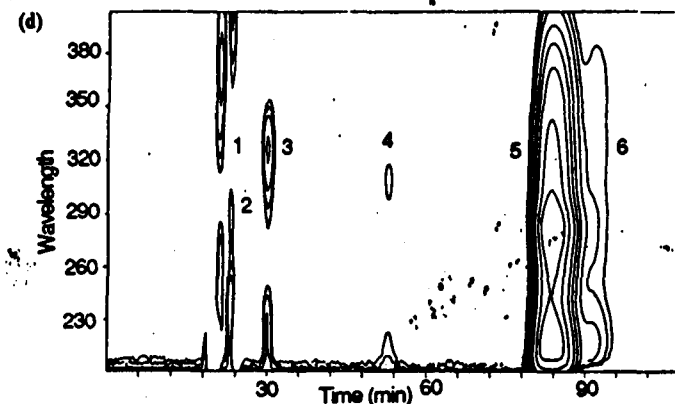
Figure 4.29(d). Contour plot of data for azathioprine and impurities in (b) and (c), showing the isoabsorbance contours (from 1 000 to 5 m AU) plotted in the wavelength-time plane. Key to the peaks, as in (b) and (c)
