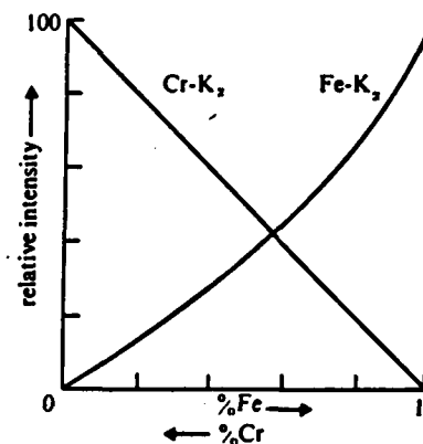
Figure 8.34. Analytical curves for the determination of iron and chromium in a mixture of the two
