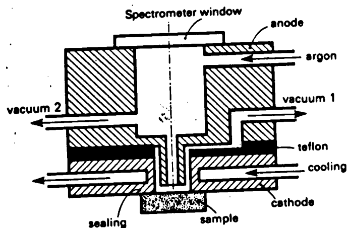
Figure 8.8. Glow discharge lamp (with permission from Jobin-Yvon)
