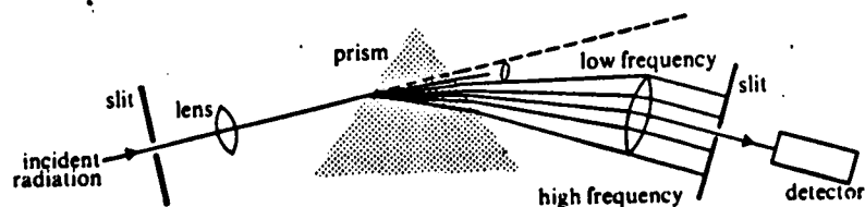
Figure 7.6. Dispersion of radiation by a prism monochromator
