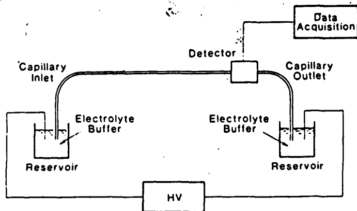
Figure 4.46. Schematic diagram of a capillary electrophoresis system
