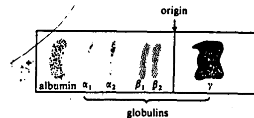
Figure 4.45. Electropherogram of blood serum on cellulose acetate. (Buffer: 0.50 M barbitone, pH = 8.6)
