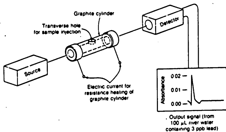
Figure 8.25. Graphite furnace for atomic absorption analysis and typical output signal
