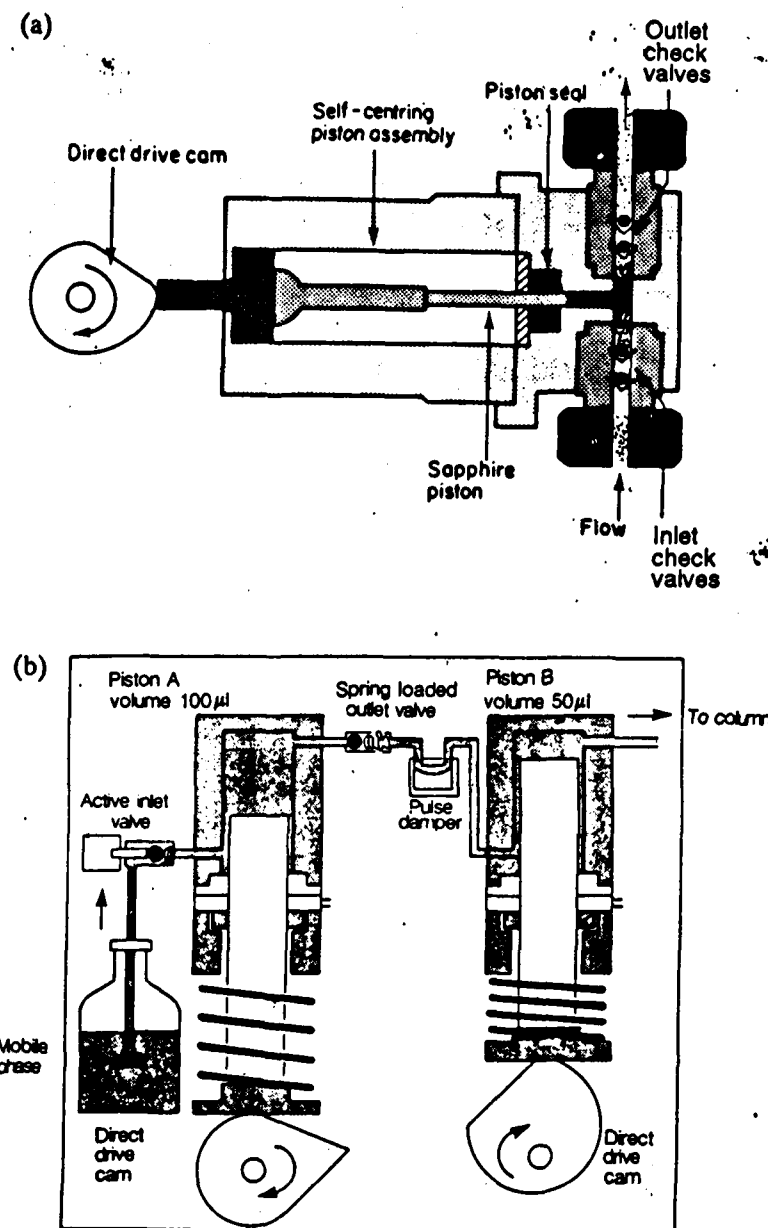
Figure 4.26. (a) Single-head reciprocating pump (Reproduced by permission of Gilson Medical Electronics, Inc.). (b) Double-head 'in-series' reciprocating pump
