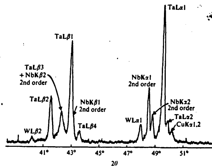
Figure 8.38. X-ray spectra of niobium and tantalum
