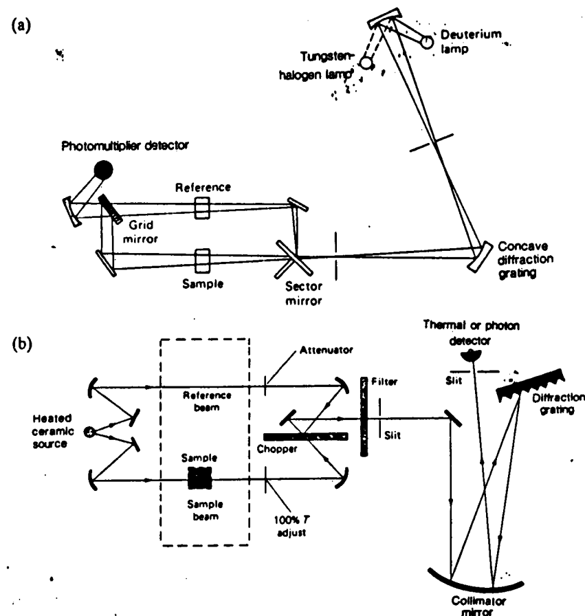
Figure 9.1. (a) Double-beam recording UV/visible spectrophotometer. (b) Double-beam recording IR spectrophotometer (courtesy of Beckman Instruments, Inc., Fullerton, California)
