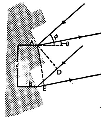
Figure 7.7. Operating principle of a diffraction grating. \phi is the angle of incidence; d is the groove spacing; \theta is the angle of reflection
