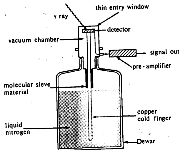
Figure 10.14. Construction of a 'dipstick' type semiconductor detector system
