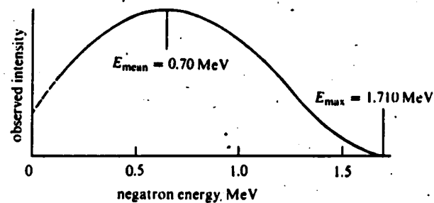
Figure 10.3. Energy spectrum of ^{32}\text{P} negatrons
