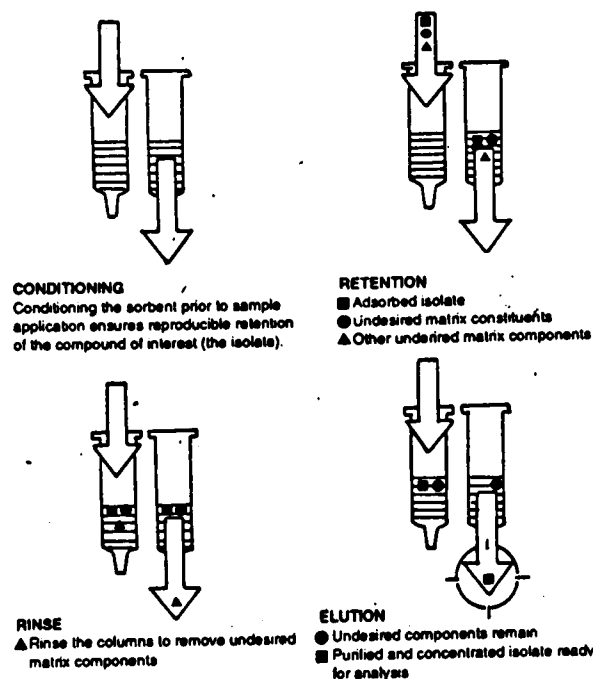
Figure 12.3. Principle of solid phase extraction
