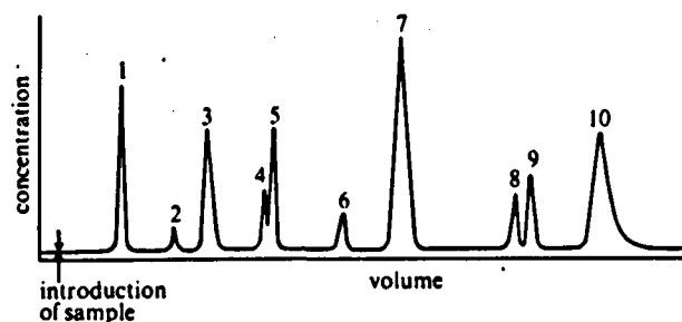
Figure 4.12. A typical elution profile; the separation of aliphatic esters by gas-liquid chromatography
