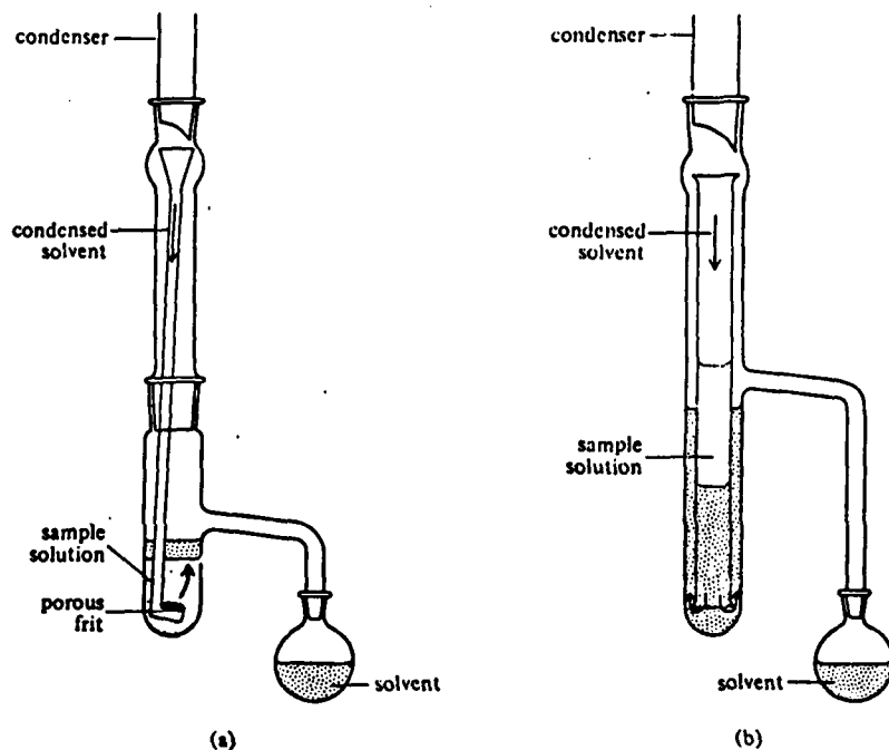
Figure 4.3. Continuous extraction apparatus. (a) Extraction with a solvent lighter than water. (b) Extraction with a solvent heavier than water
