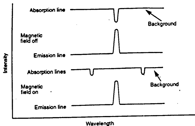
Figure 8.23. Zeeman effect splitting of atomic absorption lines. (Redrawn from Concepts Instrumentation and Techniques in Atomic Absorption Spectrophotometry (R. D. Beaty and J. D. Kerber). Perkin-Elmer, Norwalk, Connecticut, USA)
