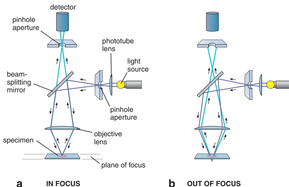
FIGURE 1.11 ▲ Diagram of the in-focus and out-of-focus emitted light in the confocal microscope.
