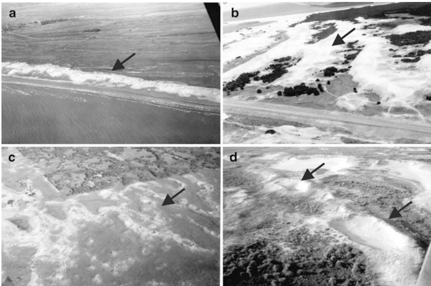
Fig. 19.3 Examples of aeolian landforms in coastal zones. (a) Foredune, (b) Transverse ridges. (c) Parabolic with blowouts sobreimposed. (d) Blowouts
