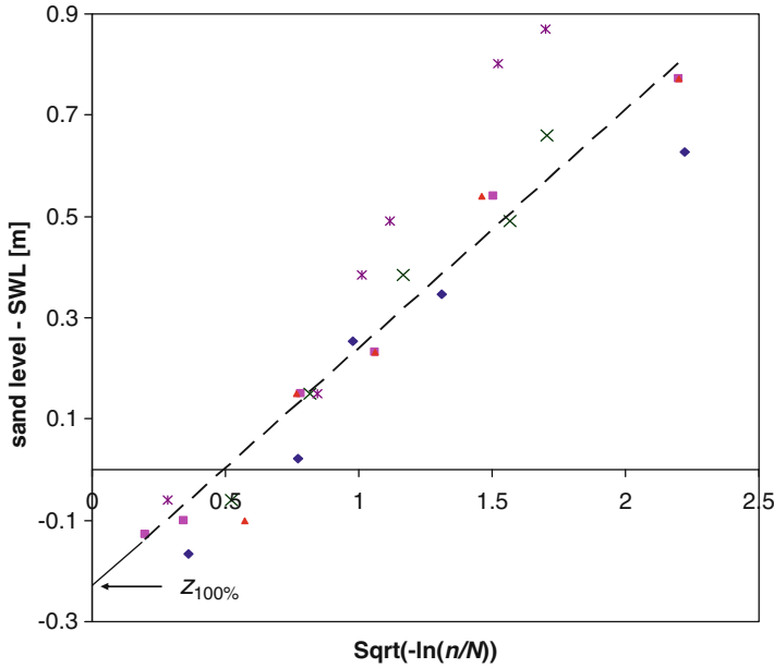
Fig. 22.30 Rayleigh plots of 5 sets of runup data from Moreton Island, 10–11 Dec 2007. H_{orms} = 0.9 m, T_z = 5.6 s, \tan\beta_F = 0.08 . The trend line corresponds to the data marked \blacksquare . Z_{100\%} is the highest level transgressed by all waves according to the best fit Rayleigh distribution. After Nielsen (2009a)
