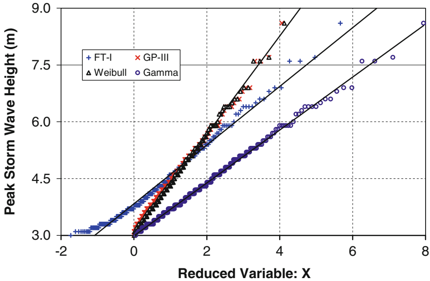
Fig. 22.16 The parameters of the two-parameter FT-I and three-parameter Weibull, GP-III and Pearson-III distributions are estimated with the least-squares method (You 2012)
