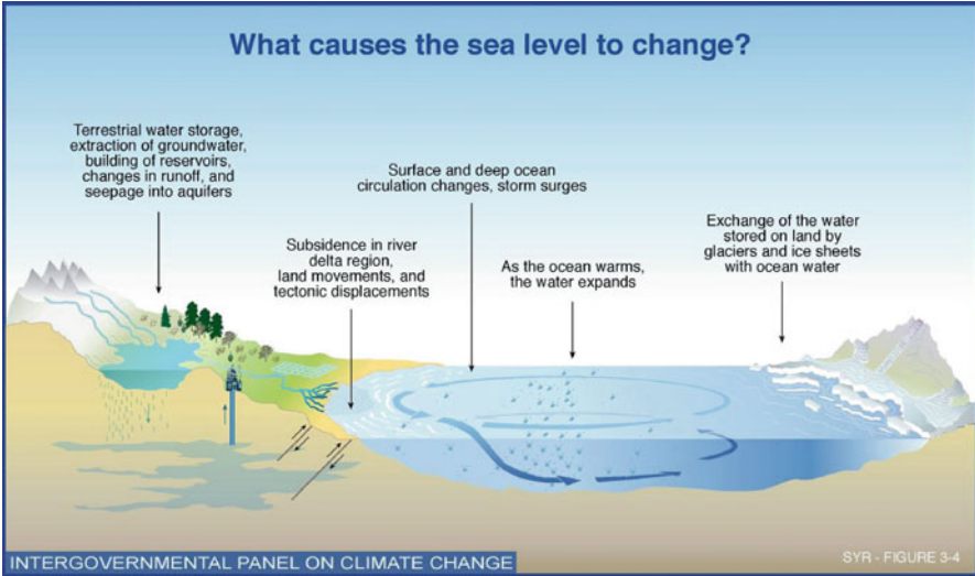
Fig. 10.1 Contributors to relative sea level change (Interagency Panel on Climate Change)
