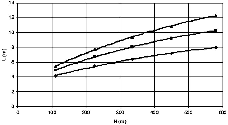
Fig. 12.6 The horizontal brine jet length L as a function of seawater depth H for three values of nozzle diameter ratio, d_{nozzle}/d_X (▲-0.2; ■-0.25; ◆- 0.33)
