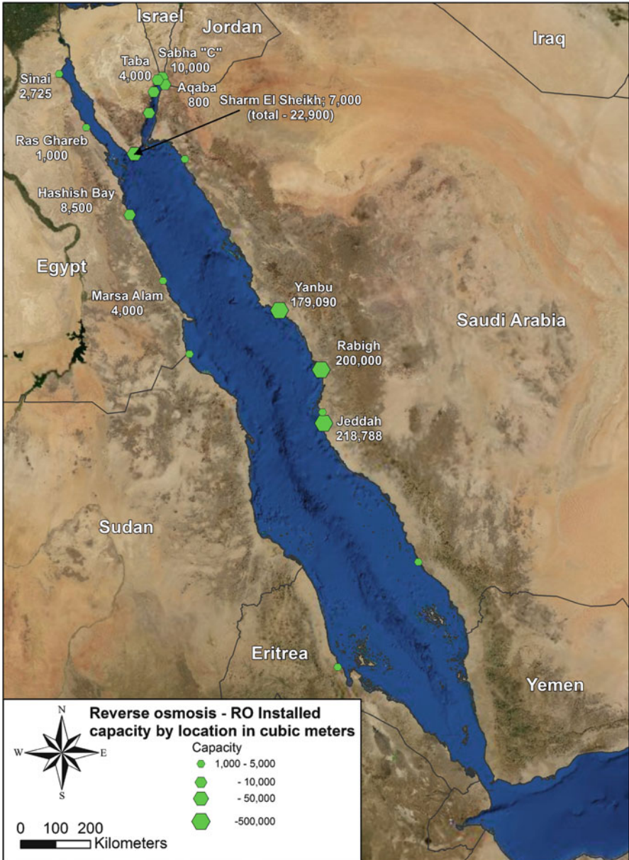
Fig. 12.2 Several RO desalination plants on Red Sea coast (El-Sadek 2010; Lattemann and Höpner 2008; Mohsen 2007; Khalil 2004; Semiat 2001) (Source of background: Esri, i-cubed, USDA, USGS, AEX, GeoEye, Getmapping, Aerogrid, IGN, IGP, and the GIS User Community)
