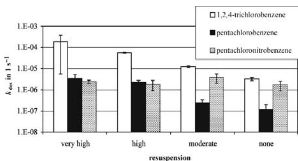
Fig. 6.16. Effect of hydrodynamic conditions on the desorption rate constant, k_{des}
