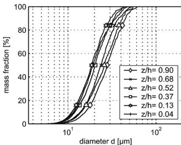
Fig. 3.16. Distribution of floc size of kaoline over depth at t = 240 min with a mean concentration of 500 \text{ mg l}^{-1}
