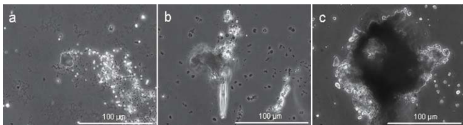
Fig. 3.21. Phase contrast micrographs of sediment particles eroded at different shear stress ( a 0.50 \text{ N m}^{-2} ; b 1.00 \text{ N m}^{-2} ; c 1.25 \text{ N m}^{-2} ) from sediments of the river Neckar
