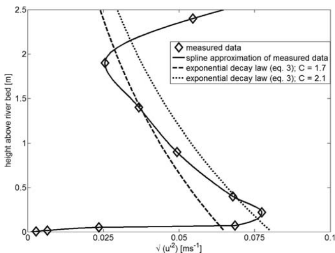
Fig. 3.8. Representative results for depth-dependent flow turbulence obtained with a lowered Single-Point-ADV system (same location and time as data from Fig. 3.7)
