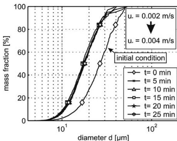
Fig. 3.17. Segregation of kaoline flocs with a mean concentration of 500 \text{ mg l}^{-1} by doubling the turbulent intensity at z/h = 0.68
