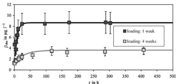
Fig. 6.17. Influence of the HOC/sediment preloading contact time on the desorption process of 1,2,4-trichlorobenzene in a moderately resuspended system
