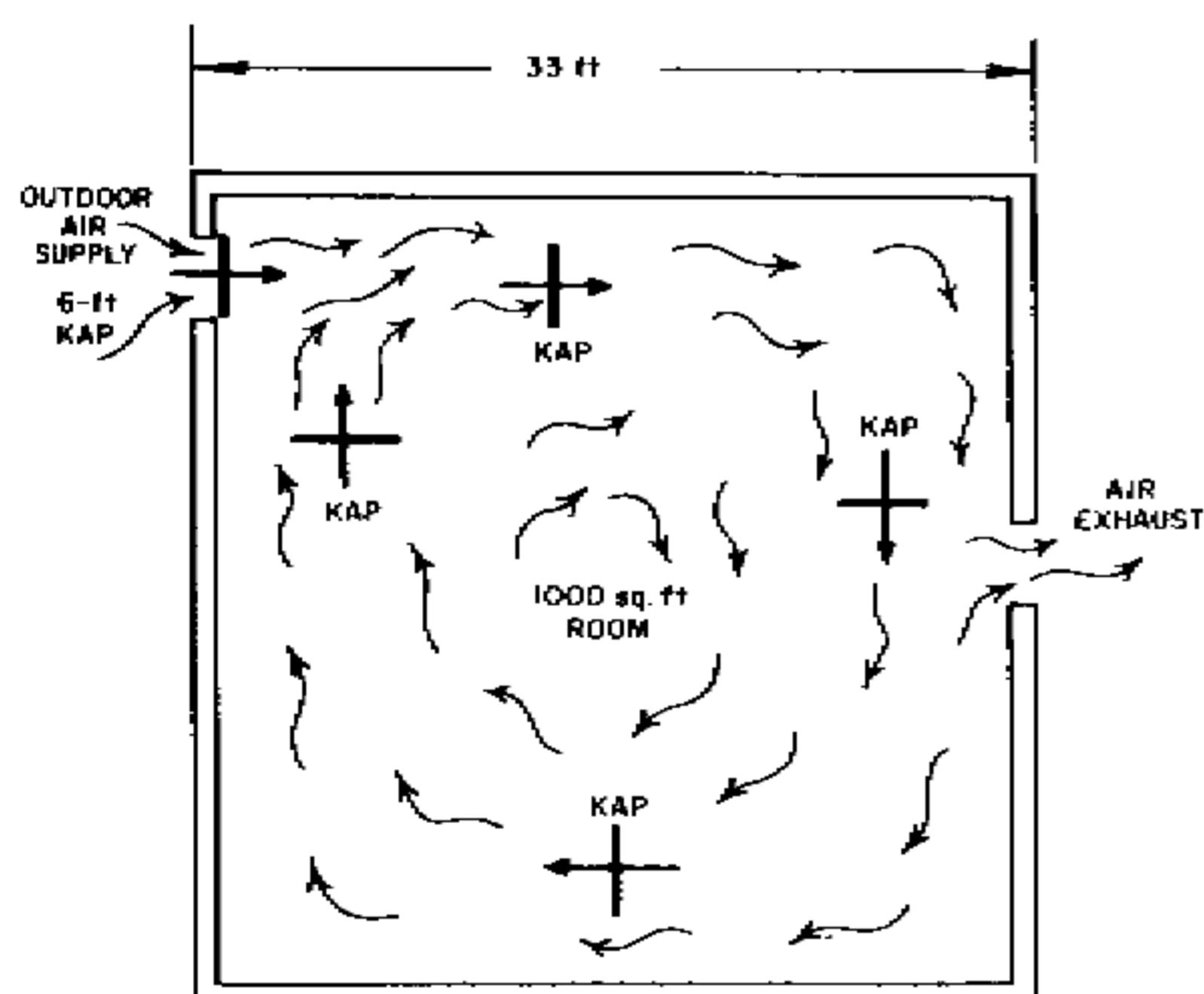
Fig. 16. The use of air-distribution KAPs.
