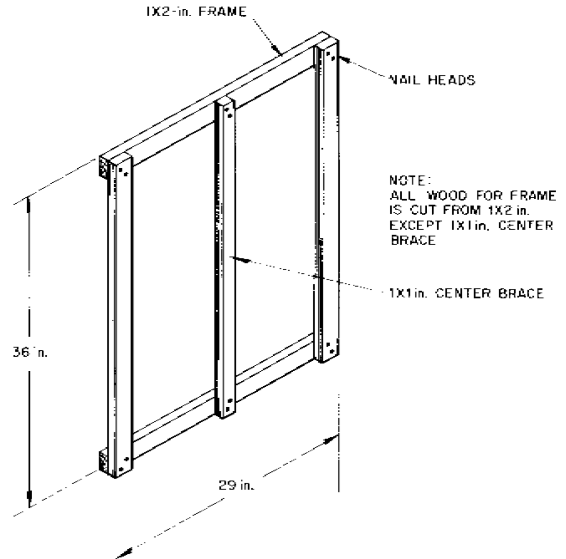
Fig. 3. KAP frame (looking at the back side of the frame).
