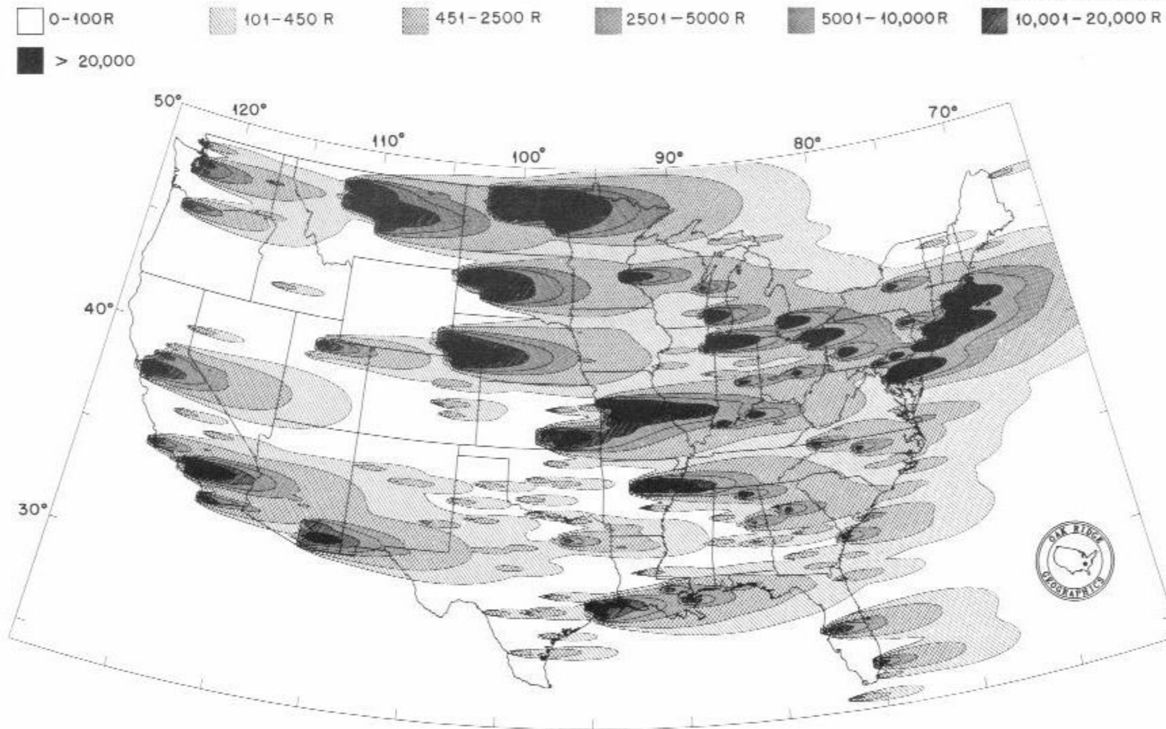
Fig. 4.2. Simplified, outdated fallout patterns showing total radiation doses that would be received by persons on the surface and in the open for the entire 14 days following the surface bursting of 5050 megatons on the targets indicated, if the winds at all elevations blew continuously from the west at 25 mph.
