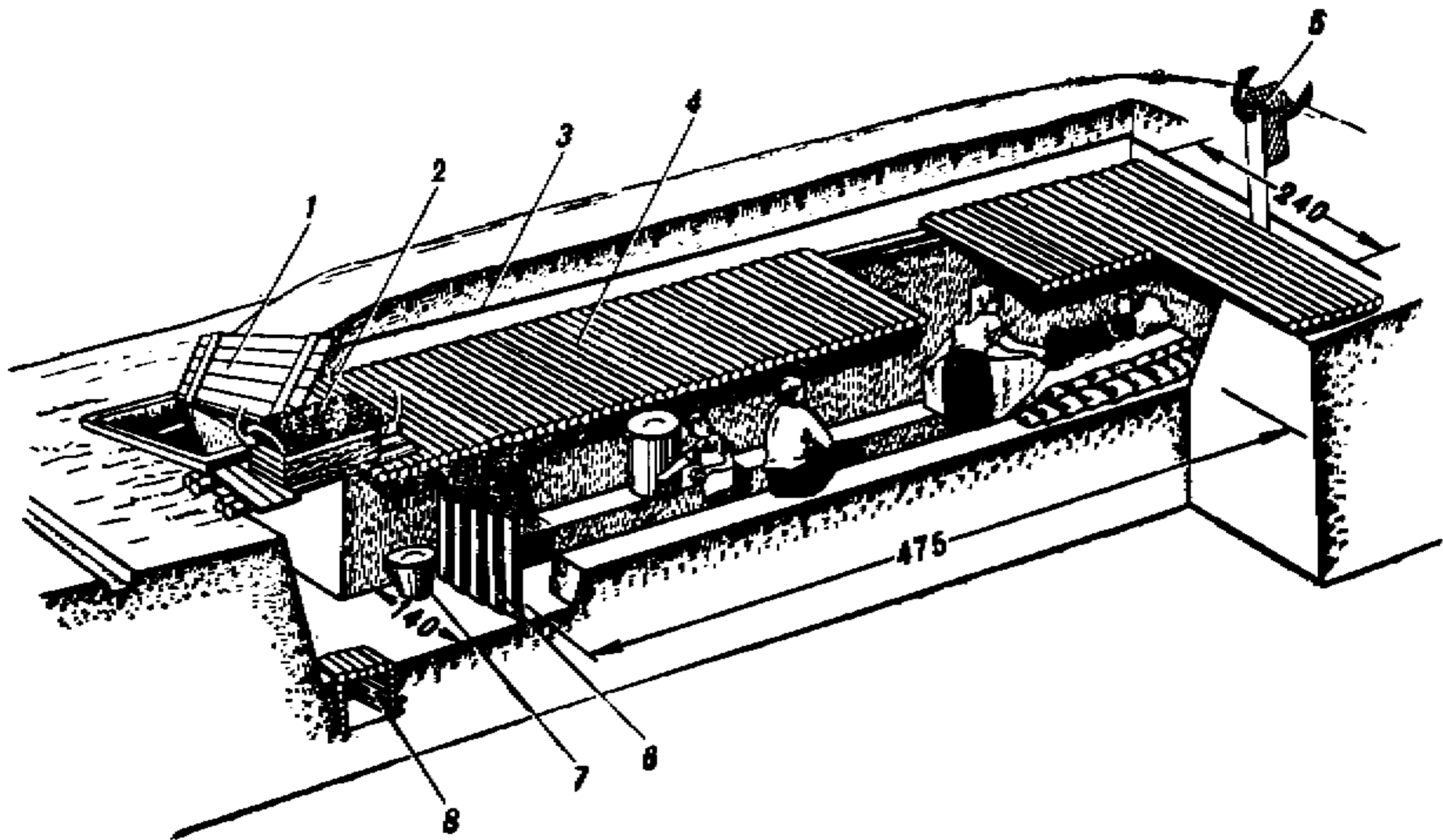
Fig. 6.5. Figure 20. Wood-Earth Shelter without Lining of the Walls for Clay Soils, 10 Occupants: 1 - Trap Door; 2 - Dust Filter with a Straw Packing (hay); 3 - Earth Cover 60-80 cm thick; 4 - Roofing made of Poles; 5 - Exhaust Duct with Damper; 6 - Curtain made of Tightly Woven Cloth; 7 - Removable Container for Wastes; 8 - Water Collecting Sump.
