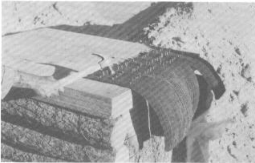
Fig. D.15. Tire-strip hinges nailed to an expedient, 4-inch-thick blast door made of plywood, designed to withstand 50-psi blast effects of very large weapons and undamaged by blast at the 53-psi range.
