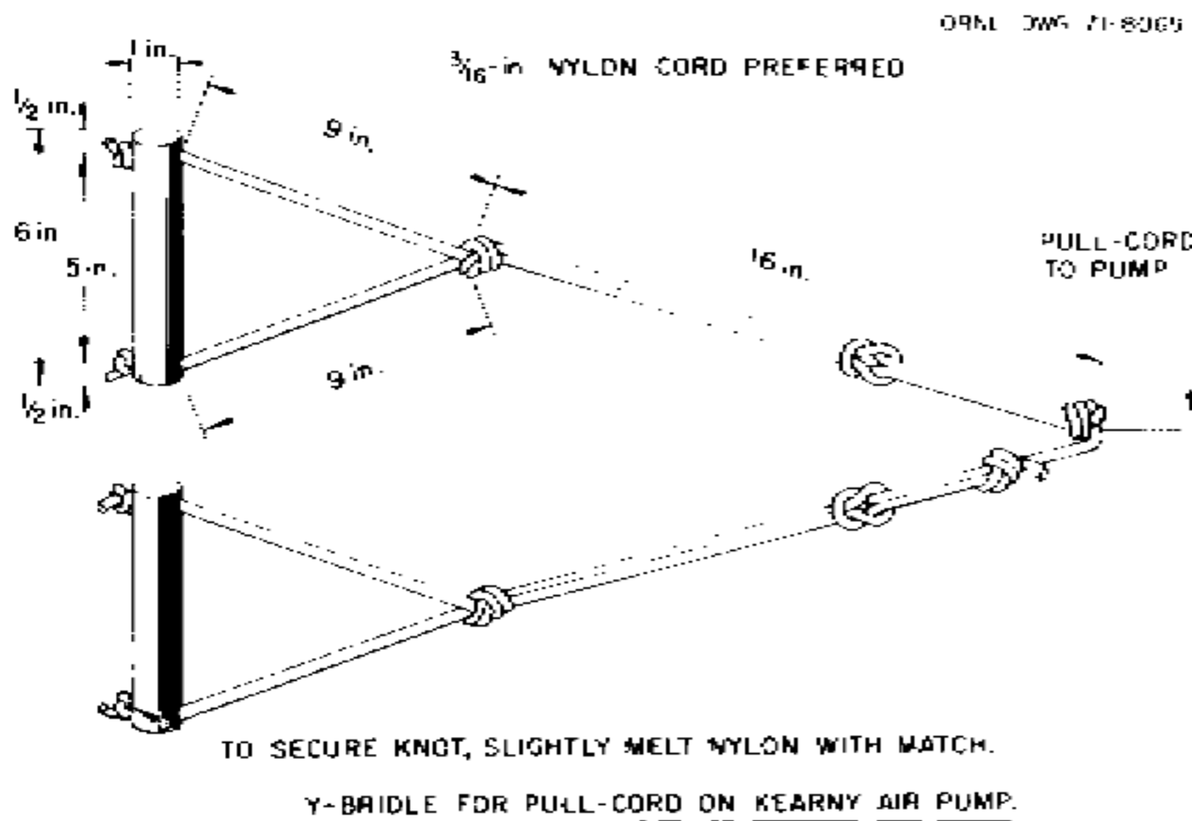
Fig. 23. Y-bridle for pull-cord on KAP.
