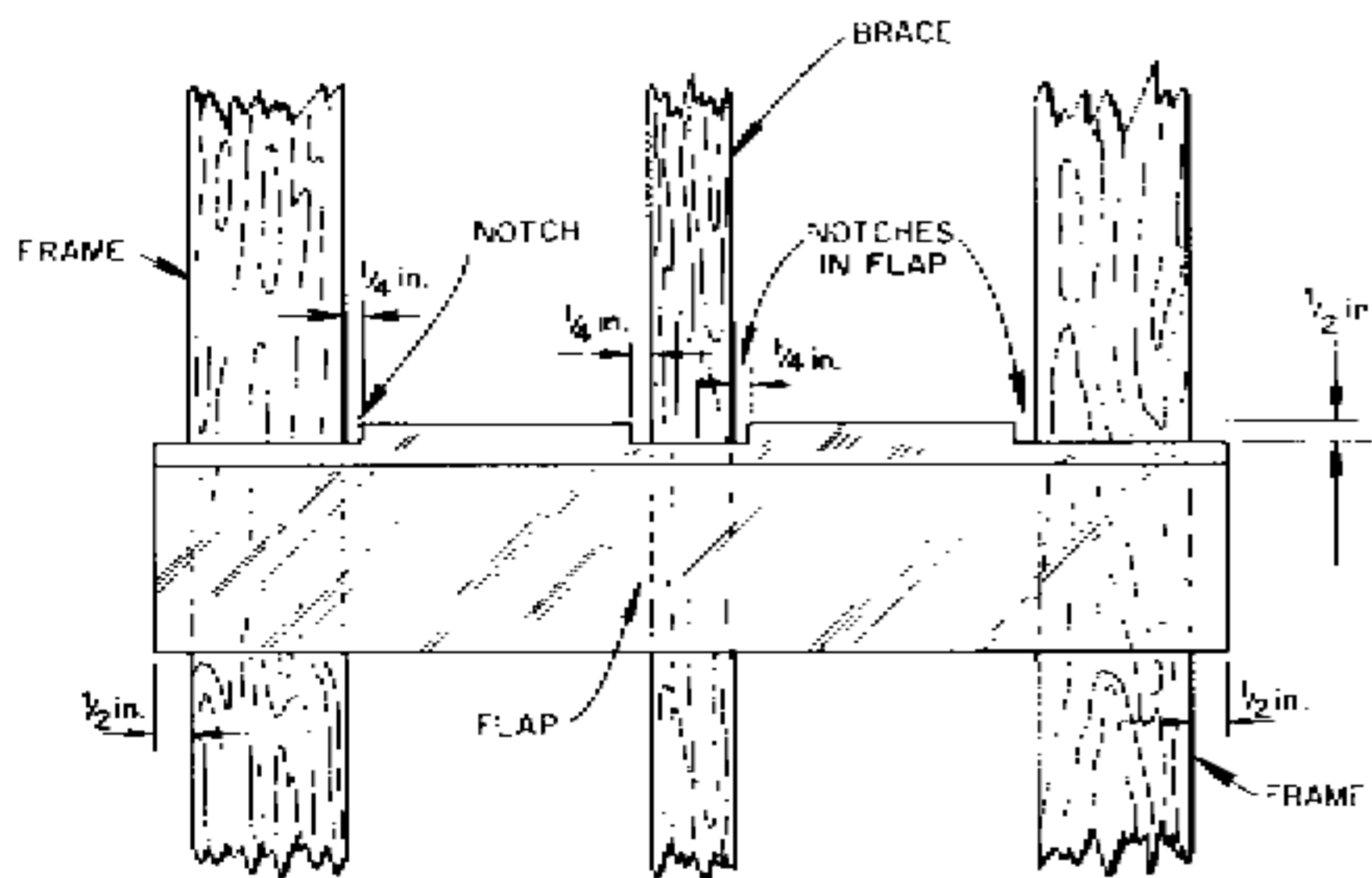
Fig. 6. Sizes of notches in flaps.
