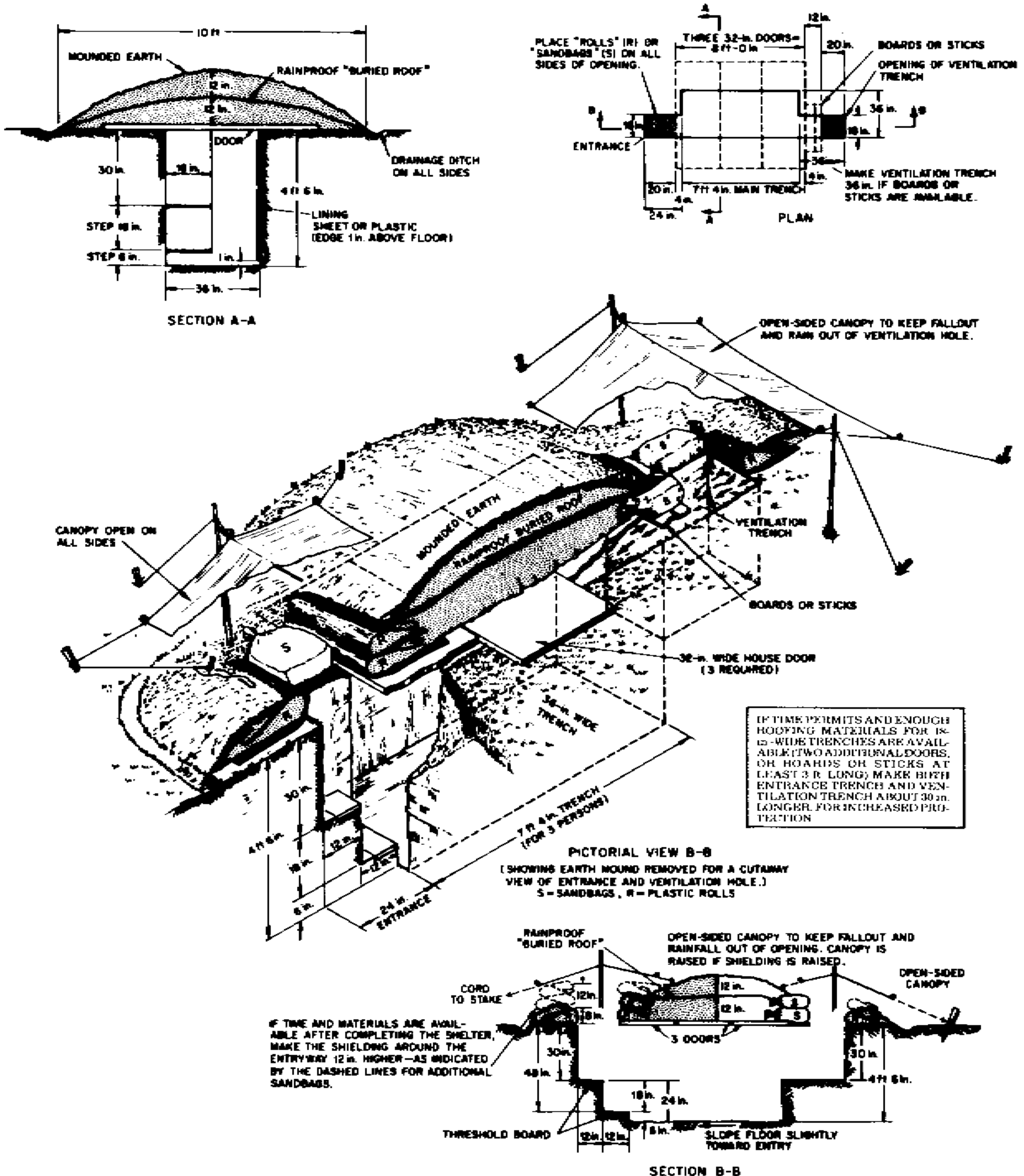
Fig. A.1. Door-Covered Trench Shelter.
