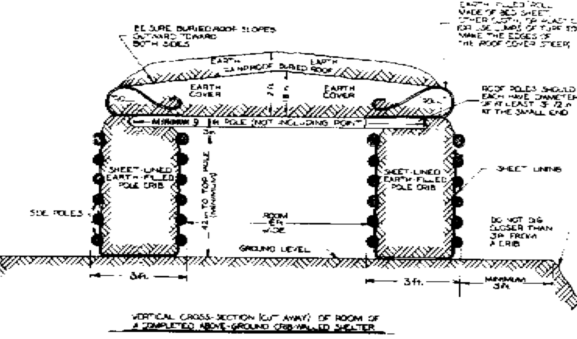
Fig. A.6. Aboveground, Crib-Walled Shelter.
