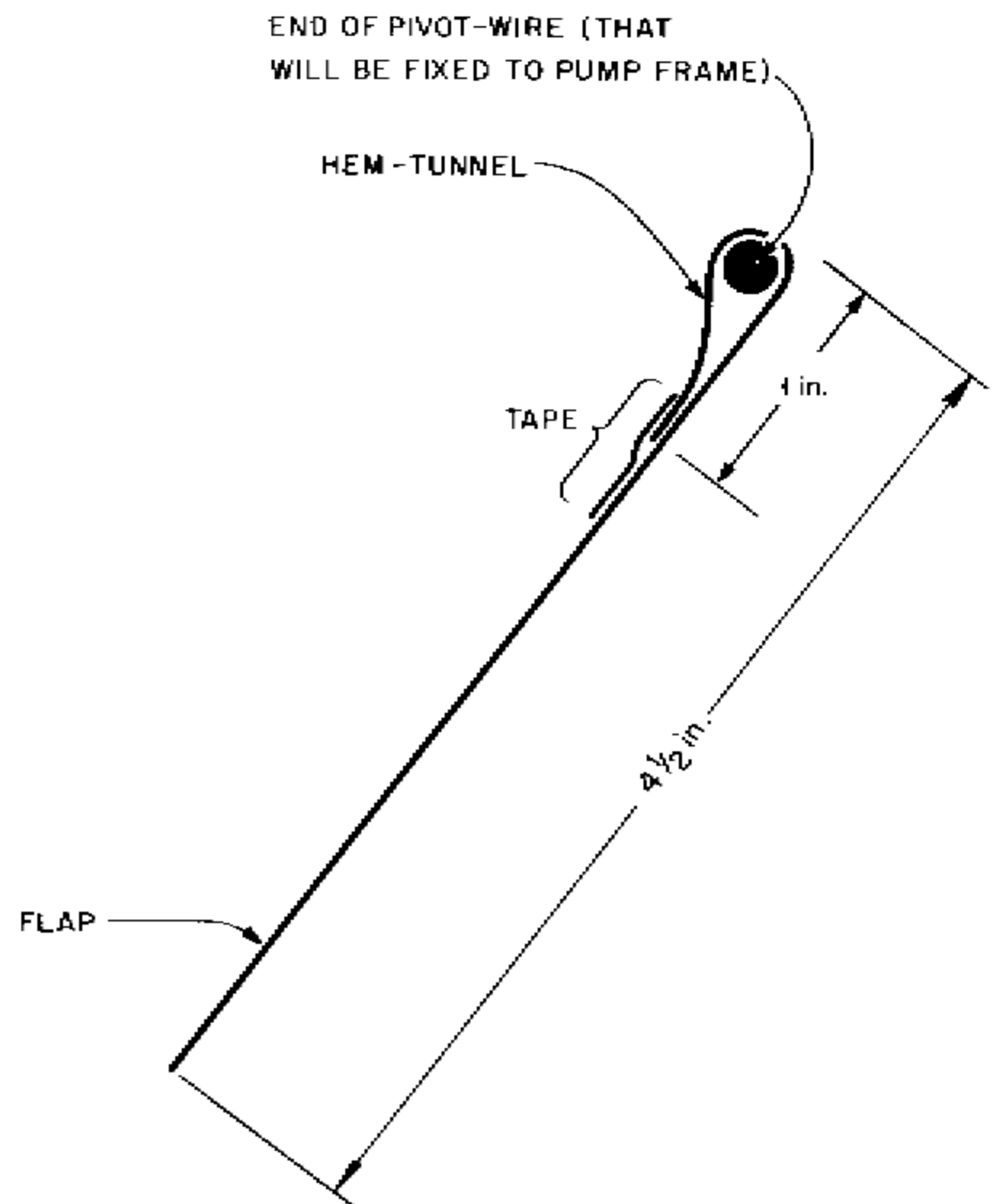
Fig. 7. End view.
