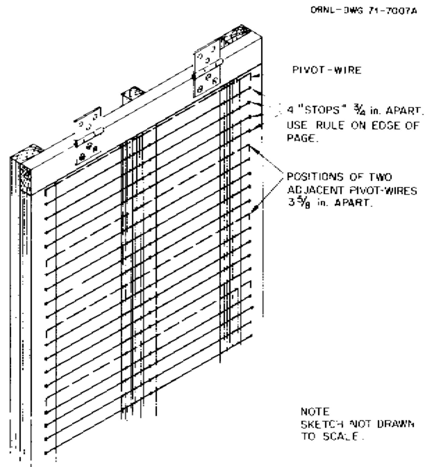
Fig. 11. Positions of pivot-wires and flap-stops.
