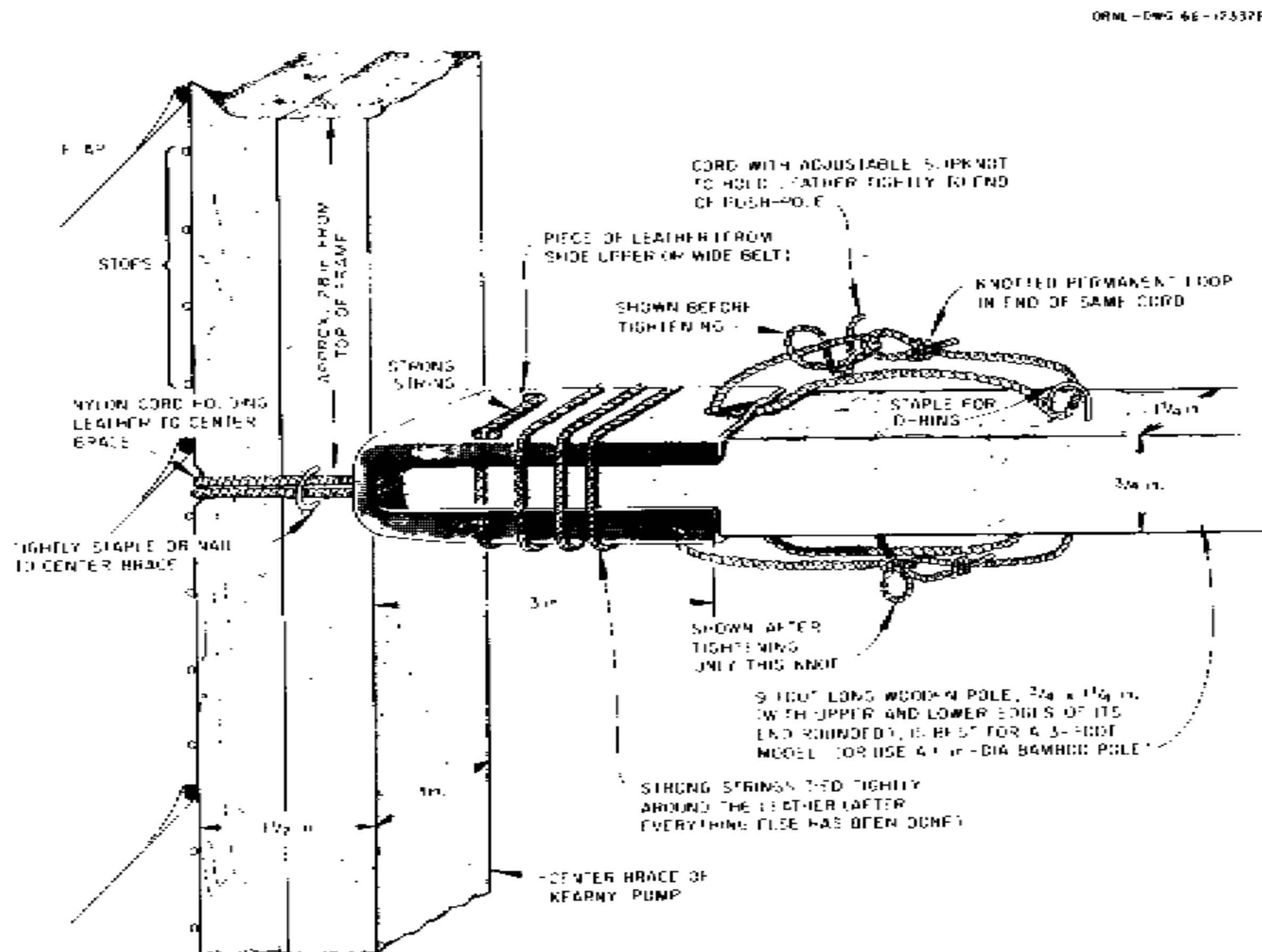
Fig. 26. Push-pole flexible connection.
