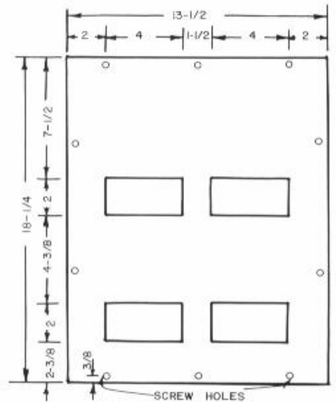
Fig. 8. Back End. Only the plywood is shown.
