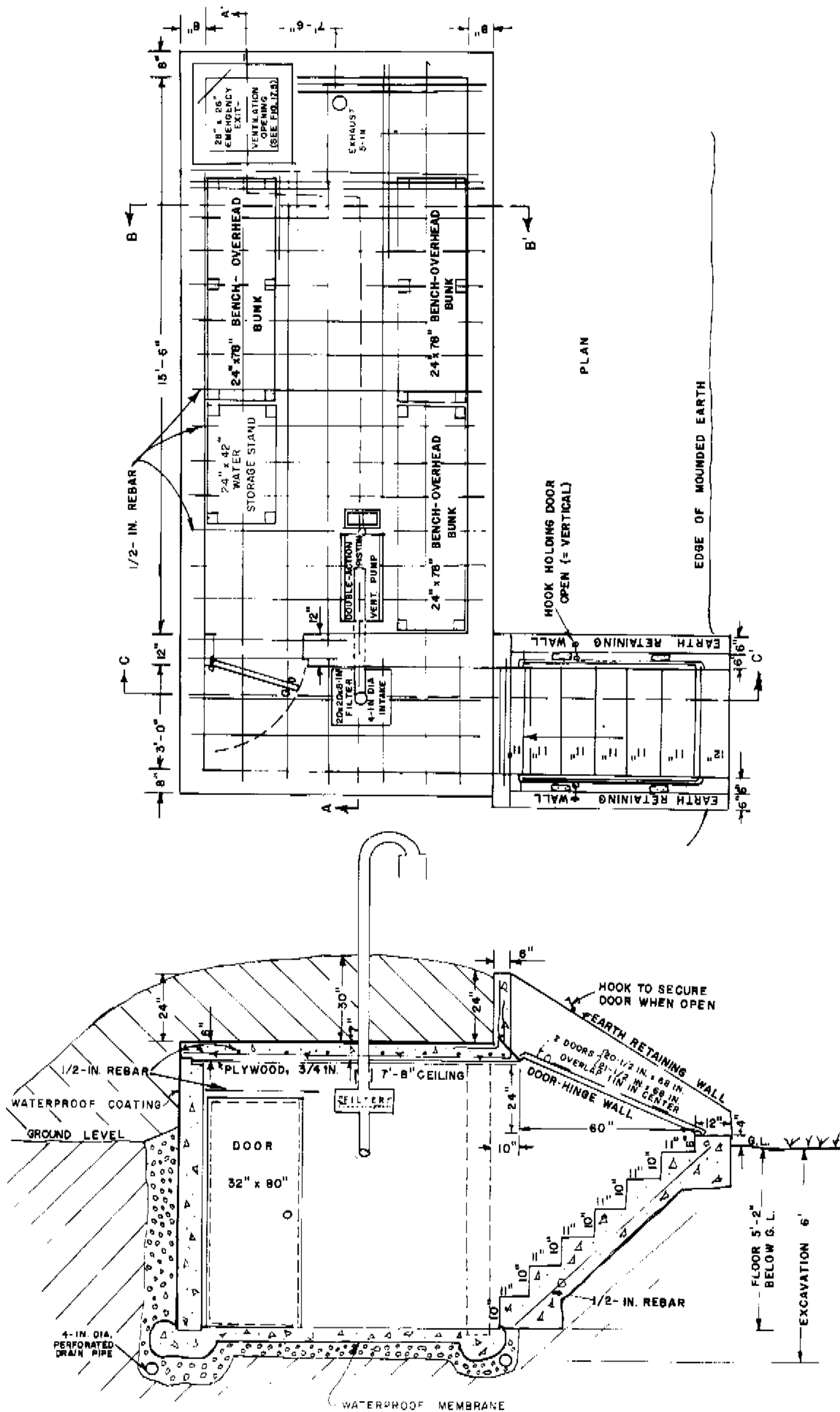
Fig. 17.1. Permanent Family Fallout Shelter for Dual Use.
