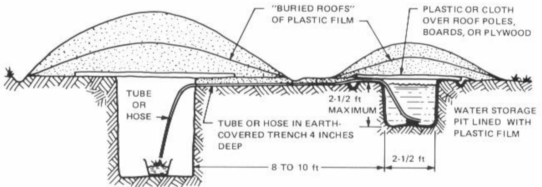
Fig. 8.7. Water siphoned into a belowground shelter.
