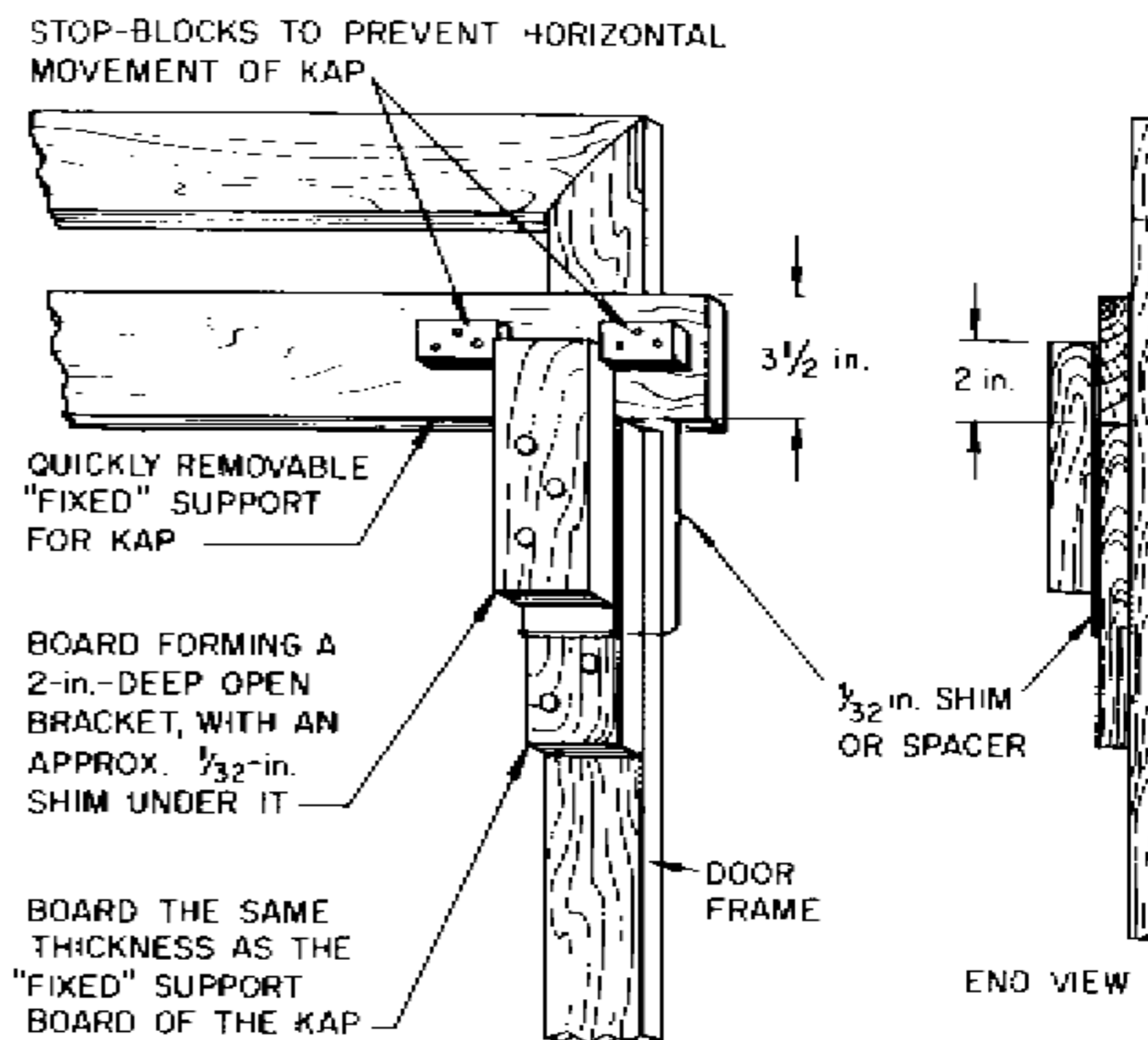
Fig. 19. Quick-removal bracket for KAP.
