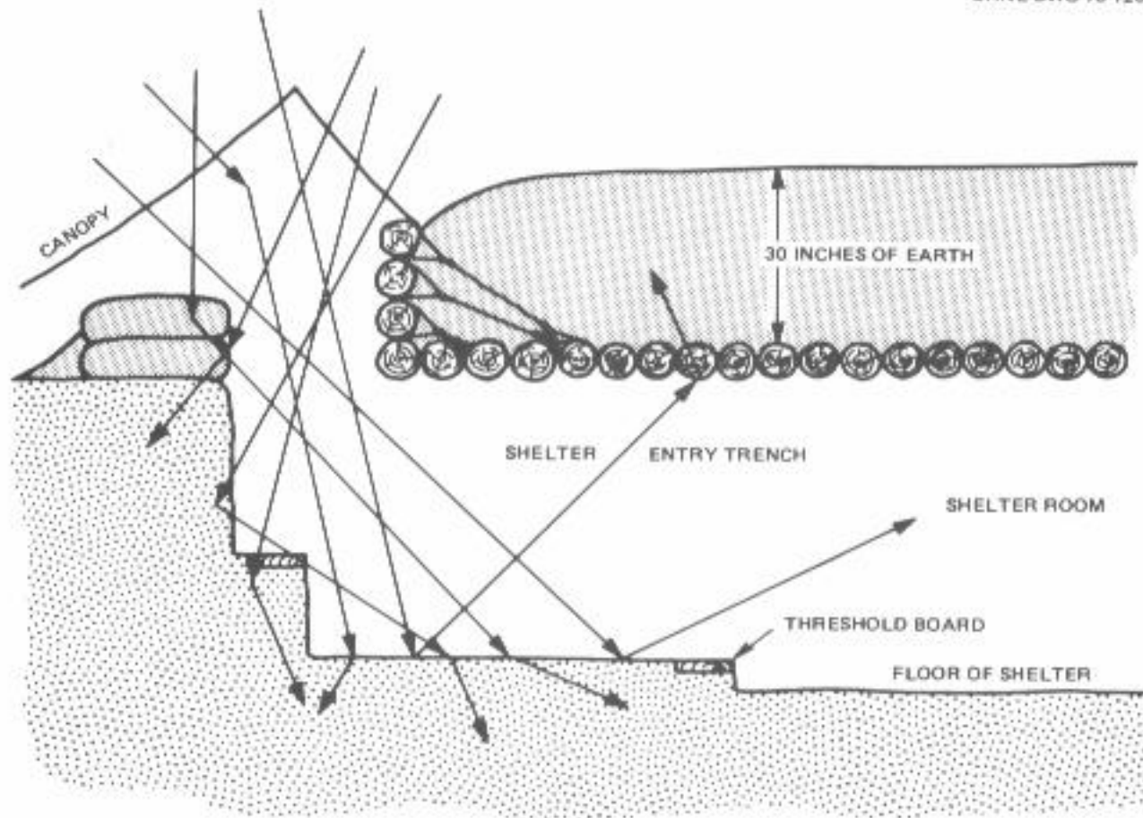
Fig. 5.5. Skyshine coming into a shelter through a vertical entry would be mostly absorbed while turning into and traveling down the entryway trench.
