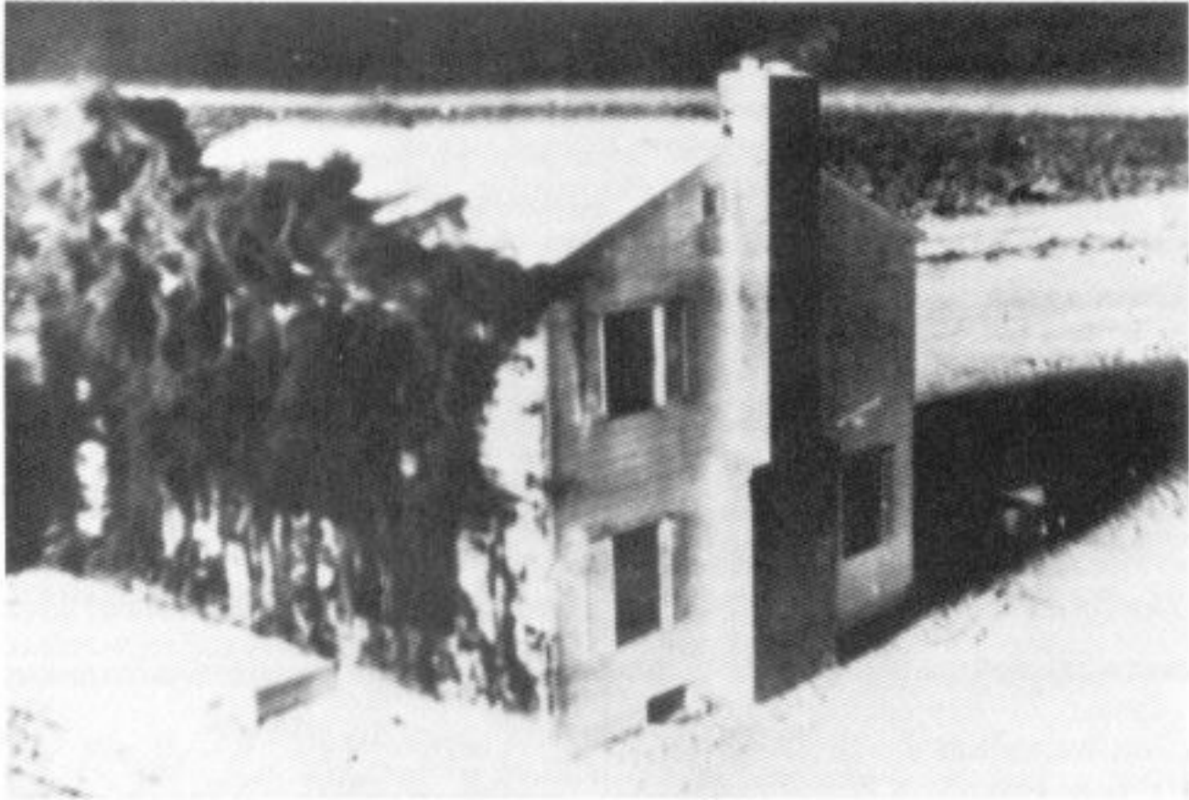
Fig. 7.1. Heat radiation charred the paint on this house, which had been painted white to reflect heat rays. The charring instantaneously produced the smoke. However, precautions had been taken to prevent this typical U.S. house from being destroyed by fire, because the test was made to enable engineers to study the effects of blast, rather than fire. The house was demolished by the 5-psi overpressure blast that struck seconds later, but it did not burn.
