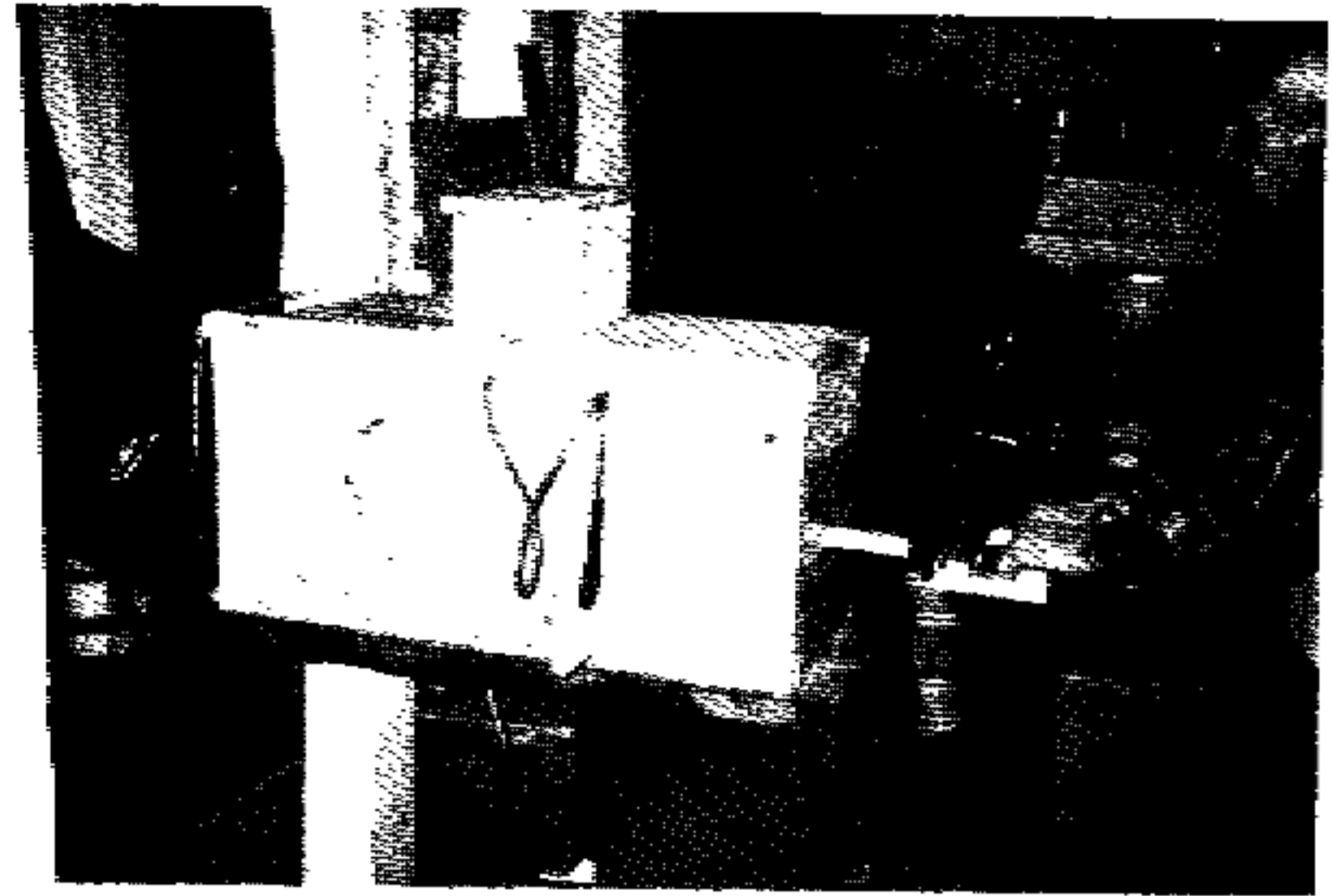
Fig. 1. Plywood Double-Action Piston Pump, with manometer attached for tests.
