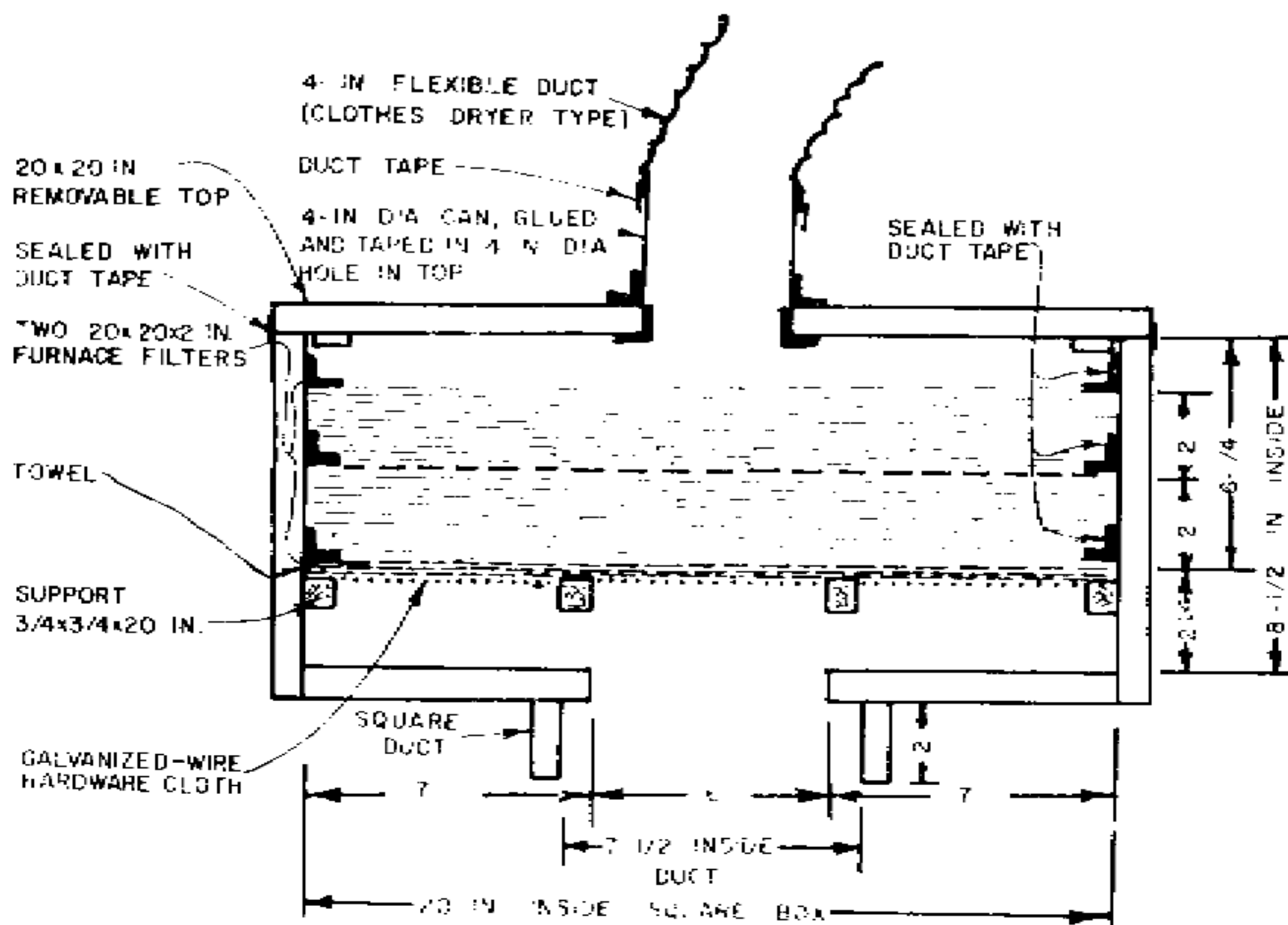
Homemade Filter To Fit On Plywood Double-Action Piston Pump, and To Be Connected to a 4-Inch-Diameter Air-Intake Pipe.
