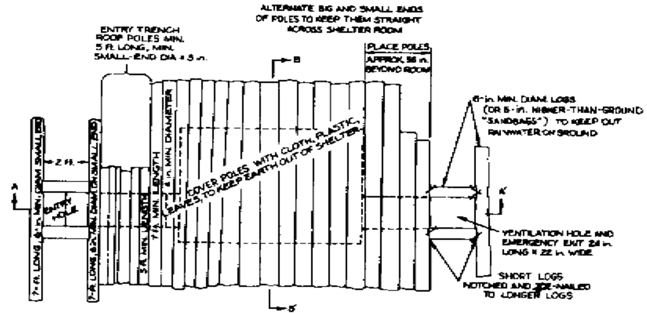
ROOF POLES = MINIMUM 7-FT LONG, 4- IN. MINIMUM DIAMETER LAID ABOUT 2 FT. PAST EACH END OF SHELTER ROOM. PLAN VIEW OF TOP OF SHELTER SHOWING PLACEMENT OF POLES FOR ROOF (EARTH FILL NOT SHOWN)
