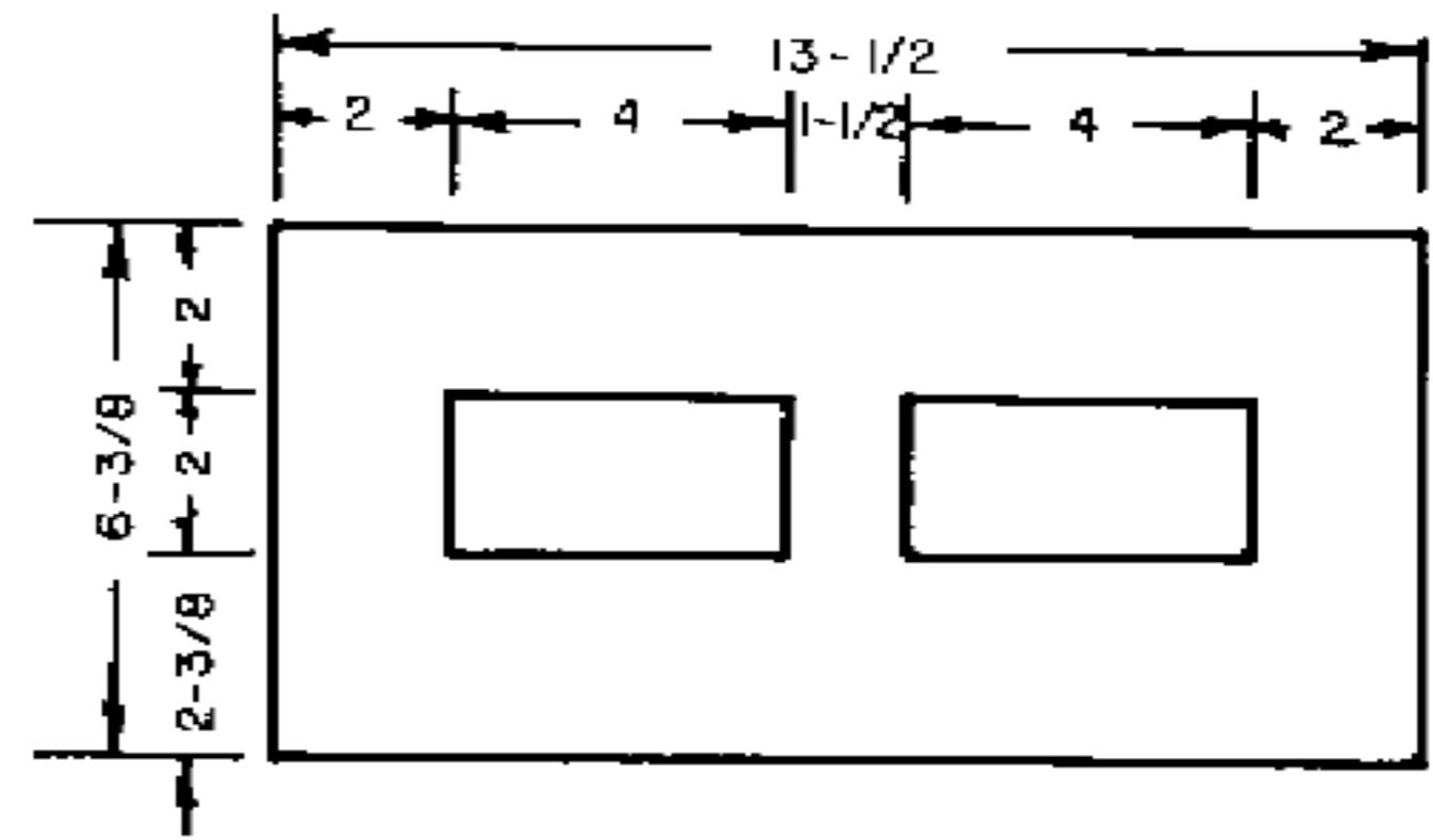
Fig. 10. Fixed Part of Front End, Unfinished. Only the plywood is shown.
