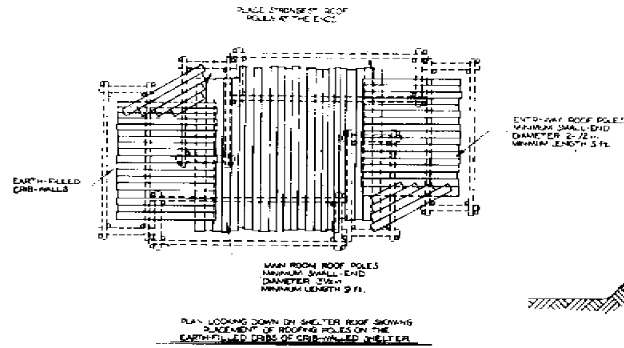
Fig. A.6. Aboveground, Crib-Walled Shelter.
