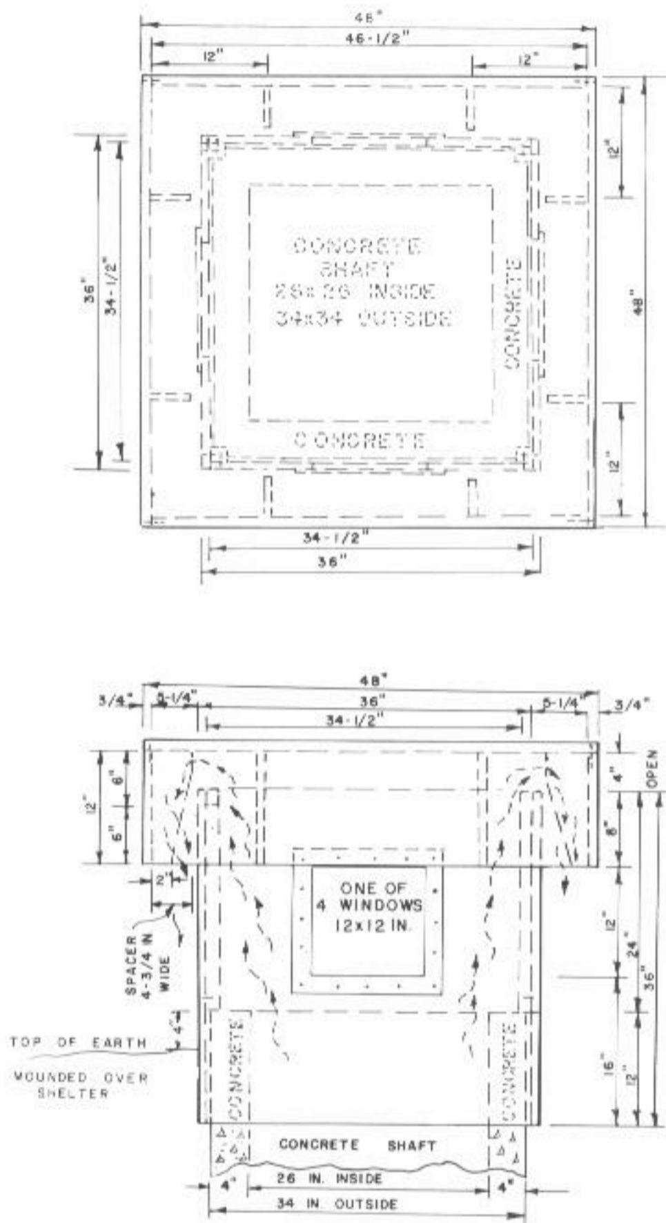
Fig. F.2. Plan and Side View of Multi-Purpose Emergency Exit Housing, on a Square Emergency Exit with 34 x 34-Inch Cross-Sectional Outside Dimensions.
