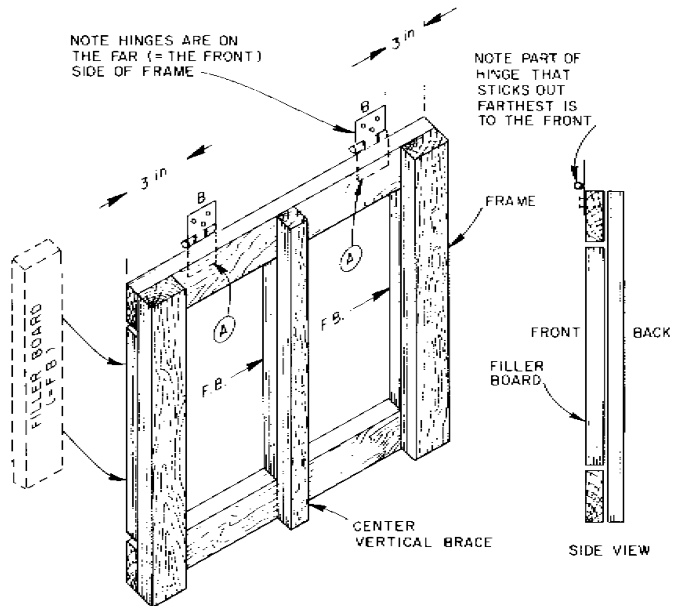
Fig. 4. Completing the frame.
