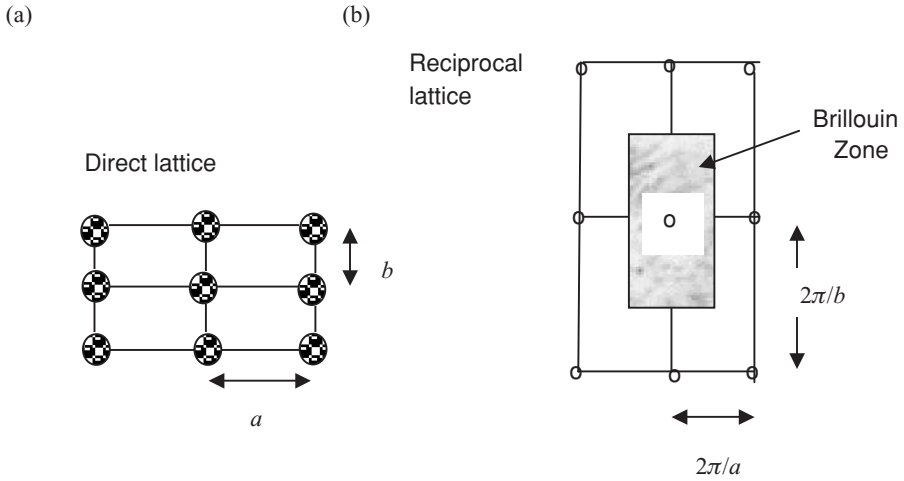
Fig. 5.2.3 (a) Rectangular lattice in real space. (b) Corresponding reciprocal lattice.
