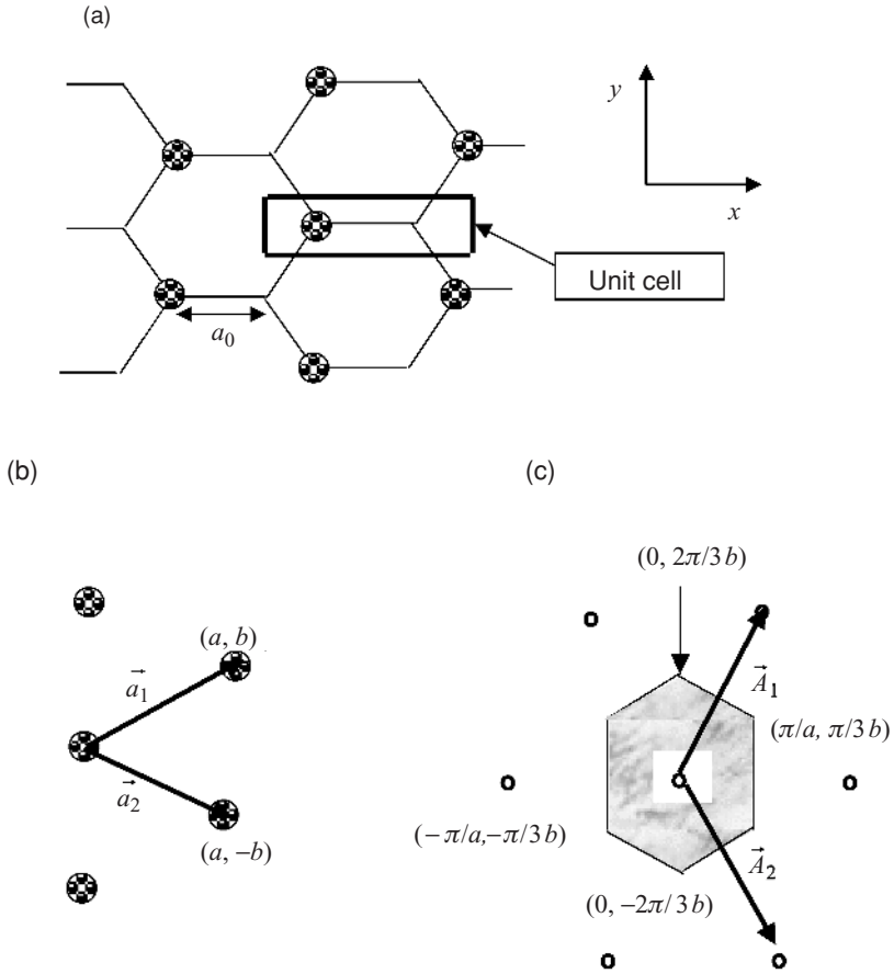
Fig. 5.2.5 (a) Arrangement of carbon atoms on the surface of graphite, showing the unit cell of two atoms. (b) Direct lattice showing the periodic arrangement of unit cells with basis vectors \vec{a}_1 and \vec{a}_2 . (c) Reciprocal lattice with basis vectors \vec{A}_1 and \vec{A}_2 determined such that \vec{A}_1 \cdot \vec{a}_1 = \vec{A}_2 \cdot \vec{a}_2 = 2\pi and \vec{A}_1 \cdot \vec{a}_2 = \vec{A}_2 \cdot \vec{a}_1 = 0 . Also shown is the Brillouin zone (shaded) obtained by drawing the perpendicular bisectors of the lines joining the origin (0, 0) to the neighboring points on the reciprocal lattice.
