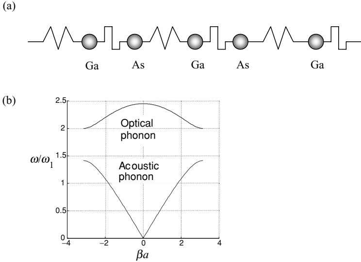
Fig. 10.4.5 (a) Snapshot of a GaAs lattice viewed along the (111) direction. (b) Dispersion law \omega/\omega_1 vs. \beta a showing acoustic and optical phonons assuming \omega_2 = \sqrt{2}\omega_1 .
