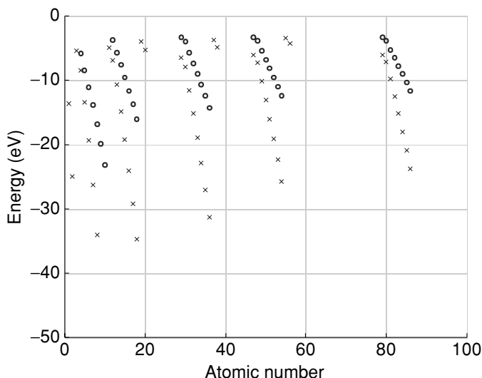
Fig. 3.3.1 Energy of the outermost s (×) and p levels (◦) of the first 86 elements of the periodic table excluding the d- and f-shell transition metals ( Z = 21\text{--}28, 39\text{--}46, \text{ and } 57\text{--}78 ). The numbers are taken from Harrison (1999) and Mann (1967).
