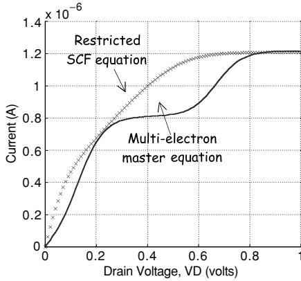
Fig. 3.4.3 Current vs. drain voltage V_D calculated assuming V_G = 0 with \mu = 0 , \varepsilon = 0.2 \text{ eV} , k_B T = 0.025 \text{ eV} , \gamma_1 = \gamma_2 = 0.005 \text{ eV} , U_L = -qV_D / 2 . The two approaches (the SCF and the multi-electron master equation) agree well for U_0 = 0.1 \text{ eV} , but differ appreciably for U_0 = 0.25 \text{ eV} , showing evidence for Coulomb blockade or single-electron charging.
