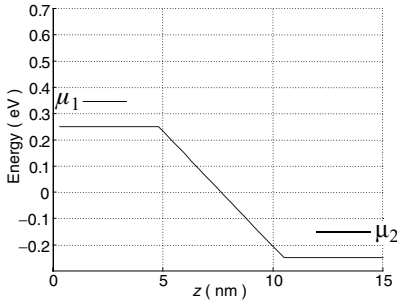
(b) Tunneling device
