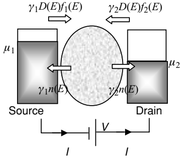
Fig. 9.1.1 Flux of electrons into and out of a channel: independent level model, see Eqs. (1.6.4)–(1.6.6).
