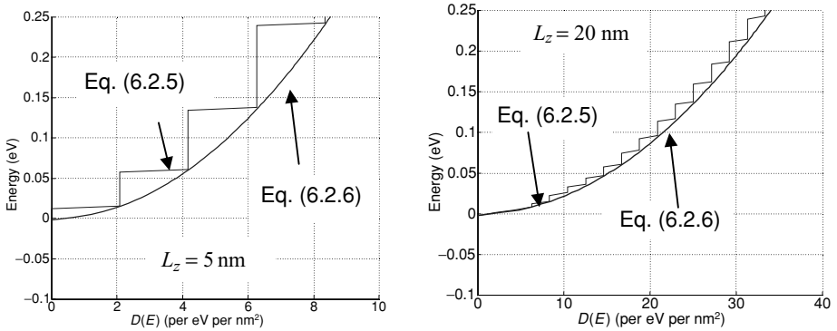
Fig. 6.2.1 Density of states D(E) for a 2D box calculated from Eq. (6.2.5) (2D with quantized subbands) and compared with that obtained from the 3D relation in Eq. (6.2.6). As the width L_z of the box is increased from 5 to 20 nm, the DOS approaches the 3D result (the conduction band effective mass m_c is assumed equal to the free electron mass m ).
