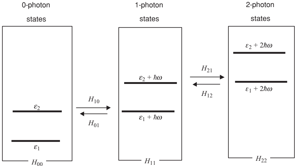
Fig. 10.1.3 In the multi-particle viewpoint, the electron–photon coupling causes transitions between |2, N\rangle and |1, N-1\rangle , which are degenerate states of the composite system.
