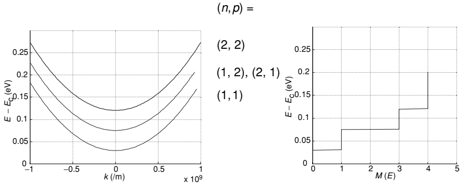
Fig. 6.3.3 Energy dispersion relation showing the four lowest conduction band subbands (see Eq. (6.3.4)) in a rectangular wire with L_y = L_z = 10 \text{ nm} , m_c = 0.25m .
