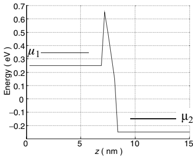
(c) Resonant tunneling device
