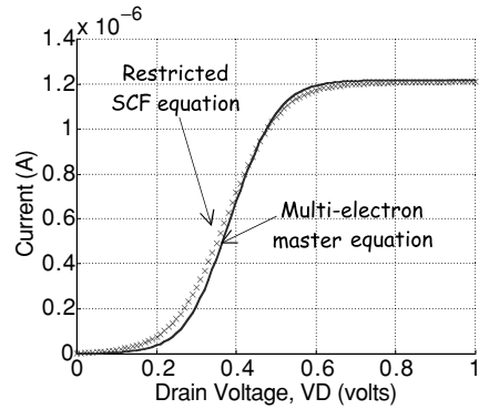
Fig. 3.4.3 Current vs. drain voltage V_D calculated assuming V_G = 0 with \mu = 0 , \varepsilon = 0.2 \text{ eV} , k_B T = 0.025 \text{ eV} , \gamma_1 = \gamma_2 = 0.005 \text{ eV} , U_L = -qV_D / 2 . The two approaches (the SCF and the multi-electron master equation) agree well for U_0 = 0.1 \text{ eV} , but differ appreciably for U_0 = 0.25 \text{ eV} , showing evidence for Coulomb blockade or single-electron charging.
