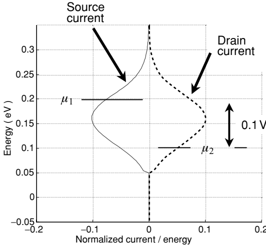
Fig. 11.3.1 Normalized current per unit energy \tilde{I}_i(E) in a one-dimensional wire with phase-breaking elastic scattering.
