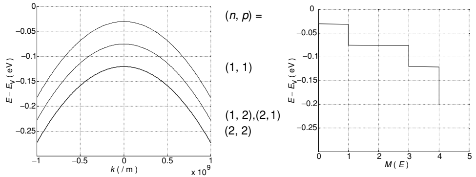
Fig. 6.3.4 Energy dispersion relation showing the four lowest valence band subbands (see Eqs. (6.3.5) and (6.3.6)) in a rectangular wire with L_y = L_z = 10 \text{ nm} , m_v = 0.25m .
