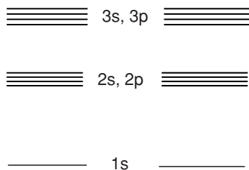
Fig. 4.1.5 Eigenstates of a \text{H}_2 molecule when the atoms are not too close. All these states could be used as basis functions for a more accurate treatment of the hydrogen molecule.
