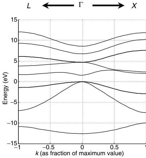
Fig. 5.3.2 E(\vec{k}) calculated by finding the eigenvalues of the matrix in Eq. (5.3.3) for each value of \vec{k} along the \Gamma - X (that is, from \vec{k} = 0 to \vec{k} = \hat{x} 2\pi/a ) and \Gamma - L (that is, from \vec{k} = 0 to \vec{k} = (\hat{x} + \hat{y} + \hat{z})\pi/a ) directions. The former is plotted along the positive axis and the latter along the negative axis. Only eight (rather than ten) lines are visible because some are degenerate.
