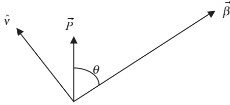
Fig. 10.2.3 Emission of photon with wavevector \vec{\beta} and polarization \hat{v} by an atomic transition with an equivalent dipole moment \vec{P} .
