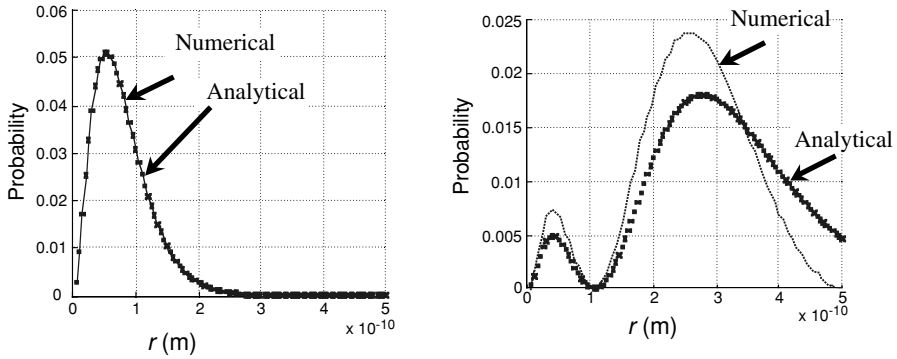
Fig. 2.3.6 Radial probability distribution |f(r)|^2 corresponding to the two lowest eigenvalues ( -13.56\text{ eV} and -2.96\text{ eV} ) for l = 0 (which correspond to the 1s and 2s levels). The dots show the analytical result (Eqs. (2.1.10a, b)) while the solid curve denotes the numerical result obtained using a lattice with 100 points spaced by a = 0.05\text{ \AA} .
