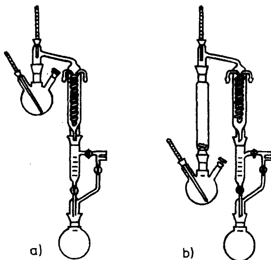
Fig. 136 Apparatus from standard parts for: a) simple distillation, b) rectified distillation
