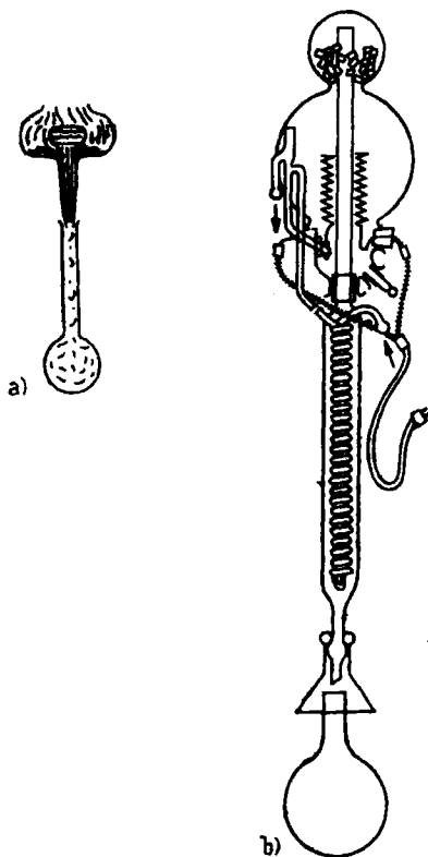
Fig. 2b) Vacuum still for mercury with collecting collar for the distillate (20th century)
