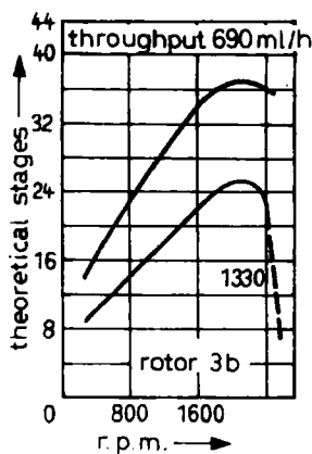
Fig. 288 Dependence of the number of stages on the load and the speed of rotation for Jost's rotating-cylinder column with rotor 3 b
