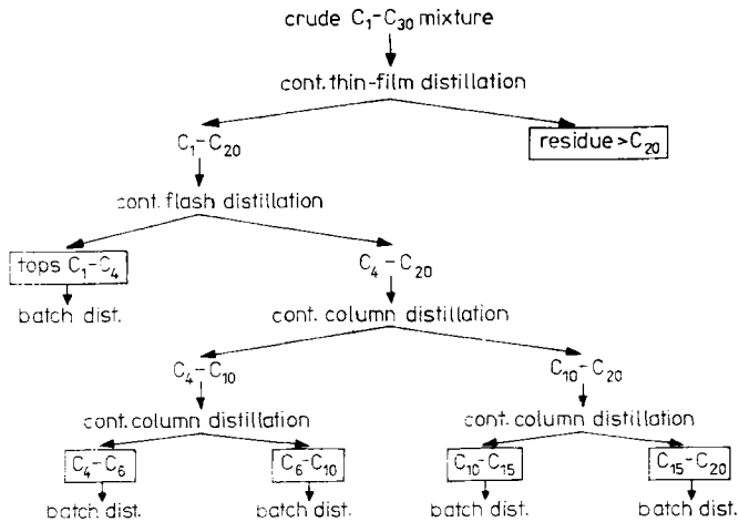
Fig. 163 Distillation scheme for a C_1-C_{20} multicomponent mixture
