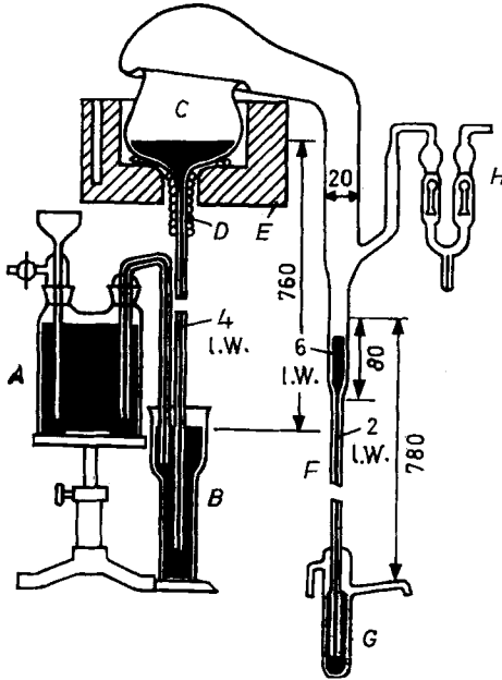
Fig. 184 Apparatus for the distillation of mercury (dimensions in mm)
