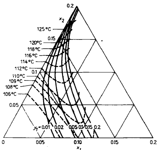
Fig. 230 Isobaric equilibrium HCl-H 2 SO 4 -H 2 O at 750 torr: x_2 molar fraction of H 2 SO 4 in liquid phase — lines of constant vapour composition - - - isotherms
