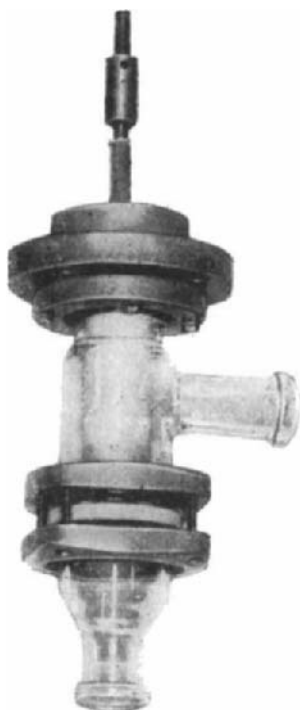
Fig. 247 Precision valve of glass with PTF spindle for the control of liquid and gas flow (face and tube diameter d = 4 and 7 mm)
