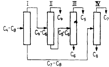
Fig. 86 Scheme for the continuous distillation of the C_4 – C_8 n-fatty acids C_4 , C_5 and C_7 collected as distillates, C_6 and C_8 as bottom products
