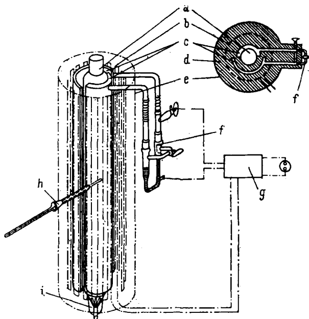
Fig. 368 Automatic control of the column jacket temperature according to the inner column temperature
