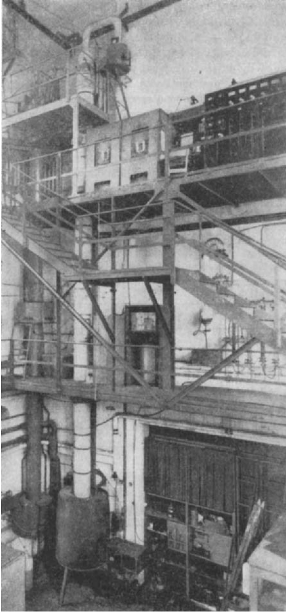
Fig. 160 The author's still for enriching H 2 18 O
