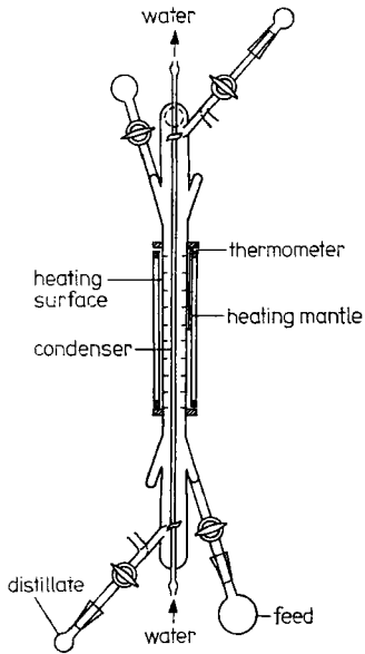
Fig. 132 Micro-form of molecular distillation apparatus after Breger (falling film principle) for less than 4 g charge
