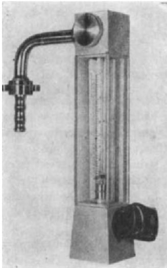
Fig. 395 Laboratory flow meter, type SW 16.1 Measuring range I: 0.5 to 3.0 l/min; range II: 3.0 to 12.0 l/min
