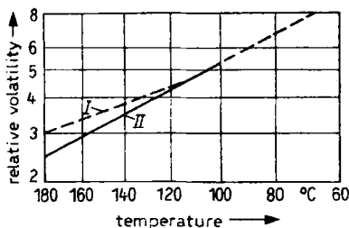
Fig. 215 Relative volatility of the test mixture EHP/EHS EHP: K p 0.5 torr 183–184°C; EHS: K p 0.5 torr 199–202°C I: From an equilibrium apparatus of flask type II: from an apparatus operating on the falling-film principle
