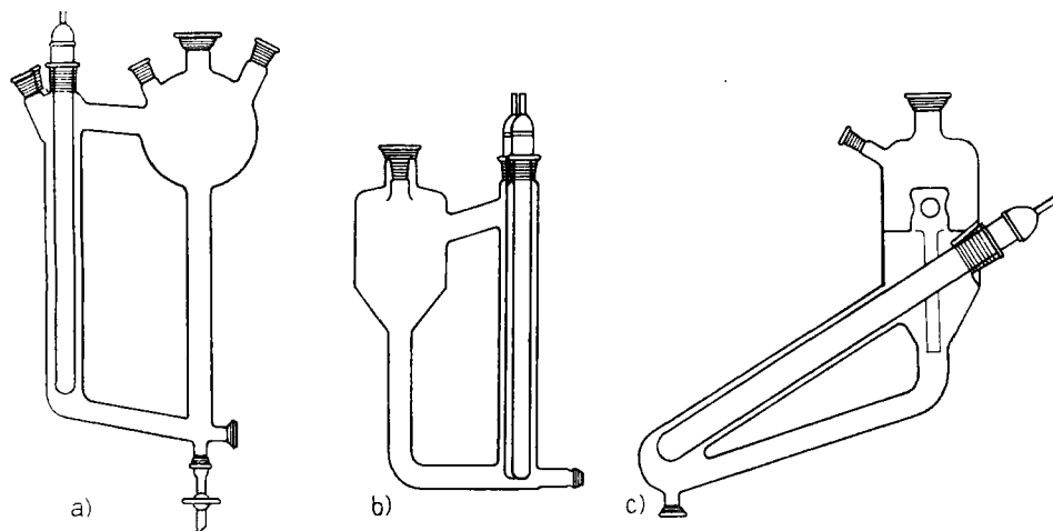
Fig. 338 Circulation heaters with vertical and inclined immersion heaters a) "Normschliff" model b) "Normag" model c) "Schmidt" model
