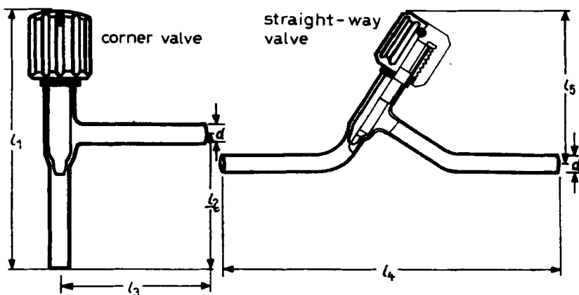
Fig. 247 Precision valve of glass with PTF spindle for the control of liquid and gas flow (face and tube diameter d = 4 and 7 mm)
