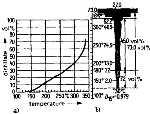
Fig. 118 Boiling point diagram (a) and surface diagram (b) for a shale oil
