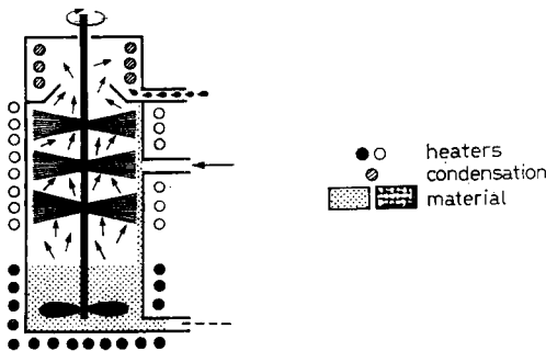
Fig. 201 Fractionating brush
