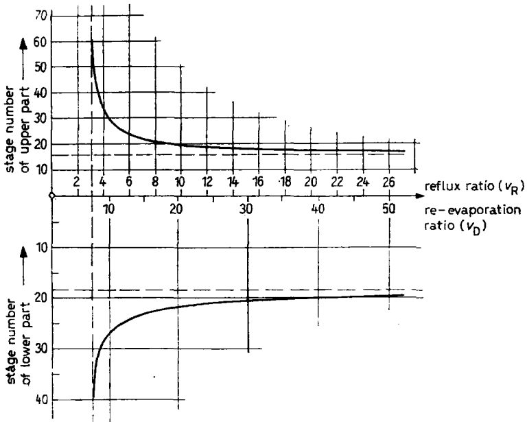
Fig. 121 Data for a continuous distillation [251] with x = 1.5 ; x_Z = 65 \text{ mol\%} ; x_E = 99.9 \text{ mol\%} ; x_A = 0.1 \text{ mol\%}
