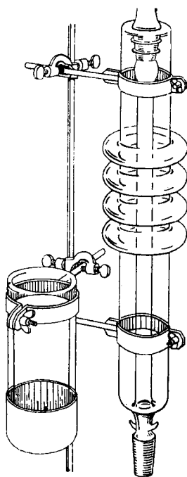
Fig. 423 Ring clamps
