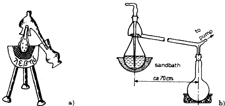
Fig. 2a) Glass distillation apparatus with sand or water bath (2nd century A.D.)
