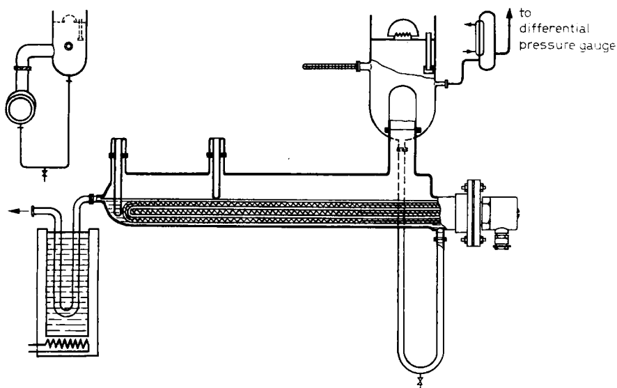
Fig. 339 Labodest horizontal circulation heater with separate pipes for vapour and reflux (Stage)
