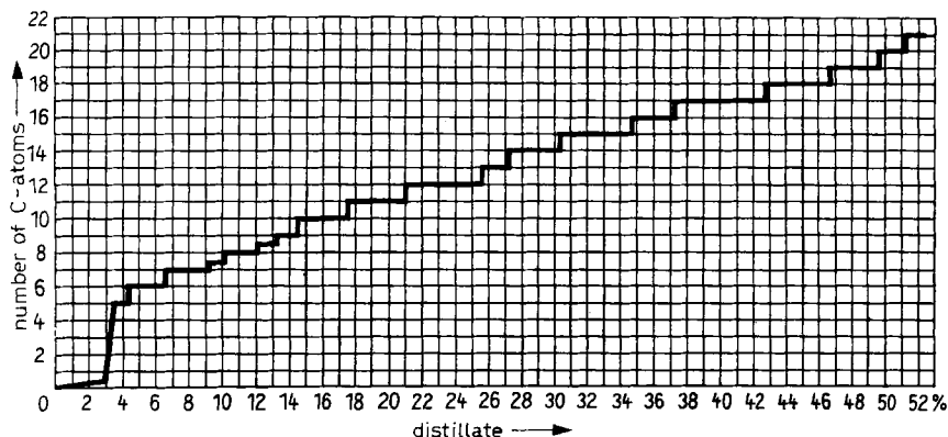
Fig. 116 Step diagram of the distillation of a crude fatty acid mixture
