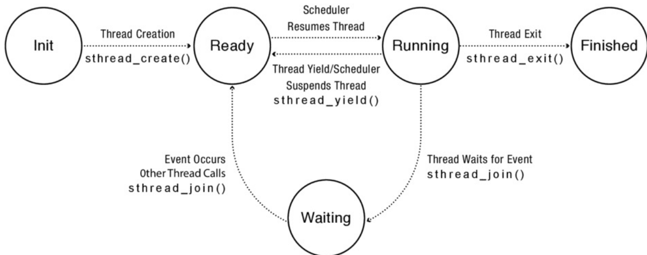
Figure 4.9: The states of a thread during its lifetime.
