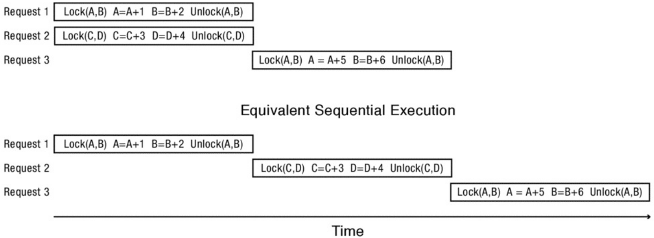
Figure 6.13: Locking multiple objects using an acquire-all/release-all pattern results in a serializable execution that is equivalent to an execution where requests are executed sequentially in some order.
