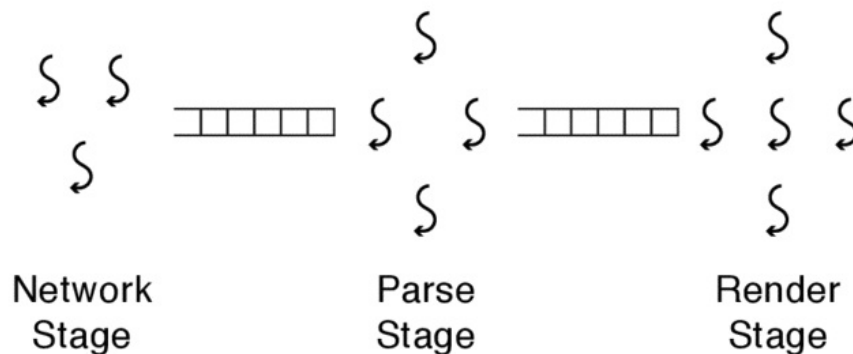
Figure 6.2: A multi-stage server based on the ownership pattern. In the first stage, one thread exclusively owns each network connection. In later stages, one thread parses and renders a given object at a time.
