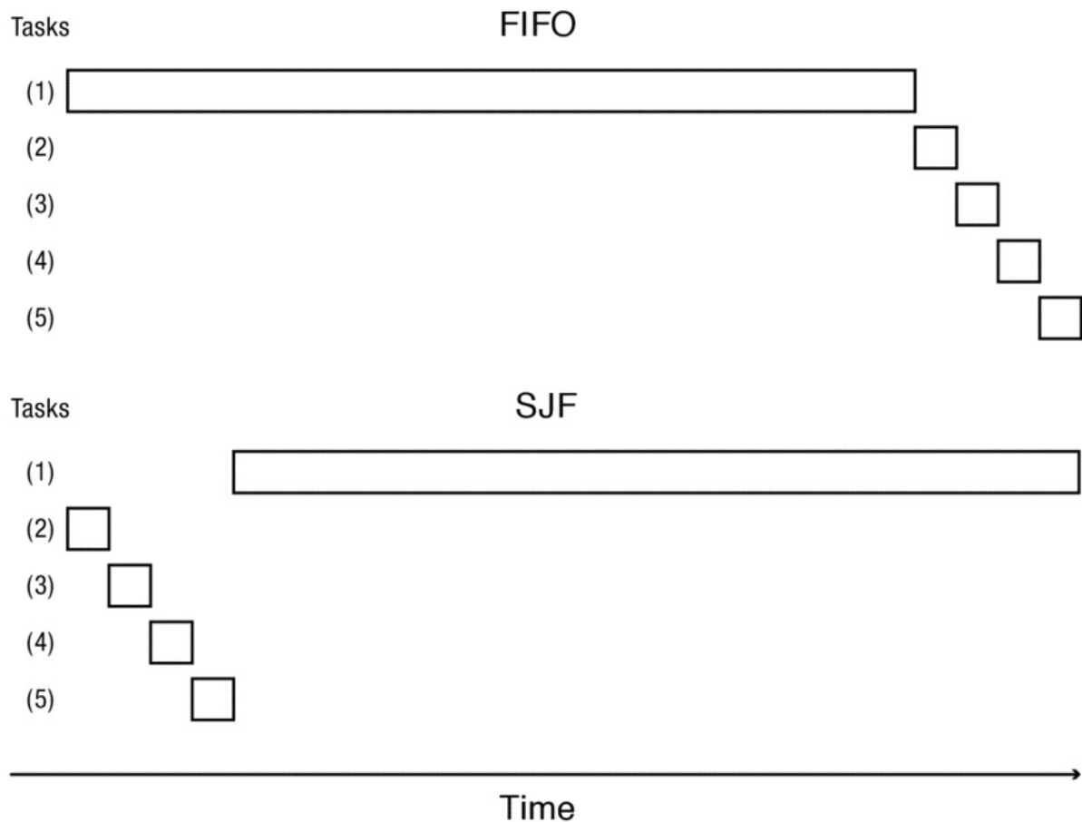
Figure 7.1: Completion times with FIFO (top) and SJF (bottom) scheduling when several short tasks (2-5) arrive immediately after a long task (1).
