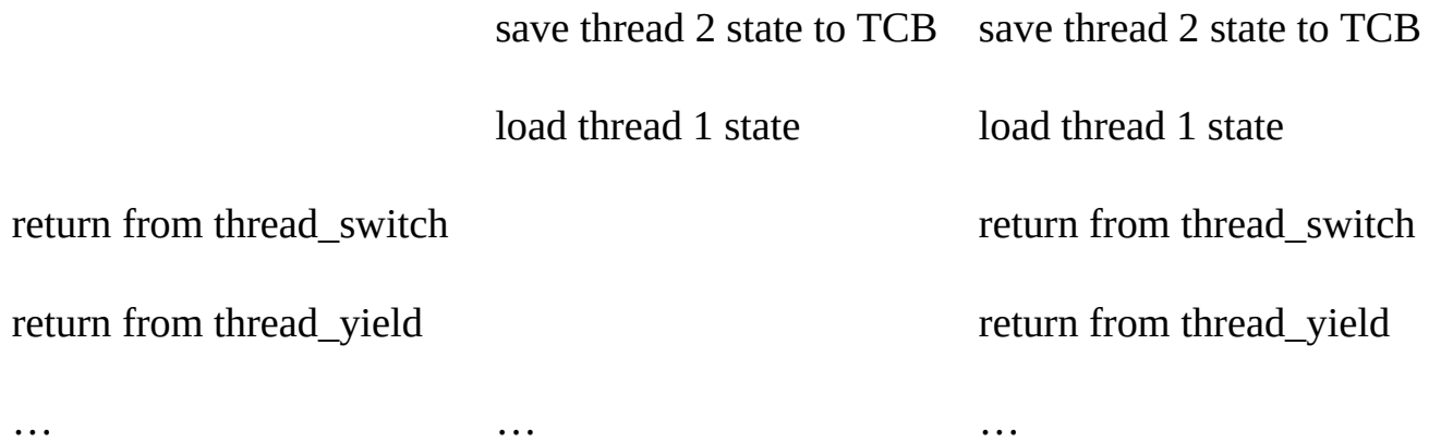
Figure 4.15: Interleaving of instructions when two threads loop and call thread_yield() .
