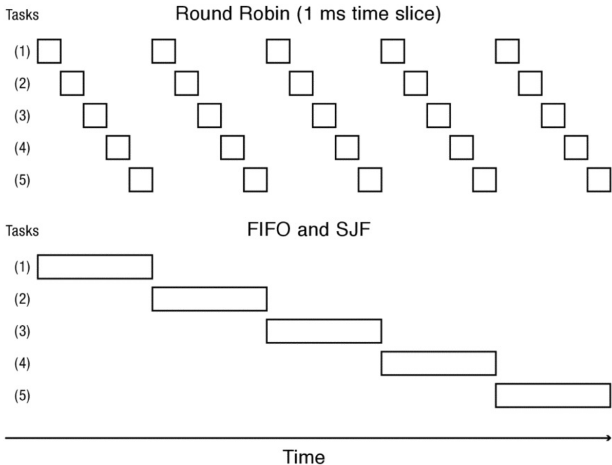
Figure 7.3: Completion times with Round Robin (top) versus FIFO and SJF (bottom) when scheduling equal length tasks.
