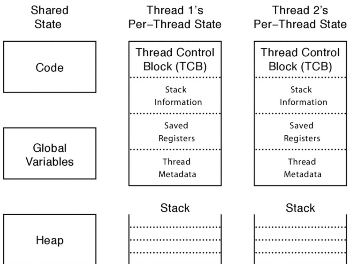
Figure 4.8: A multi-threaded process or operating system kernel has both per-thread state and shared state . The thread control block stores the per-thread state: the current state of the thread's computation (e.g., saved processor registers and a pointer to the stack) and metadata needed to manage the thread (e.g., the thread's ID, scheduling priority, owner, and resource consumption). Shared state includes the program's code, global static variables, and the heap.
