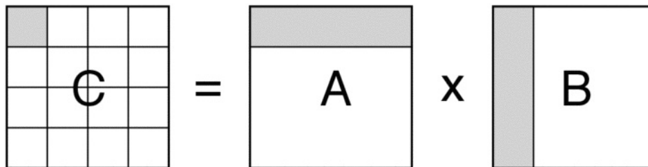
Figure 4.19: Matrix multiplication.
